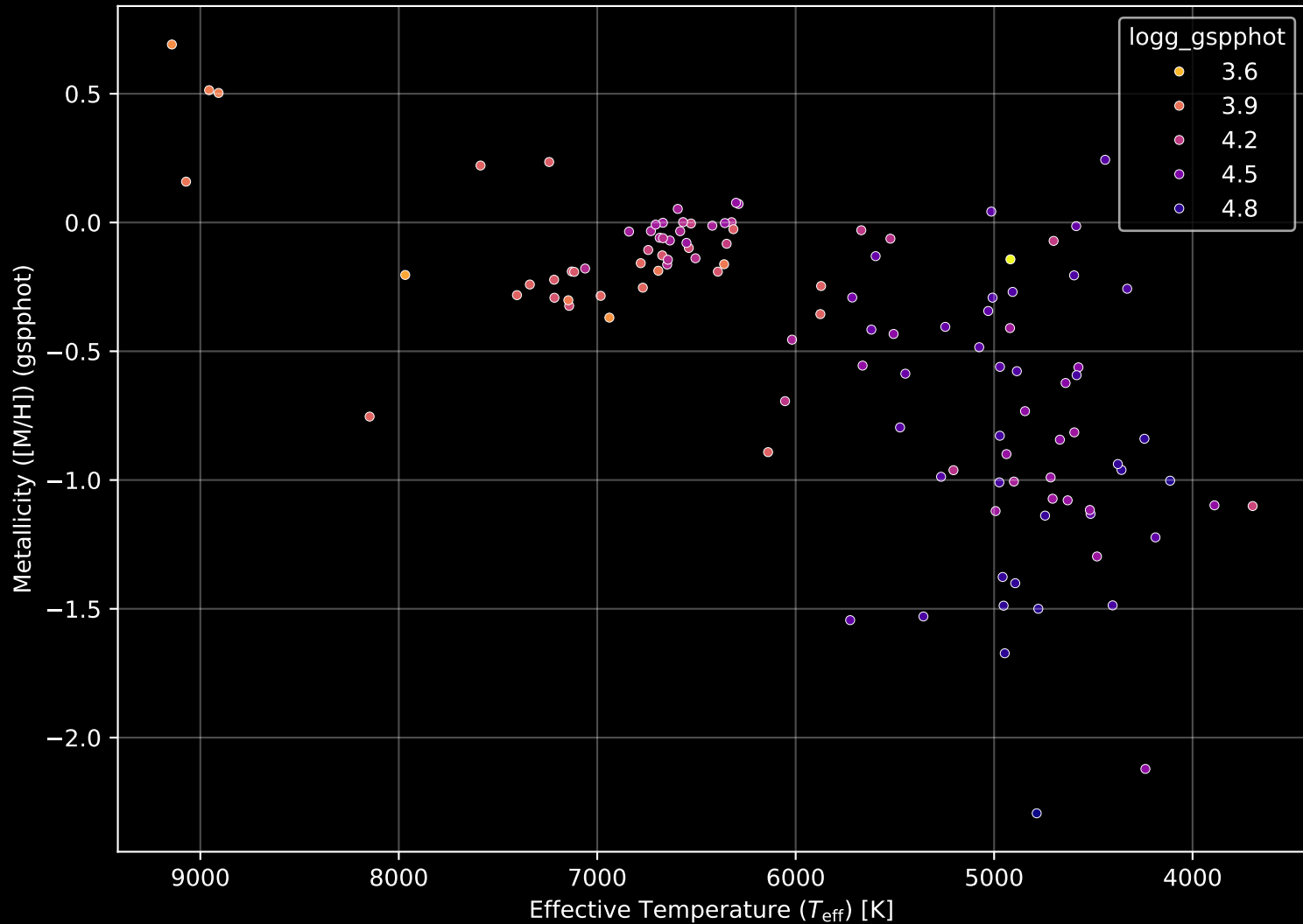
Gaia Cluster: [Gulliver_37] Stellar Population Parameters (n= 115)
