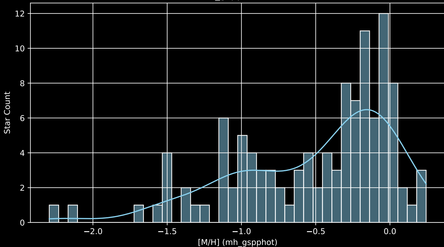
Gaia Cluster: [Gulliver_37 [M/H] (mh_gspphot) (n= 112)
