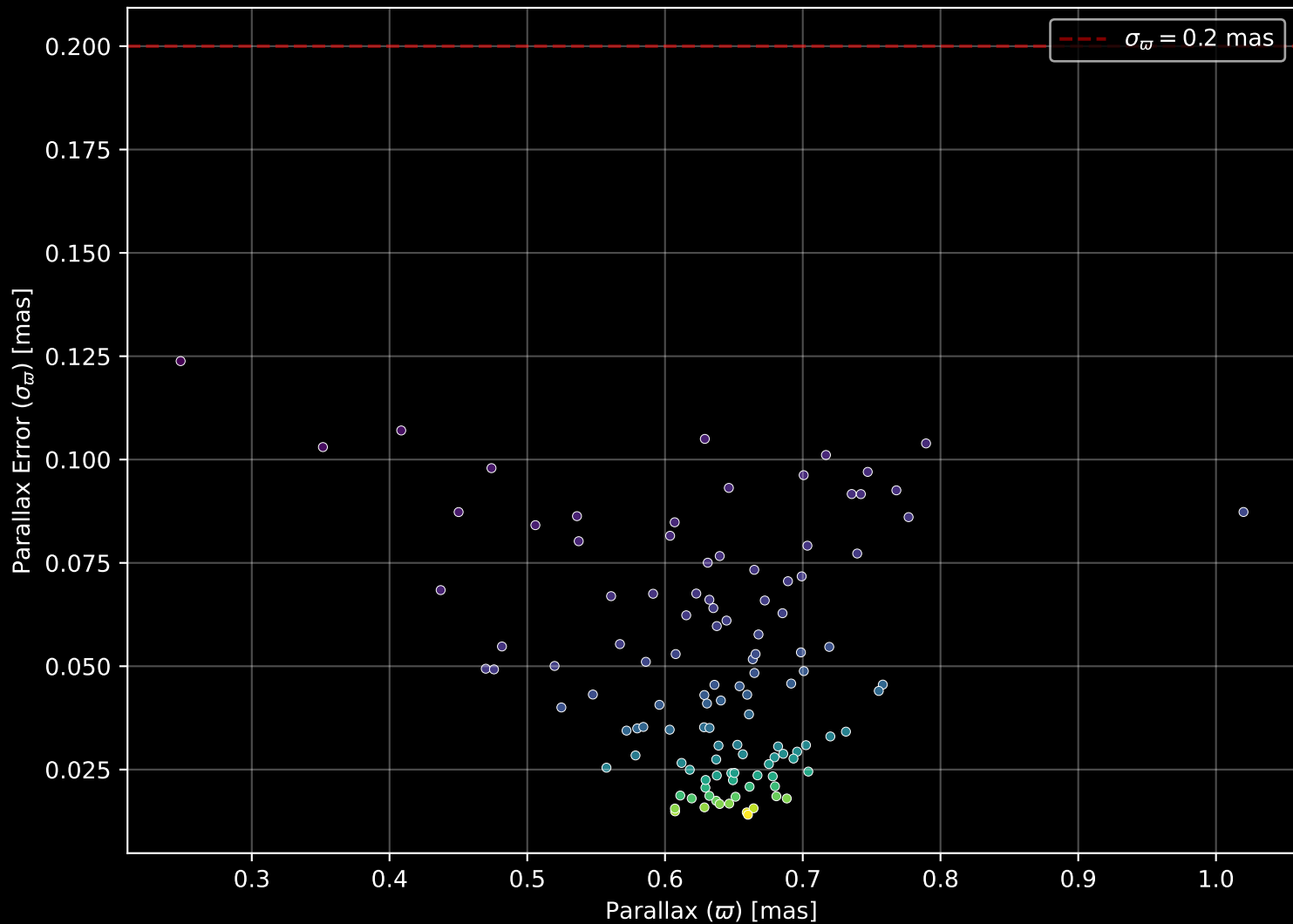
Gaia Cluster: [Gulliver_37] Parallax Quality (n= 115)
