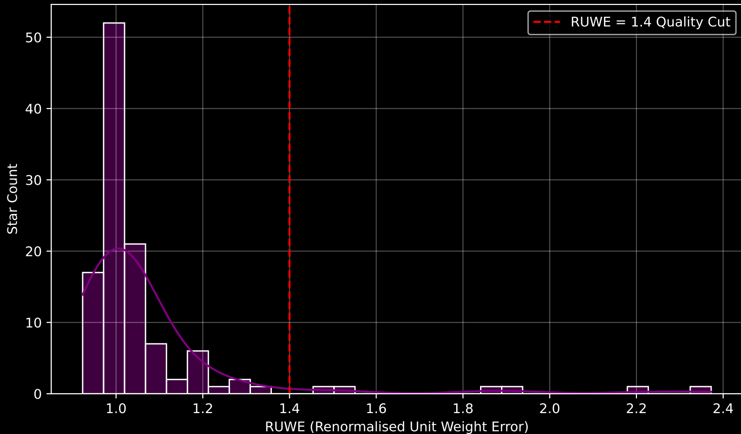
Gaia Cluster: [Gulliver_37] RUWE Distribution (n= 115)
