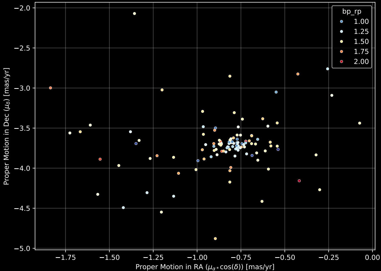
Gaia Cluster: [Gulliver_37] Proper Motion Diagram (n= 115)
