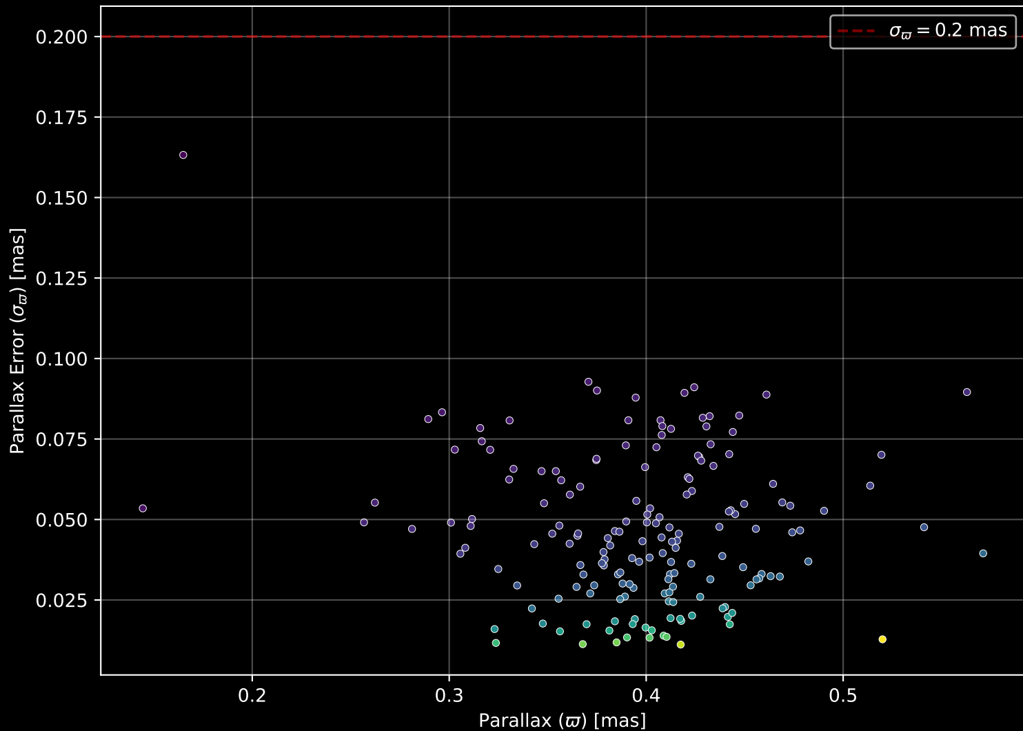
Gaia Cluster: [Gulliver_38] Parallax Quality (n= 170)
