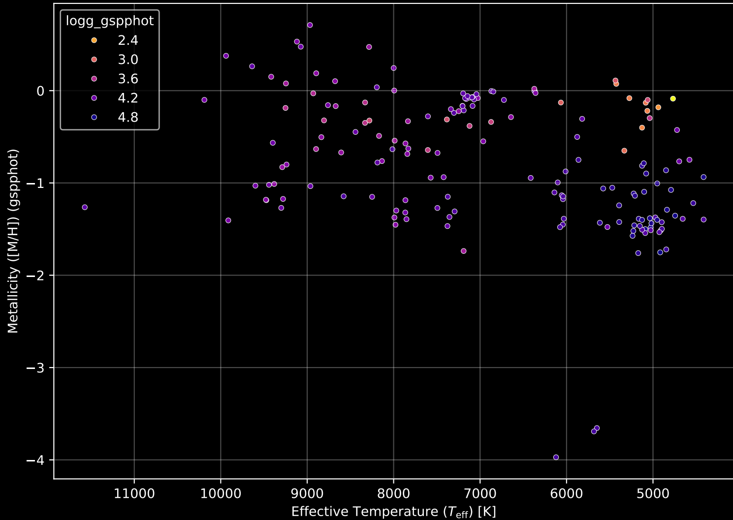
Gaia Cluster: [Gulliver_38] Stellar Population Parameters (n= 170)
