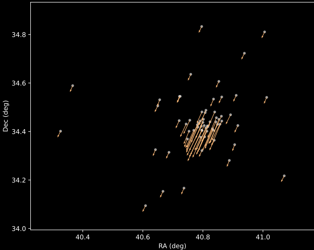
Gaia DR3 Cluster 3 Proper Motion Vectors (n=63)
