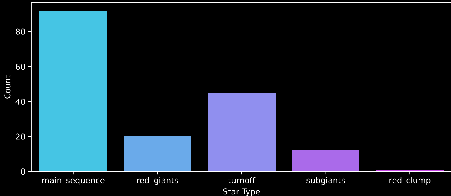
Gaia Cluster: [Gulliver_38] Count plot of Star Type
