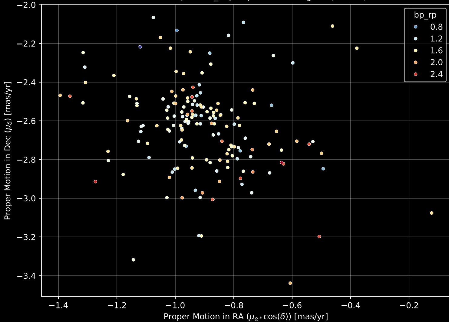
Gaia Cluster: [Gulliver_38] Proper Motion Diagram (n= 170)
