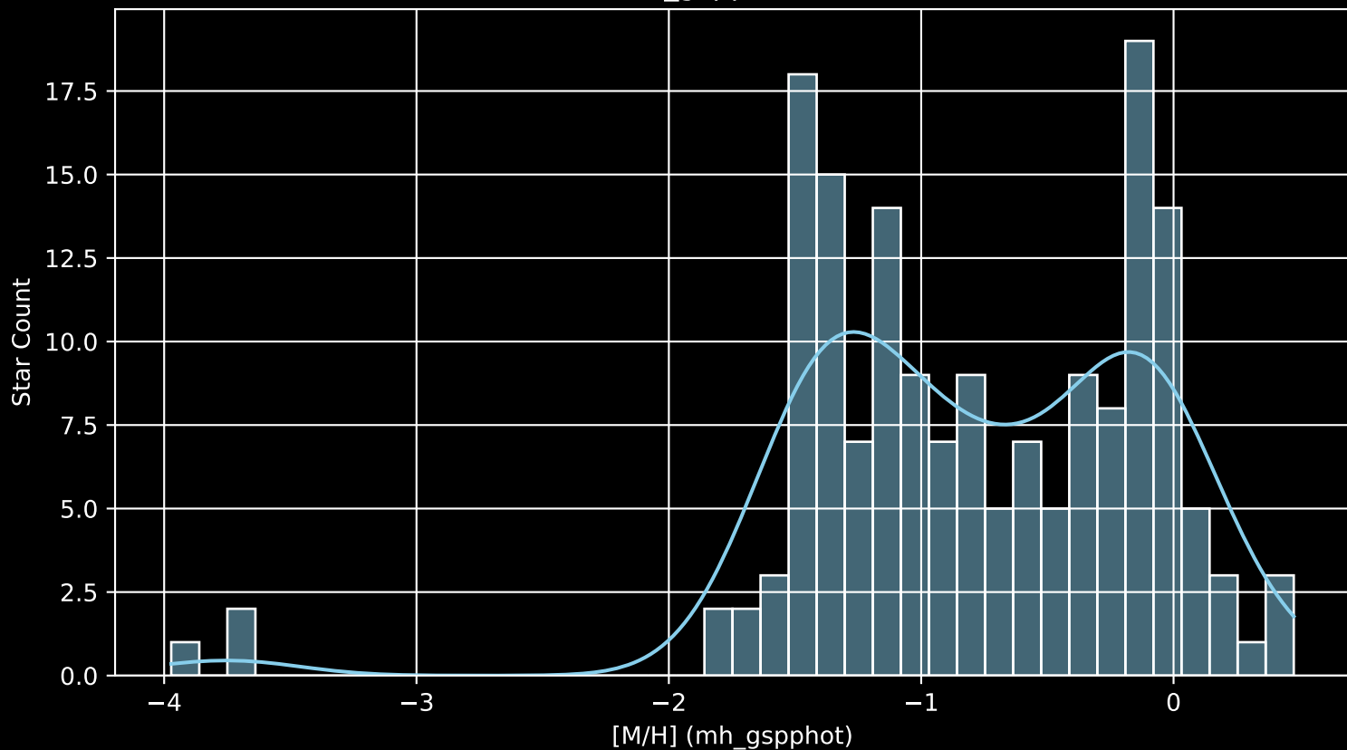
Gaia Cluster: [Gulliver_38 [M/H] (mh_gspphot) (n= 168)
