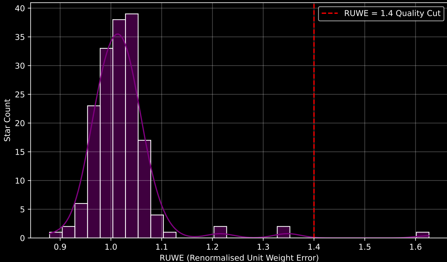
Gaia Cluster: [Gulliver_38] RUWE Distribution (n= 169)
