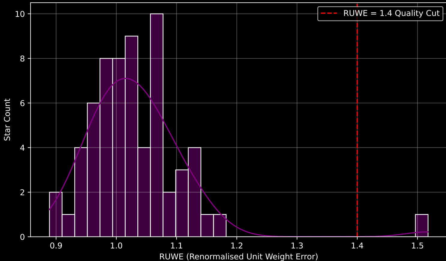
Gaia Cluster: [Gulliver_41] RUWE Distribution (n= 64)
