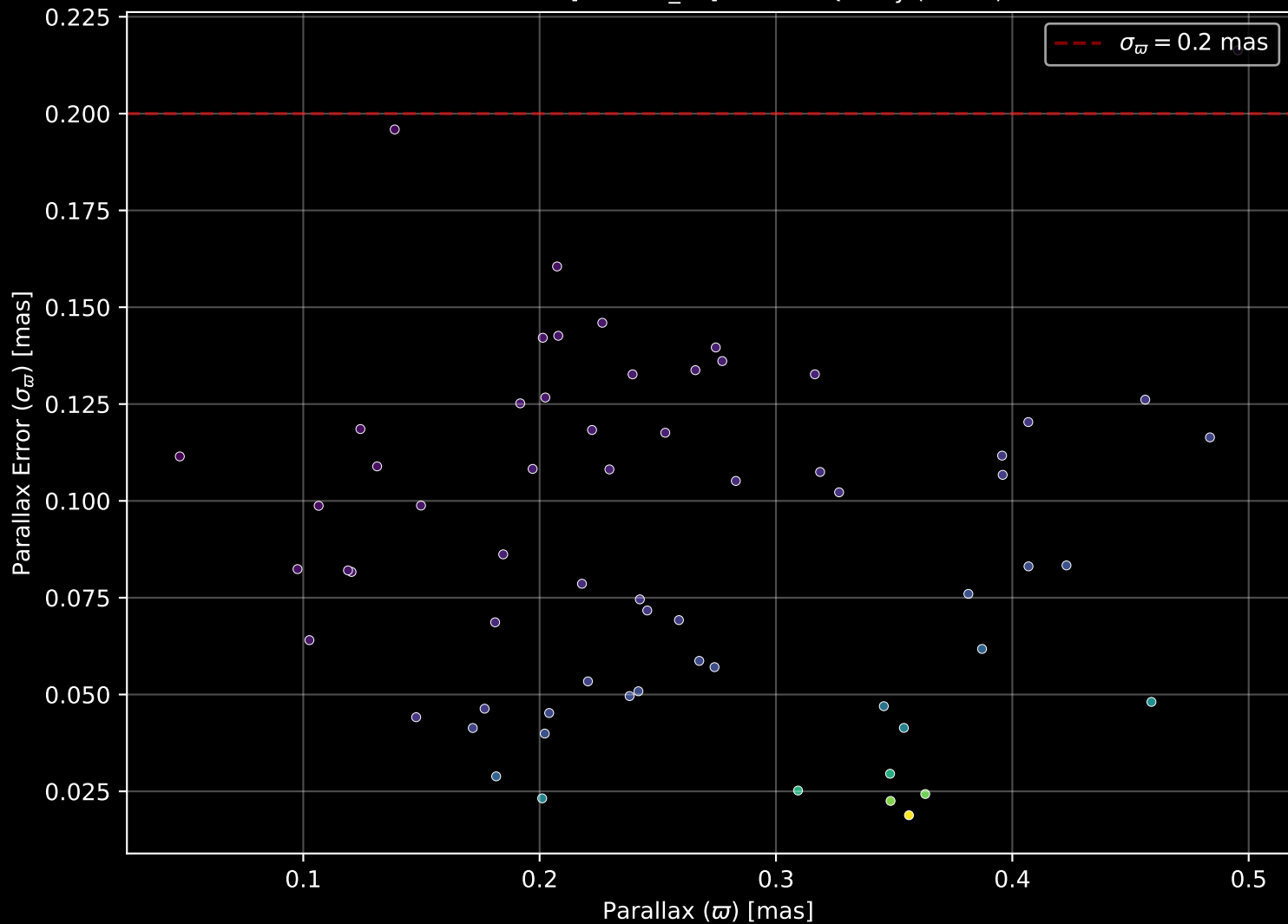
Gaia Cluster: [Gulliver_41] Parallax Quality (n= 64)
