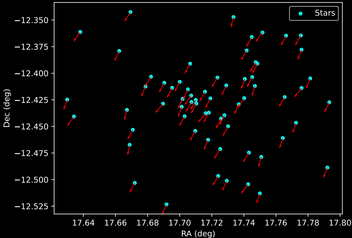
Gaia Cluster: [Gulliver_41] Proper Motion Vectors for Gaia Star Field (n= 64)
