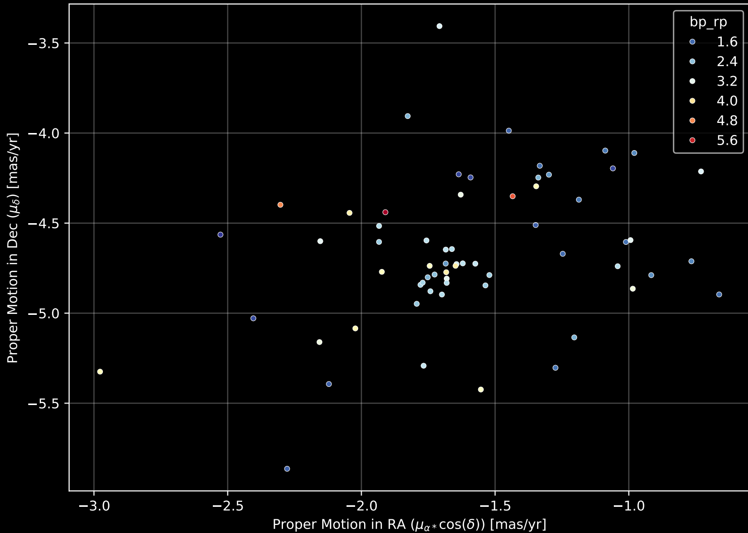
Gaia Cluster: [Gulliver_41] Proper Motion Diagram (n= 64)
