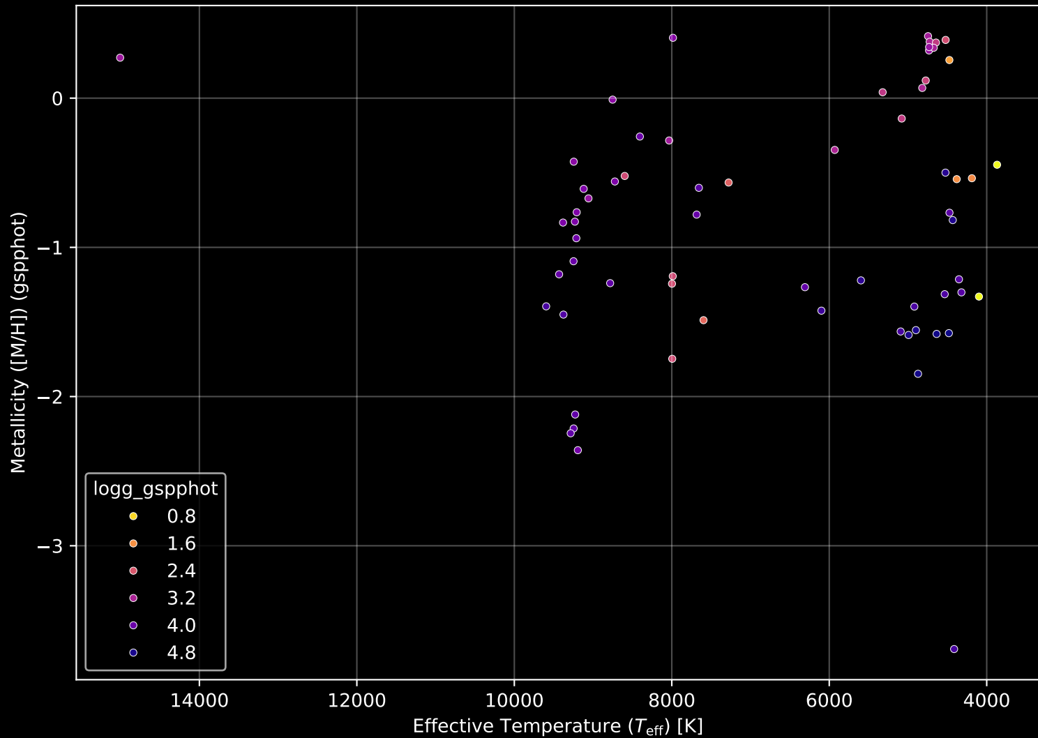
Gaia Cluster: [Gulliver_41] Stellar Population Parameters (n= 64)
