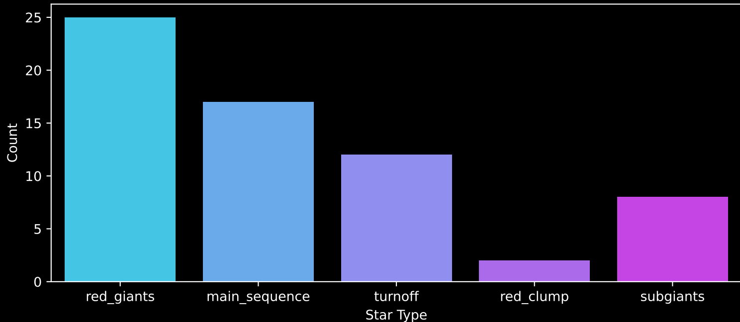
Gaia Cluster: [Gulliver_41] Count plot of Star Type
