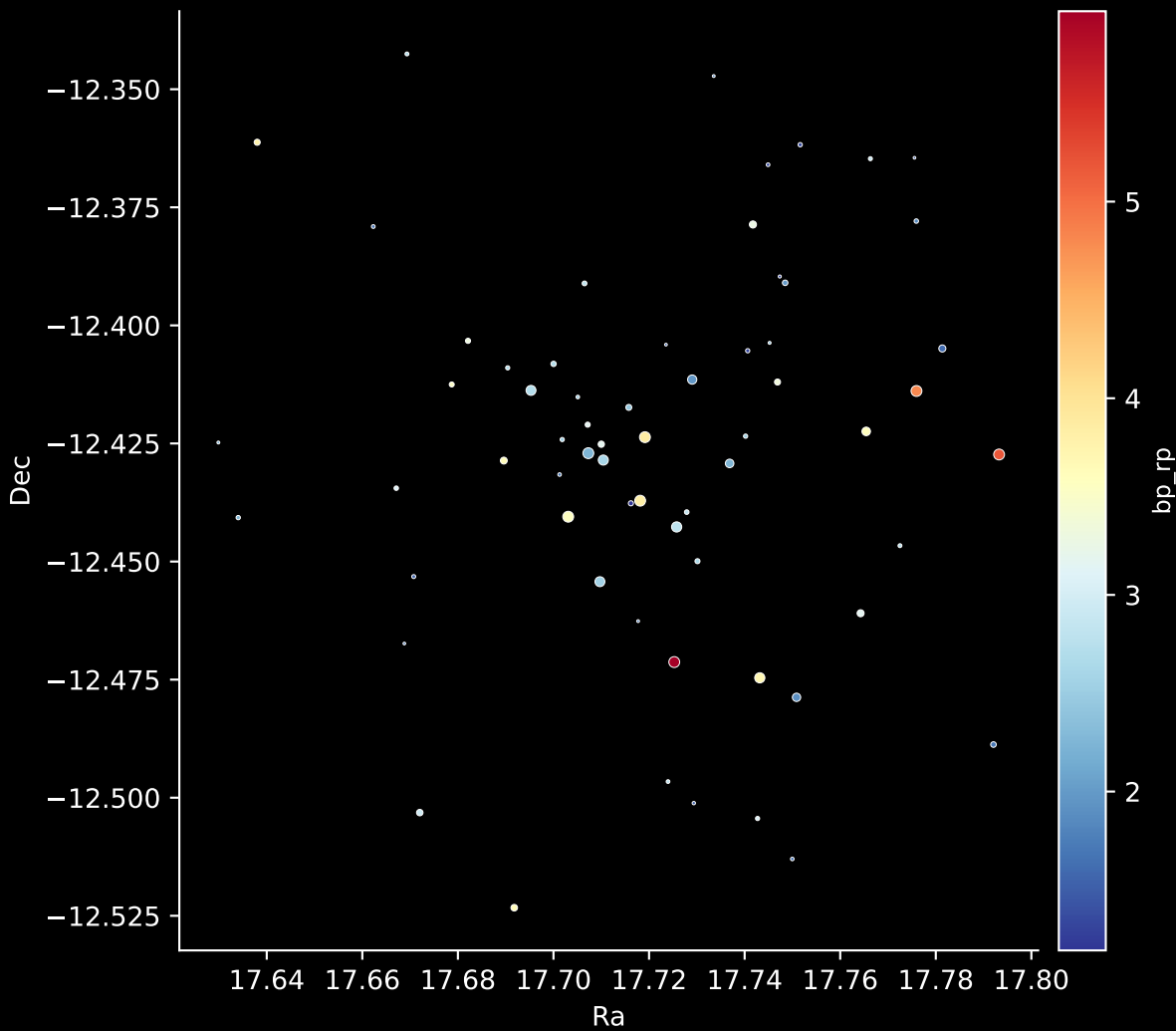
Gaia Cluster: [Gulliver_41] Stars: 64
