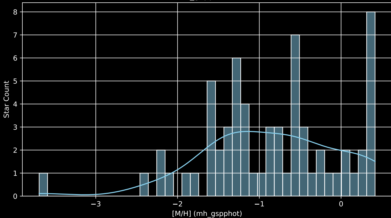
Gaia Cluster: [Gulliver_41 [M/H] (mh_gspphot) (n= 64)
