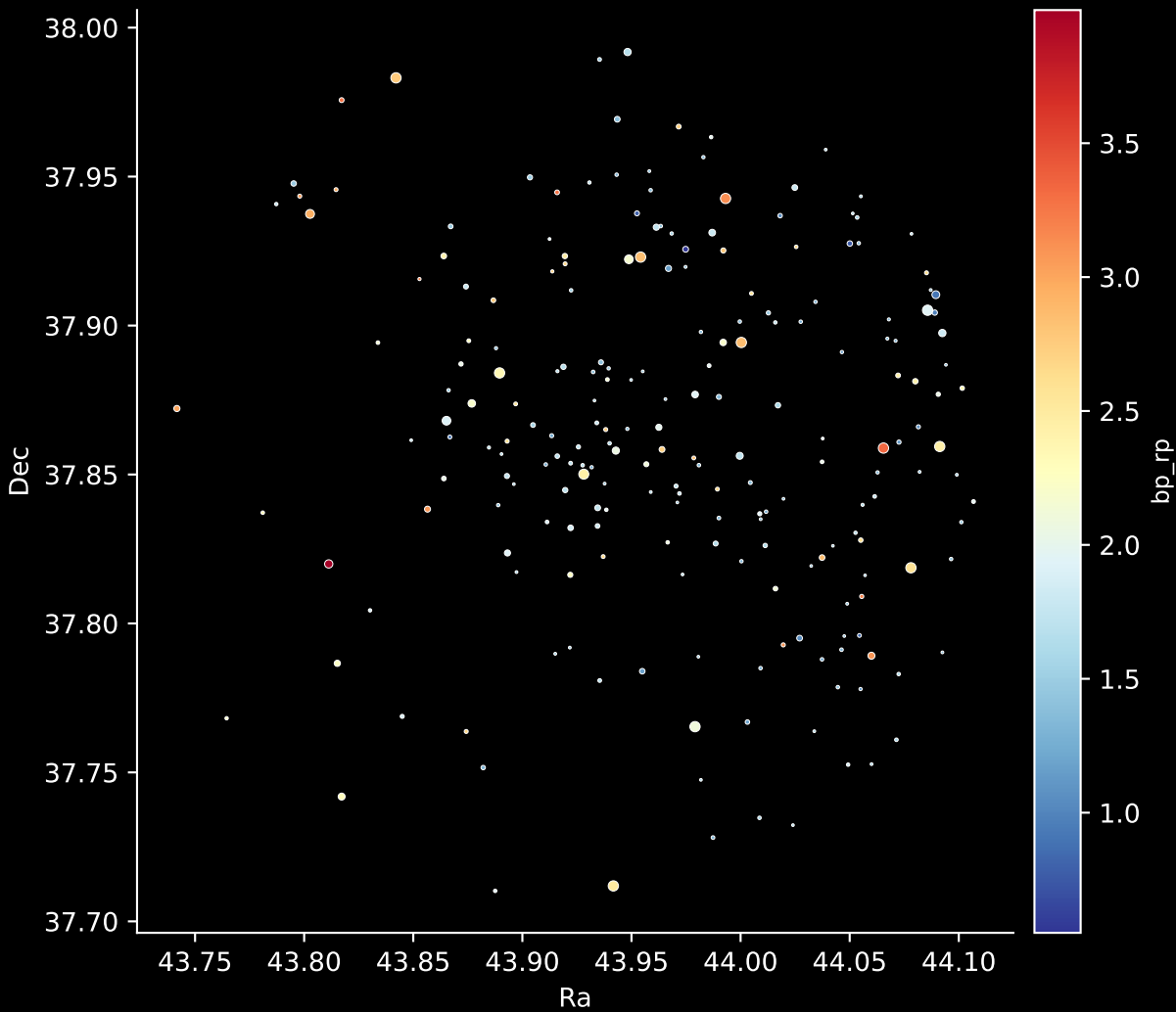
Gaia Cluster: [Gulliver_42] Stars: 218
