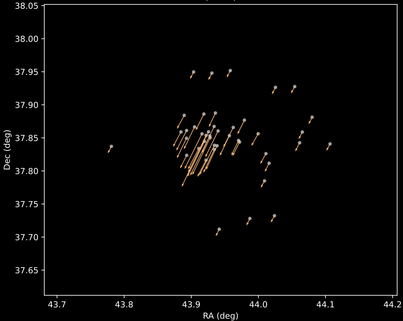
Gaia DR3 Cluster 3 Proper Motion Vectors (n=43)
