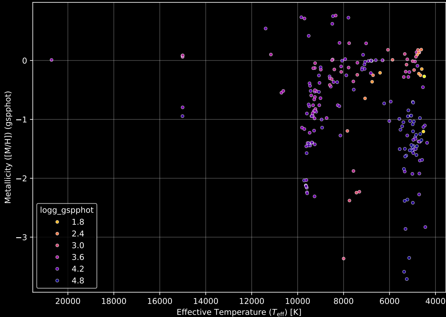
Gaia Cluster: [Gulliver_42] Stellar Population Parameters (n= 218)
