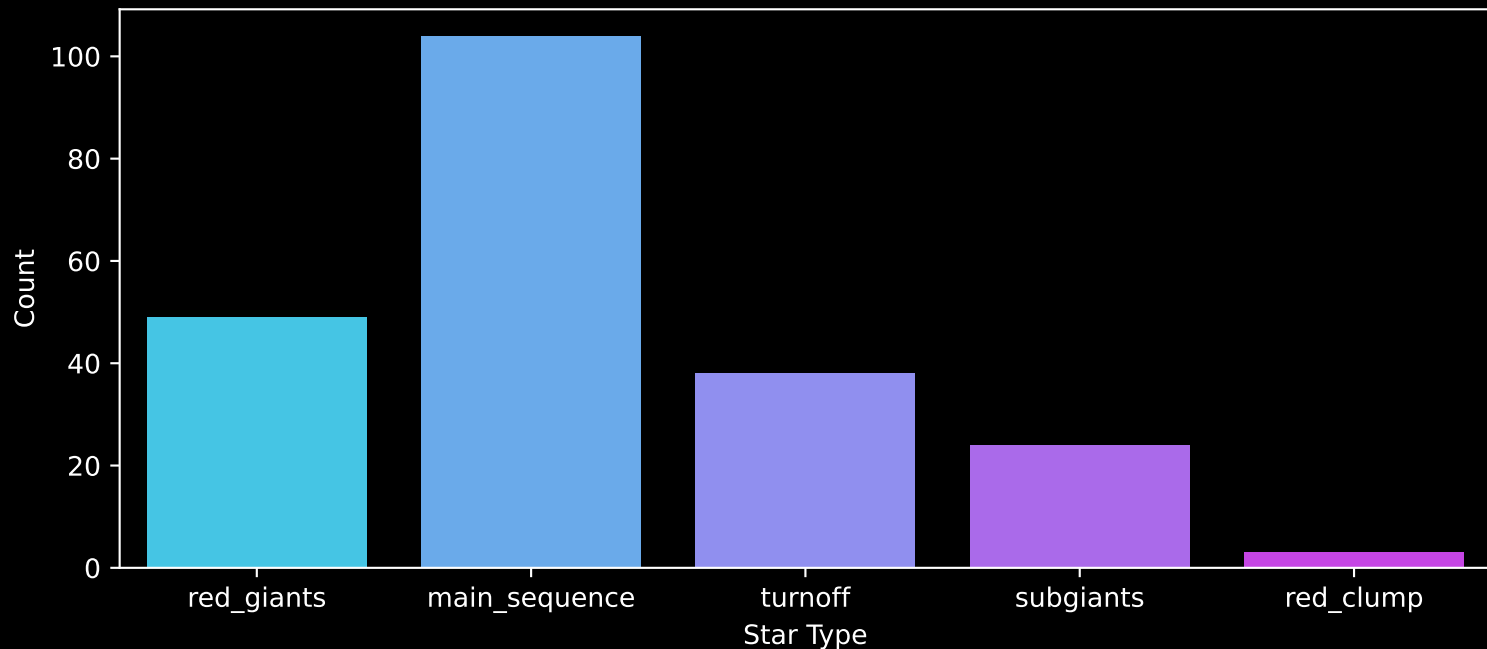
Gaia Cluster: [Gulliver_42] Count plot of Star Type
