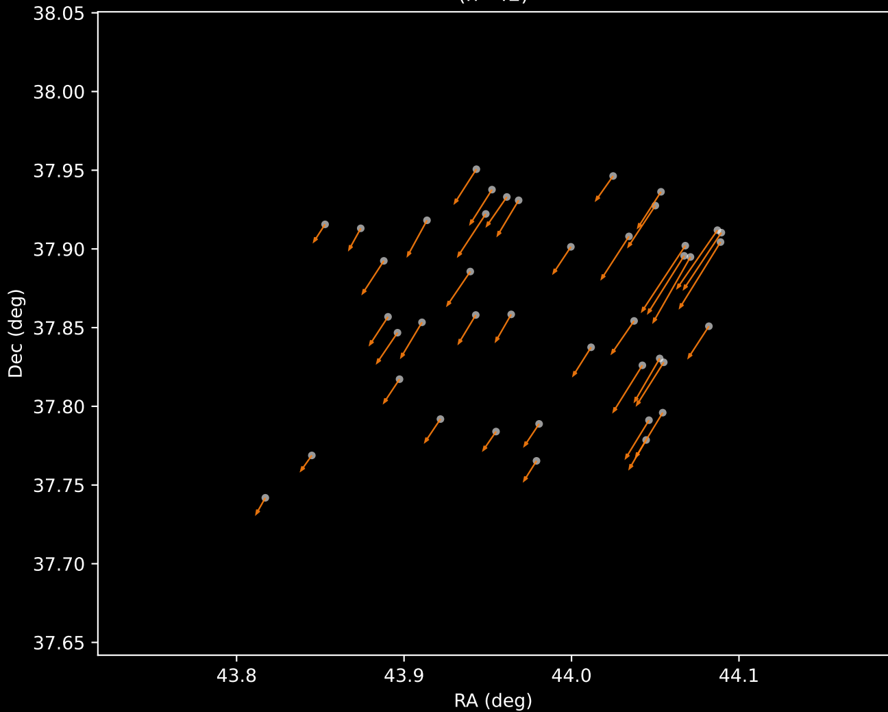
Gaia DR3 Cluster 2 Proper Motion Vectors (n=42)
