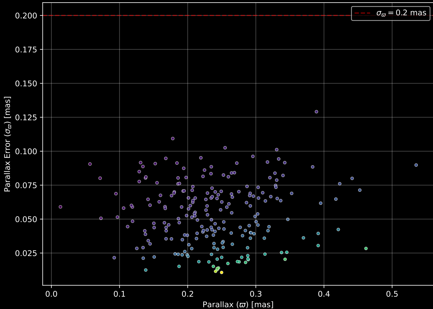
Gaia Cluster: [Gulliver_42] Parallax Quality (n= 218)
