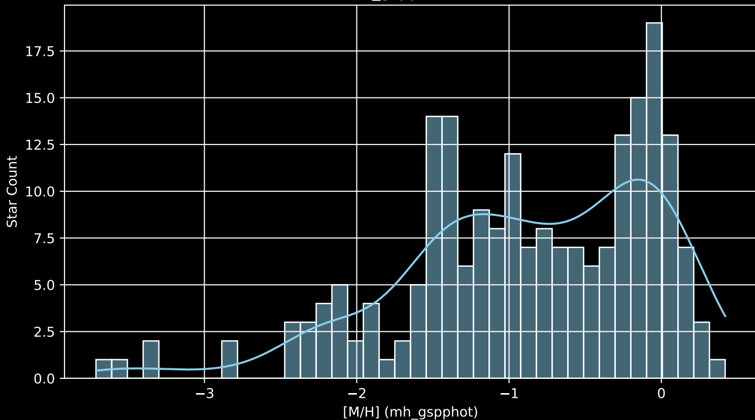
Gaia Cluster: [Gulliver_42 [M/H] (mh_gspphot) (n= 211)
