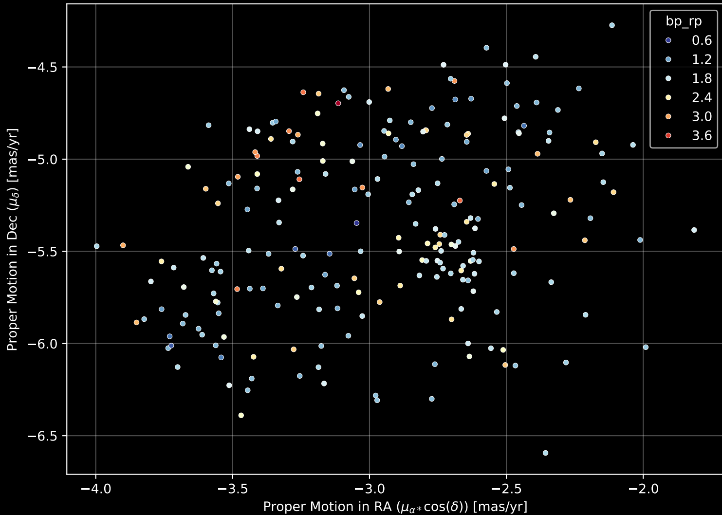
Gaia Cluster: [Gulliver_42] Proper Motion Diagram (n= 218)
