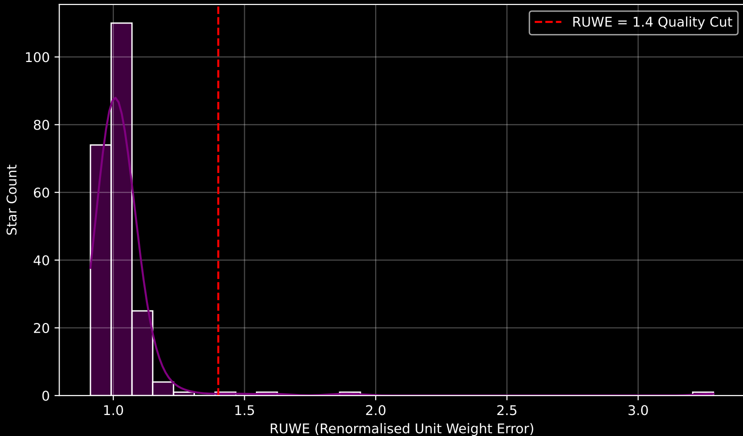
Gaia Cluster: [Gulliver_42] RUWE Distribution (n= 218)
