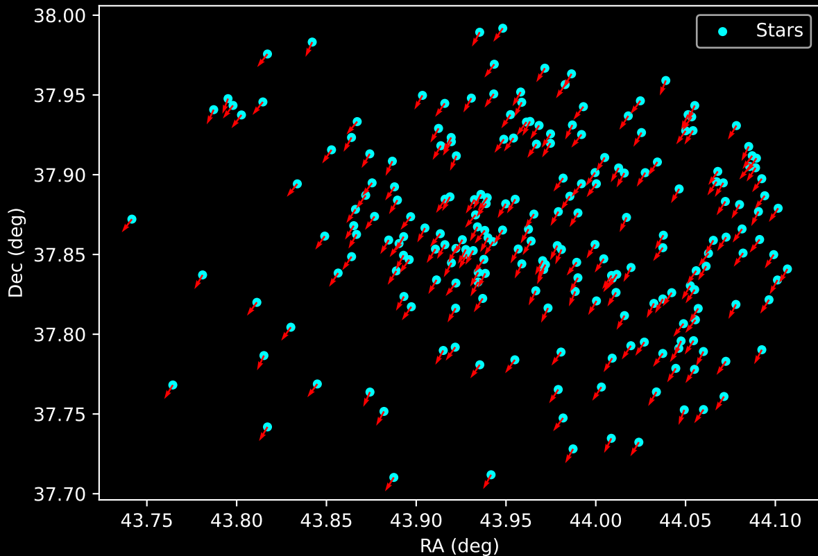
Gaia Cluster: [Gulliver_42] Proper Motion Vectors for Gaia Star Field (n= 218)
