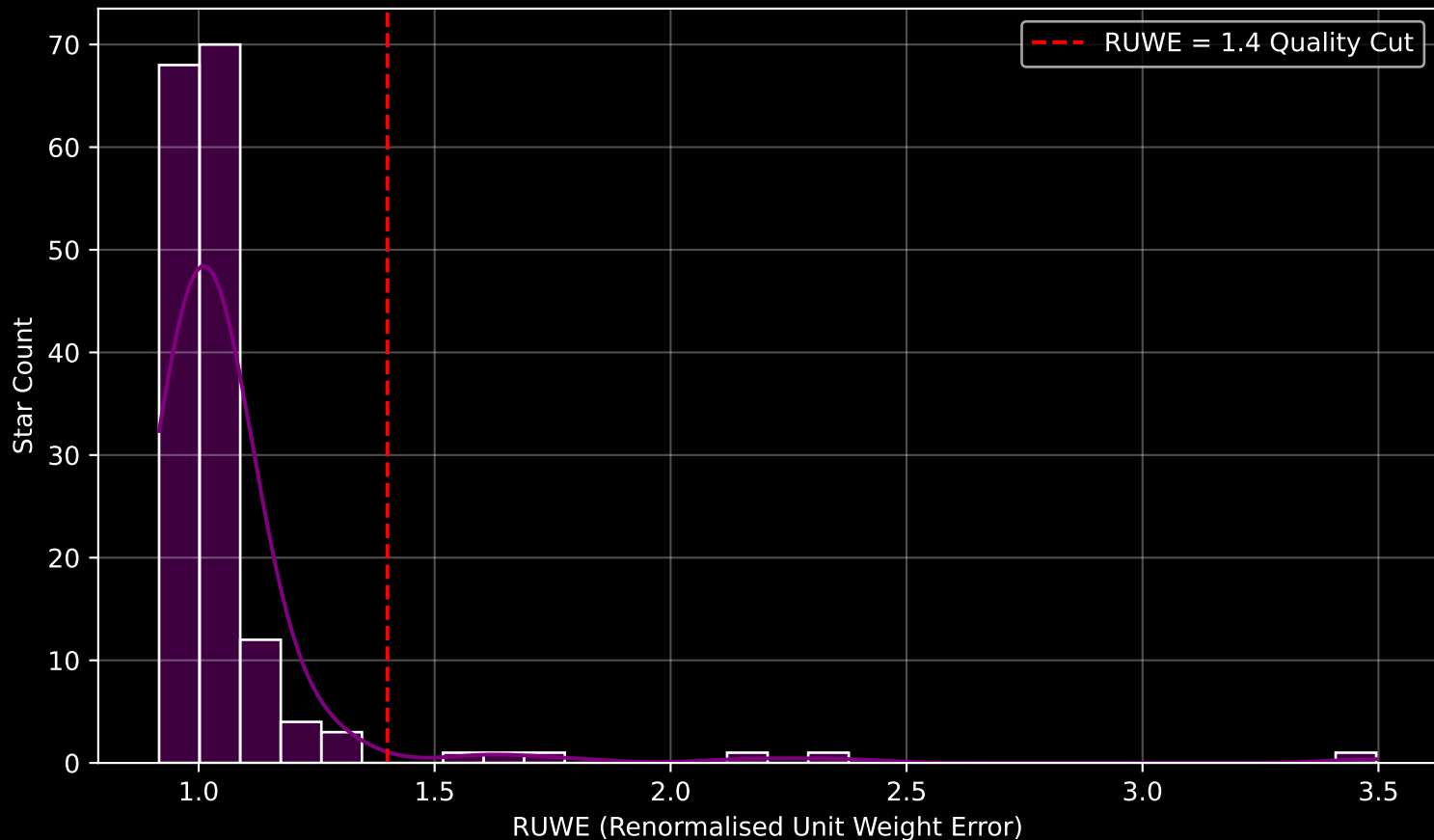
Gaia Cluster: [Gulliver_44] RUWE Distribution (n= 163)
