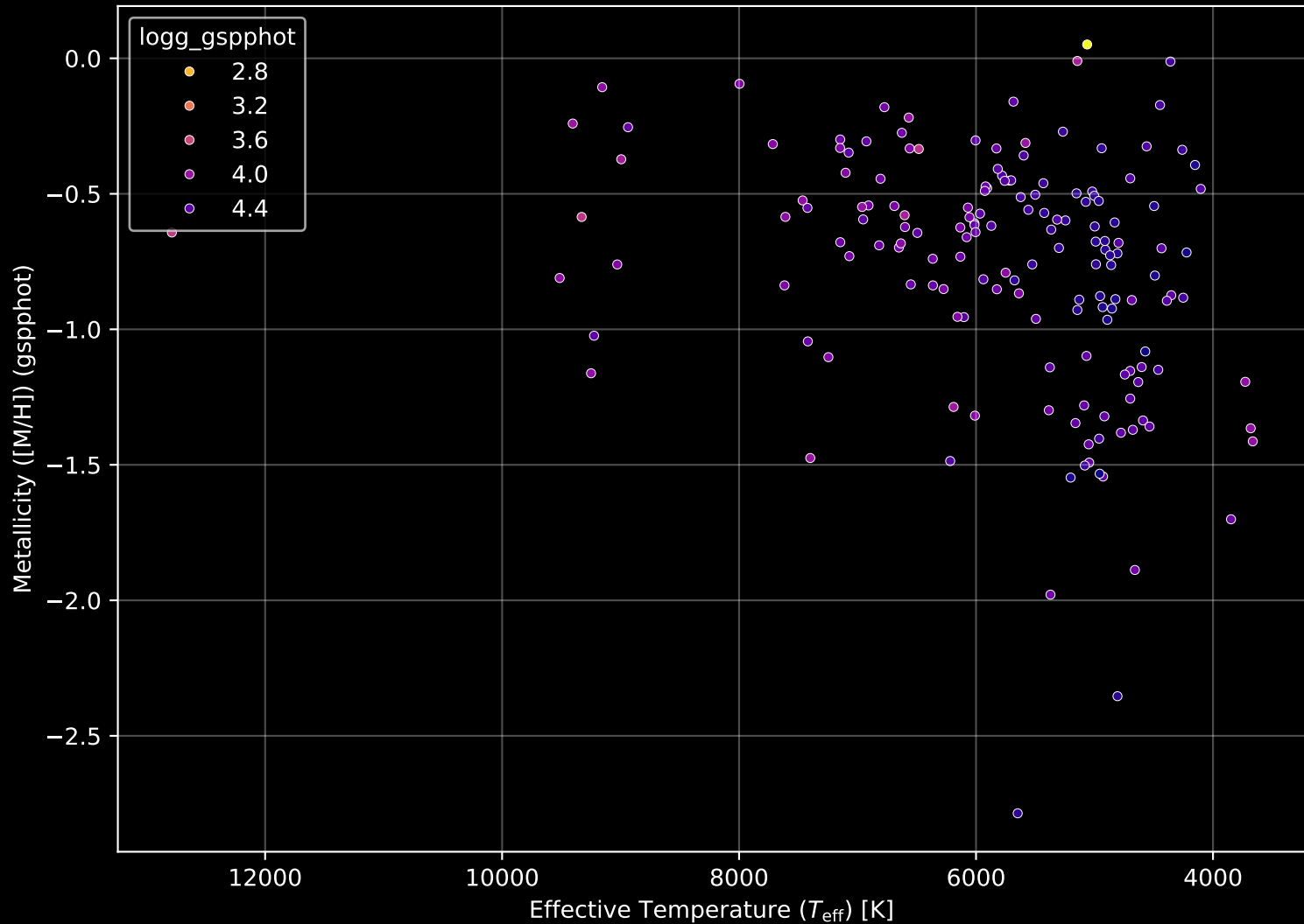
Gaia Cluster: [Gulliver_44] Stellar Population Parameters (n= 163)
