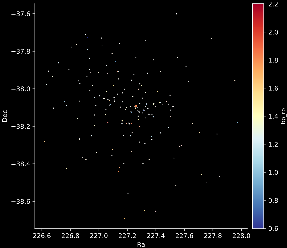
Gaia Cluster: [Gulliver_44] Stars: 163
