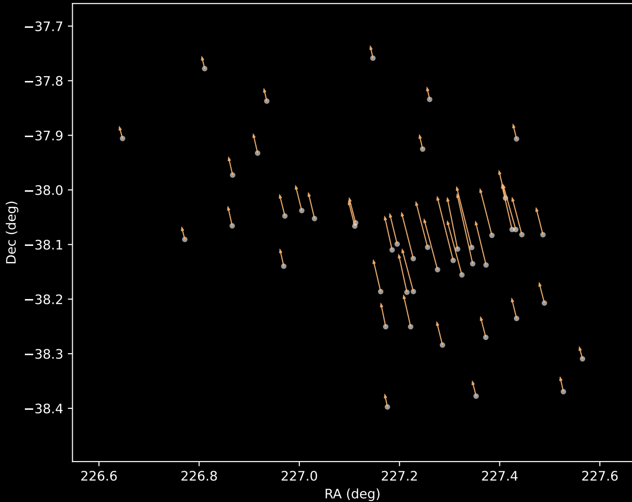
Gaia DR3 Cluster 3 Proper Motion Vectors (n=47)
