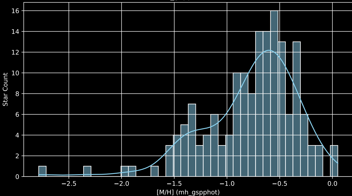
Gaia Cluster: [Gulliver_44 [M/H] (mh_gspphot) (n= 163)
