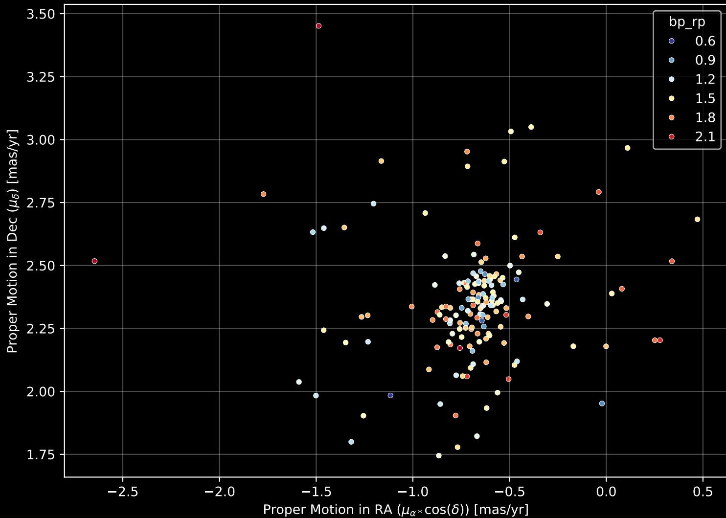
Gaia Cluster: [Gulliver_44] Proper Motion Diagram (n= 163)
