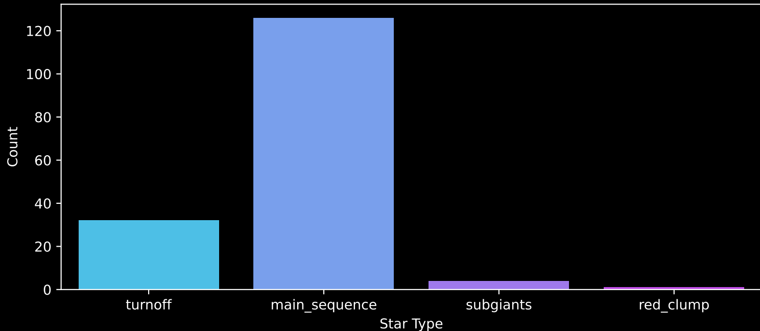
Gaia Cluster: [Gulliver_44] Count plot of Star Type
