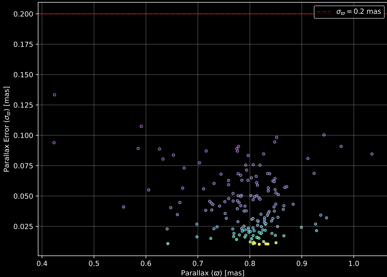
Gaia Cluster: [Gulliver_44] Parallax Quality (n= 163)
