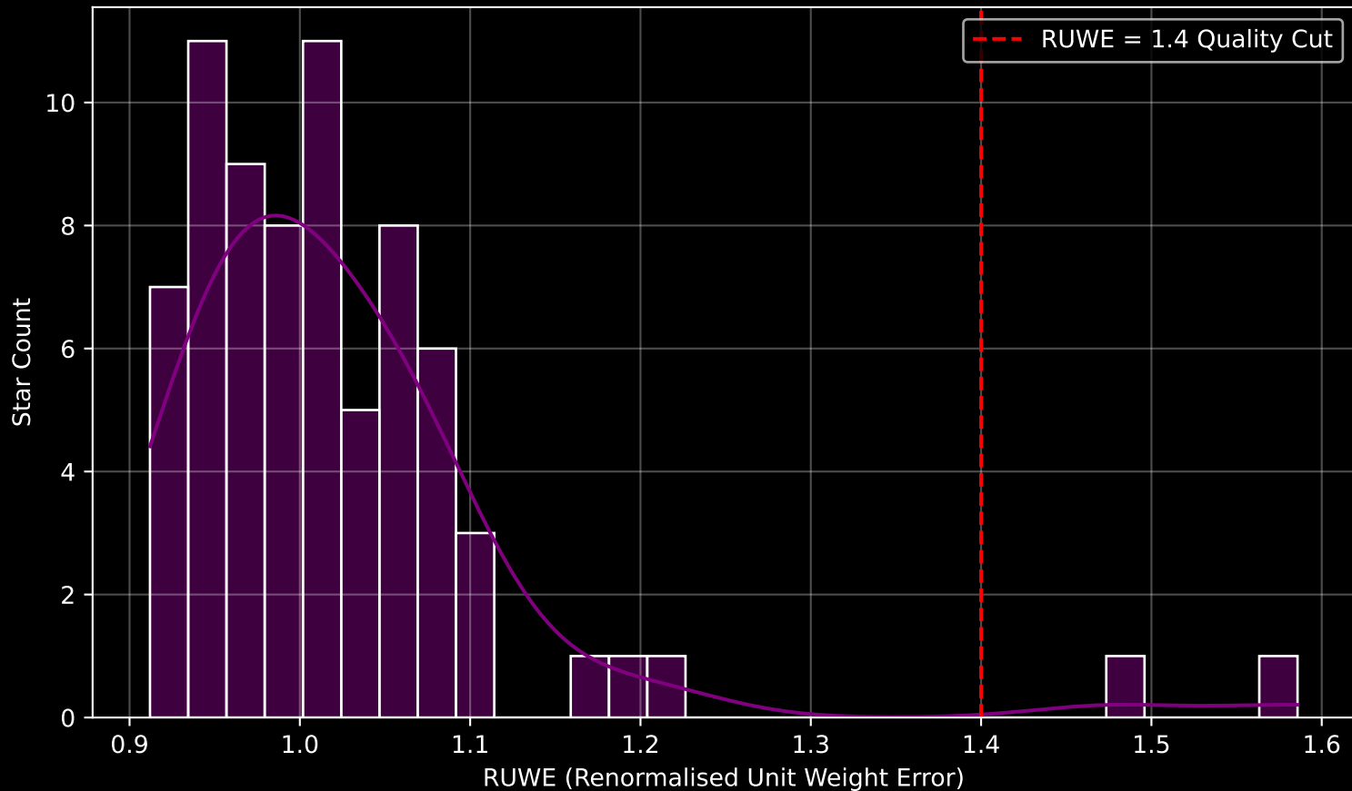
Gaia Cluster: [Gulliver_45] RUWE Distribution (n= 73)
