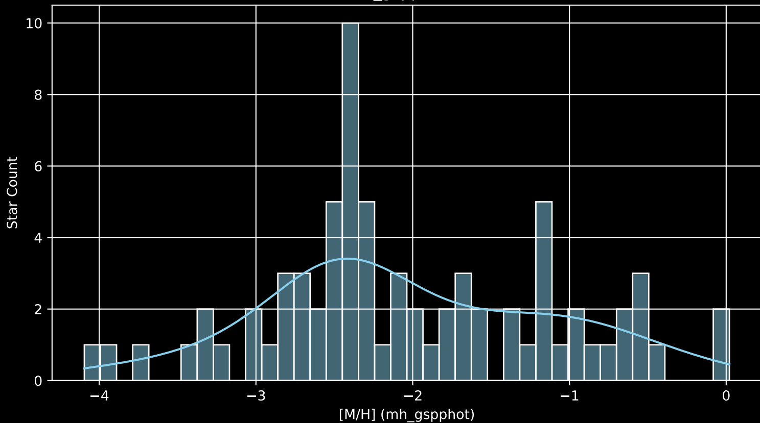
Gaia Cluster: [Gulliver_45 [M/H] (mh_gspphot) (n= 73)
