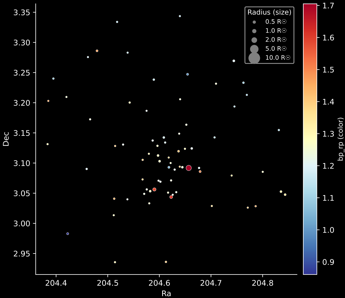
Gaia Cluster: [Gulliver_45] Stars: 73
