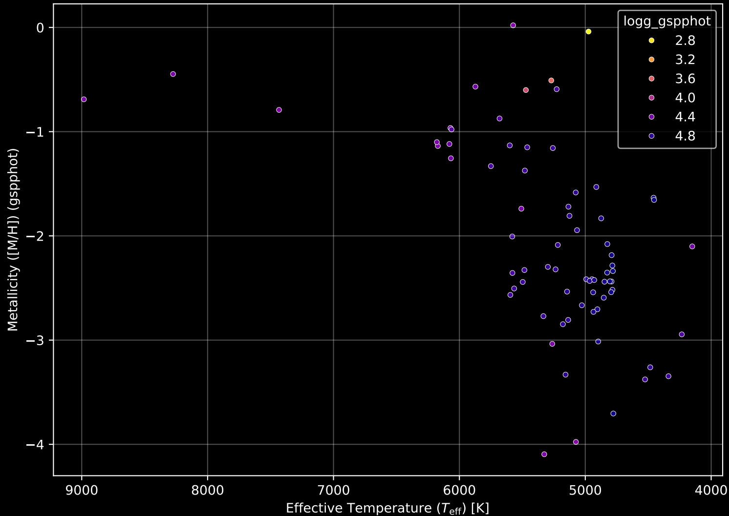
Gaia Cluster: [Gulliver_45] Stellar Population Parameters (n= 73)
