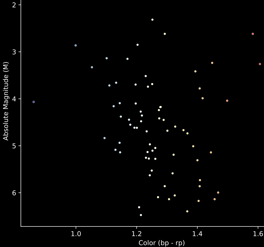
Gaia Cluster: [Gulliver_45] Stars (n= 73) Hertzsprung-Russel Diagram
