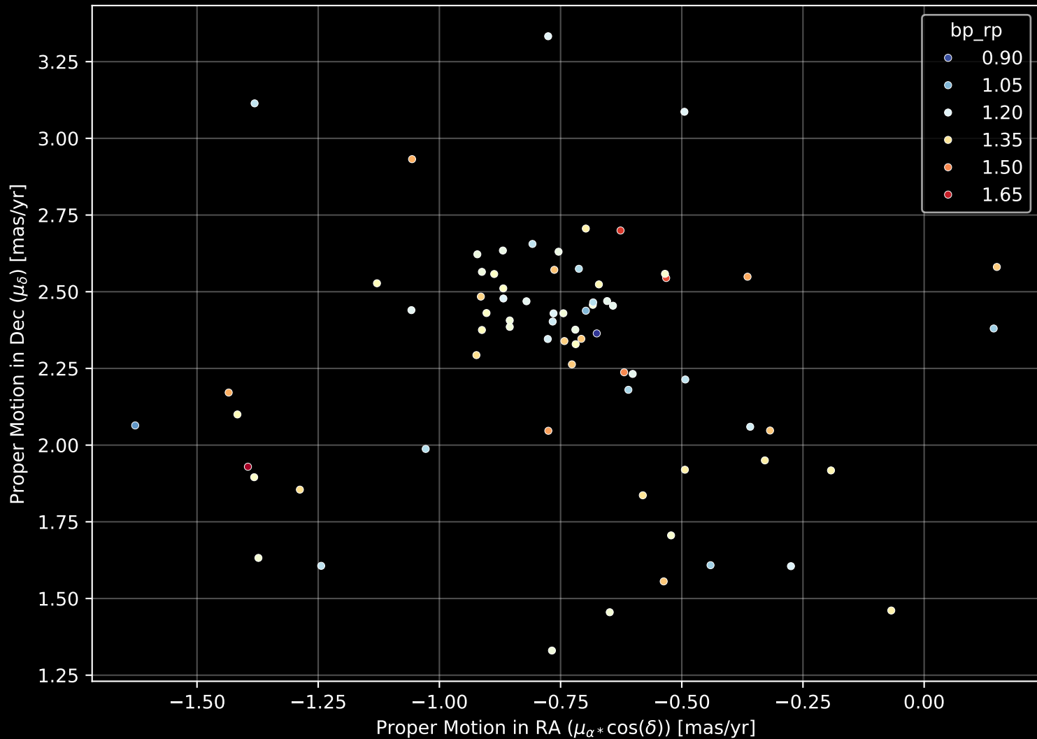
Gaia Cluster: [Gulliver_45] Proper Motion Diagram (n= 73)
