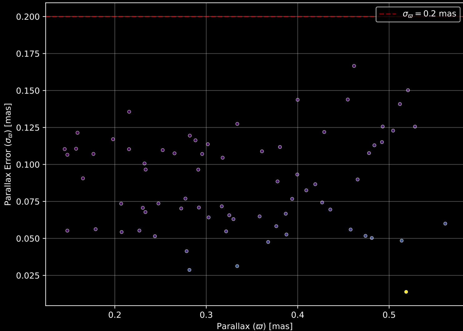
Gaia Cluster: [Gulliver_45] Parallax Quality (n= 73)
