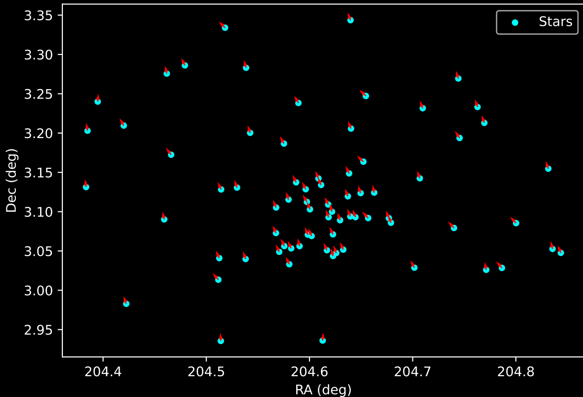
Gaia Cluster: [Gulliver_45] Proper Motion Vectors for Gaia Star Field (n= 73)
