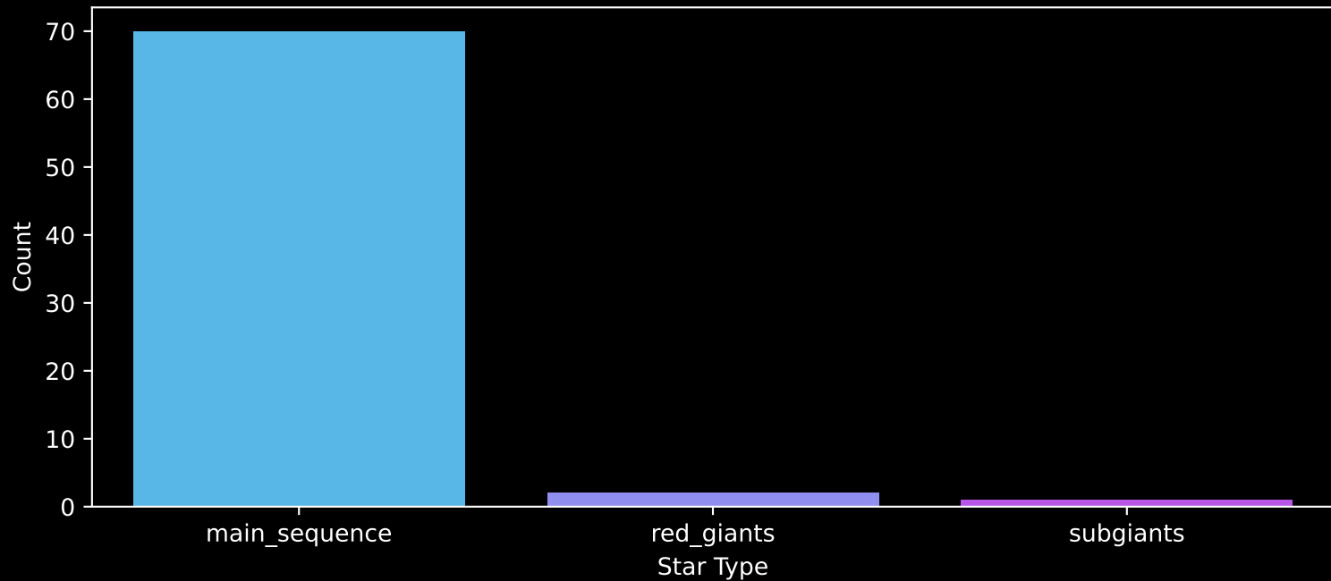
Gaia Cluster: [Gulliver_45] Count plot of Star Type
