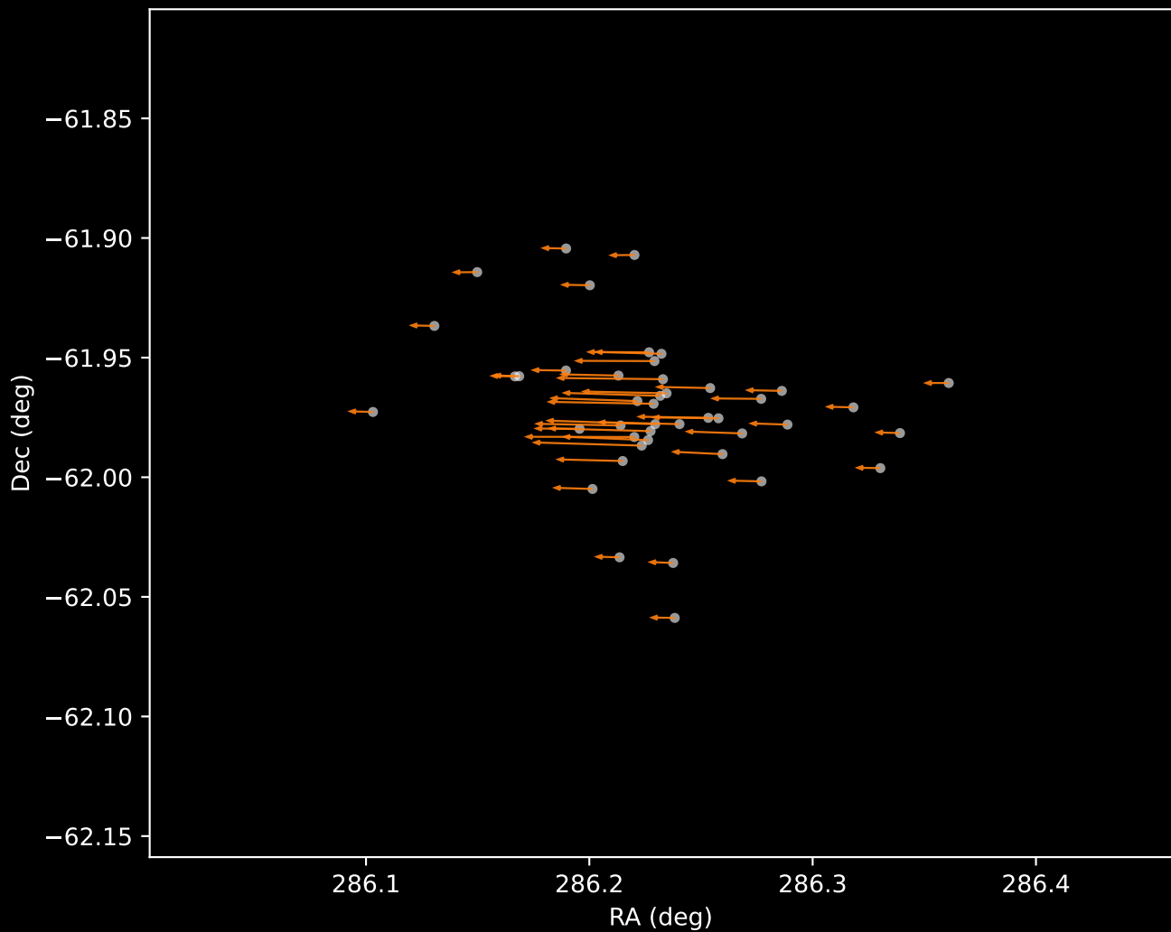
Gaia DR3 Cluster 2 Proper Motion Vectors (n=44)
