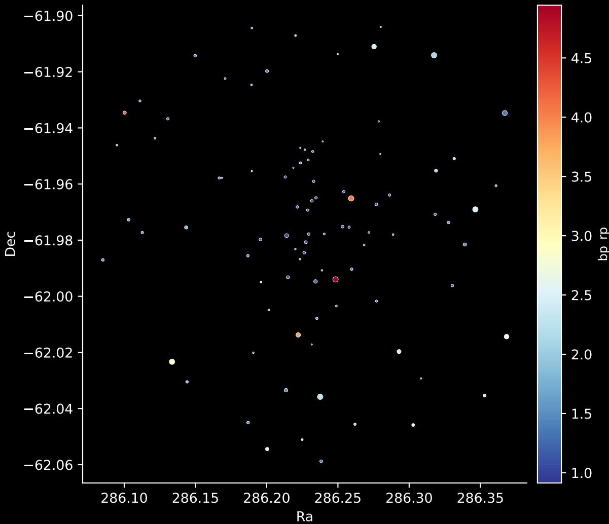
Gaia Cluster: [Gulliver_46] Stars: 91
