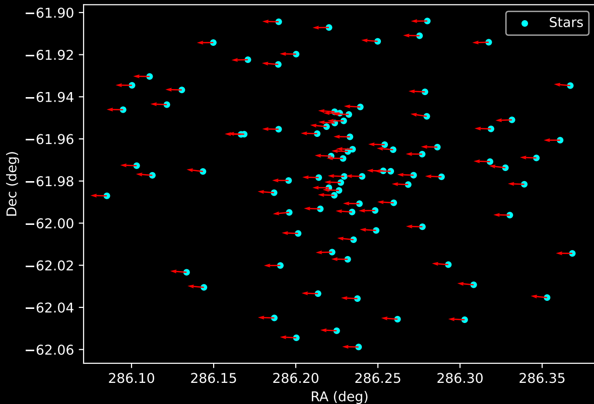
Gaia Cluster: [Gulliver_46] Proper Motion Vectors for Gaia Star Field (n= 91)
