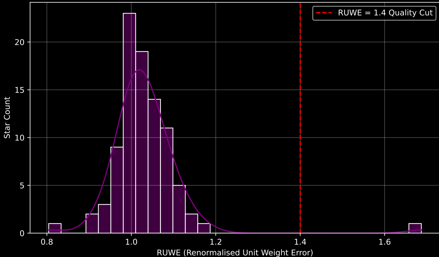
Gaia Cluster: [Gulliver_46] RUWE Distribution (n= 91)
