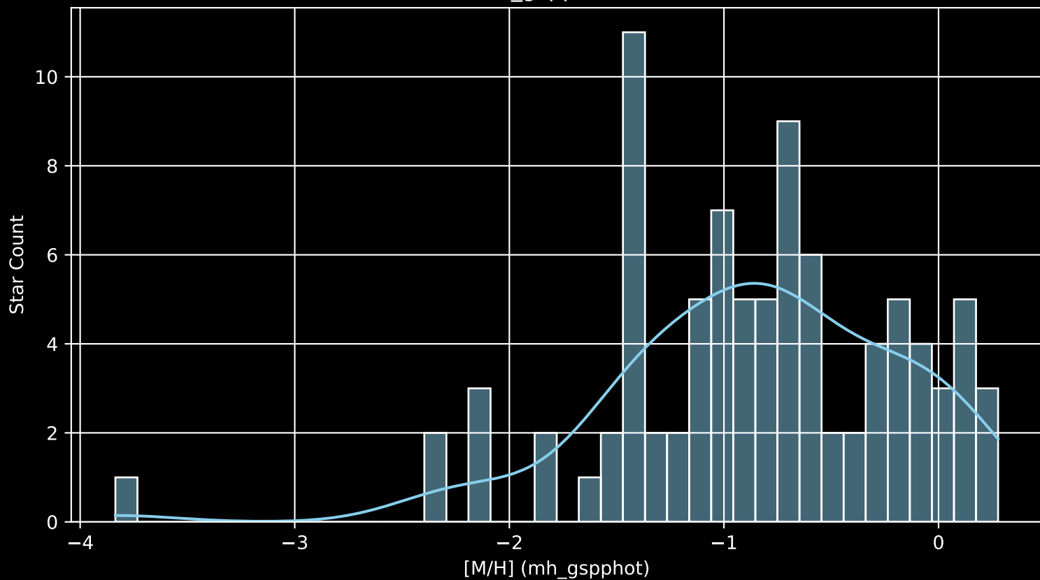
Gaia Cluster: [Gulliver_46 [M/H] (mh_gspphot) (n= 91)
