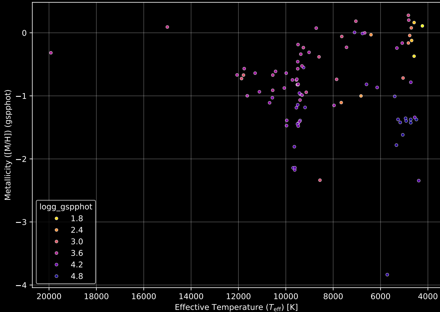
Gaia Cluster: [Gulliver_46] Stellar Population Parameters (n= 91)
