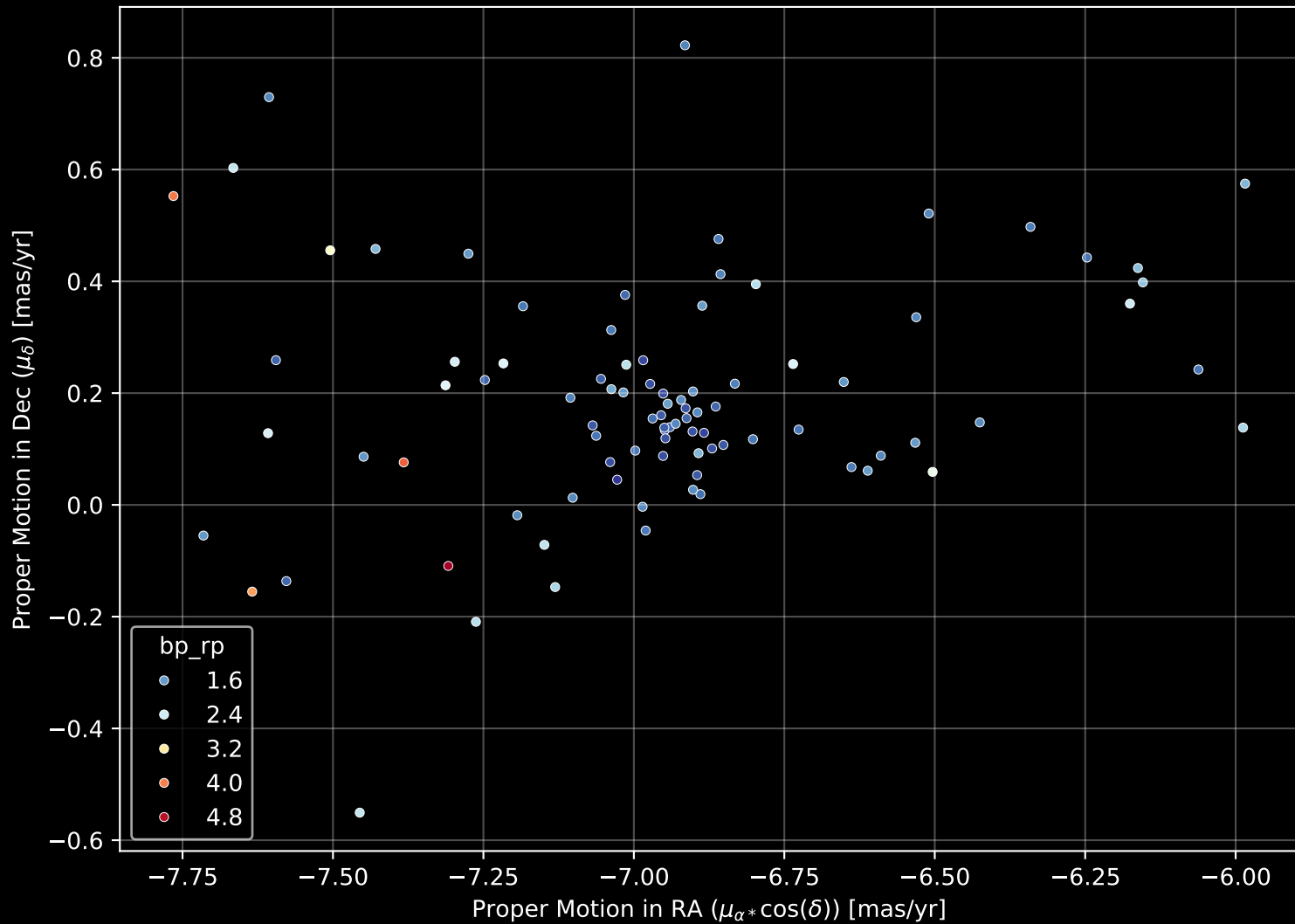
Gaia Cluster: [Gulliver_46] Proper Motion Diagram (n= 91)
