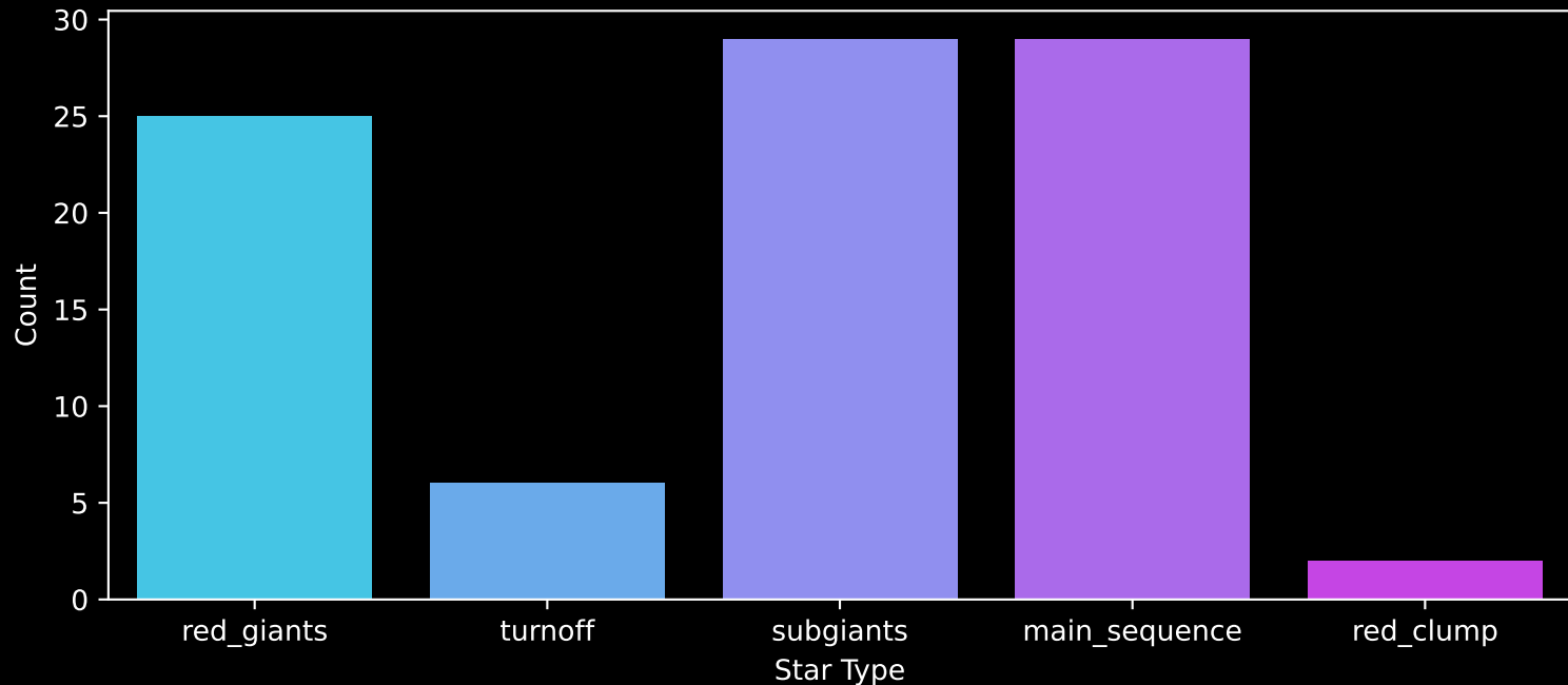
Gaia Cluster: [Gulliver_46] Count plot of Star Type
