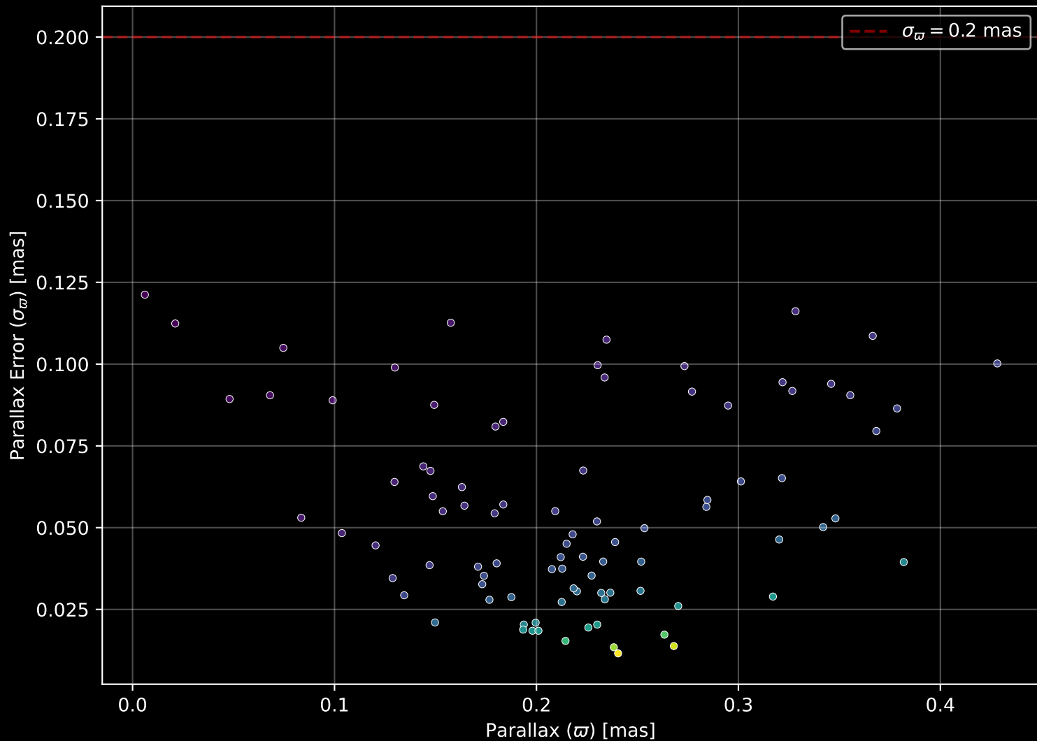
Gaia Cluster: [Gulliver_46] Parallax Quality (n= 91)
