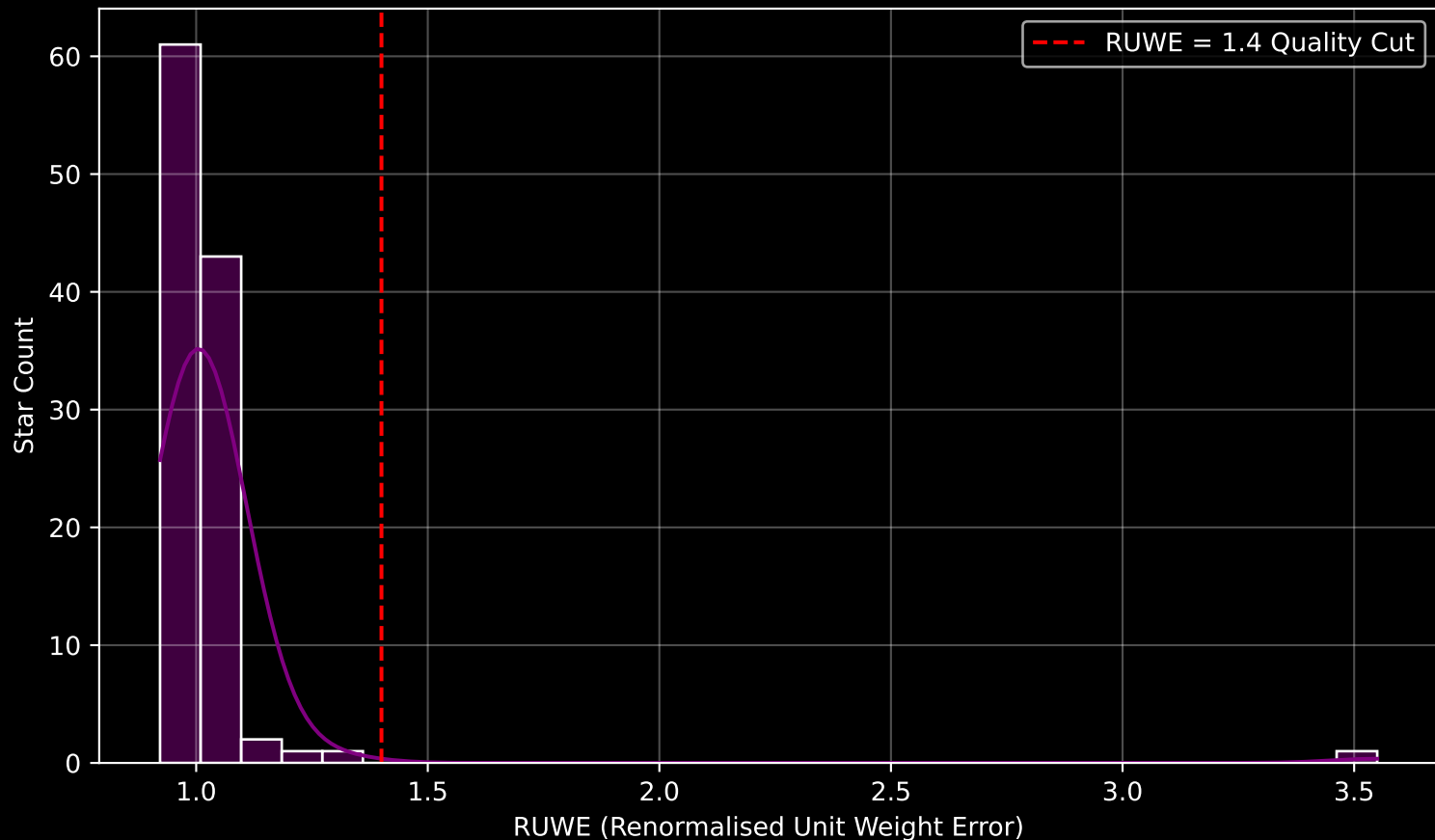
Gaia Cluster: [Gulliver_49] RUWE Distribution (n= 109)
