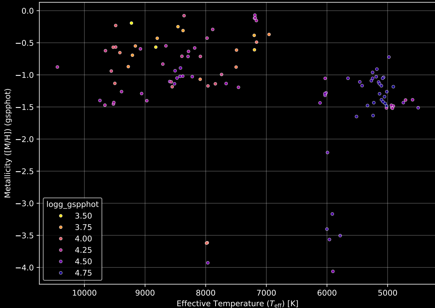
Gaia Cluster: [Gulliver_49] Stellar Population Parameters (n= 109)
