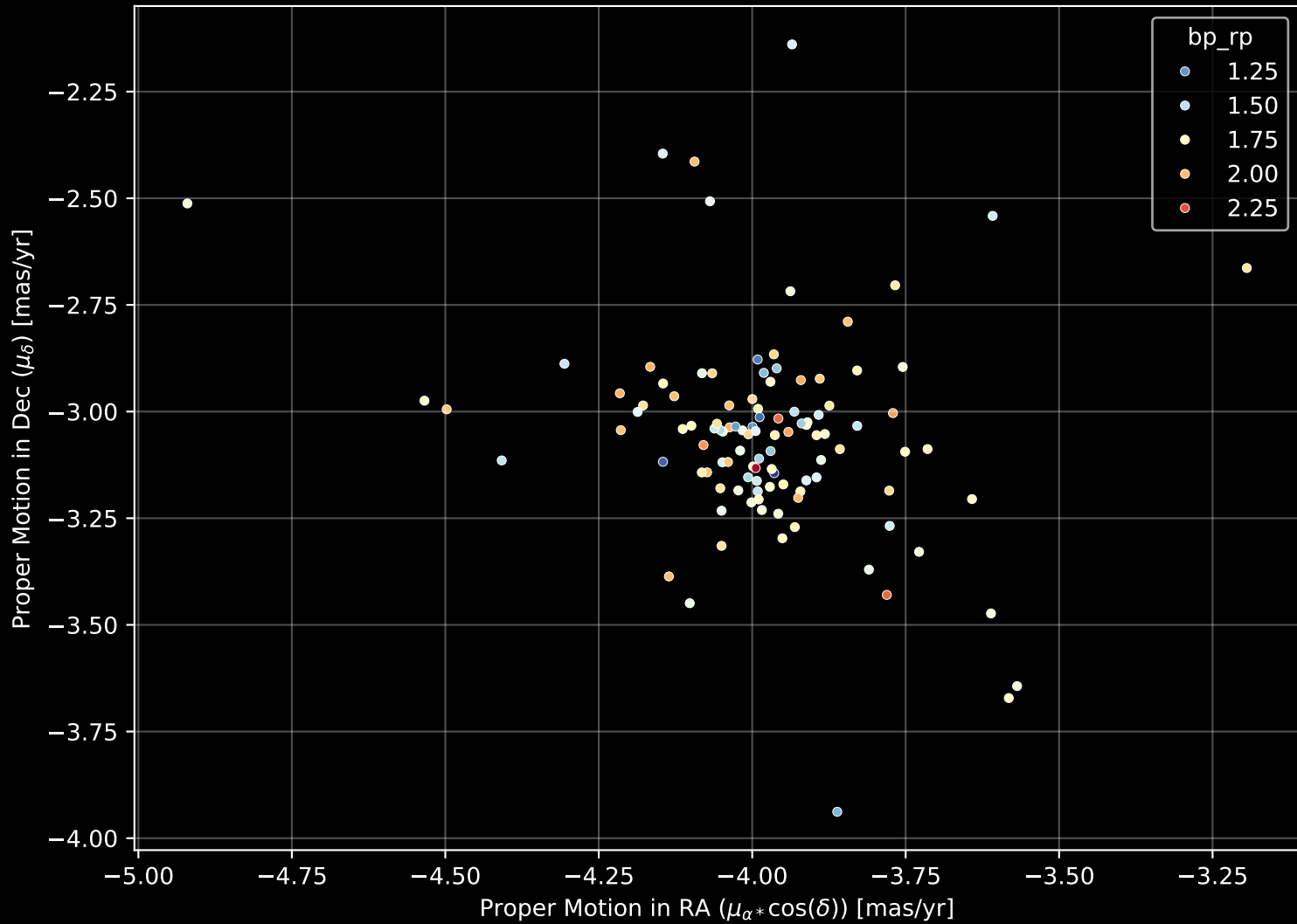
Gaia Cluster: [Gulliver_49] Proper Motion Diagram (n= 109)
