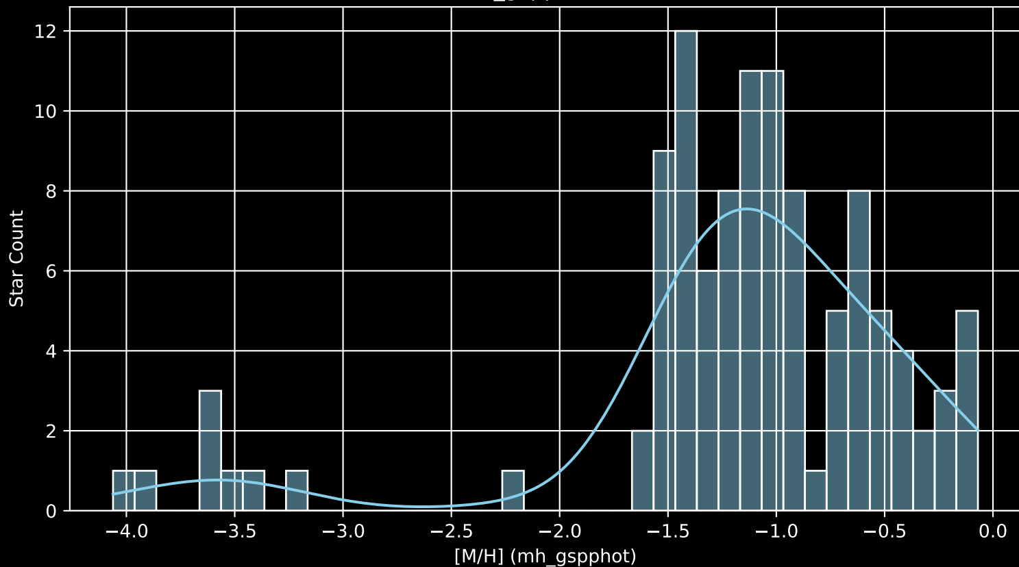
Gaia Cluster: [Gulliver_49 [M/H] (mh_gspphot) (n= 109)
