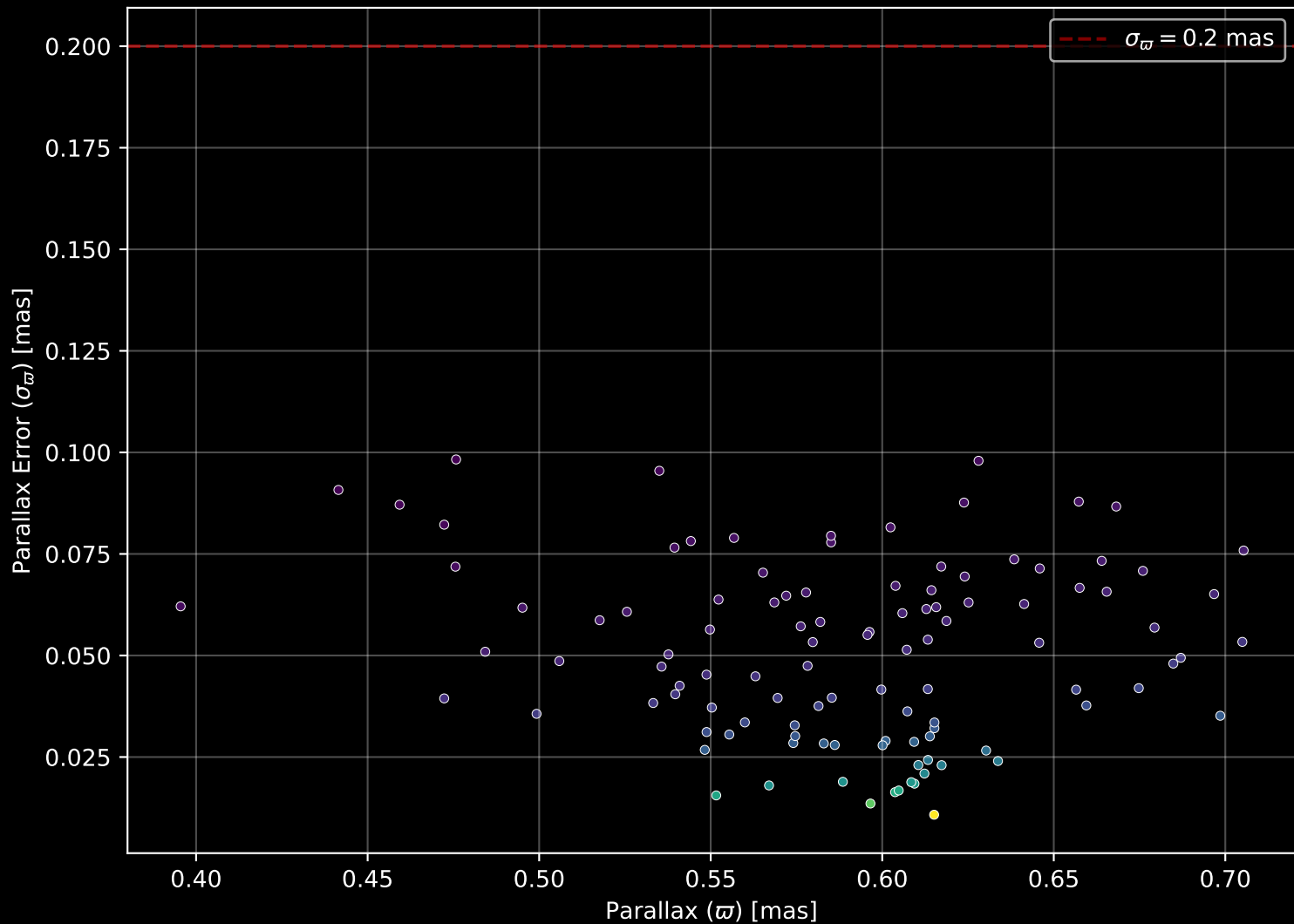
Gaia Cluster: [Gulliver_49] Parallax Quality (n= 109)
