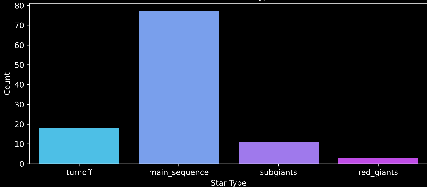
Gaia Cluster: [Gulliver_49] Count plot of Star Type
