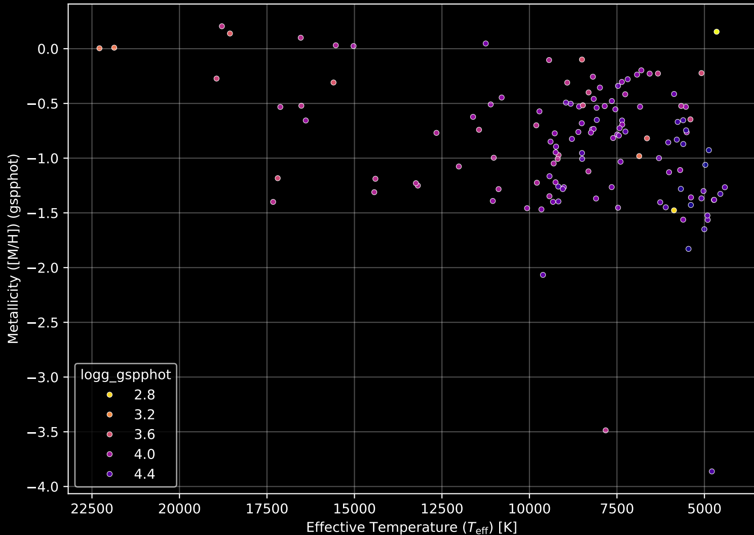
Gaia Cluster: [Gulliver_5] Stellar Population Parameters (n= 133)
