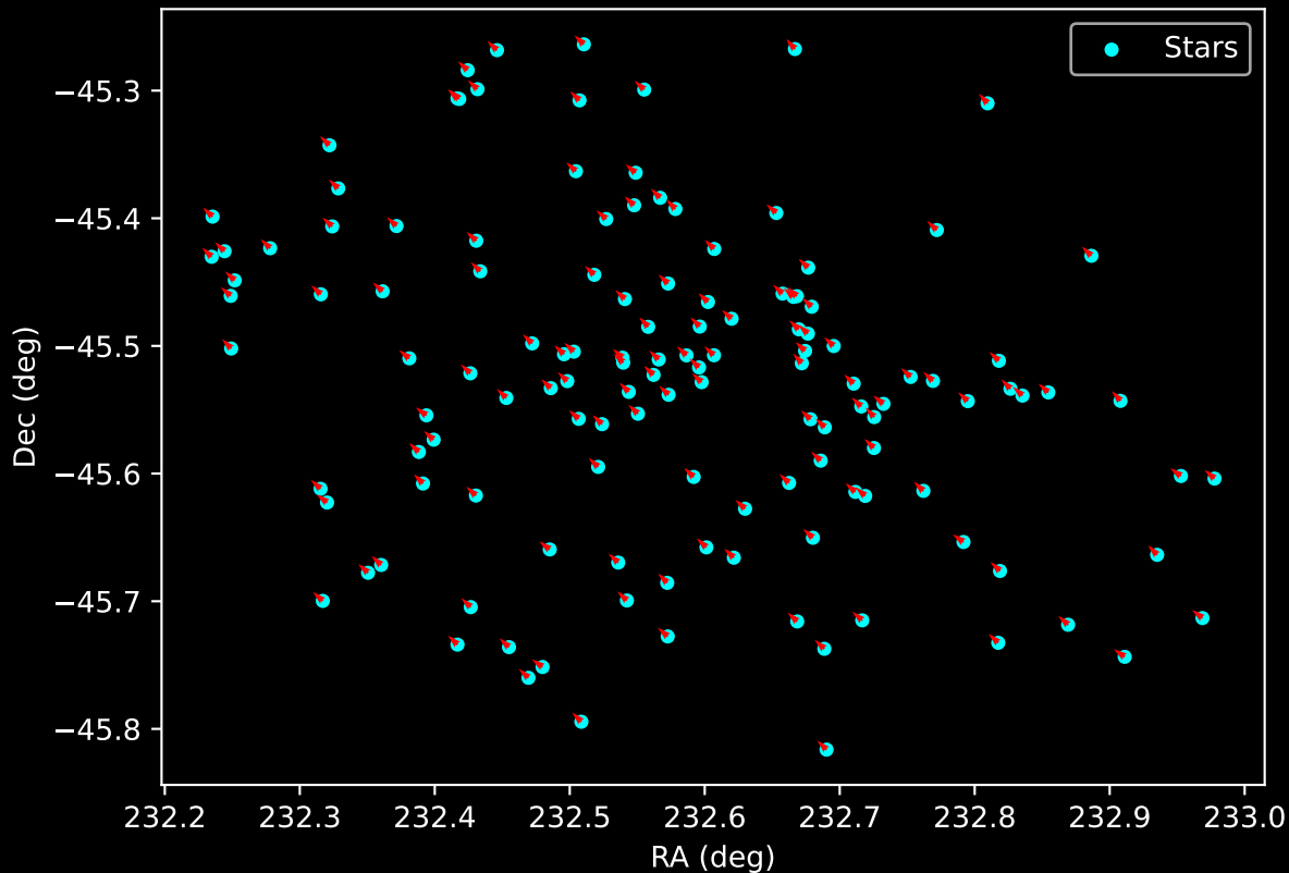
Gaia Cluster: [Gulliver_5] Proper Motion Vectors for Gaia Star Field (n= 133)
