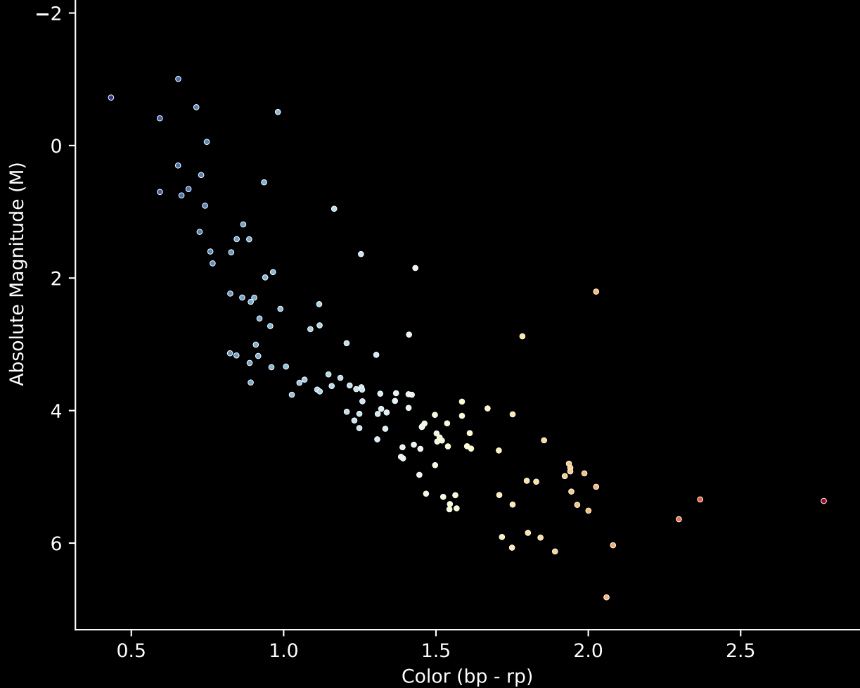
Gaia Cluster: [Gulliver_5] Stars (n= 133) Hertzprung-Russel Diagram
