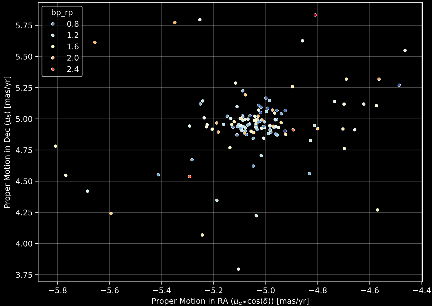
Gaia Cluster: [Gulliver_5] Proper Motion Diagram (n= 133)
