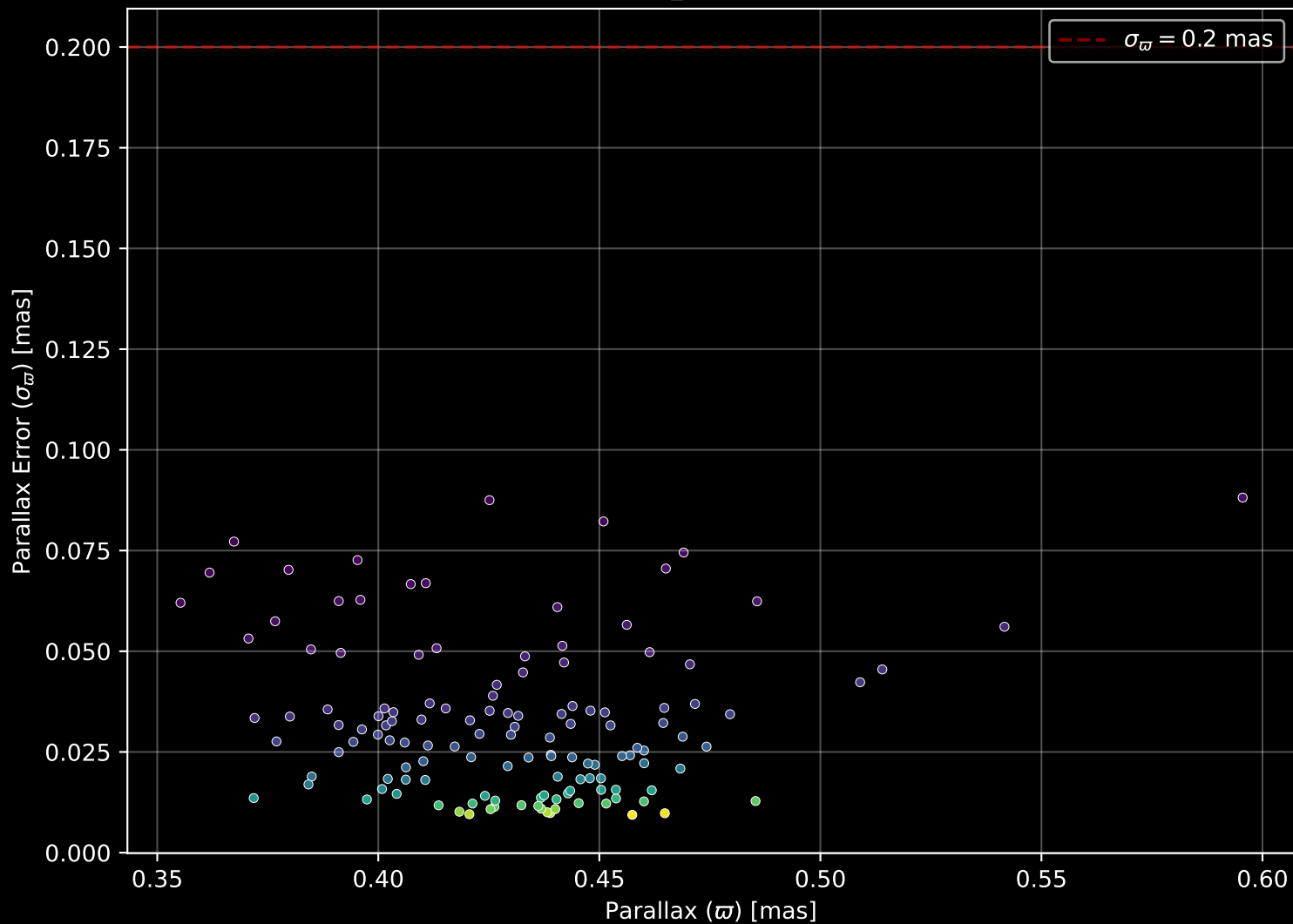
Gaia Cluster: [Gulliver_5] Parallax Quality (n= 133)
