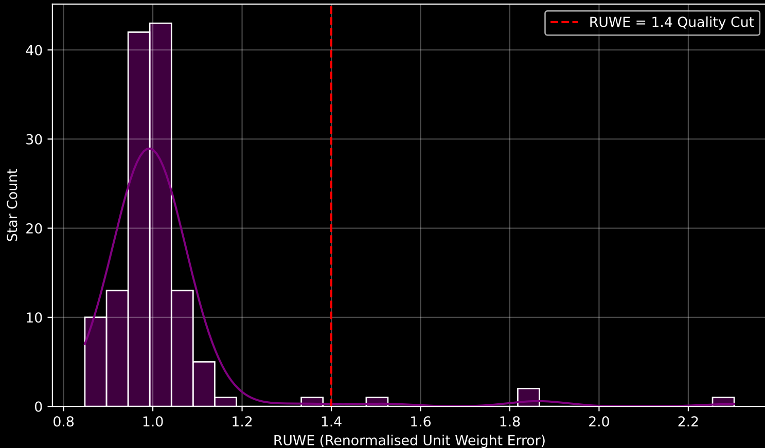
Gaia Cluster: [Gulliver_5] RUWE Distribution (n= 132)
