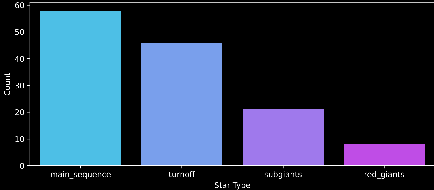
Gaia Cluster: [Gulliver_5] Count plot of Star Type
