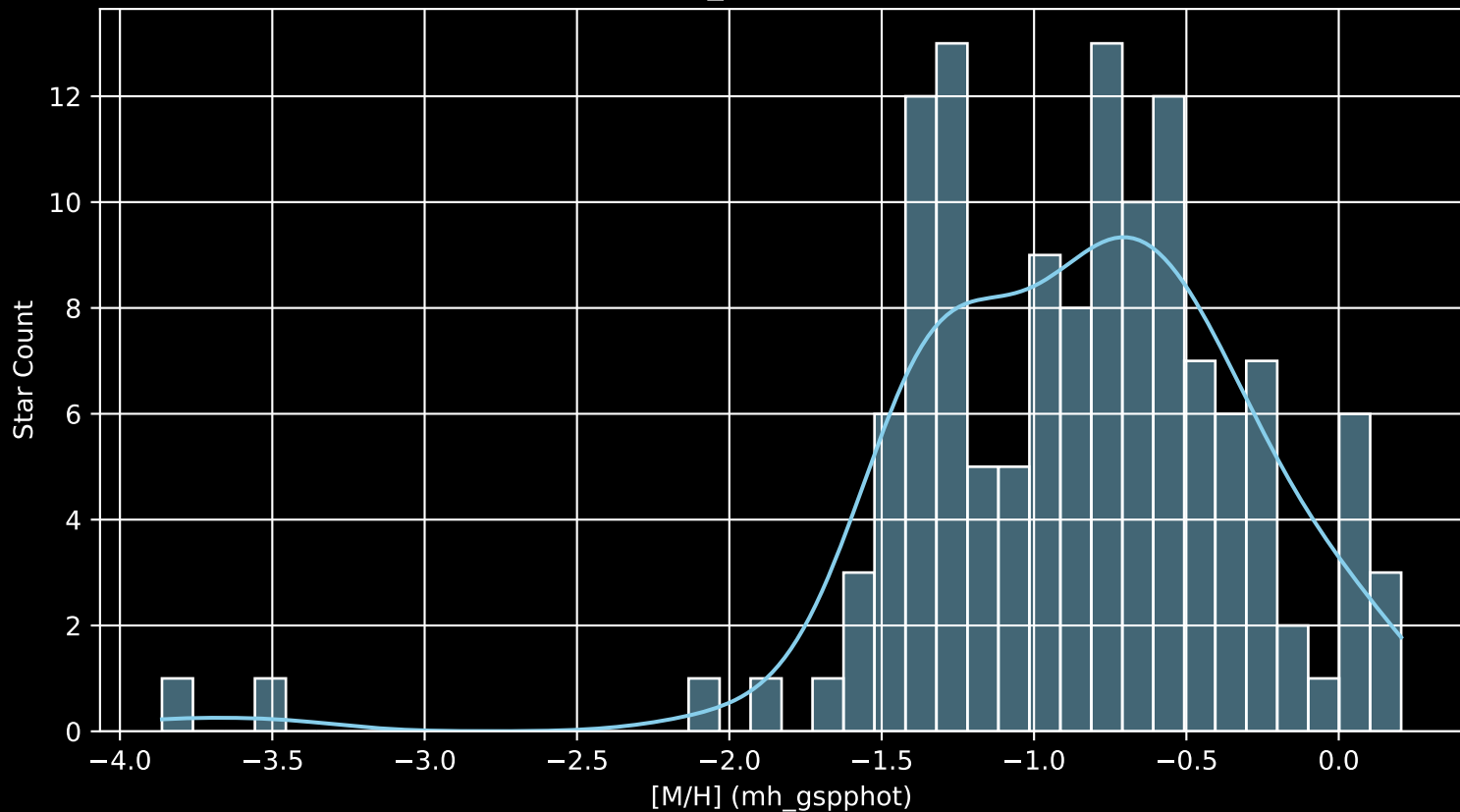
Gaia Cluster: [Gulliver_5 [M/H] (mh_gspphot) (n= 133)
