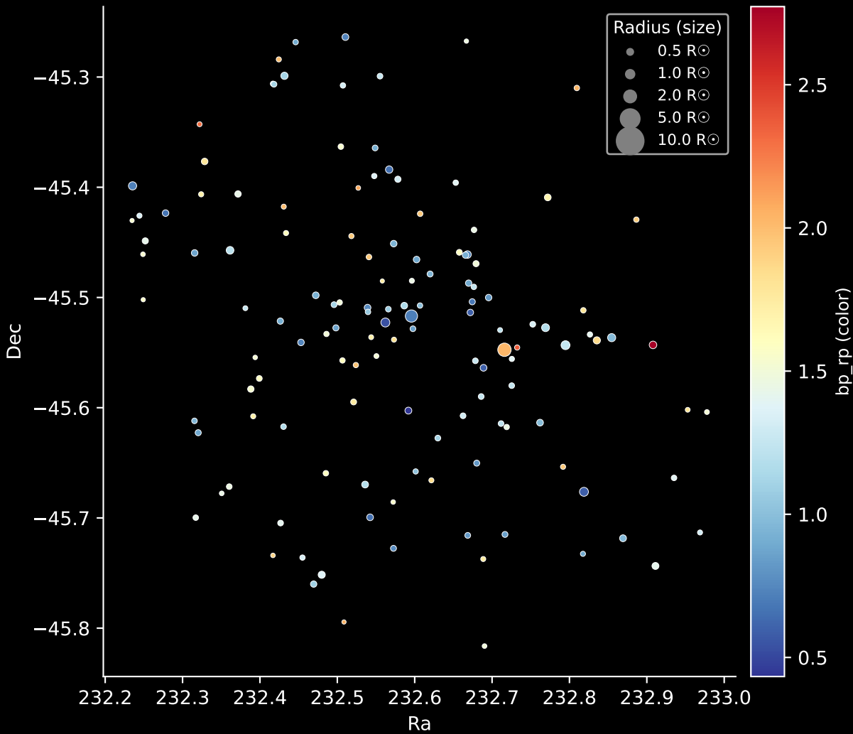
Gaia Cluster: [Gulliver_5] Stars: 133
