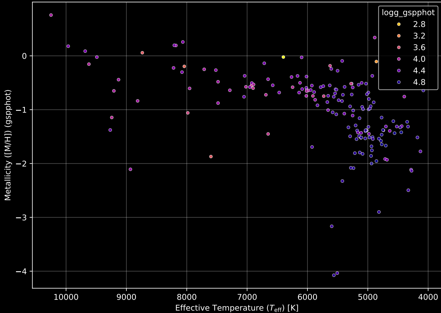
Gaia Cluster: [Gulliver_50] Stellar Population Parameters (n= 168)
