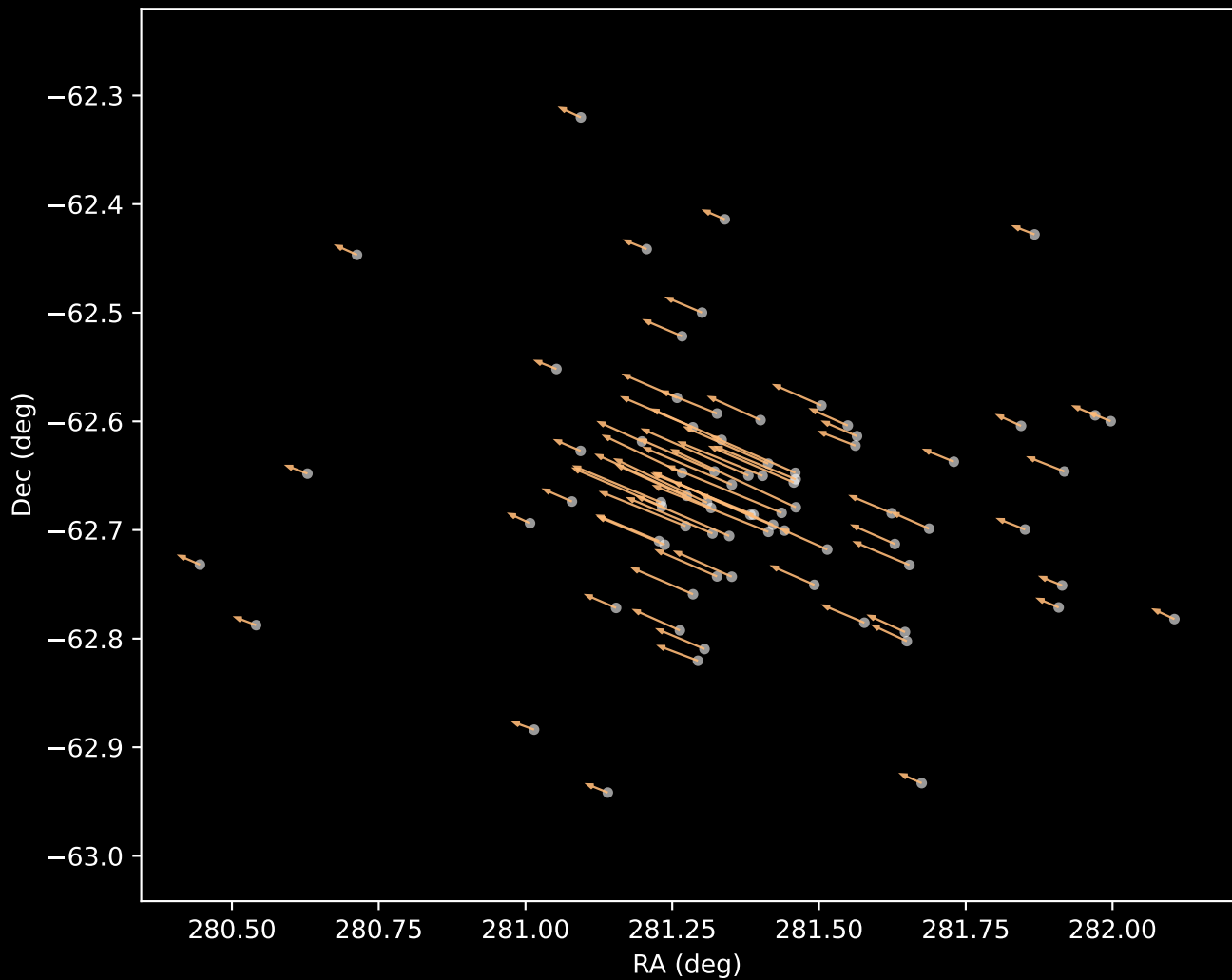
Gaia DR3 Cluster 3 Proper Motion Vectors (n=78)
