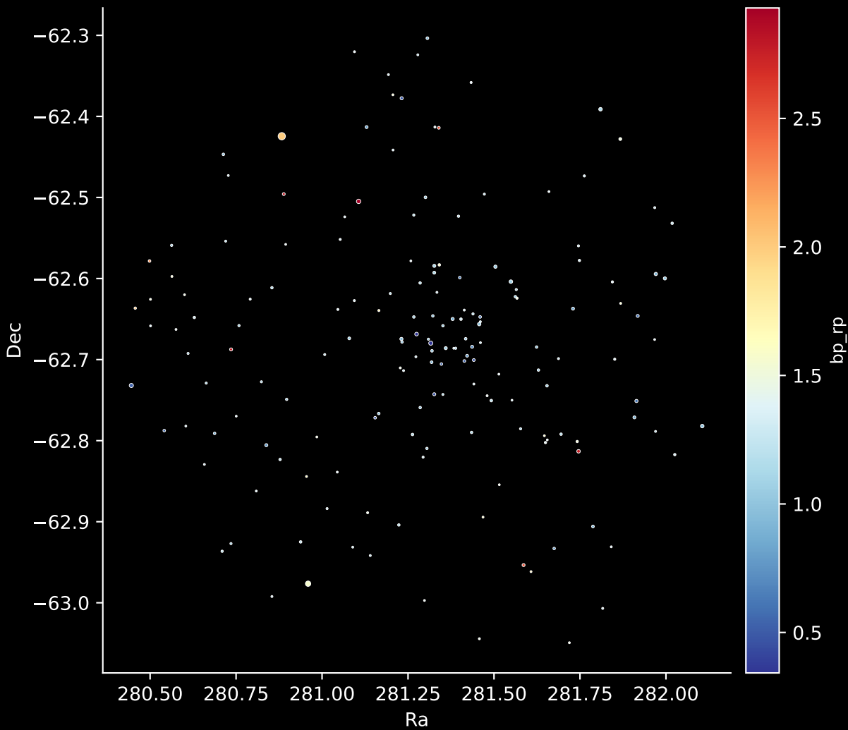
Gaia Cluster: [Gulliver_50] Stars: 168
