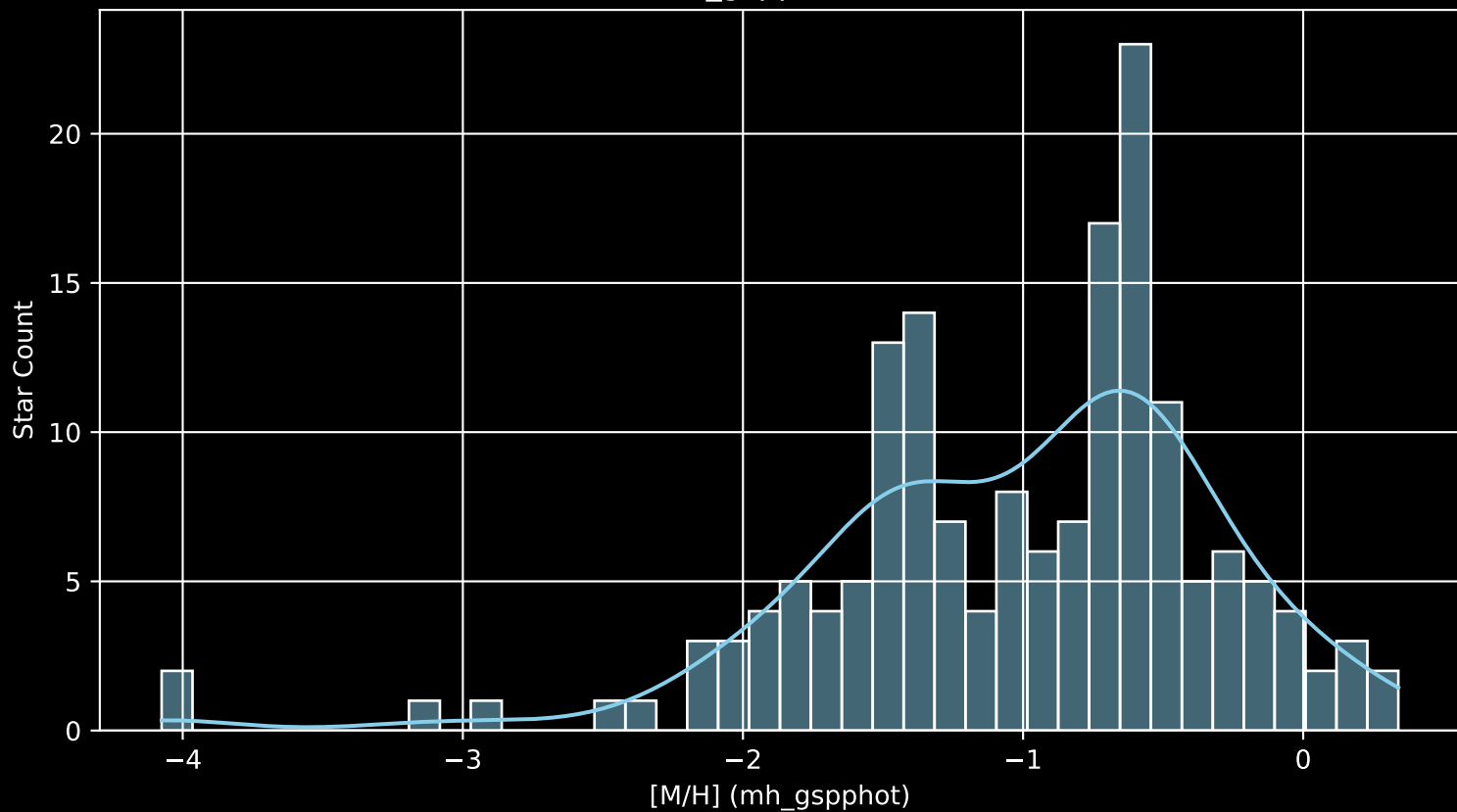
Gaia Cluster: [Gulliver_50 [M/H] (mh_gspphot) (n= 167)
