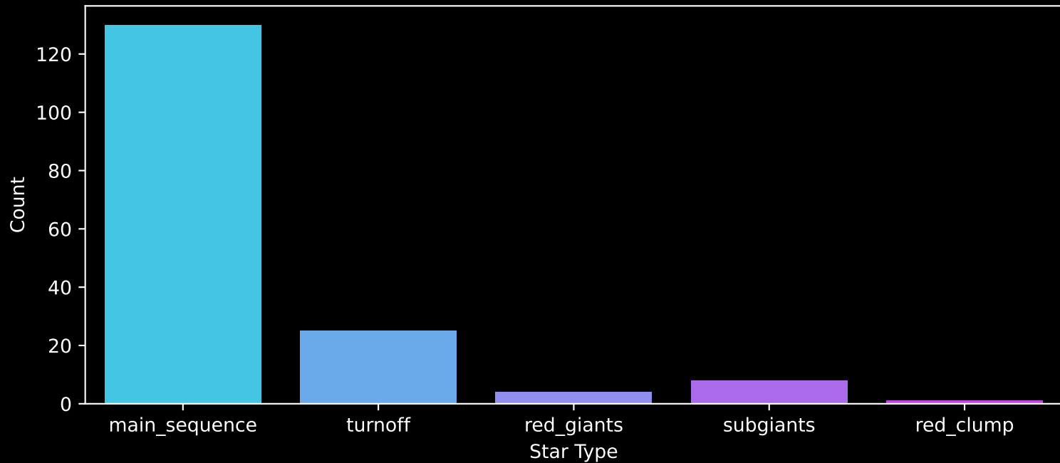
Gaia Cluster: [Gulliver_50] Count plot of Star Type
