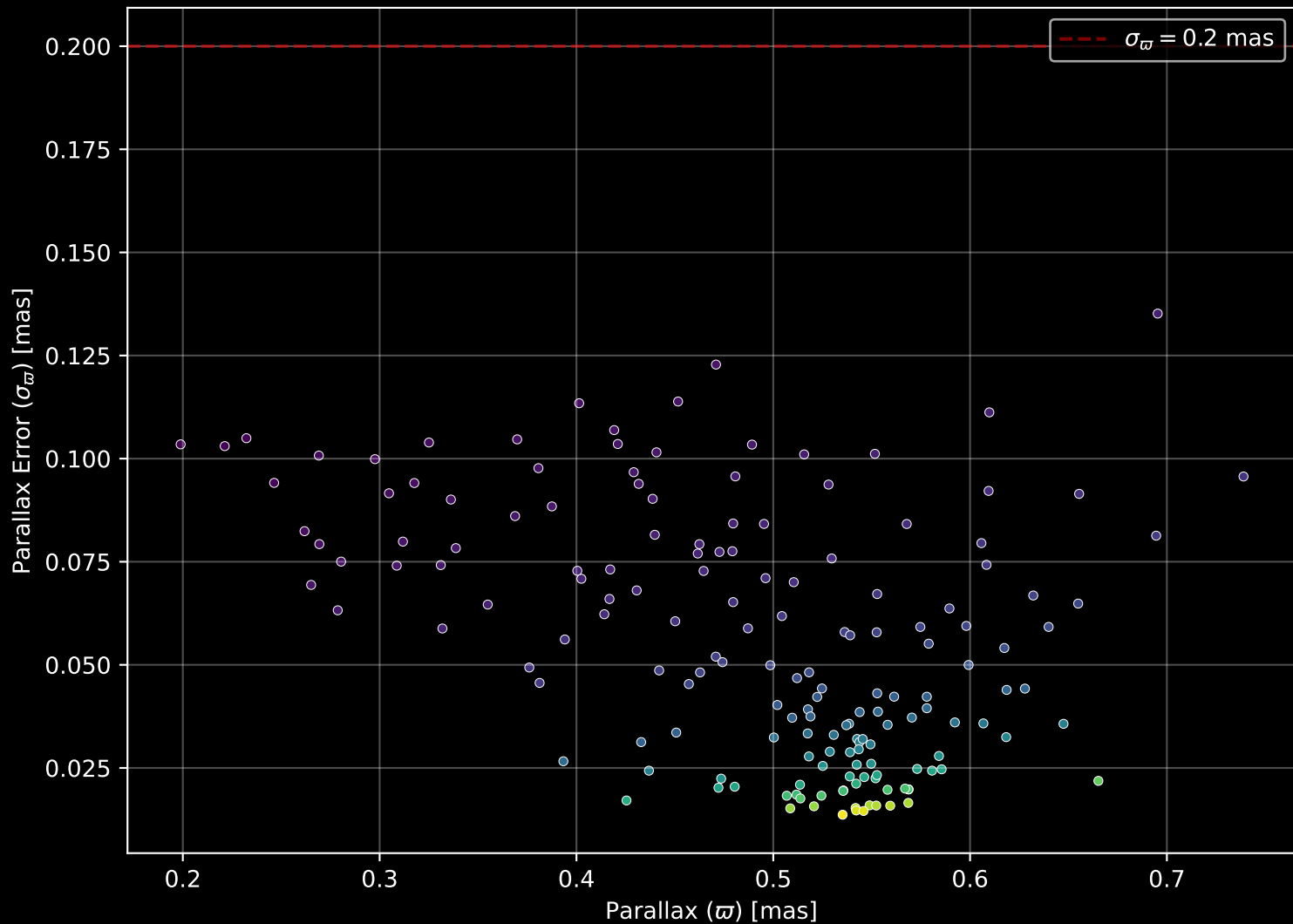
Gaia Cluster: [Gulliver_50] Parallax Quality (n= 168)
