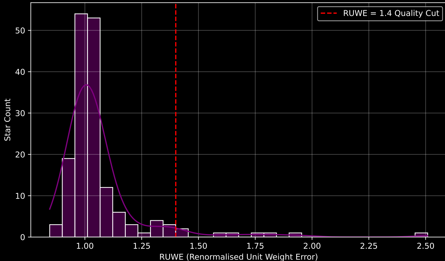
Gaia Cluster: [Gulliver_50] RUWE Distribution (n= 166)
