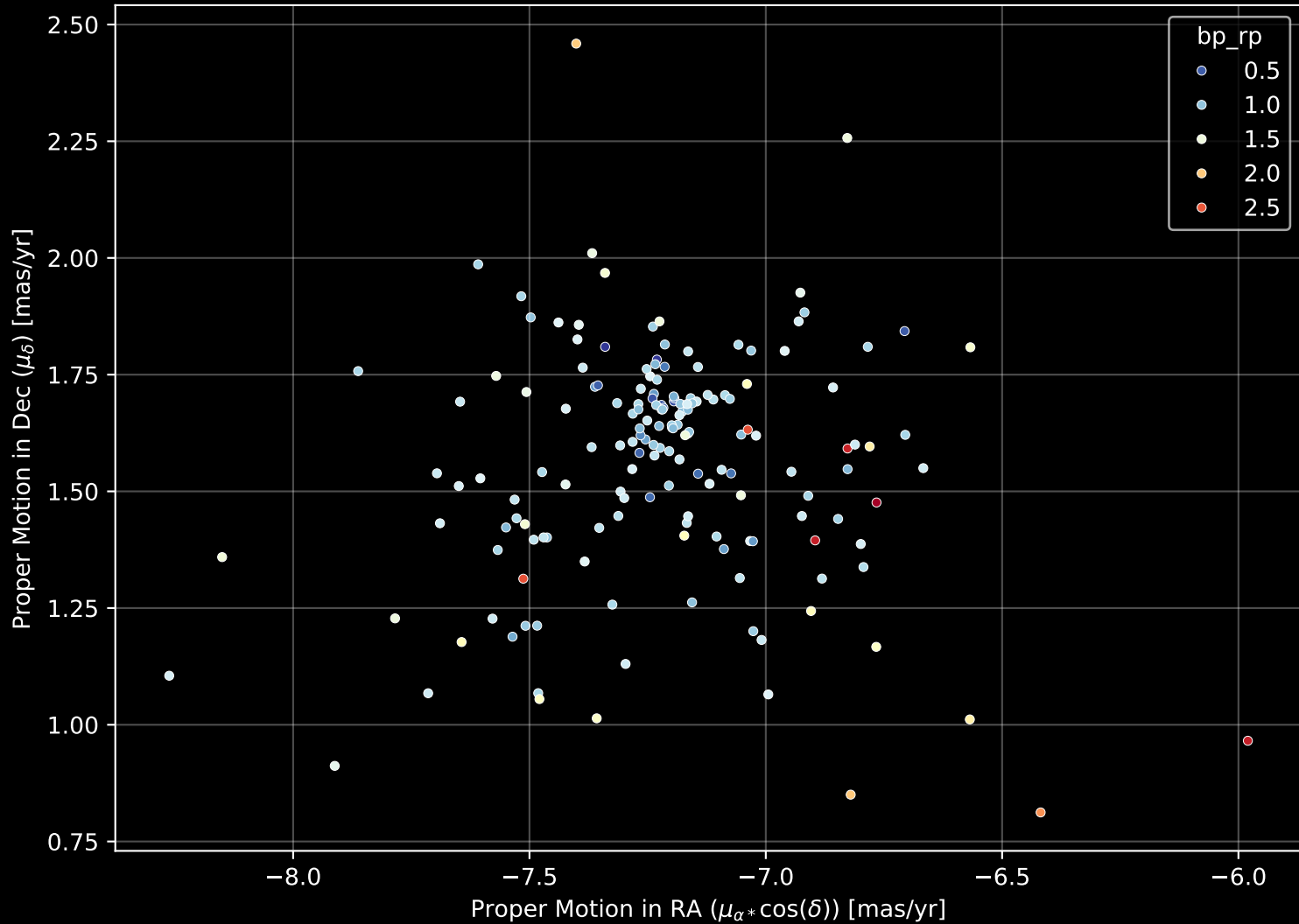
Gaia Cluster: [Gulliver_50] Proper Motion Diagram (n= 168)
