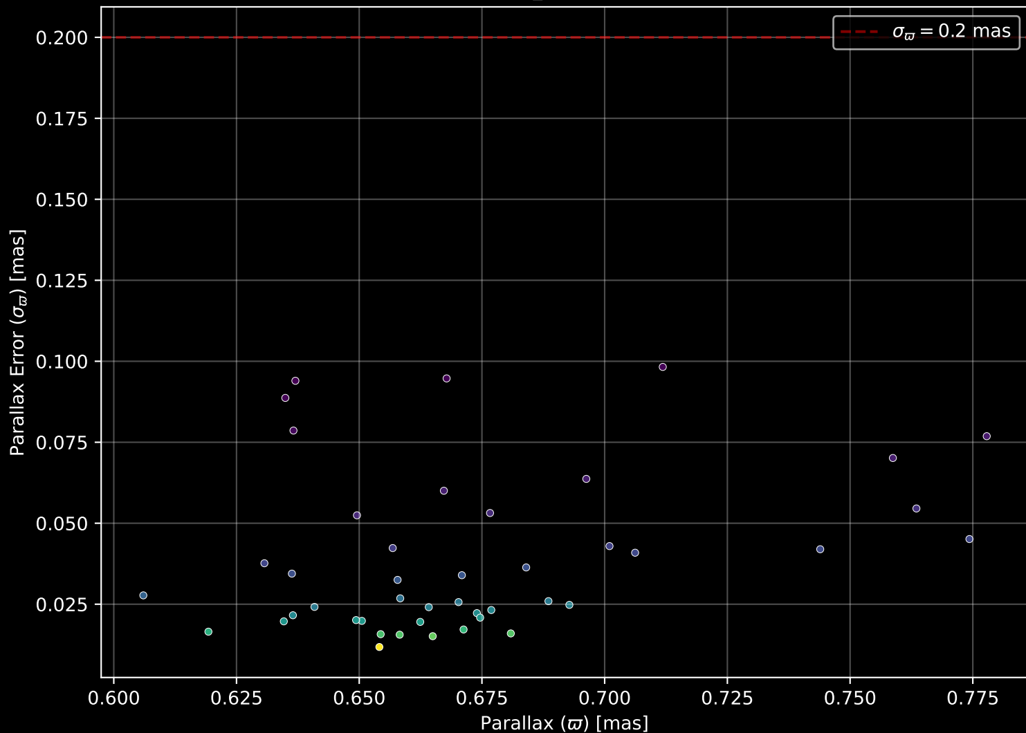
Gaia Cluster: [Gulliver_51] Parallax Quality (n= 44)
