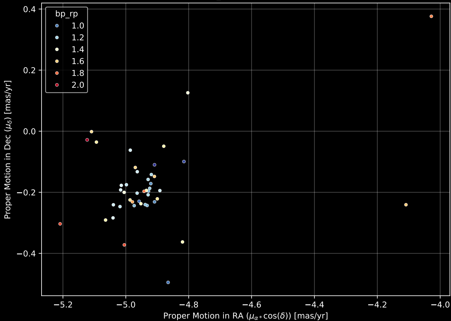
Gaia Cluster: [Gulliver_51] Proper Motion Diagram (n= 44)
