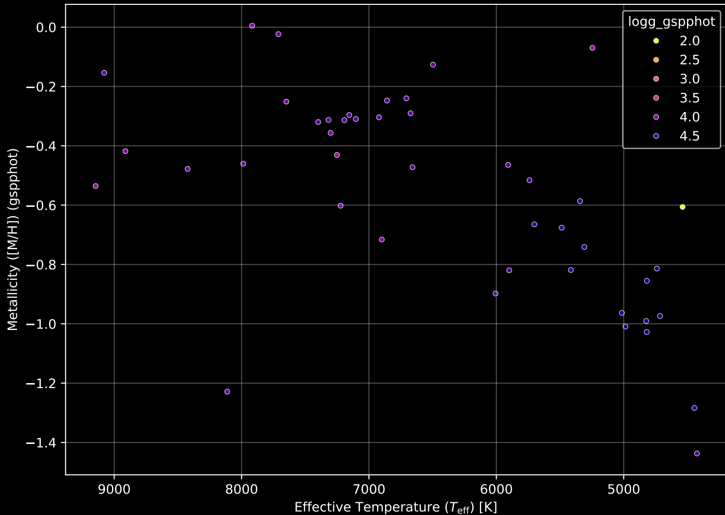
Gaia Cluster: [Gulliver_51] Stellar Population Parameters (n= 44)
