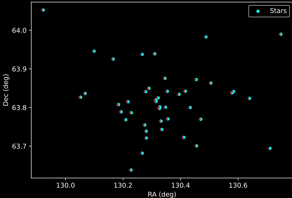
Gaia Cluster: [Gulliver_51] Proper Motion Vectors for Gaia Star Field (n= 44)
