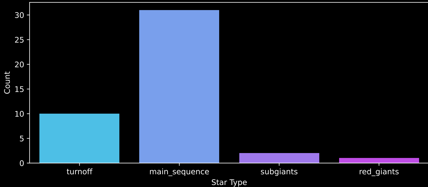
Gaia Cluster: [Gulliver_51] Count plot of Star Type
