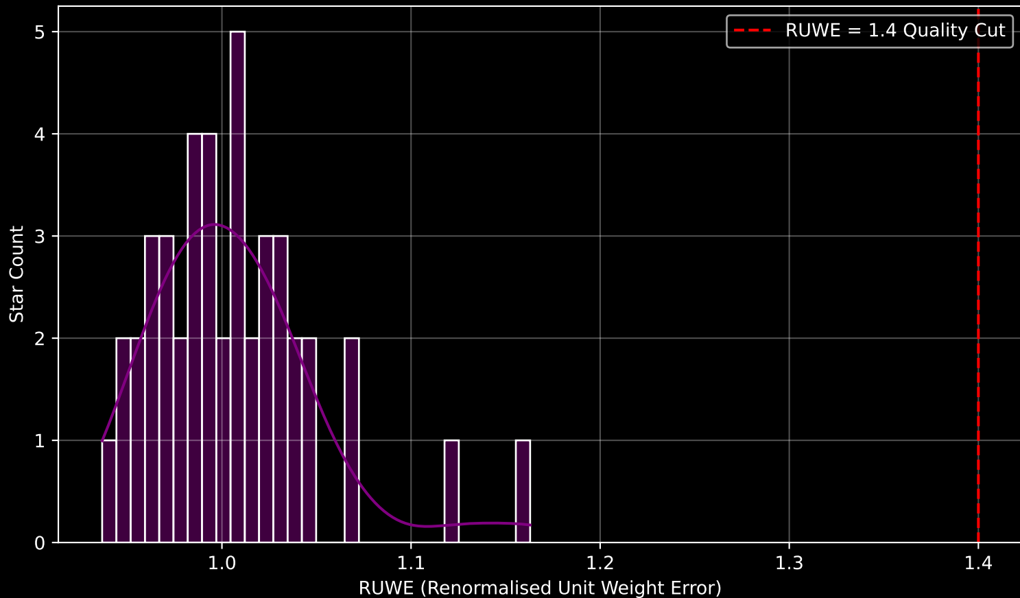
Gaia Cluster: [Gulliver_51] RUWE Distribution (n= 44)
