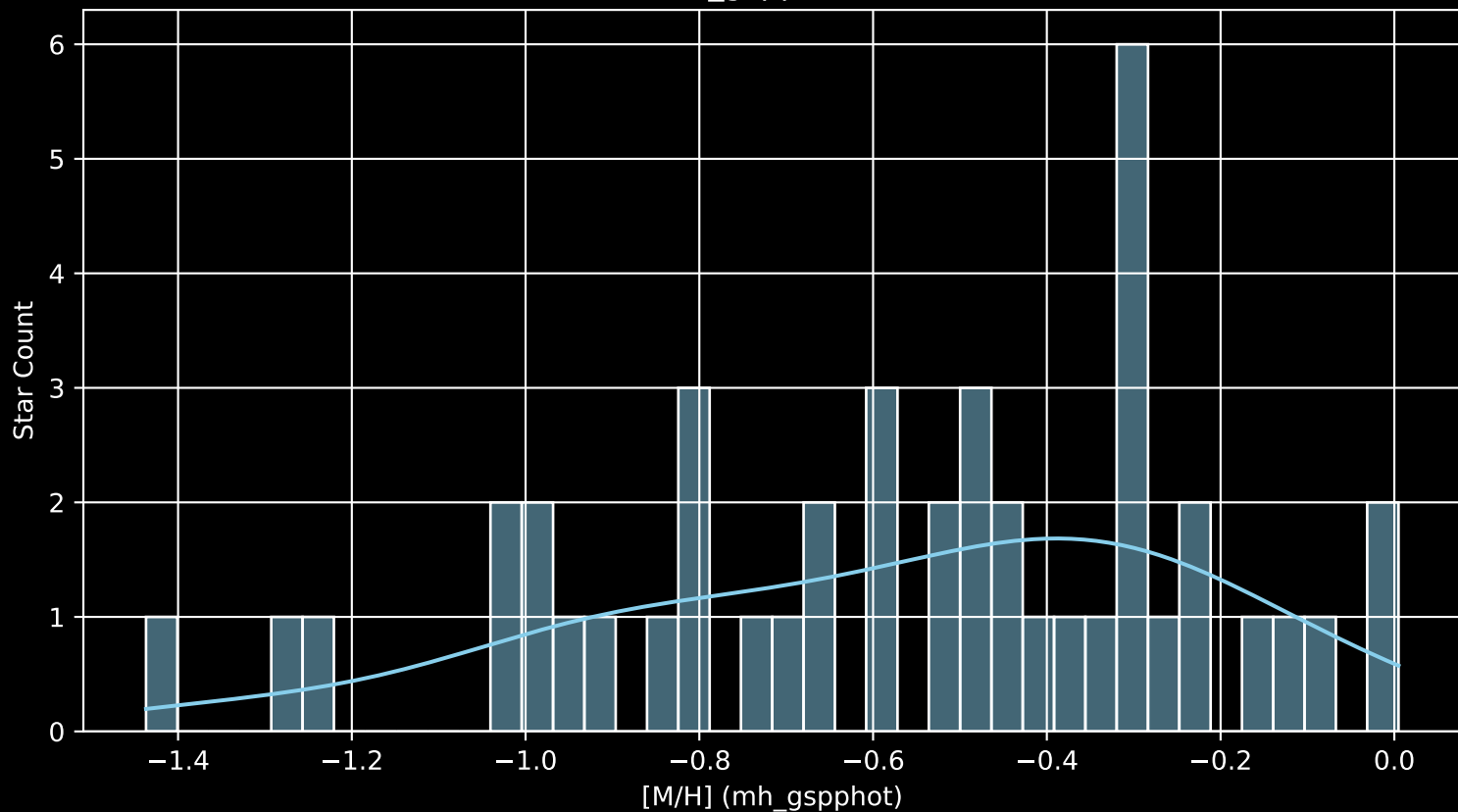
Gaia Cluster: [Gulliver_51 [M/H] (mh_gspphot) (n= 44)
