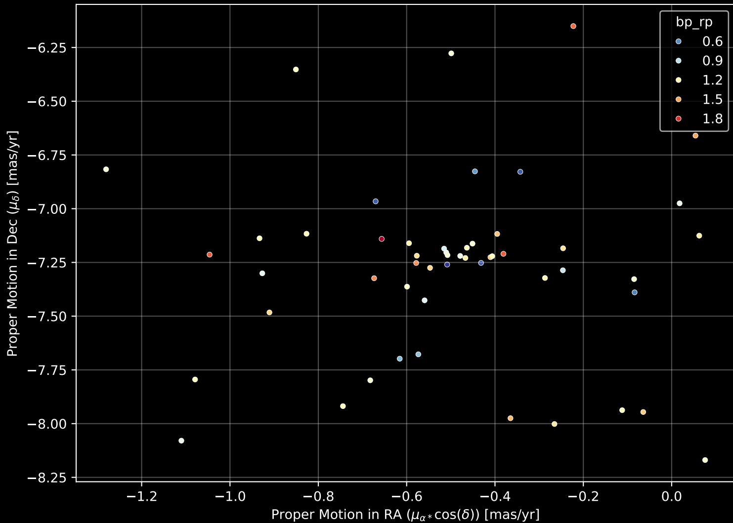
Gaia Cluster: [Gulliver_54] Proper Motion Diagram (n= 52)
