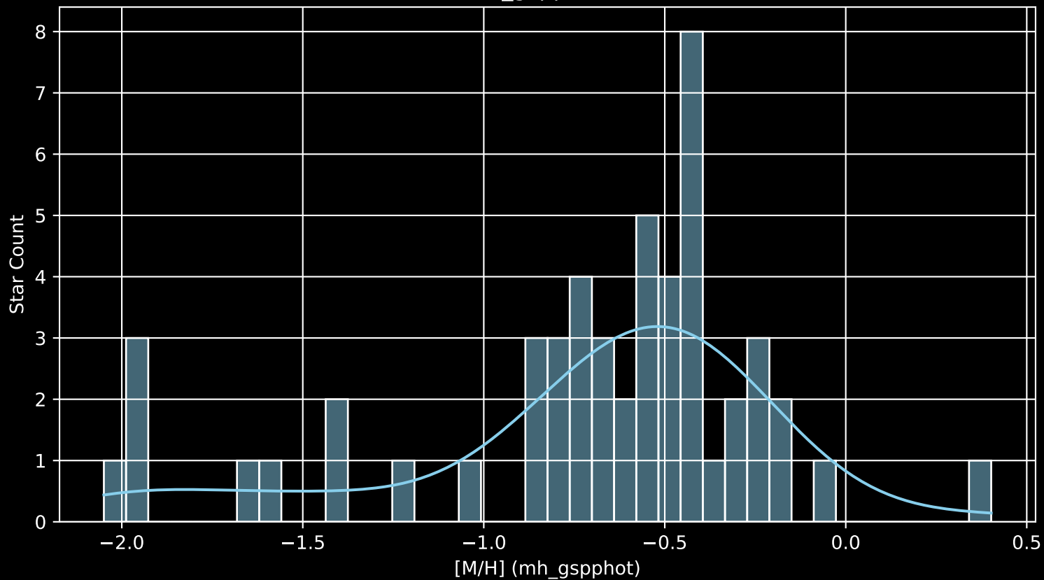
Gaia Cluster: [Gulliver_54 [M/H] (mh_gspphot) (n= 52)
