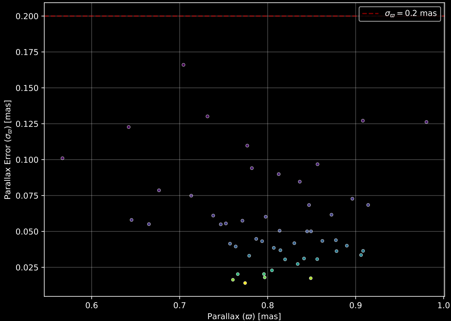
Gaia Cluster: [Gulliver_54] Parallax Quality (n= 52)
