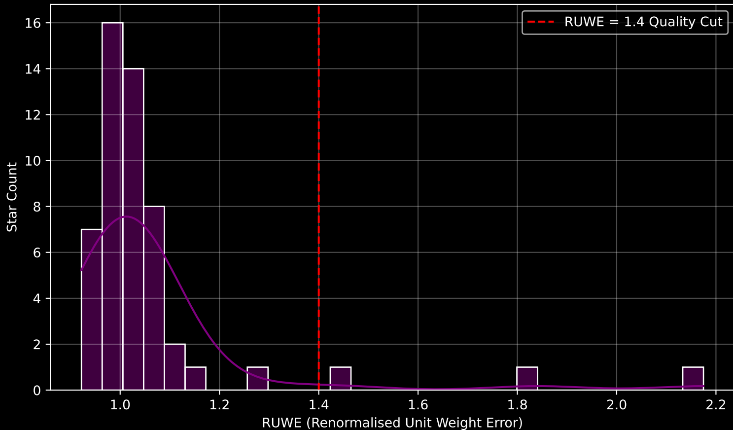
Gaia Cluster: [Gulliver_54] RUWE Distribution (n= 52)
