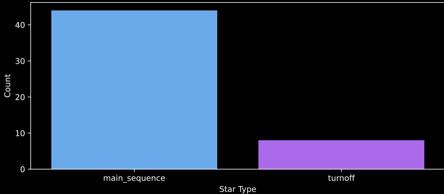
Gaia Cluster: [Gulliver_54] Count plot of Star Type
