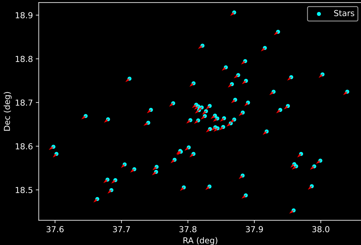
Gaia Cluster: [Gulliver_55] Proper Motion Vectors for Gaia Star Field (n= 70)
