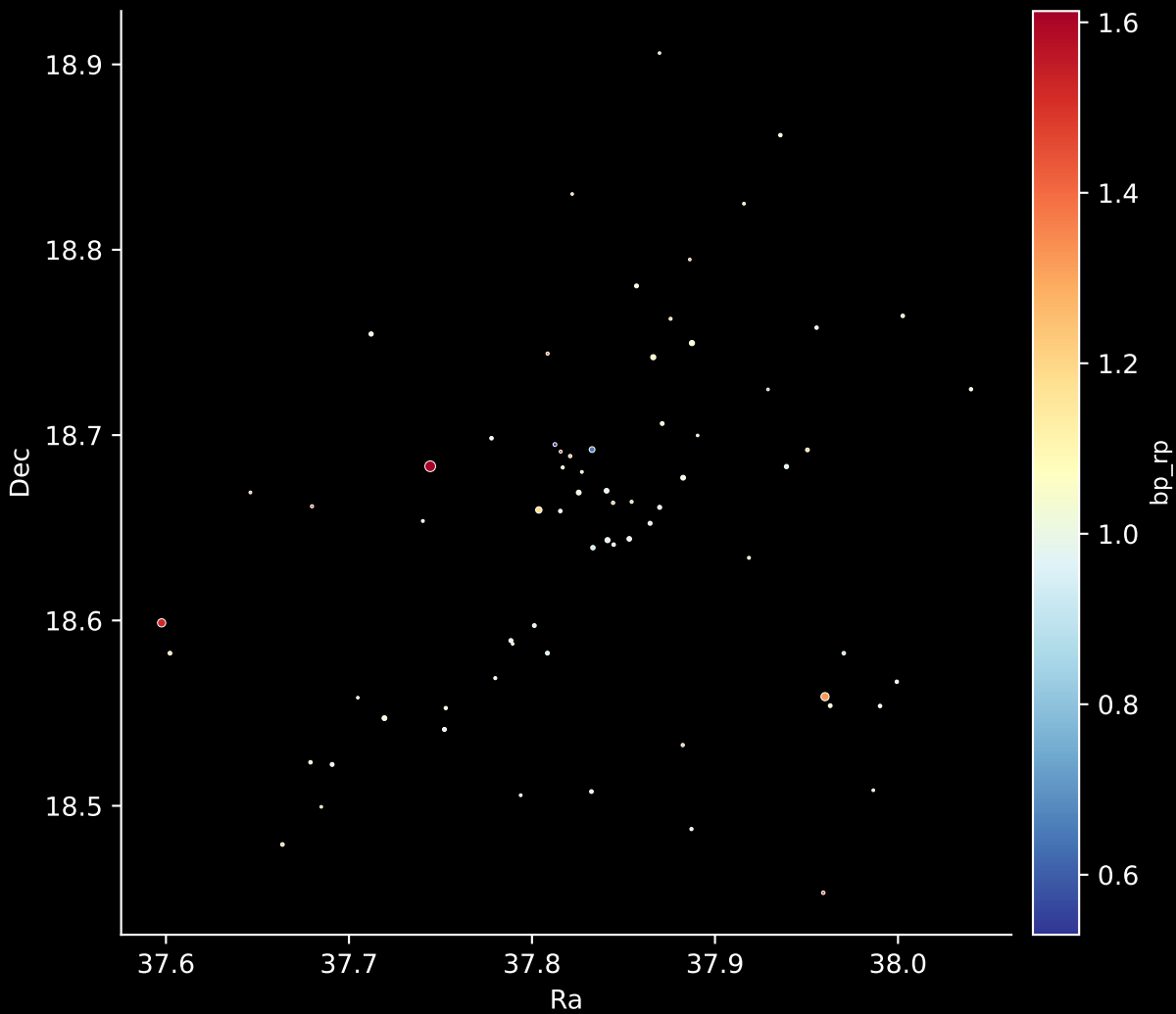
Gaia Cluster: [Gulliver_55] Stars: 70
