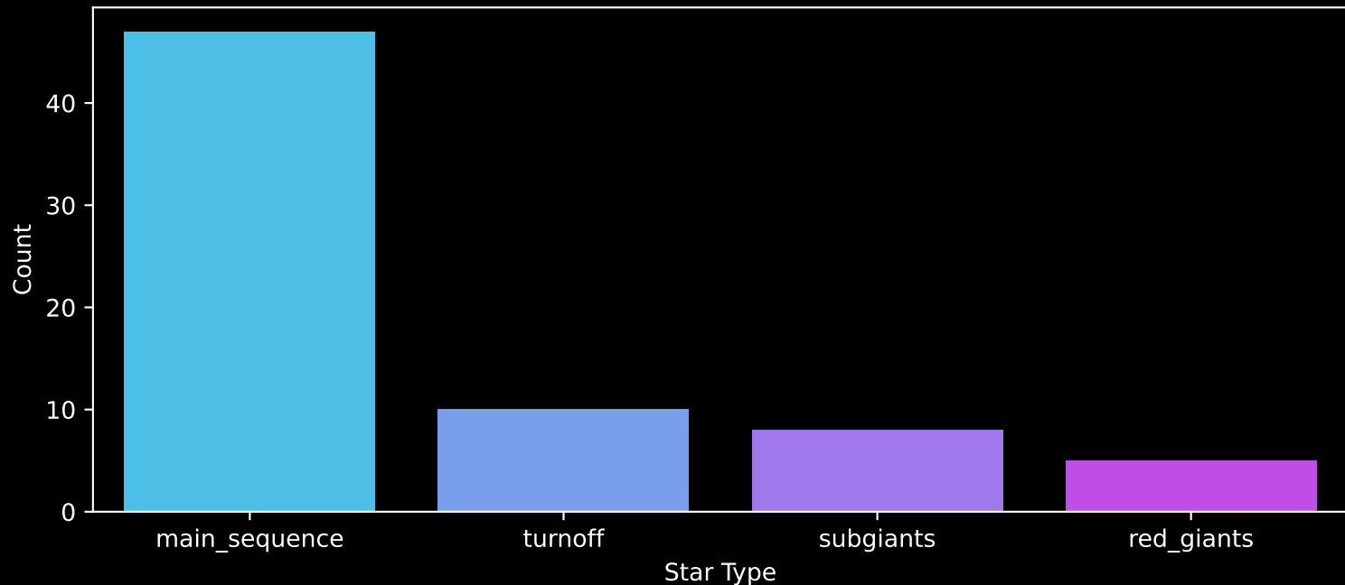
Gaia Cluster: [Gulliver_55] Count plot of Star Type
