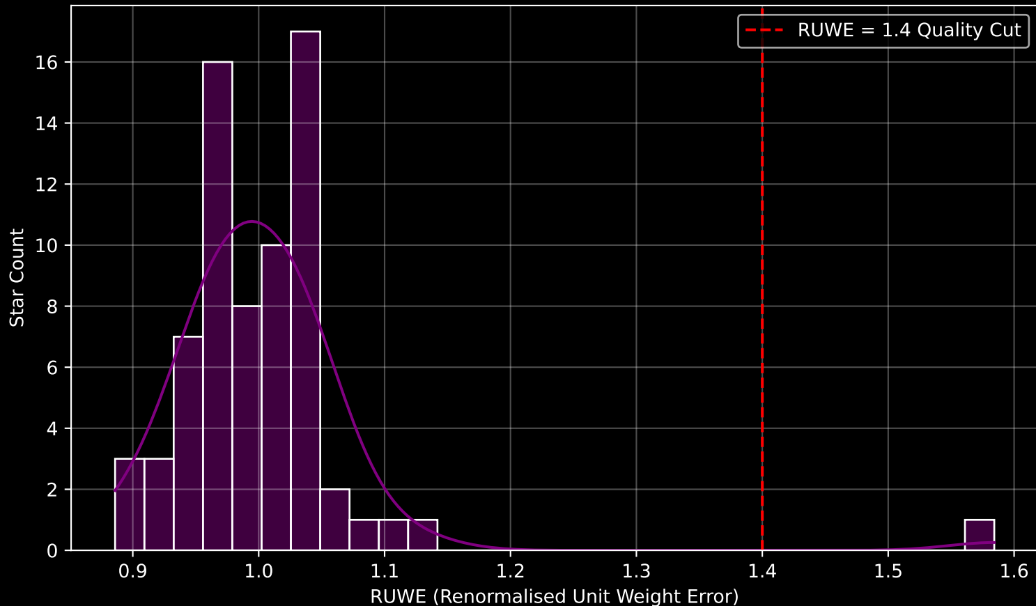
Gaia Cluster: [Gulliver_55] RUWE Distribution (n= 70)
