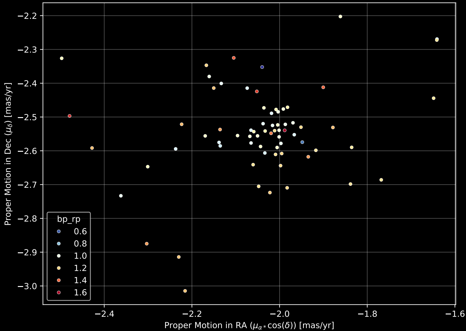
Gaia Cluster: [Gulliver_55] Proper Motion Diagram (n= 70)
