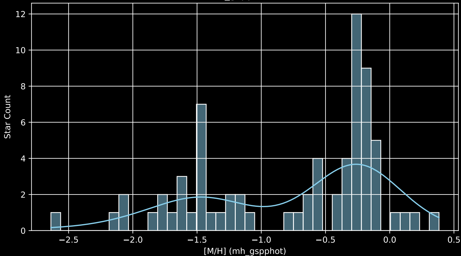
Gaia Cluster: [Gulliver_55 [M/H] (mh_gspphot) (n= 70)
