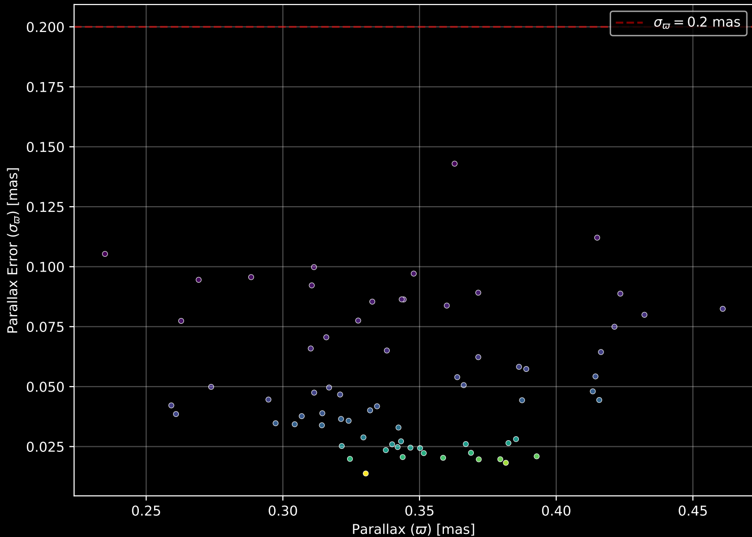
Gaia Cluster: [Gulliver_55] Parallax Quality (n= 70)
