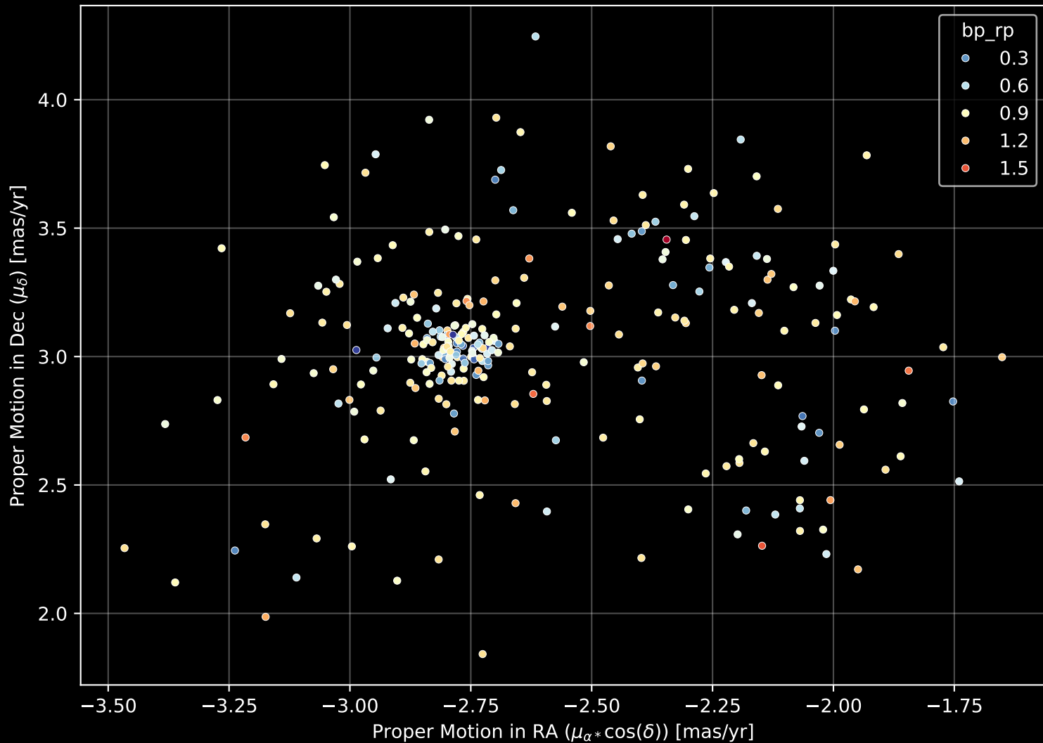
Gaia Cluster: [Haffner_16] Proper Motion Diagram (n= 286)
