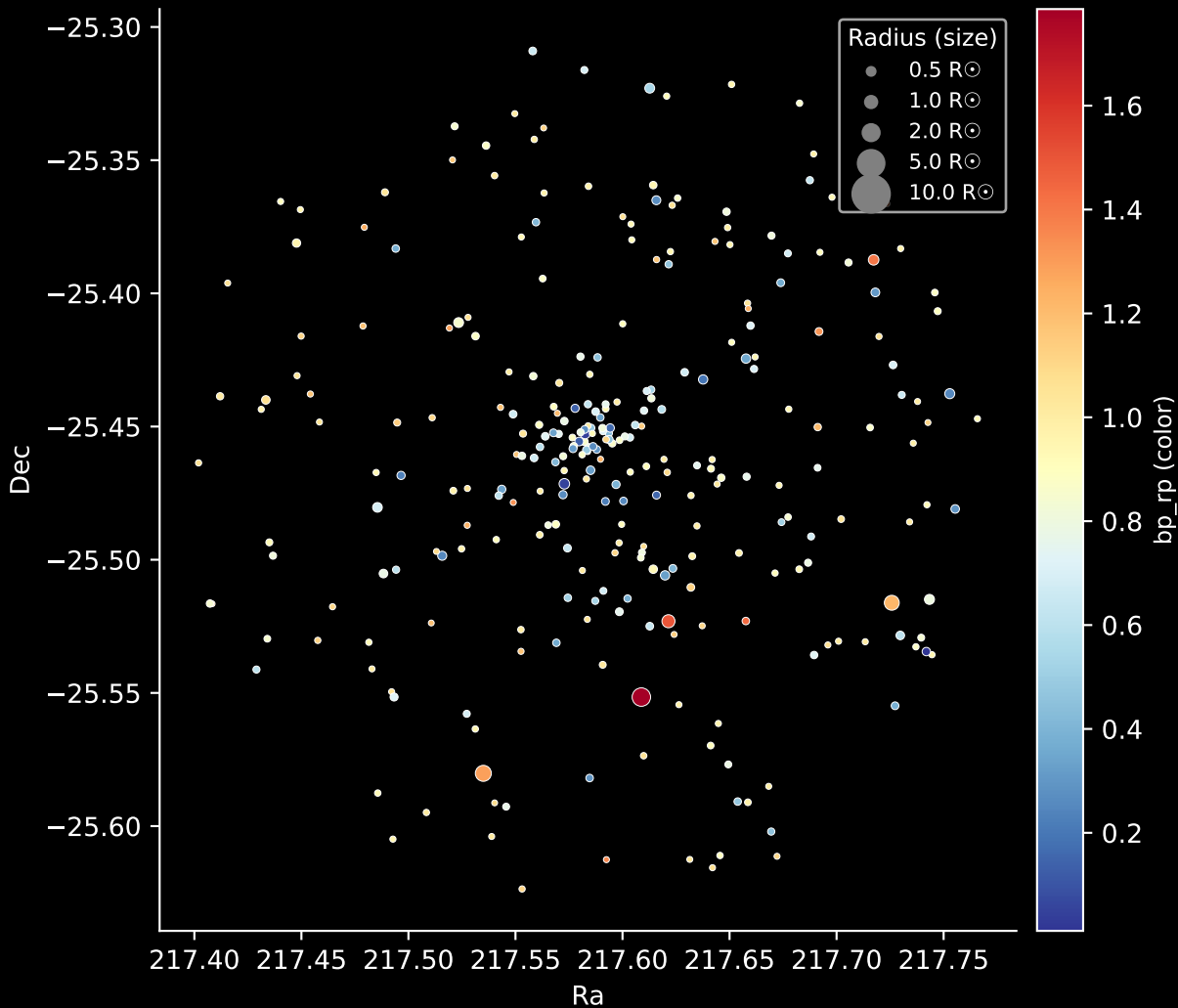
Gaia Cluster: [Haffner_16] Stars: 286
