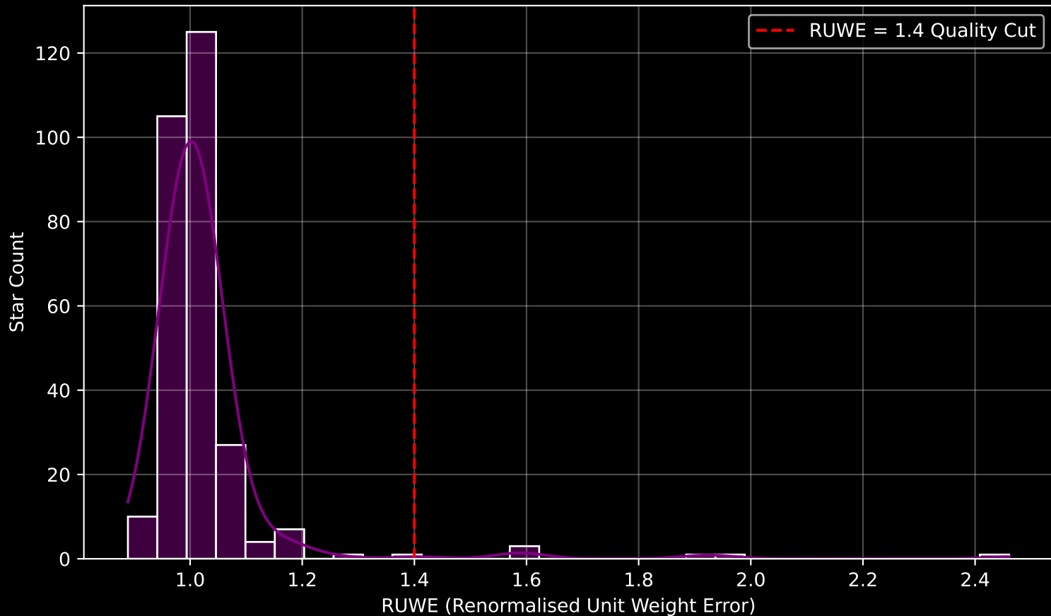
Gaia Cluster: [Haffner_16] RUWE Distribution (n= 286)
