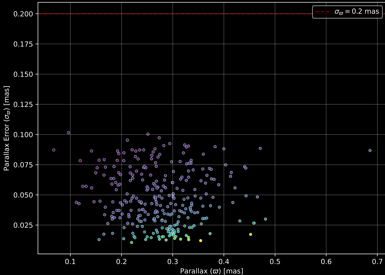
Gaia Cluster: [Haffner_16] Parallax Quality (n= 286)
