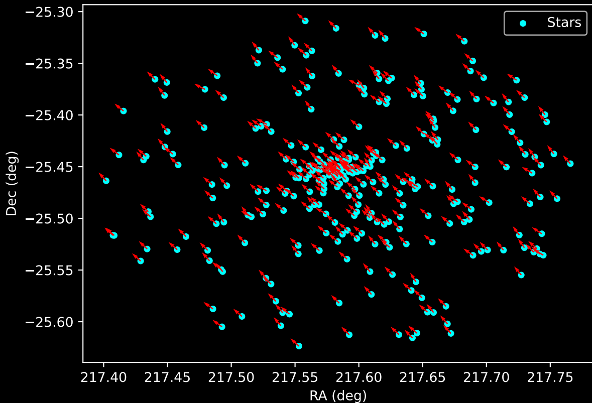
Gaia Cluster: [Haffner_16] Proper Motion Vectors for Gaia Star Field (n= 286)
