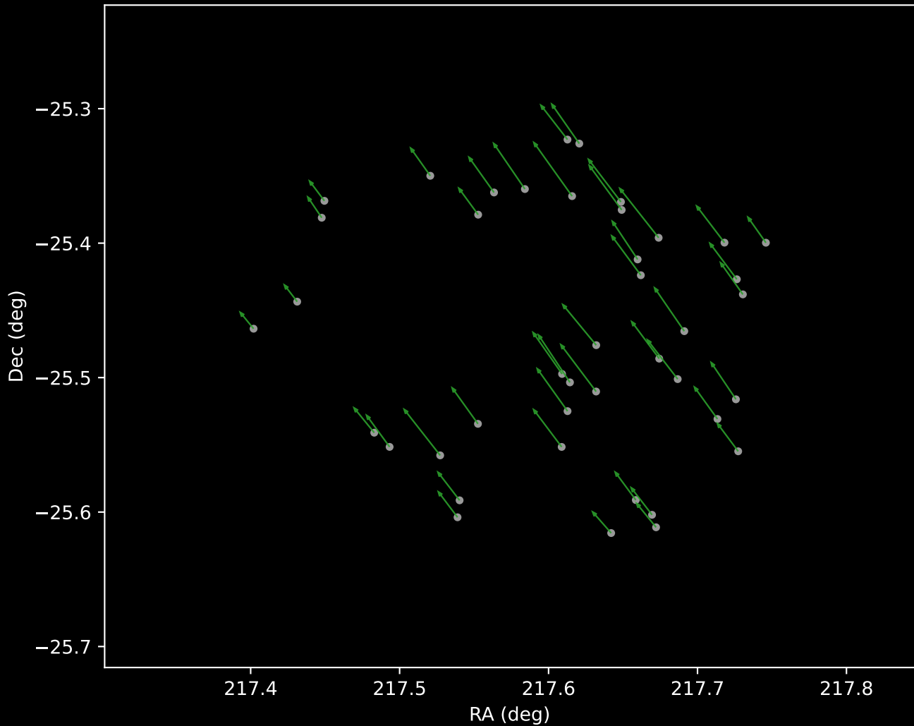
Gaia DR3 Cluster 4 Proper Motion Vectors (n=42)
