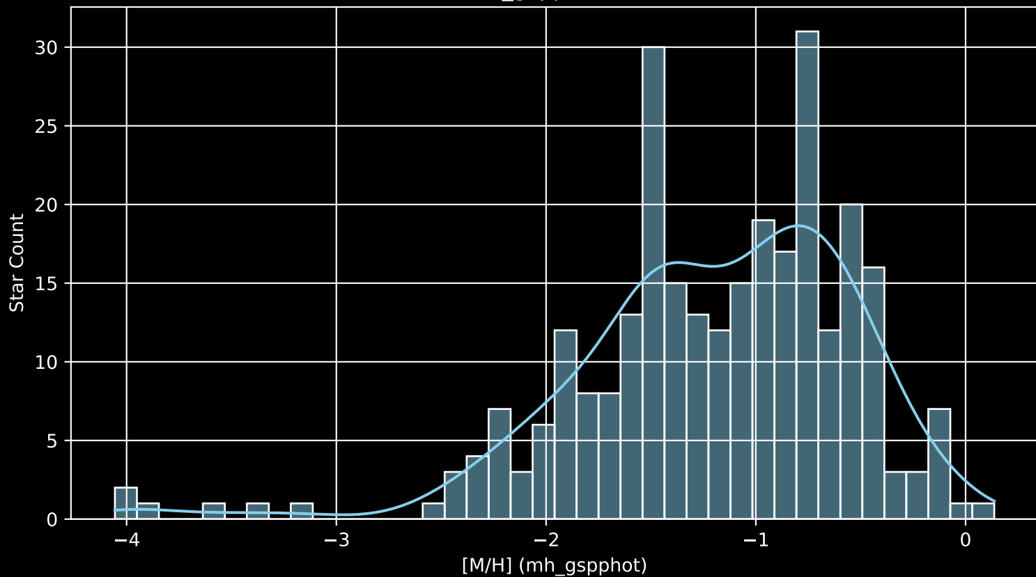
Gaia Cluster: [Haffner_16 [M/H] (mh_gspphot) (n= 286)
