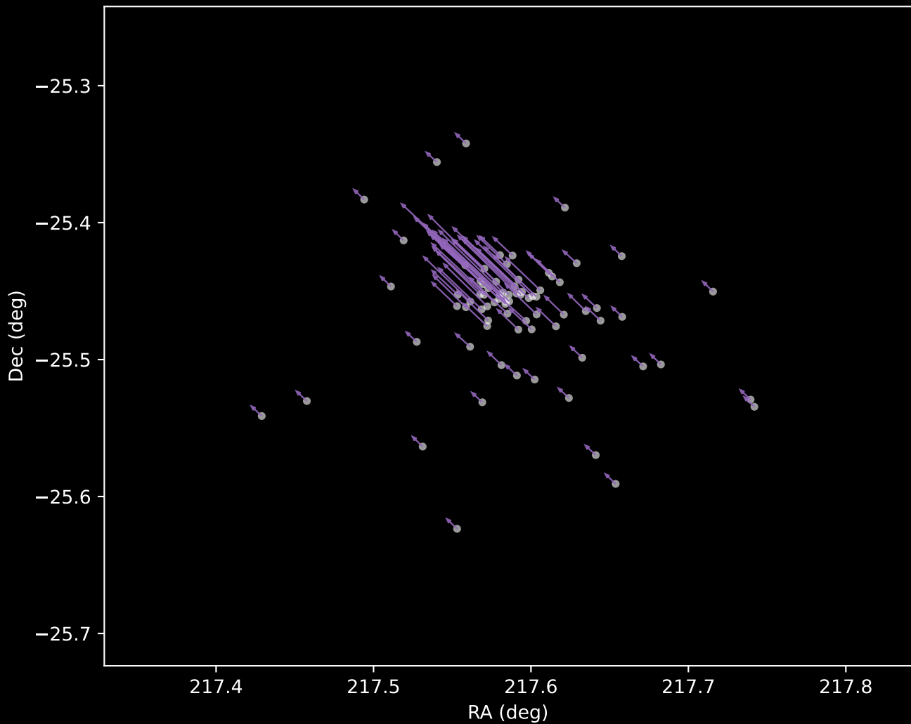
Gaia DR3 Cluster 8 Proper Motion Vectors (n=78)
