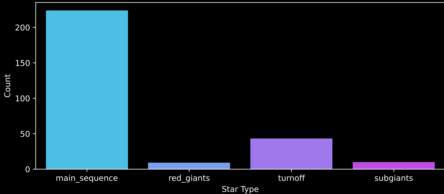
Gaia Cluster: [Haffner_16] Count plot of Star Type
