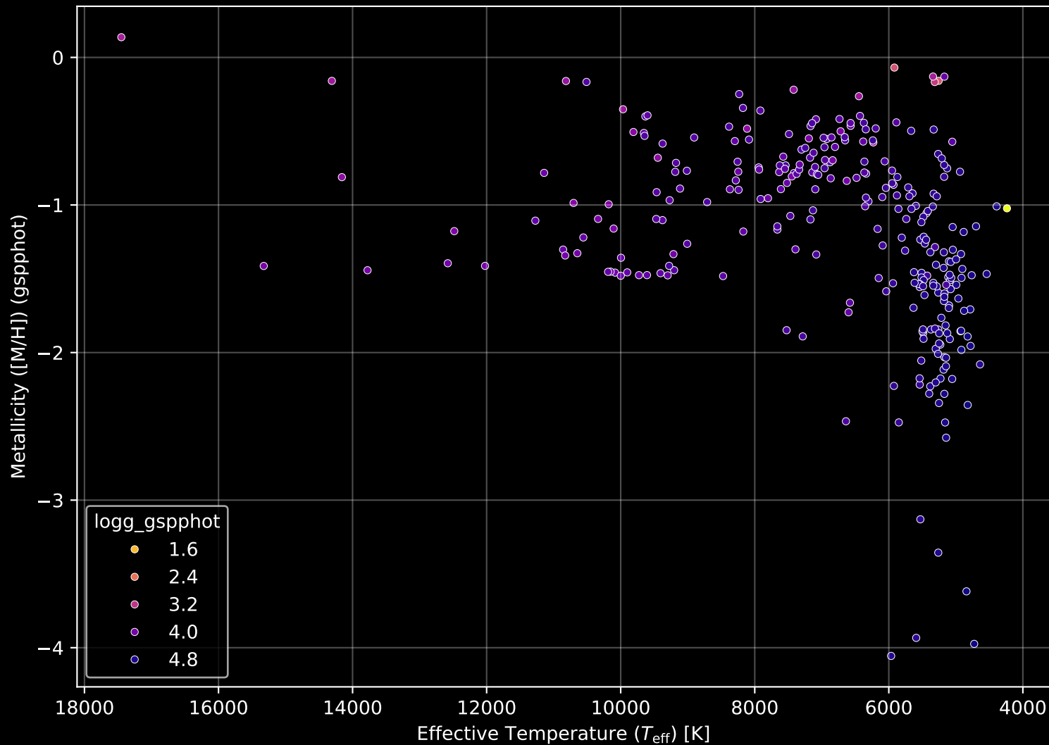
Gaia Cluster: [Haffner_16] Stellar Population Parameters (n= 286)
