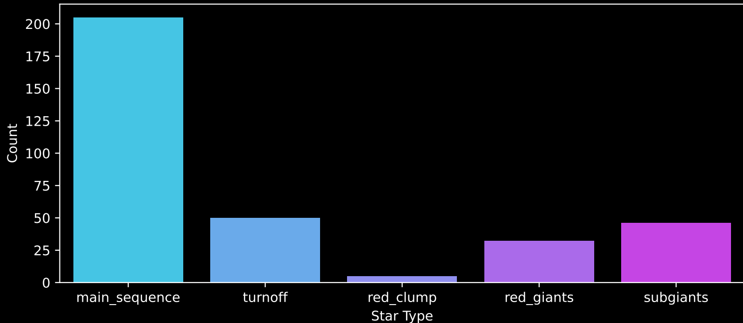
Gaia Cluster: [Haffner_22] Count plot of Star Type
