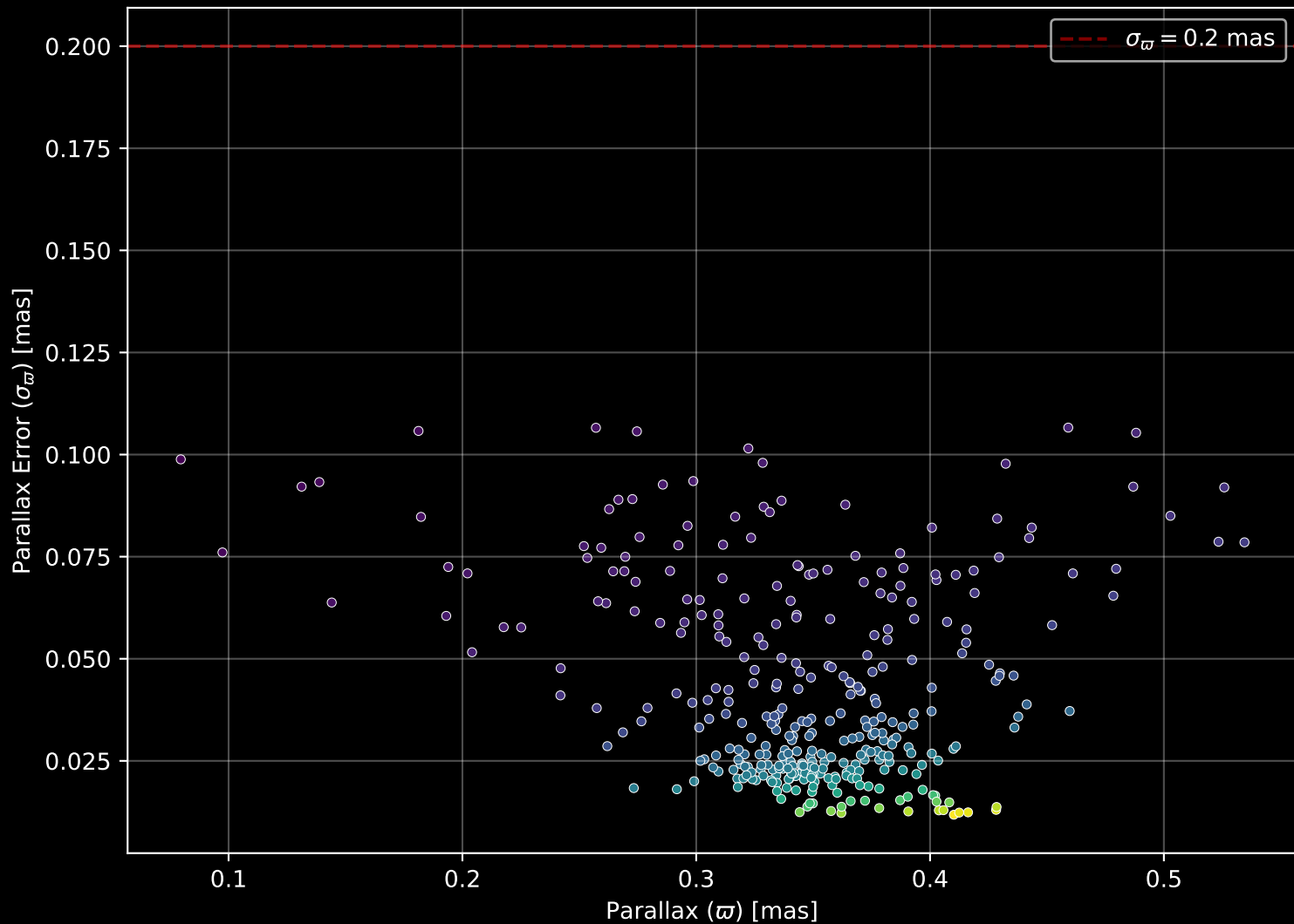
Gaia Cluster: [Haffner_22] Parallax Quality (n= 338)
