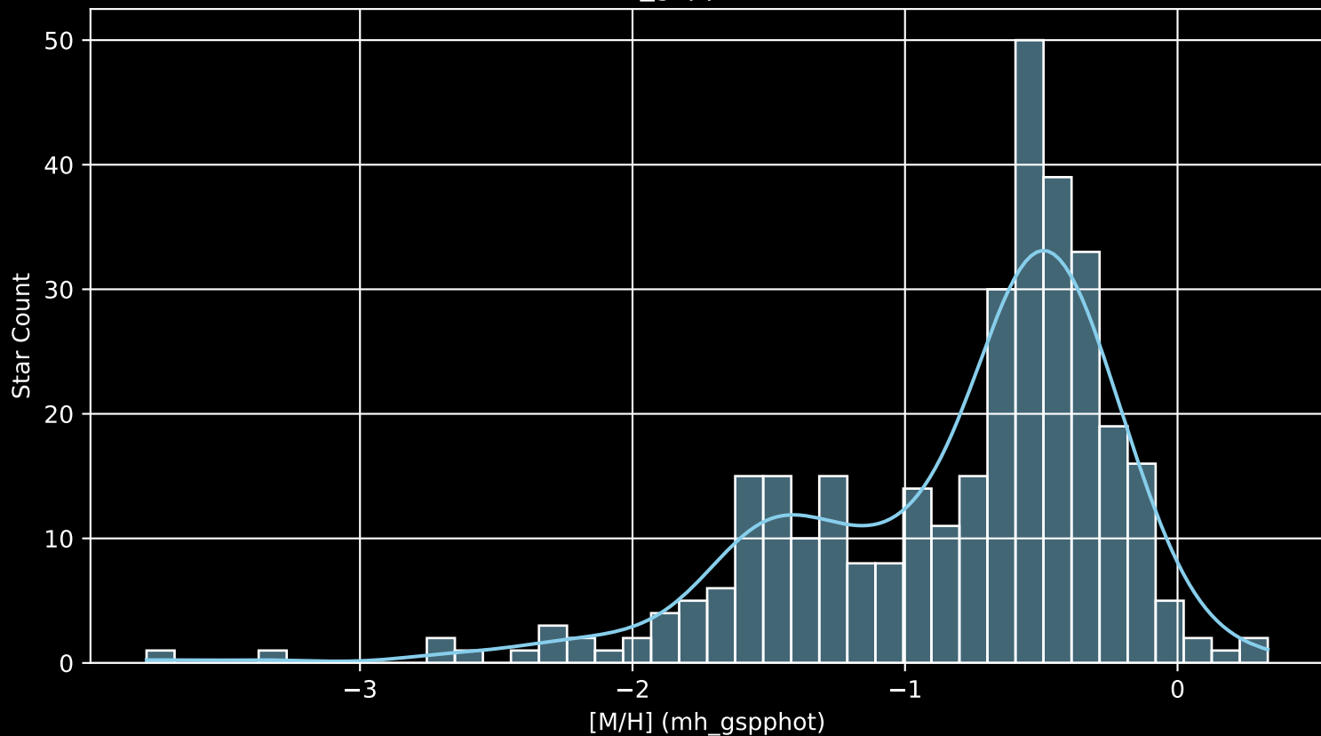
Gaia Cluster: [Haffner_22 [M/H] (mh_gspphot) (n= 337)
