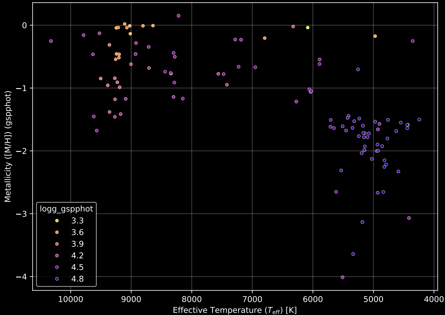
Gaia Cluster: [Haffner_3] Stellar Population Parameters (n= 110)
