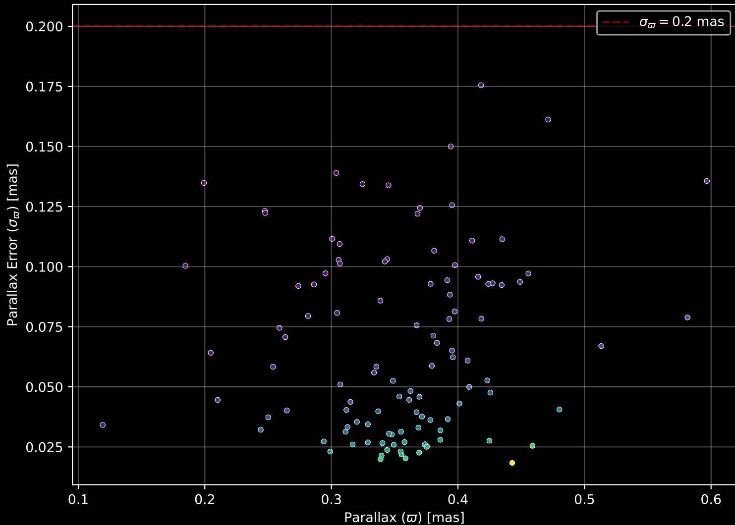
Gaia Cluster: [Haffner_3] Parallax Quality (n= 110)
