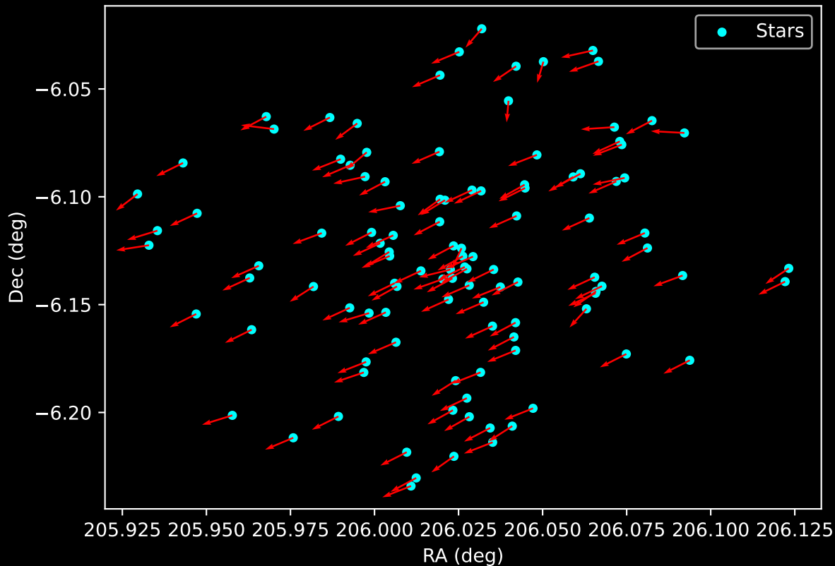
Gaia Cluster: [Haffner_3] Proper Motion Vectors for Gaia Star Field (n= 110)
