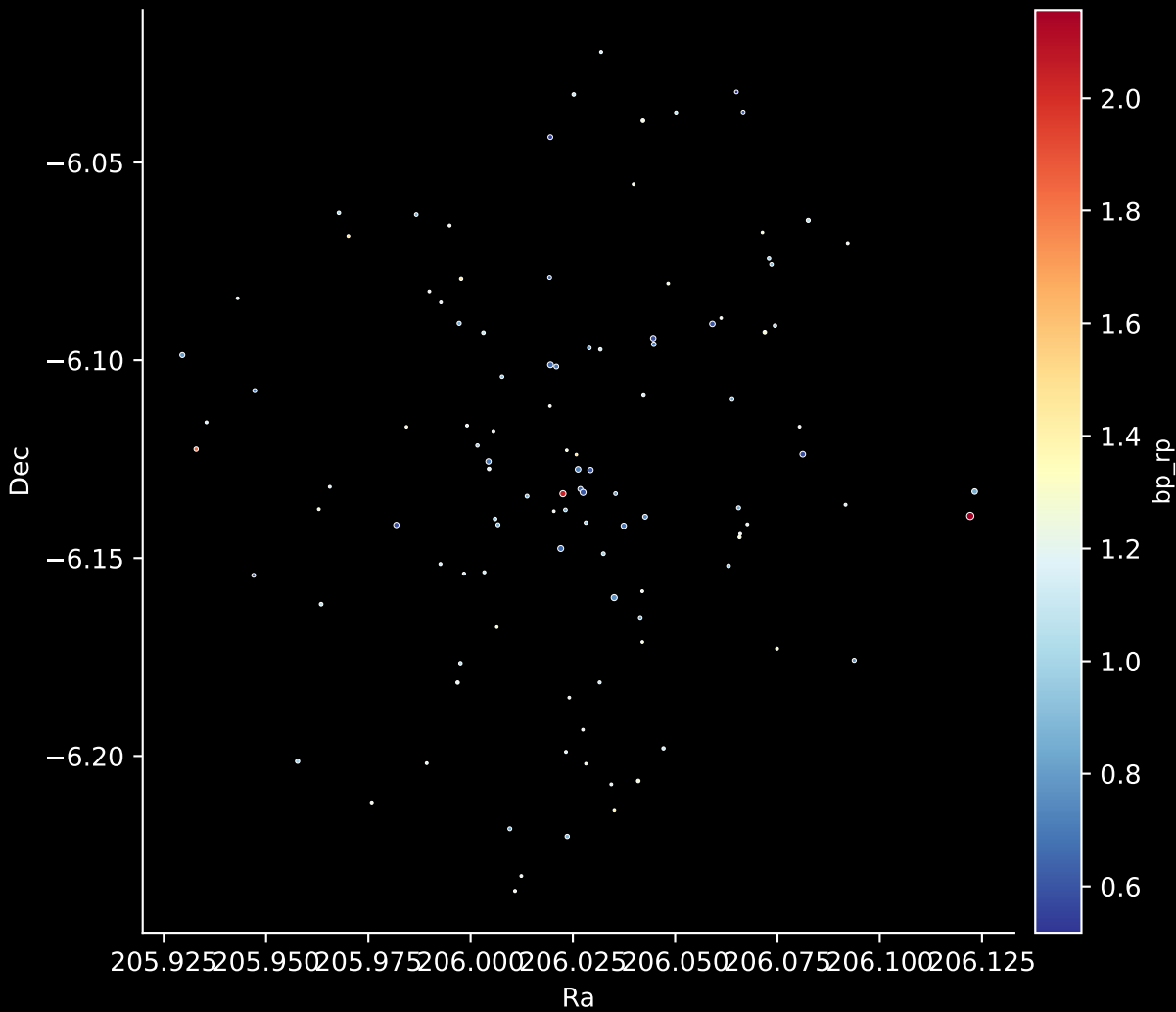
Gaia Cluster: [Haffner_3] Stars: 110
