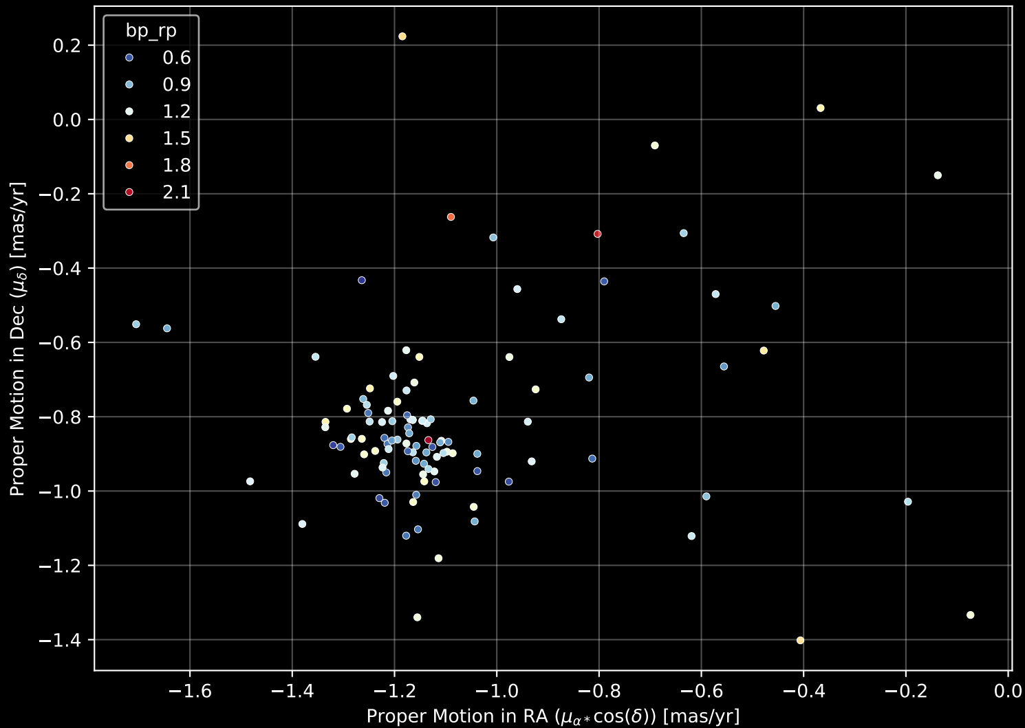
Gaia Cluster: [Haffner_3] Proper Motion Diagram (n= 110)
