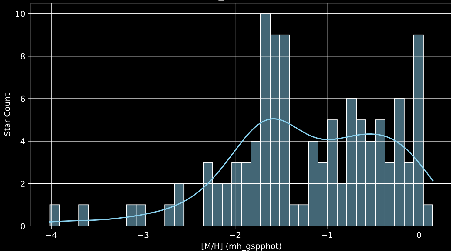
Gaia Cluster: [Haffner_3 [M/H] (mh_gspphot) (n= 110)
