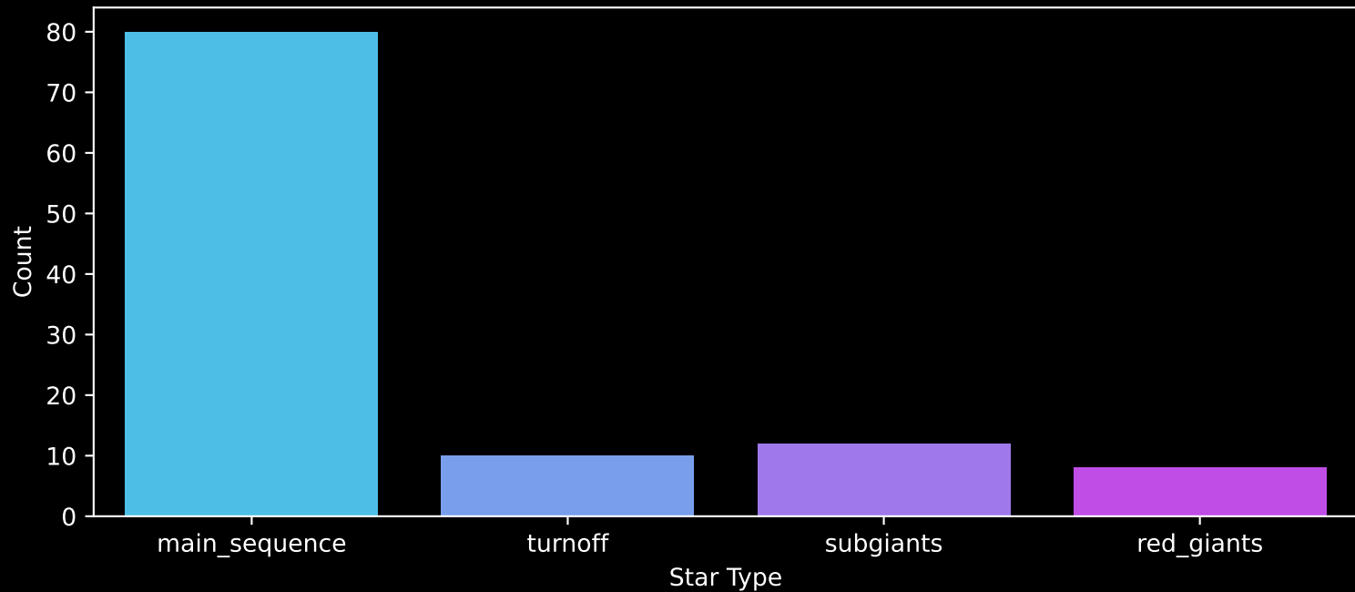
Gaia Cluster: [Haffner_3] Count plot of Star Type
