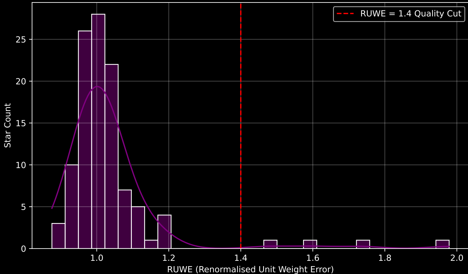
Gaia Cluster: [Haffner_3] RUWE Distribution (n= 110)
