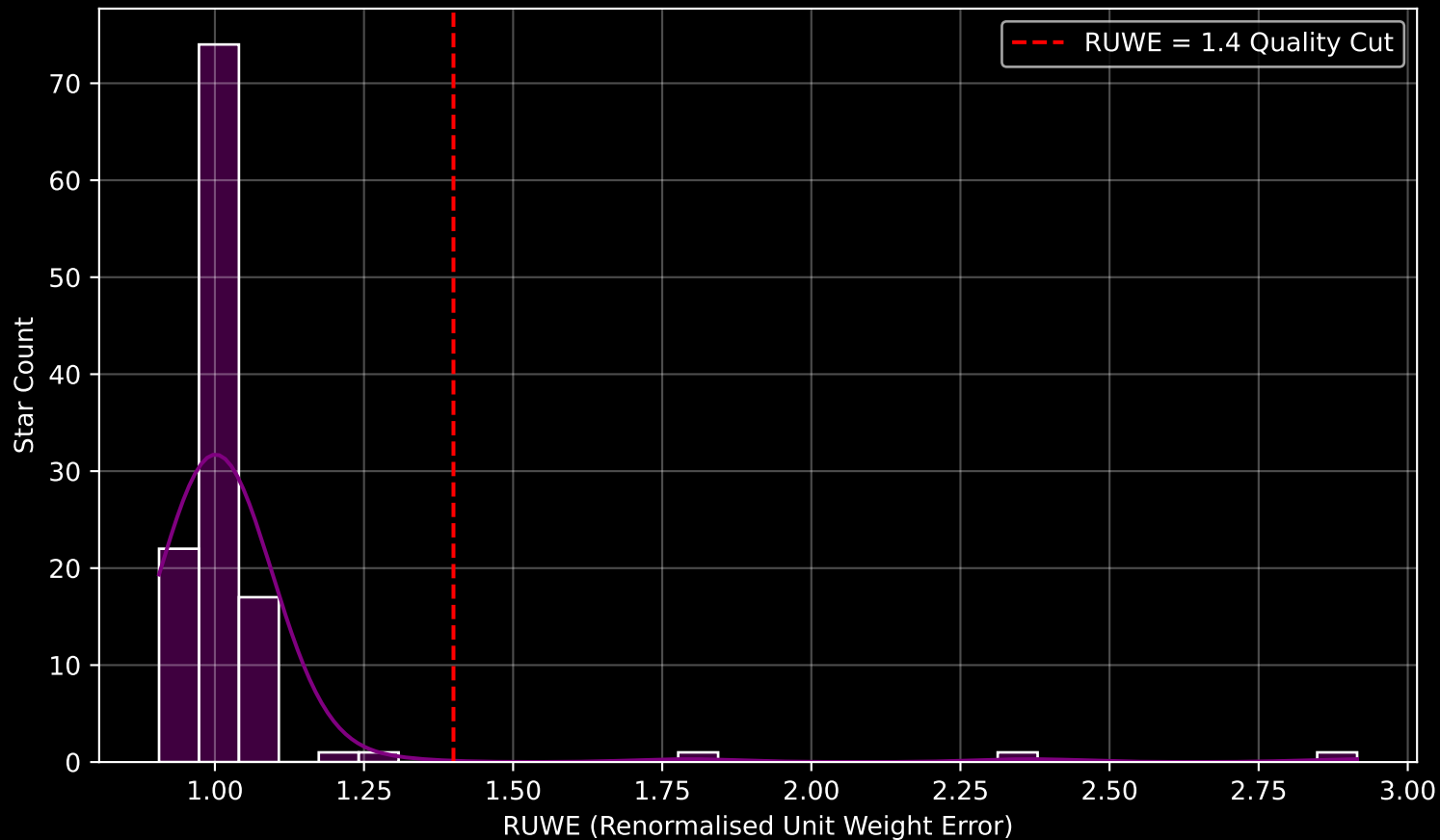
Gaia Cluster: [Haffner_7] RUWE Distribution (n= 118)
