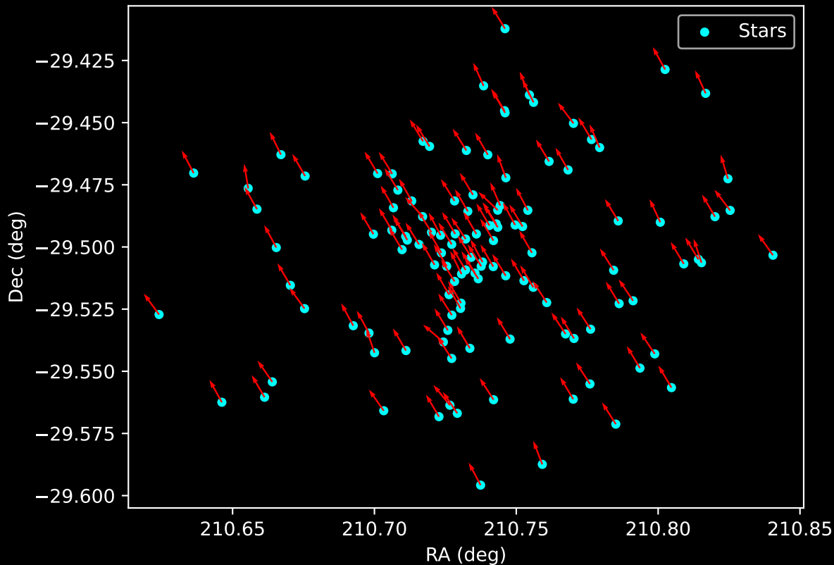
Gaia Cluster: [Haffner_7] Proper Motion Vectors for Gaia Star Field (n= 118)
