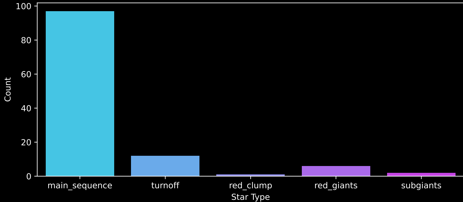
Gaia Cluster: [Haffner_7] Count plot of Star Type
