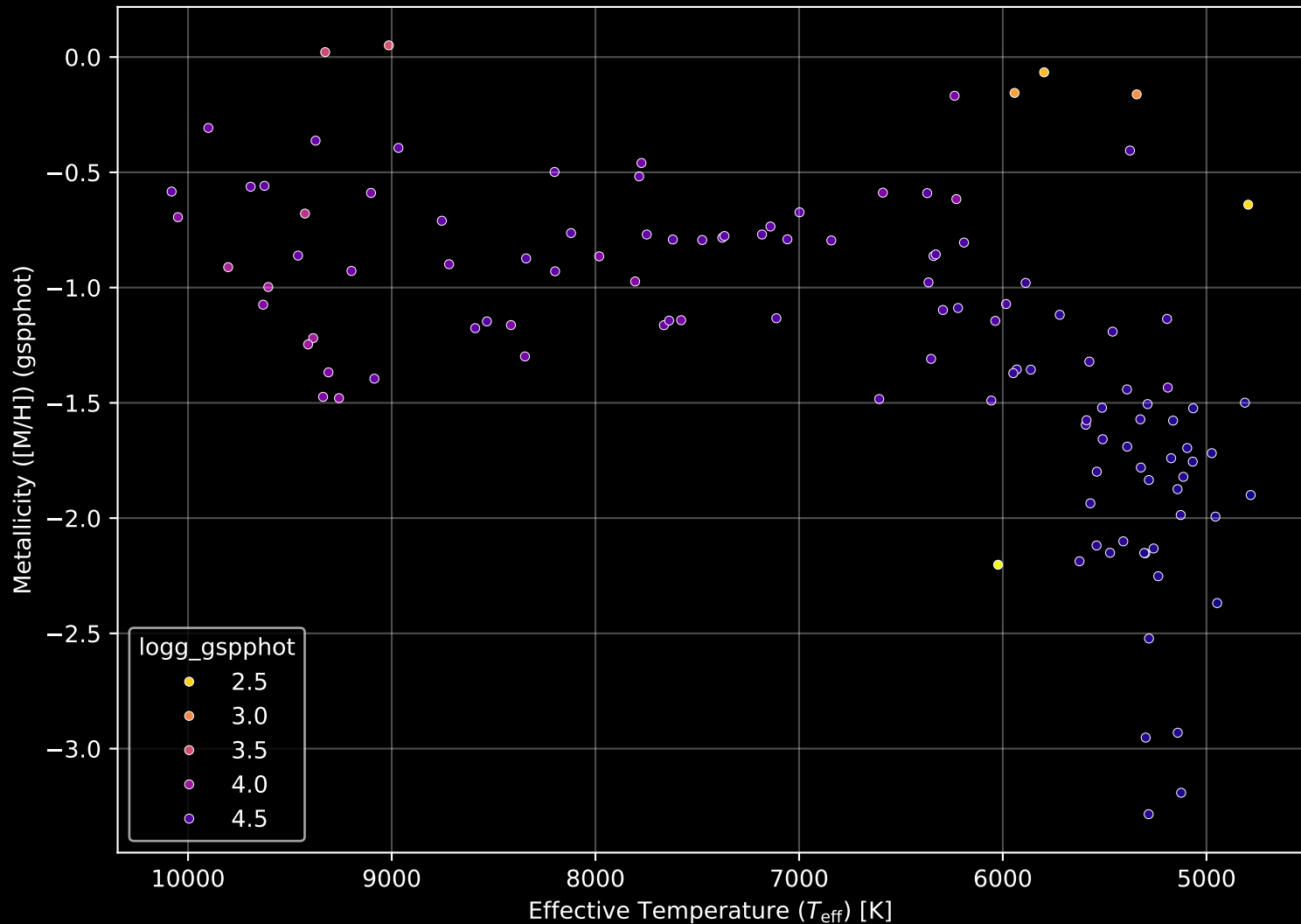
Gaia Cluster: [Haffner_7] Stellar Population Parameters (n= 118)
