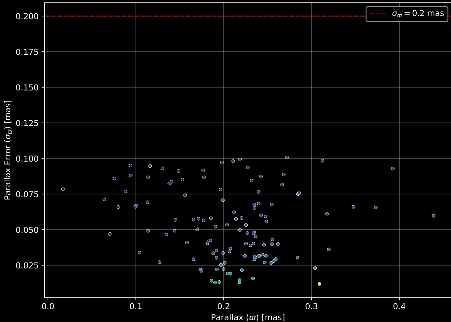
Gaia Cluster: [Haffner_7] Parallax Quality (n= 118)
