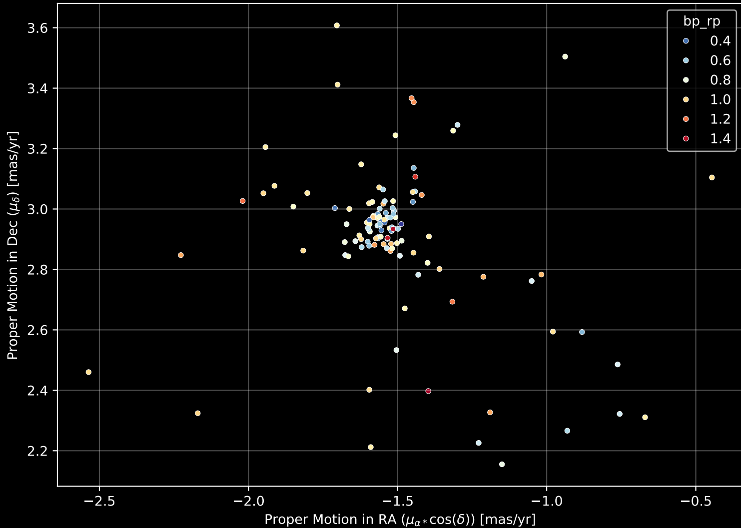
Gaia Cluster: [Haffner_7] Proper Motion Diagram (n= 118)
