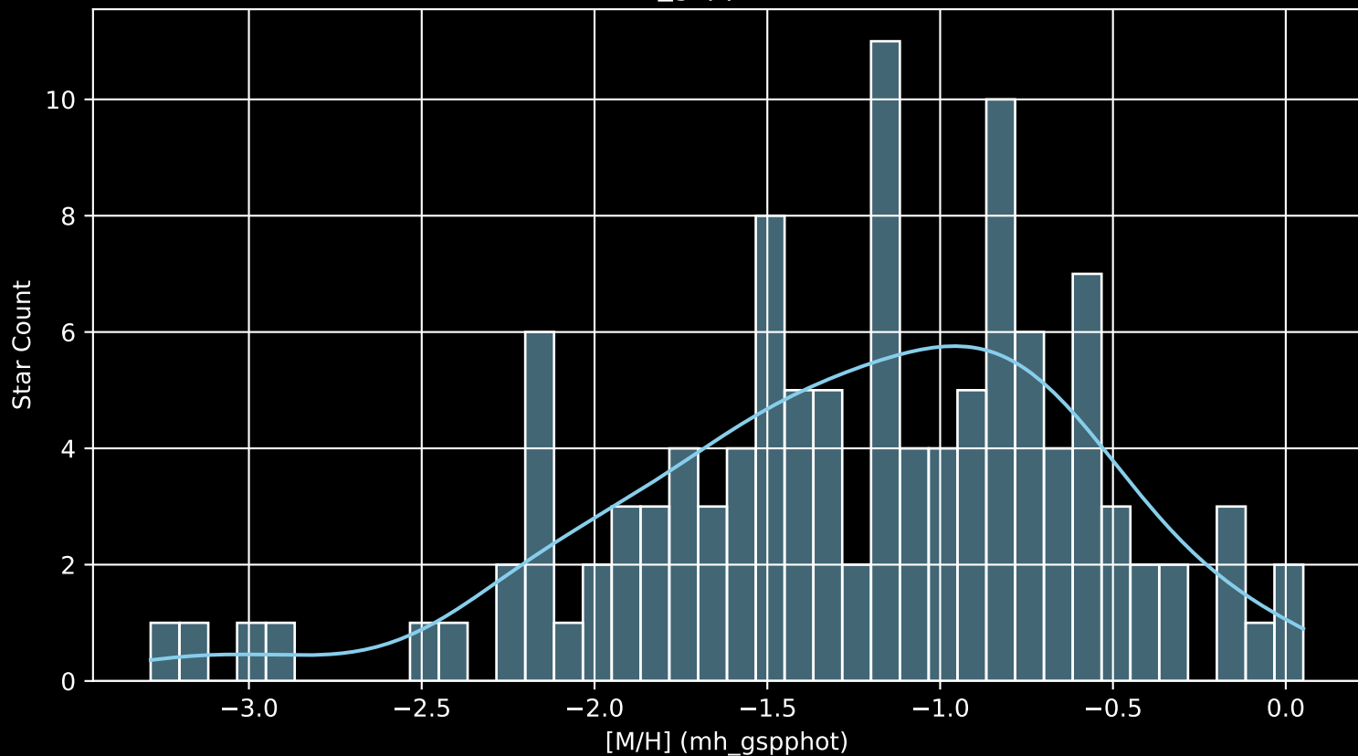
Gaia Cluster: [Haffner_7 [M/H] (mh_gspphot) (n= 118)
