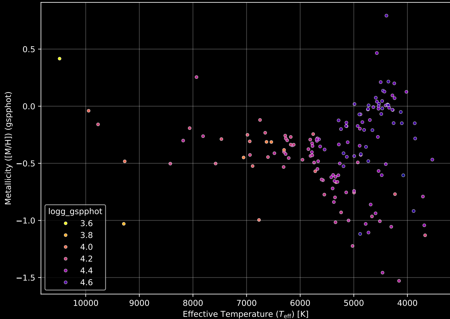
Gaia Cluster: [Harvard_10] Stellar Population Parameters (n= 157)
