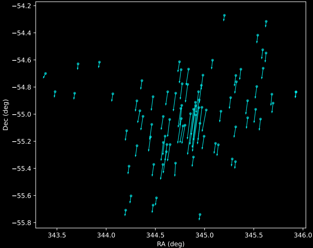
Gaia DR3 Noise Stream Proper Motion Vectors (n=84)
