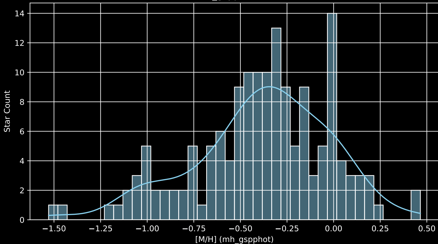
Gaia Cluster: [Harvard_10 [M/H] (mh_gspphot) (n= 156)
