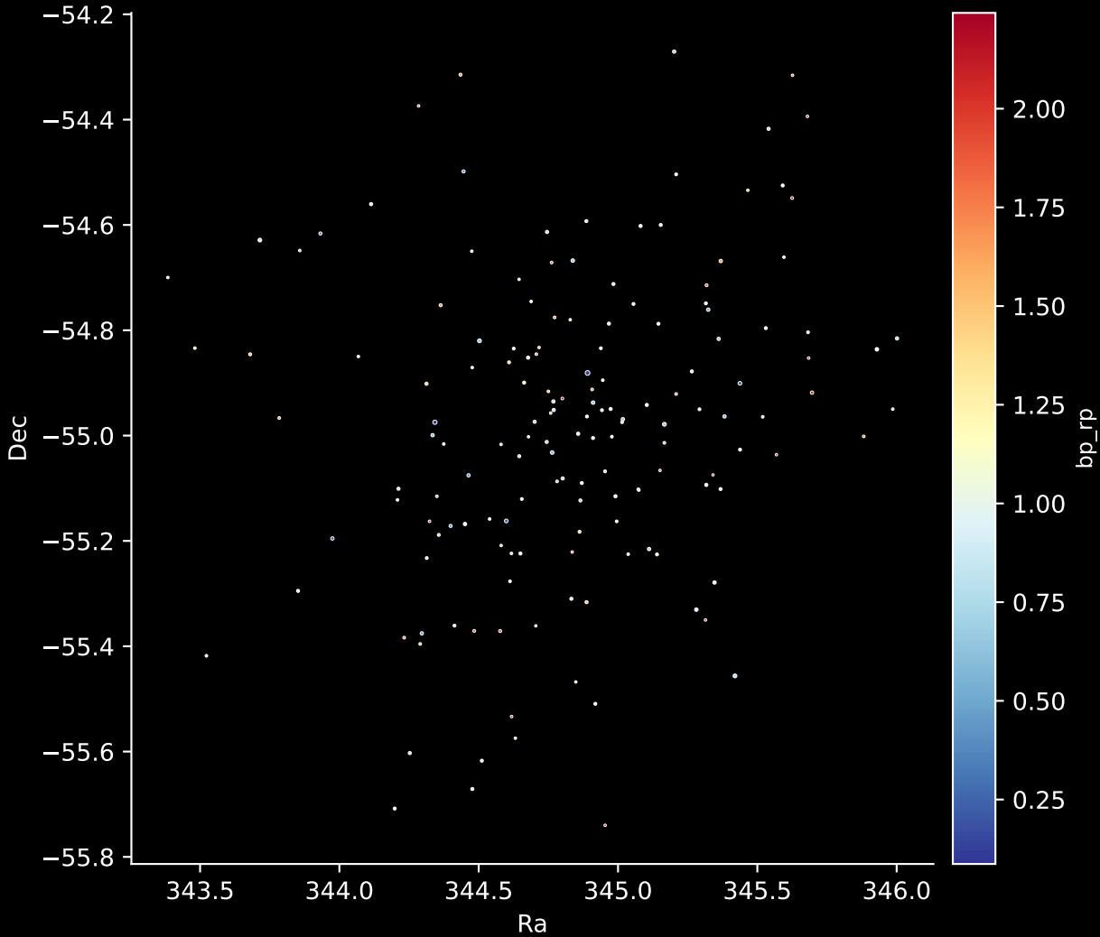
Gaia Cluster: [Harvard_10] Stars: 157
