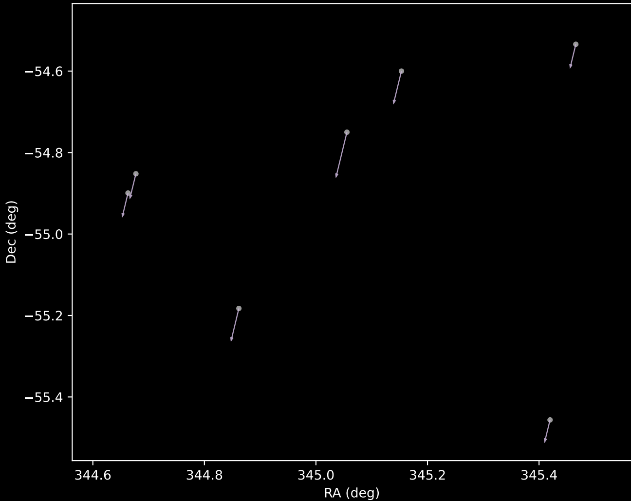
Gaia DR3 Cluster 9 Proper Motion Vectors (n=7)
