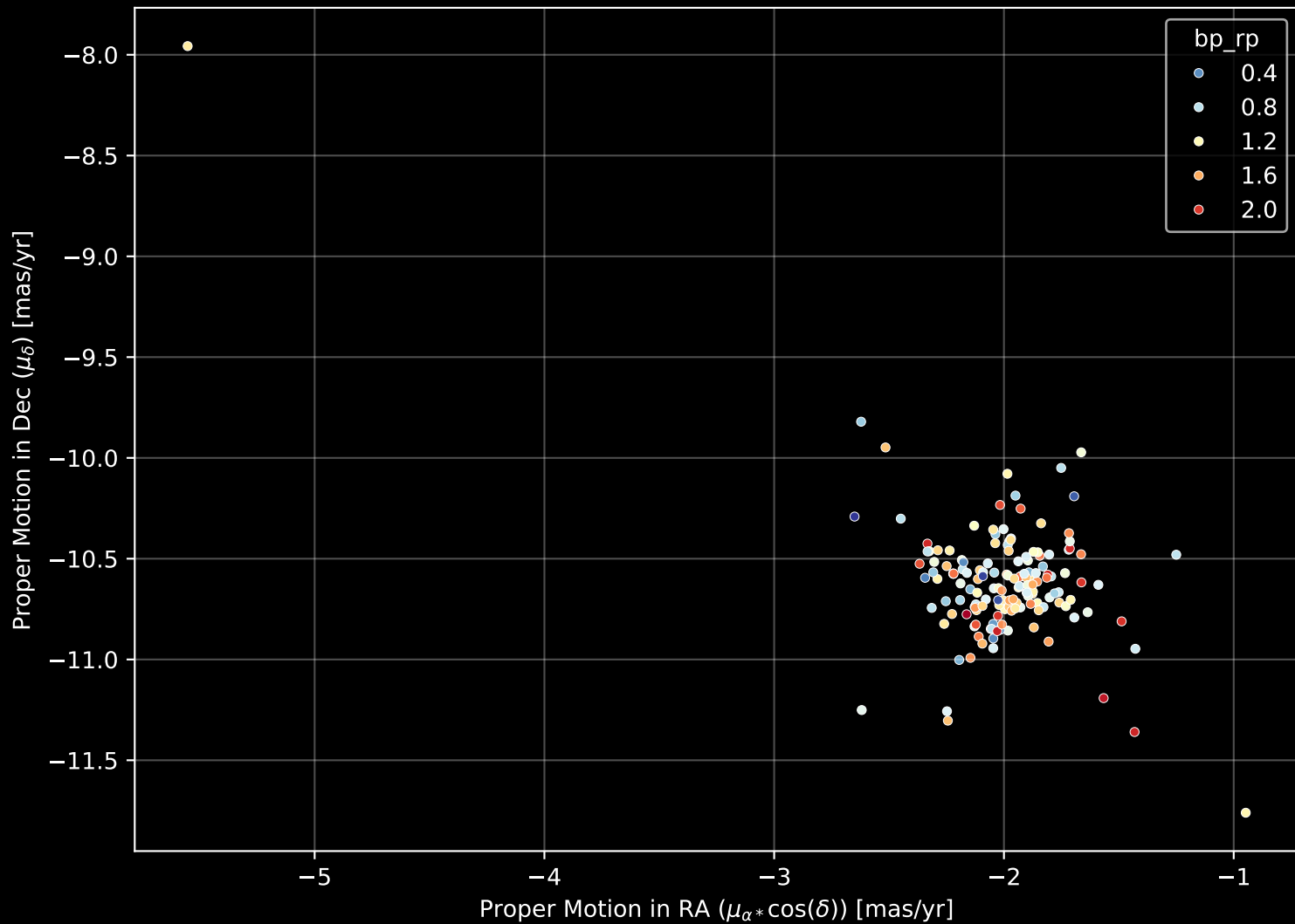
Gaia Cluster: [Harvard_10] Proper Motion Diagram (n= 157)
