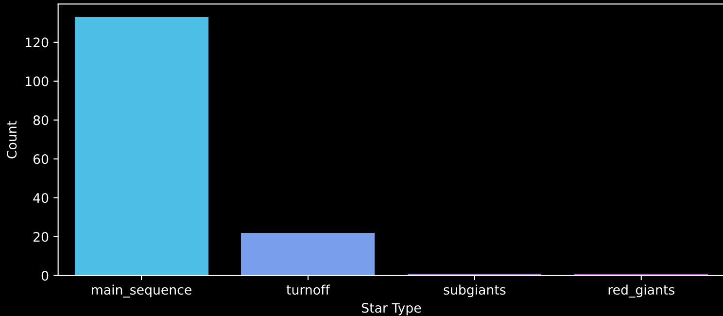
Gaia Cluster: [Harvard_10] Count plot of Star Type
