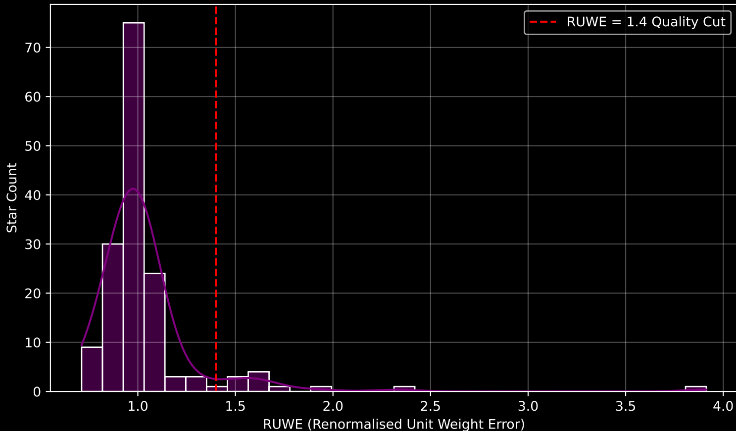
Gaia Cluster: [Harvard_10] RUWE Distribution (n= 156)
