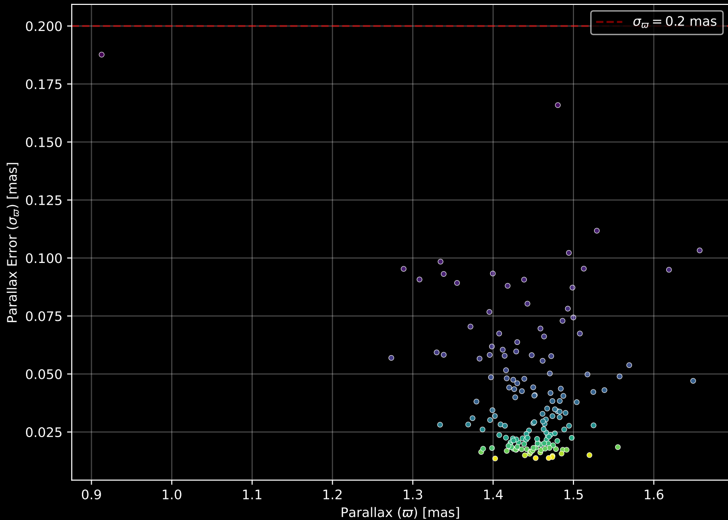
Gaia Cluster: [Harvard_10] Parallax Quality (n= 157)
