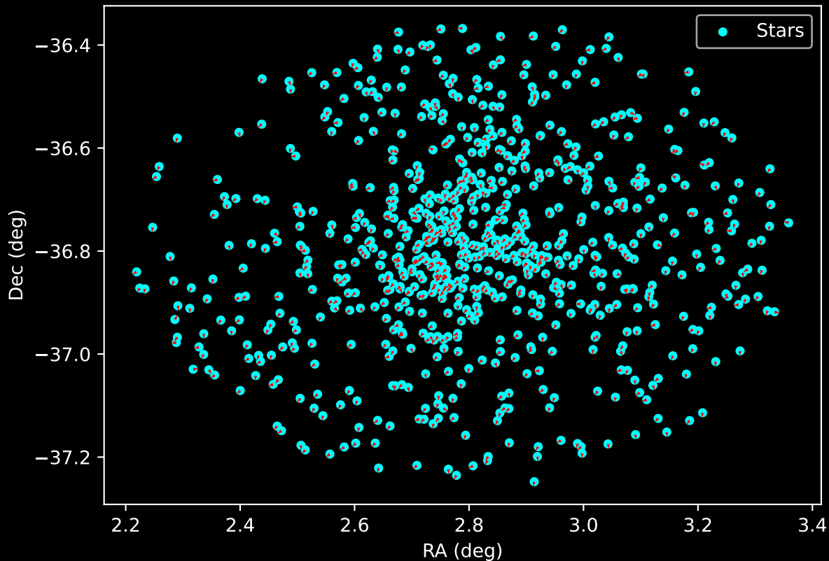
Gaia Cluster: [Harvard_16] Proper Motion Vectors for Gaia Star Field (n= 770)
