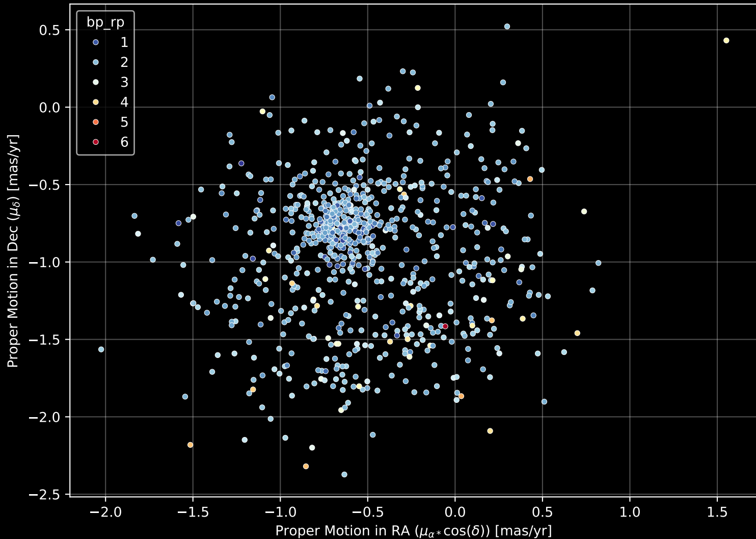
Gaia Cluster: [Harvard_16] Proper Motion Diagram (n= 770)
