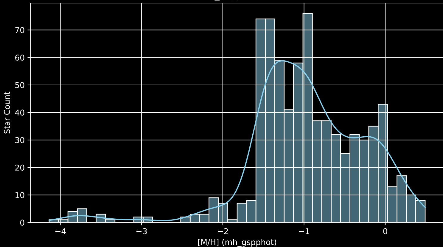
Gaia Cluster: [Harvard_16 [M/H] (mh_gspphot) (n= 760)
