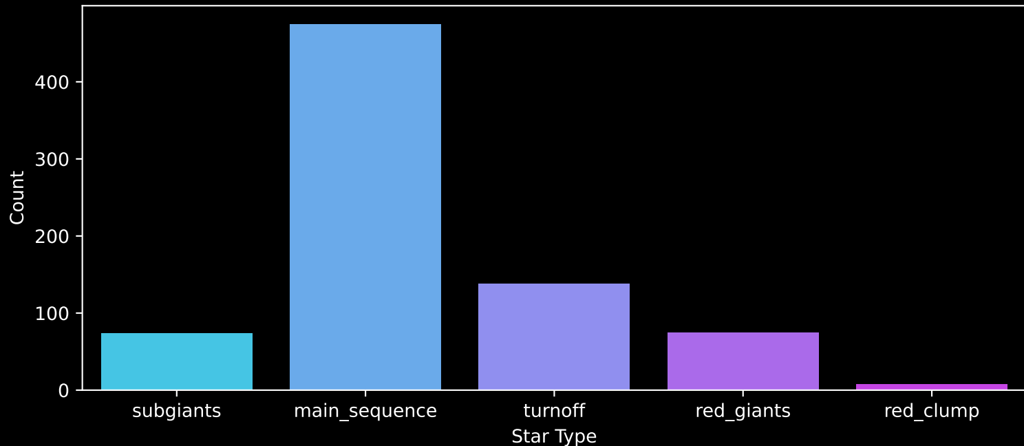
Gaia Cluster: [Harvard_16] Count plot of Star Type
