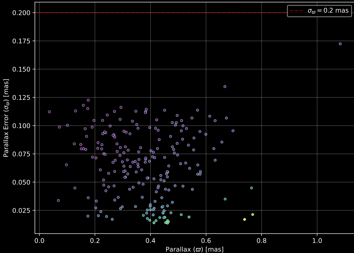
Gaia Cluster: [Harvard_20] Parallax Quality (n= 211)
