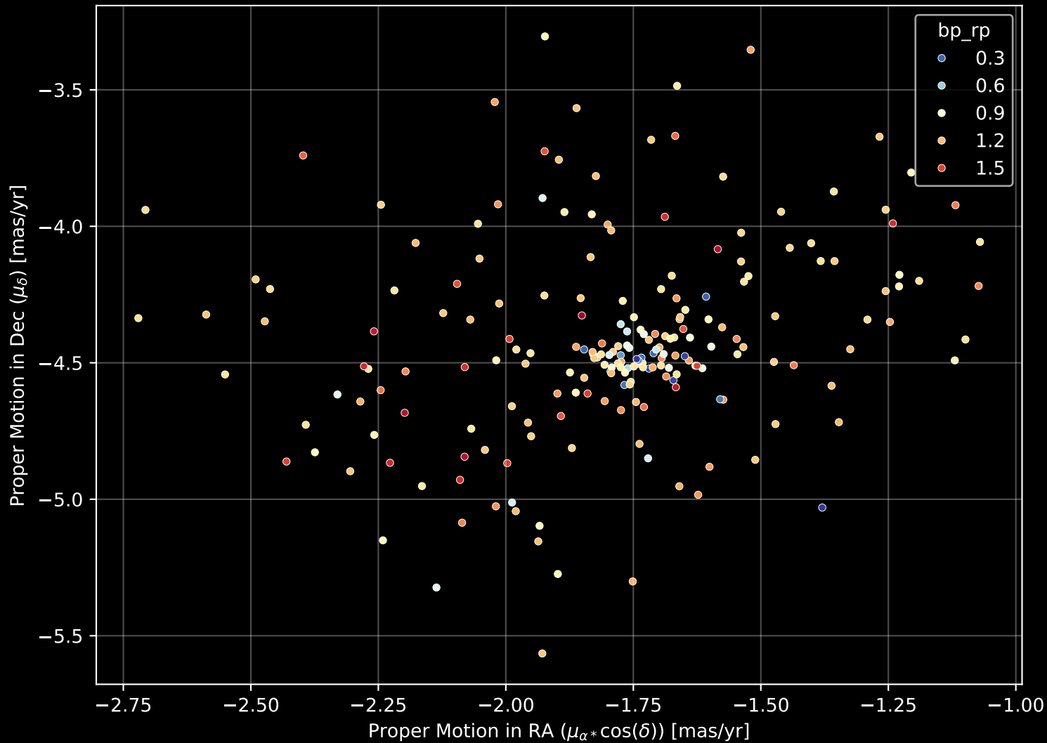
Gaia Cluster: [Harvard_20] Proper Motion Diagram (n= 211)
