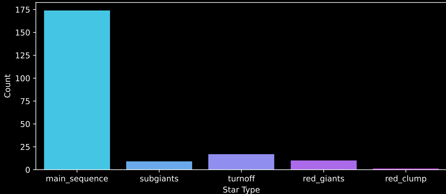
Gaia Cluster: [Harvard_20] Count plot of Star Type
