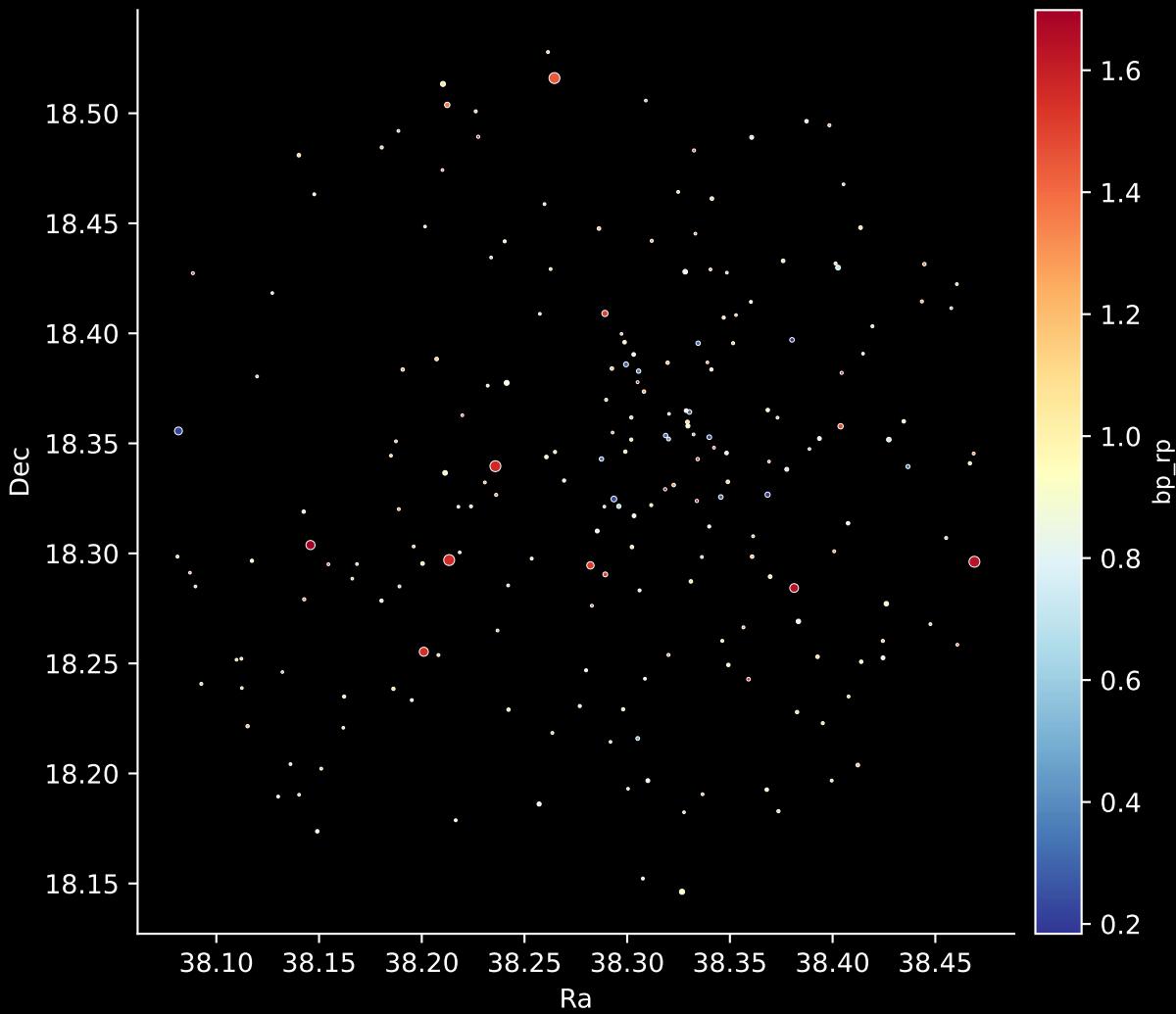
Gaia Cluster: [Harvard_20] Stars: 211
