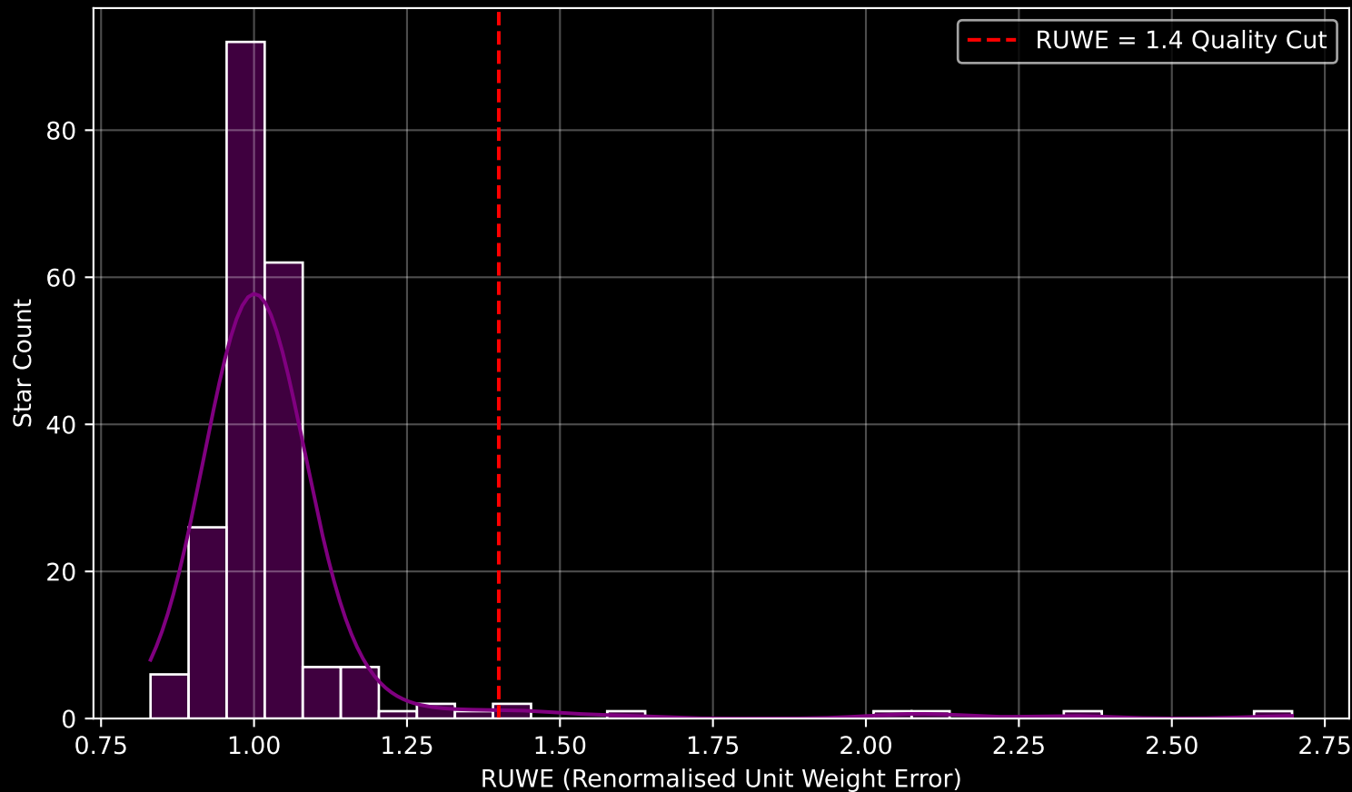
Gaia Cluster: [Harvard_20] RUWE Distribution (n= 211)
