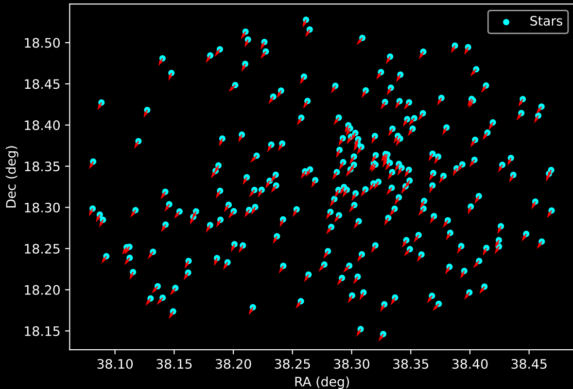
Gaia Cluster: [Harvard_20] Proper Motion Vectors for Gaia Star Field (n= 211)
