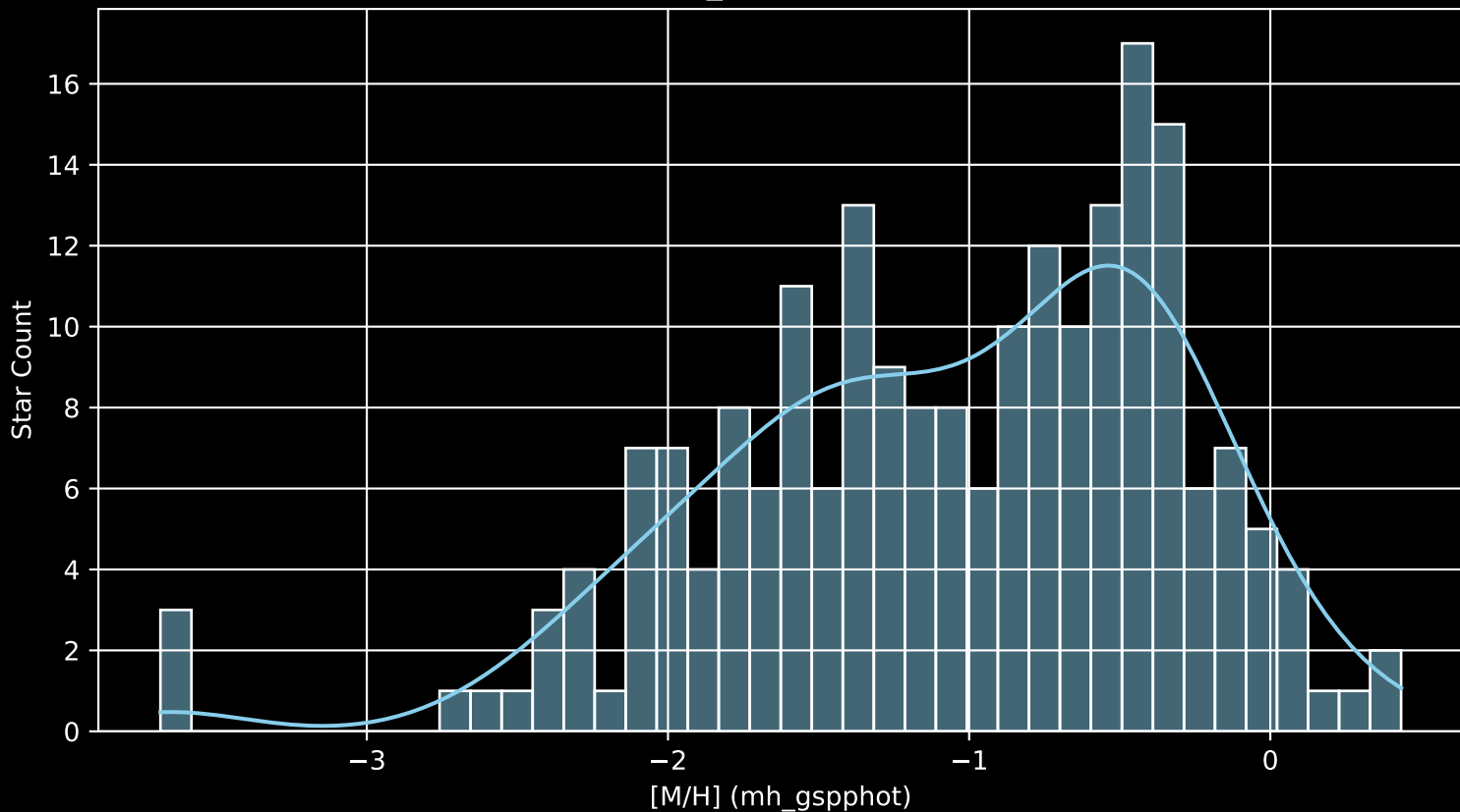
Gaia Cluster: [Harvard_20 [M/H] (mh_gspphot) (n= 210)
