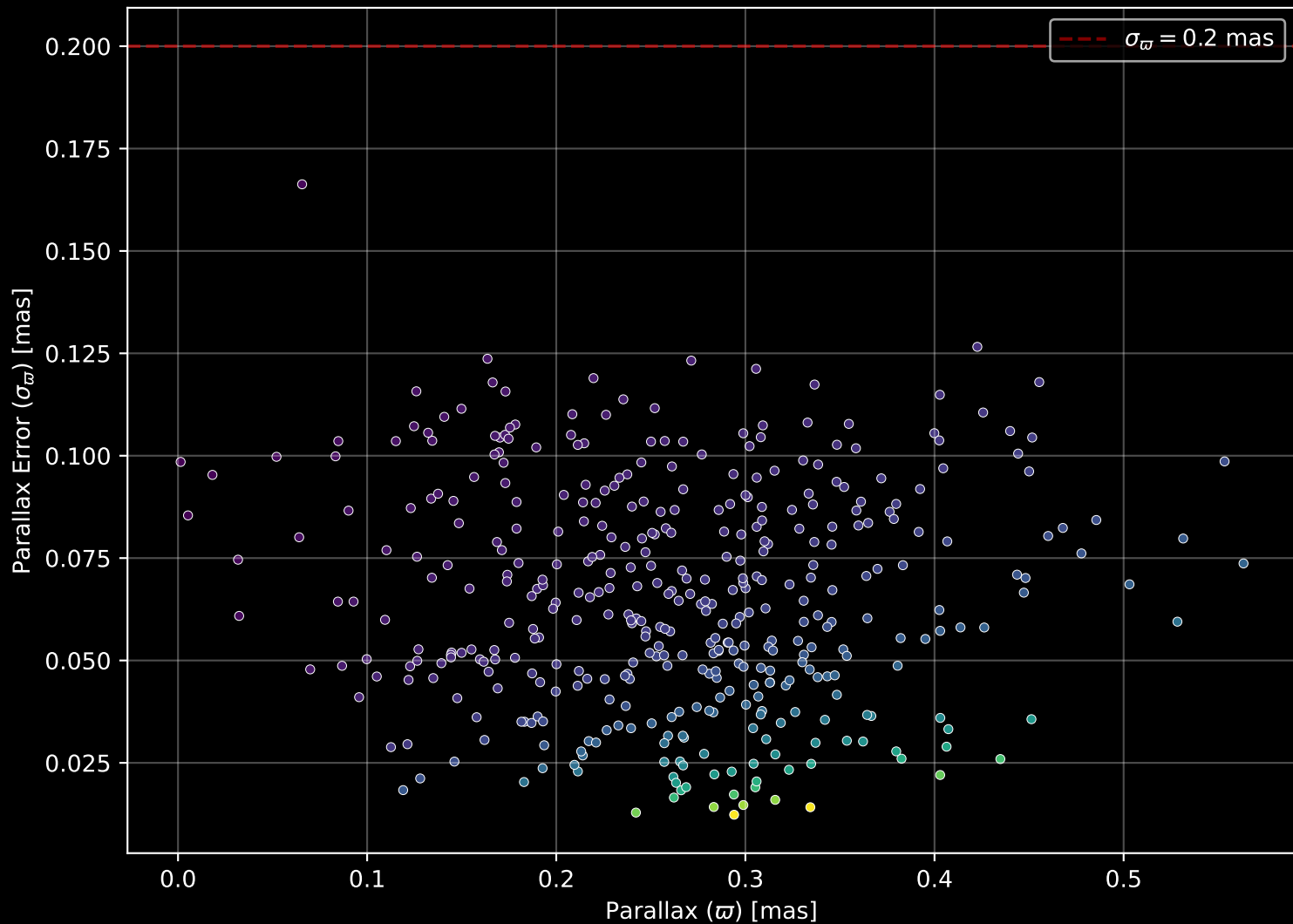
Gaia Cluster: [Hogg_15] Parallax Quality (n= 403)
