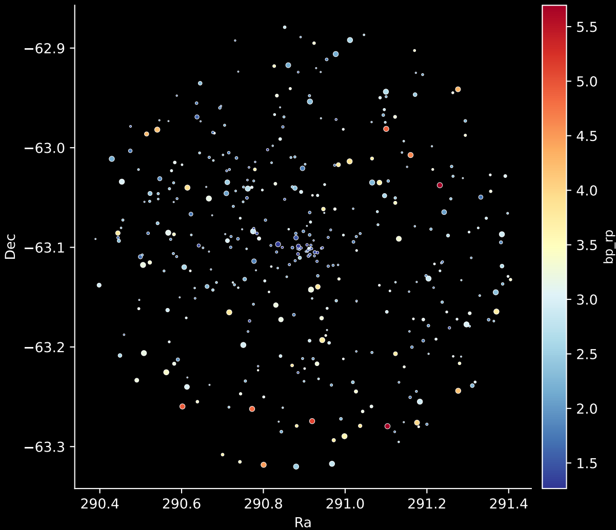
Gaia Cluster: [Hogg_15] Stars: 403
