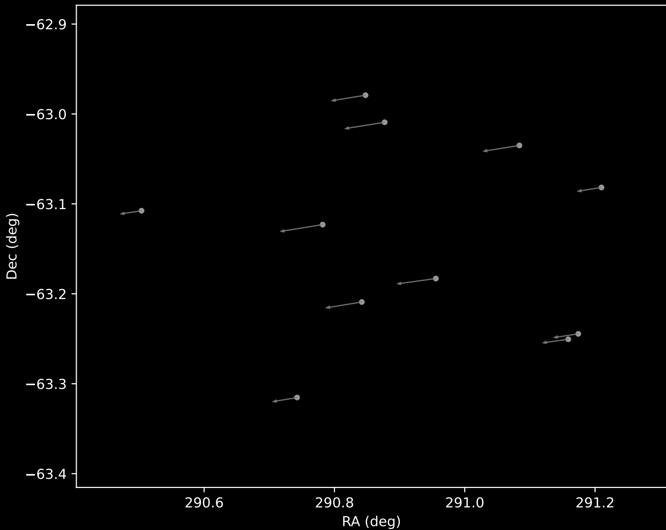
Gaia DR3 Cluster 14 Proper Motion Vectors (n=11)
