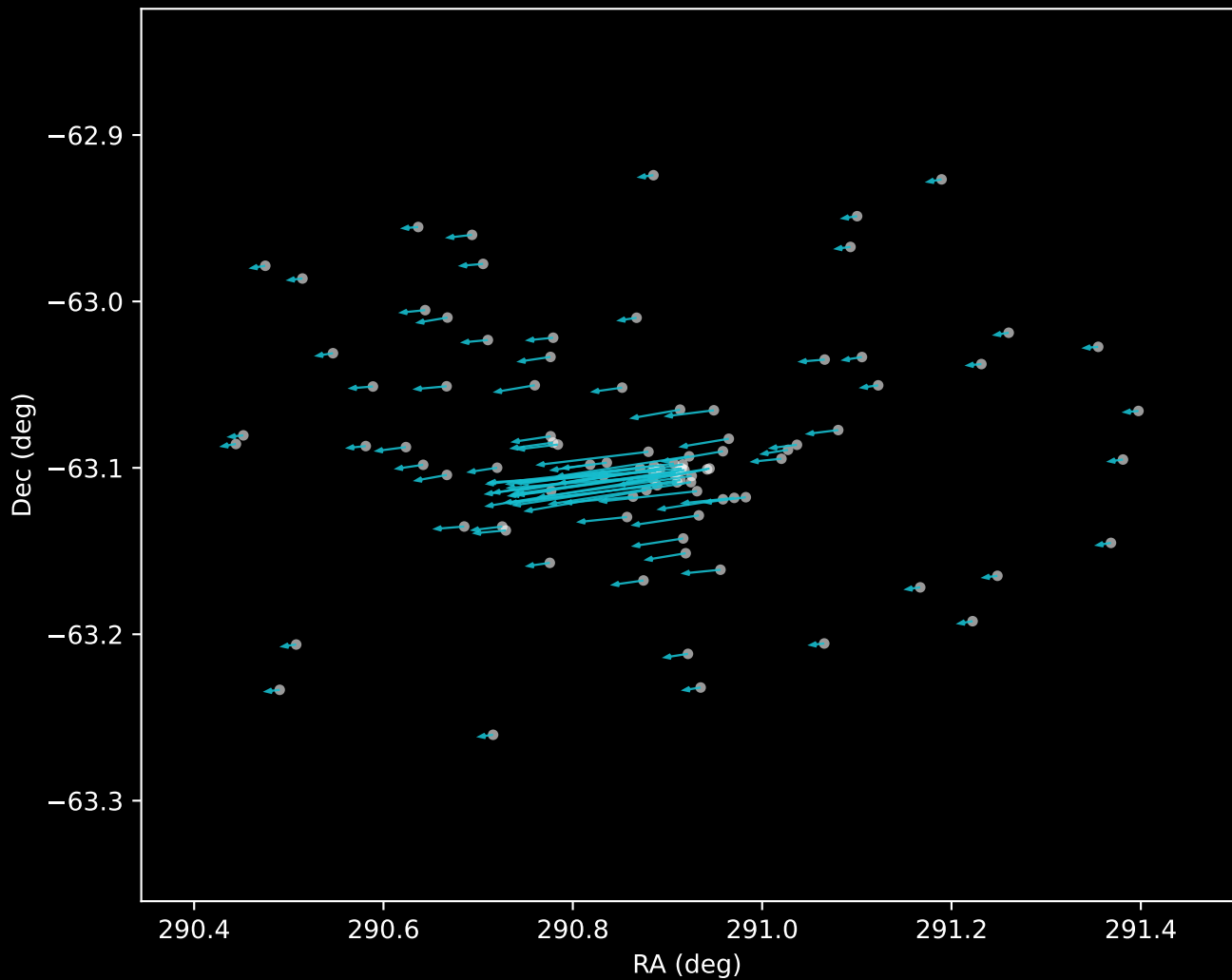
Gaia DR3 Cluster 18 Proper Motion Vectors (n=98)
