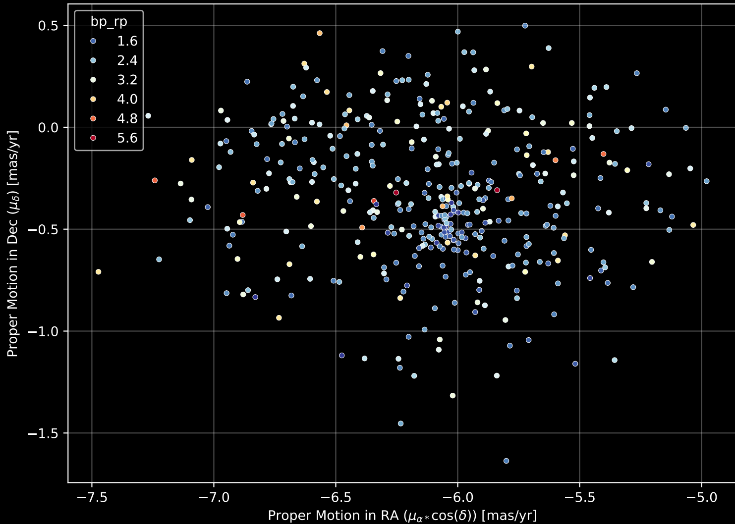
Gaia Cluster: [Hogg_15] Proper Motion Diagram (n= 403)
