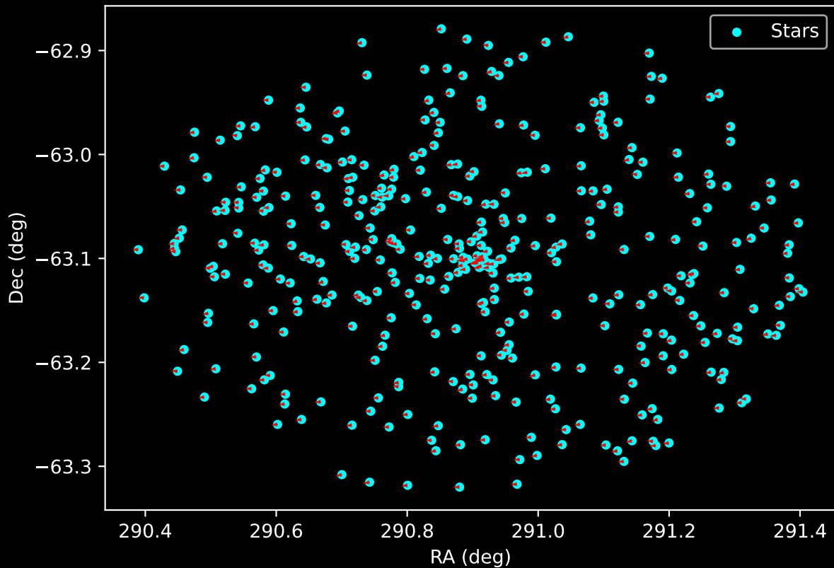
Gaia Cluster: [Hogg_15] Proper Motion Vectors for Gaia Star Field (n= 403)
