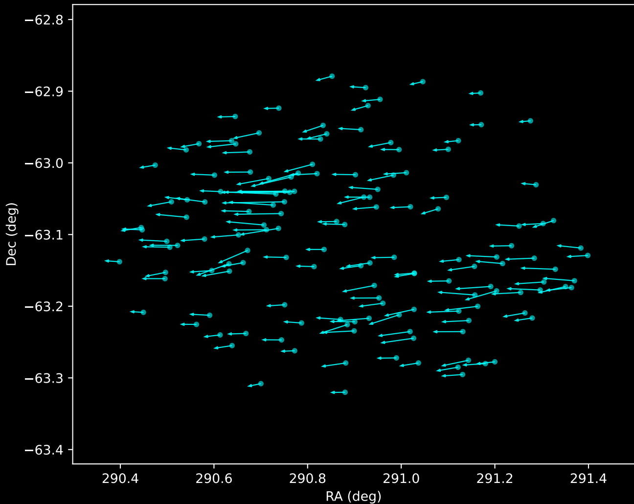
Gaia DR3 Noise Stream Proper Motion Vectors (n=144)
