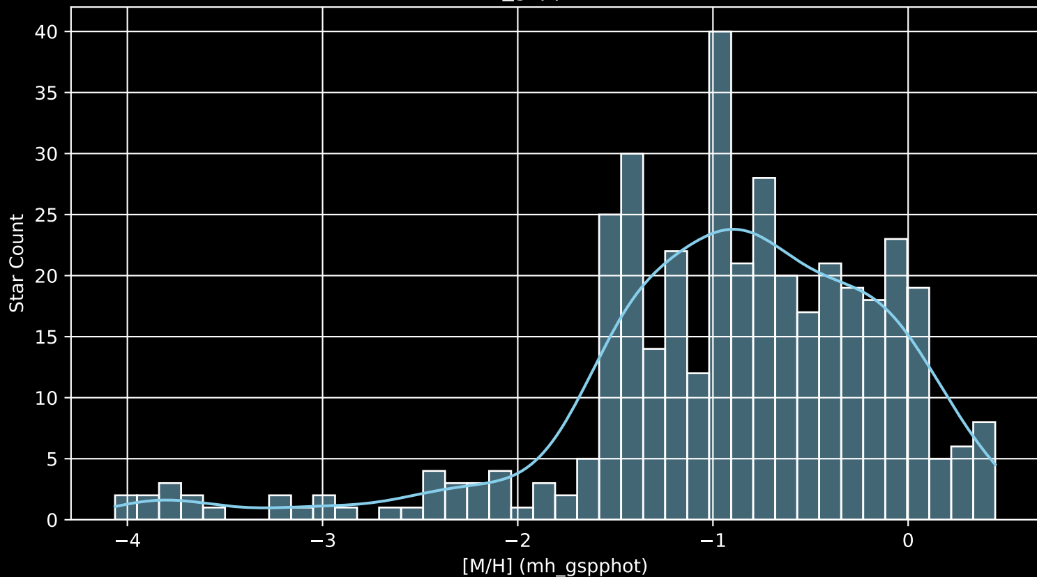
Gaia Cluster: [Hogg_15 [M/H] (mh_gspphot) (n= 391)
