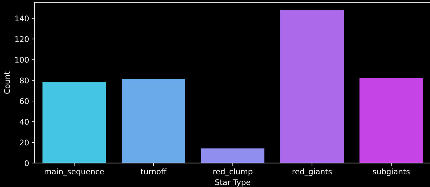
Gaia Cluster: [Hogg_15] Count plot of Star Type
