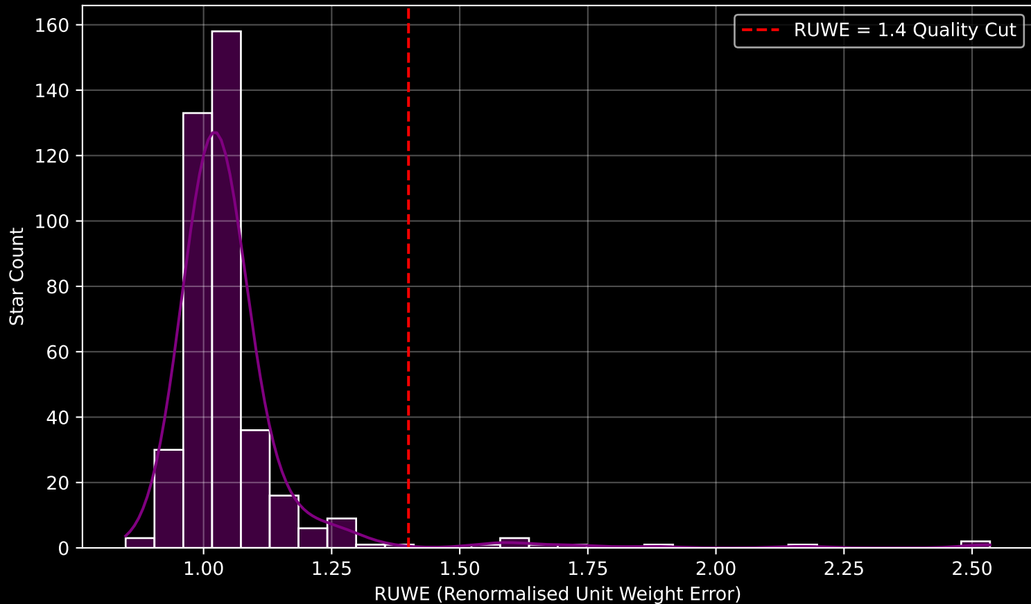
Gaia Cluster: [Hogg_15] RUWE Distribution (n= 403)
