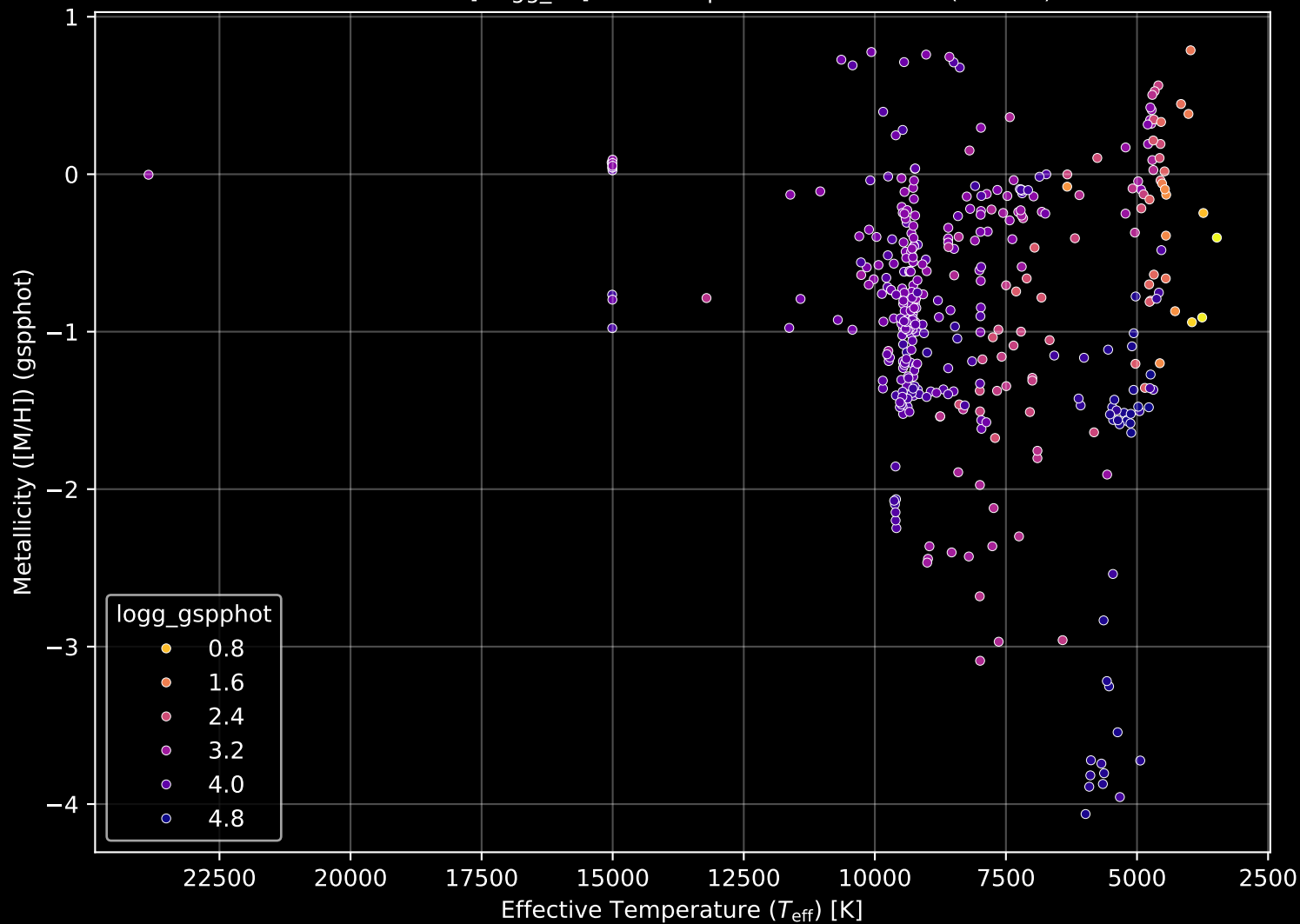
Gaia Cluster: [Hogg_15] Stellar Population Parameters (n= 403)
