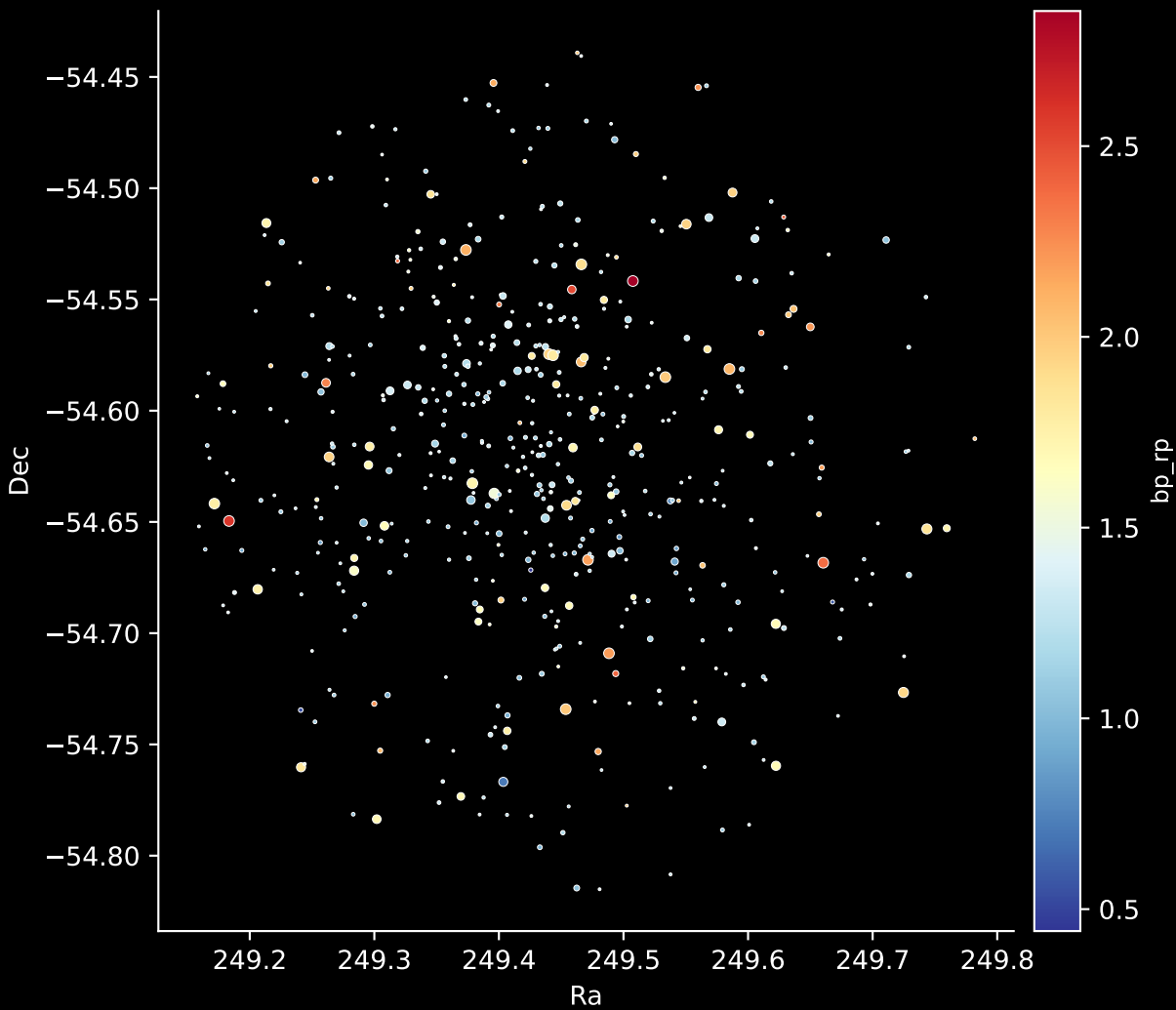
Gaia Cluster: [Hogg_4] Stars: 518
