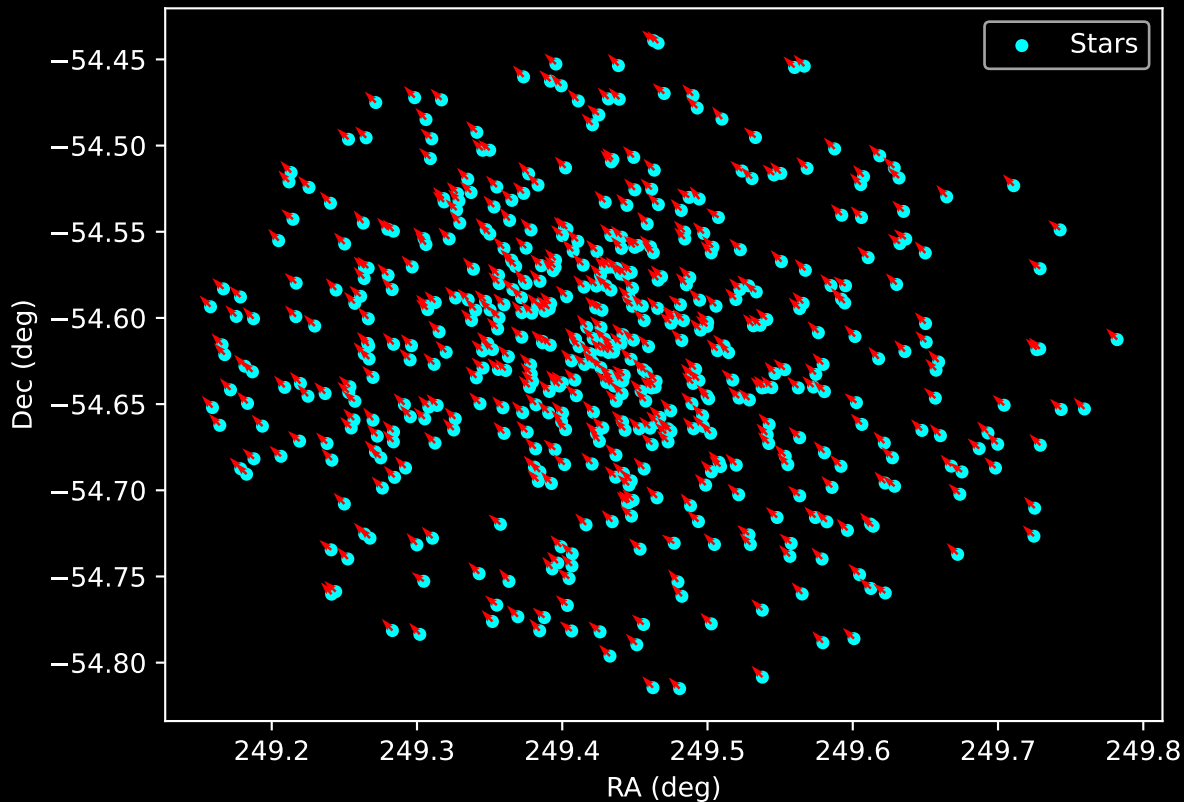
Gaia Cluster: [Hogg_4] Proper Motion Vectors for Gaia Star Field (n= 518)
