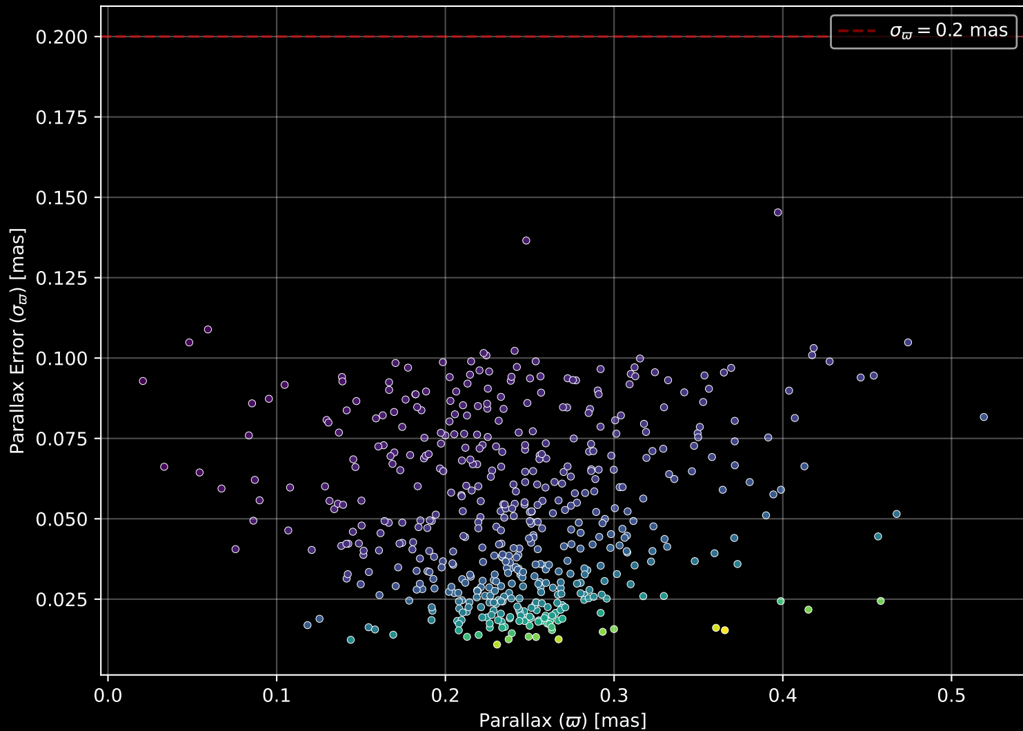
Gaia Cluster: [Hogg_4] Parallax Quality (n= 518)
