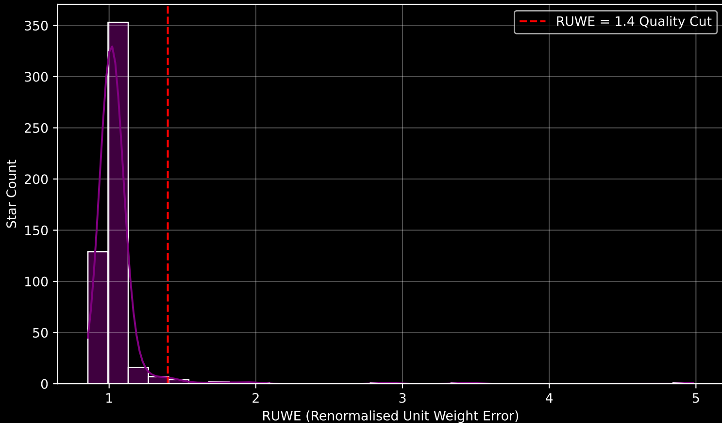
Gaia Cluster: [Hogg_4] RUWE Distribution (n= 517)
