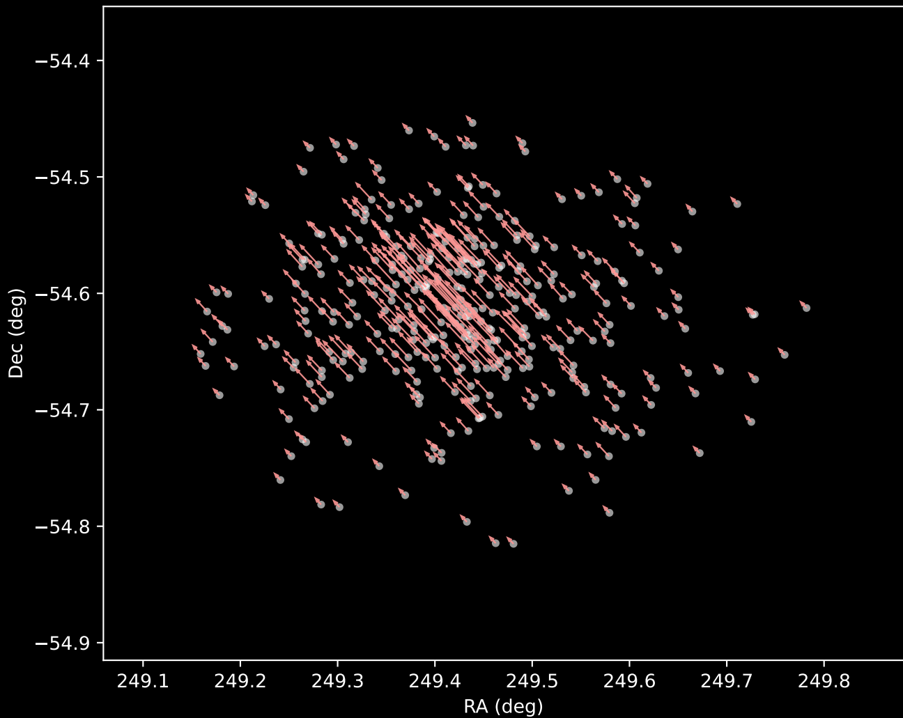
Gaia DR3 Cluster 7 Proper Motion Vectors (n=351)
