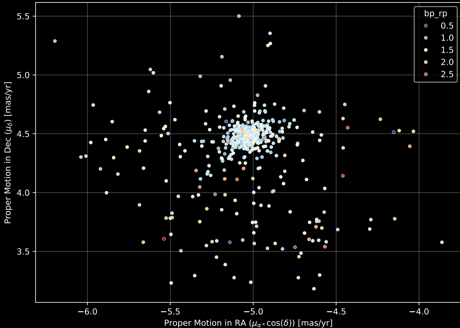
Gaia Cluster: [Hogg_4] Proper Motion Diagram (n= 518)
