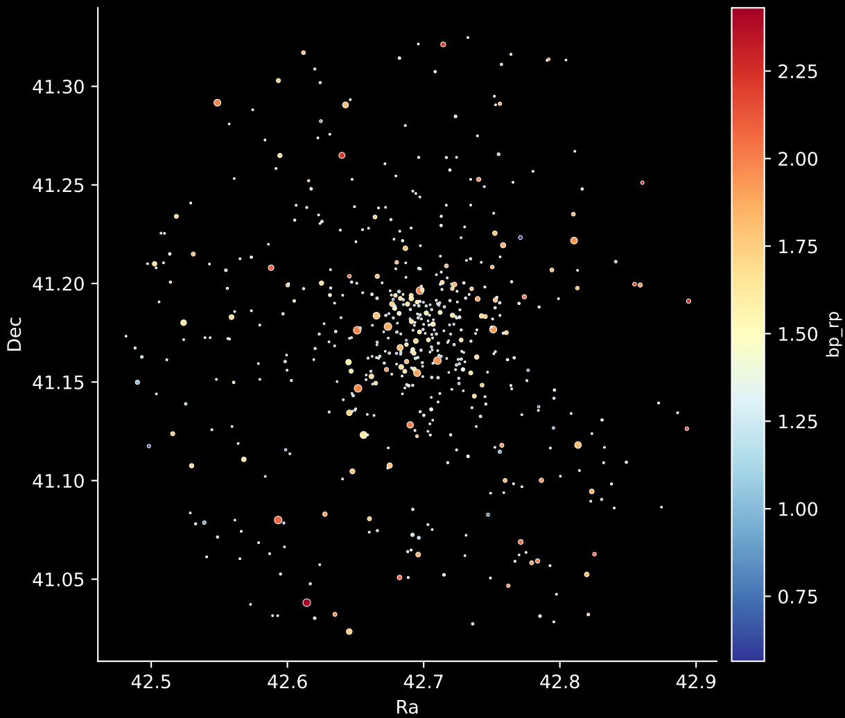
Gaia Cluster: [IC_1311] Stars: 534
