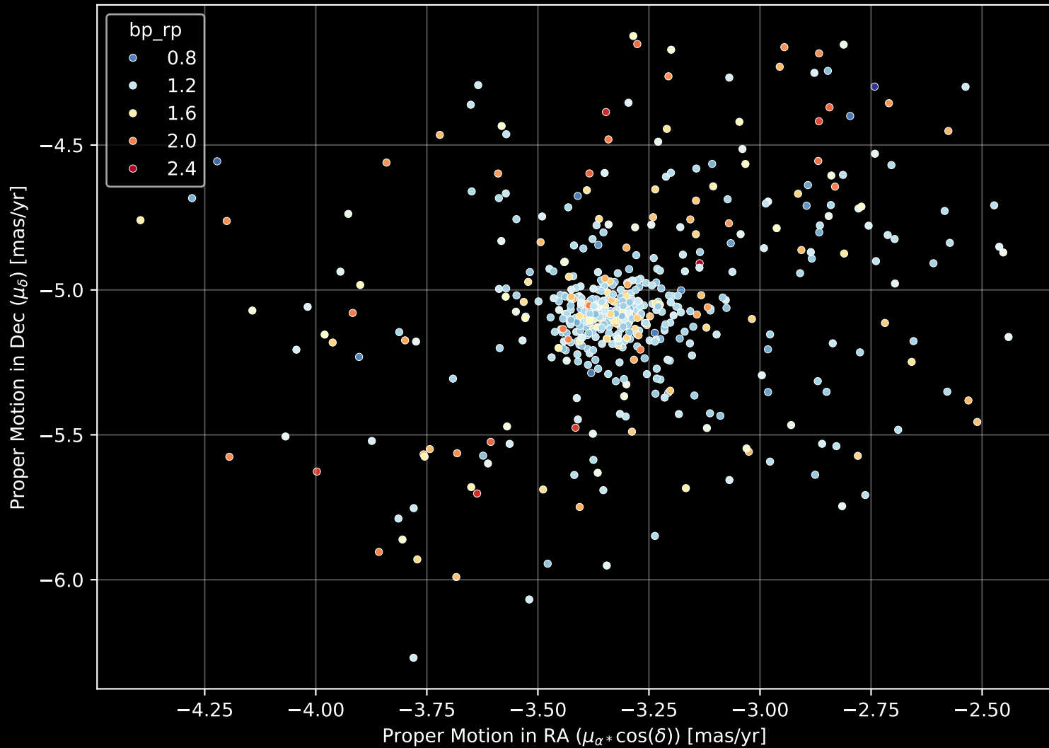
Gaia Cluster: [IC_1311] Proper Motion Diagram (n= 534)
