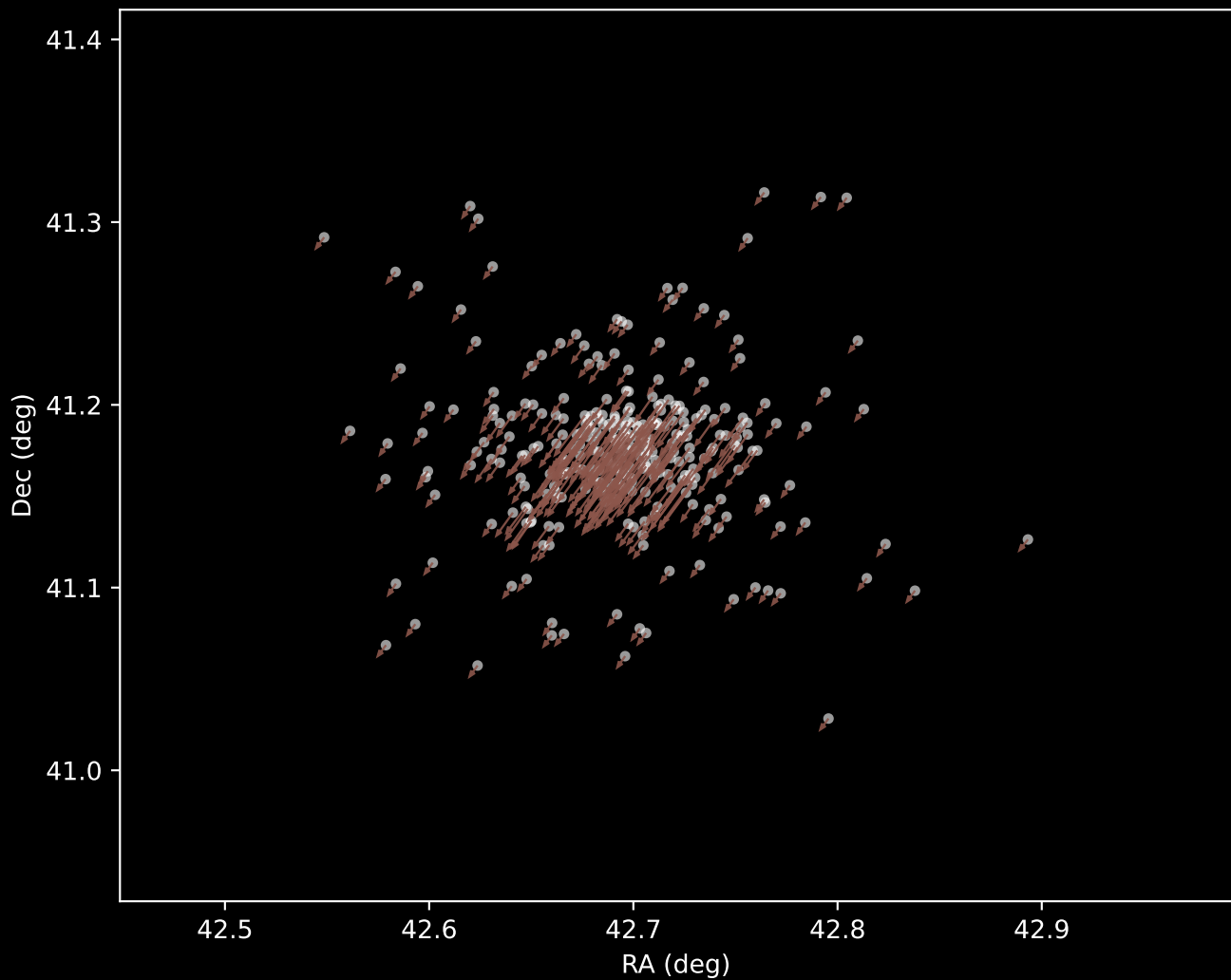
Gaia DR3 Cluster 10 Proper Motion Vectors (n=296)
