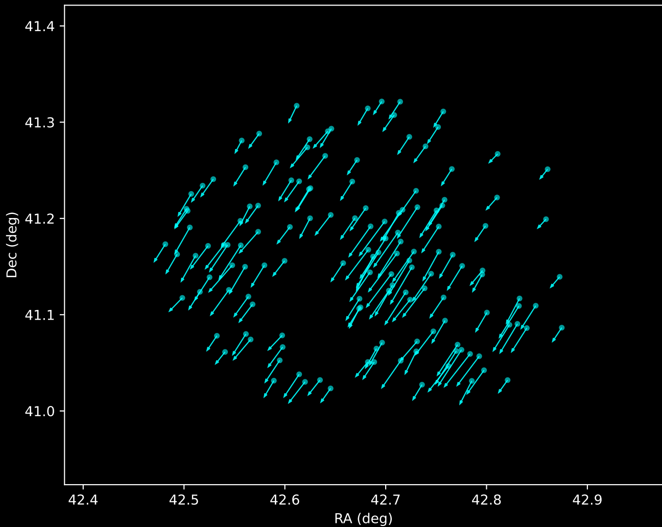
Gaia DR3 Noise Stream Proper Motion Vectors (n=140)
