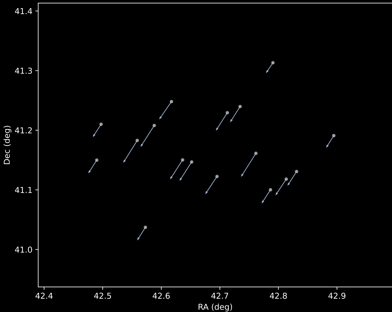
Gaia DR3 Cluster 1 Proper Motion Vectors (n=17)
