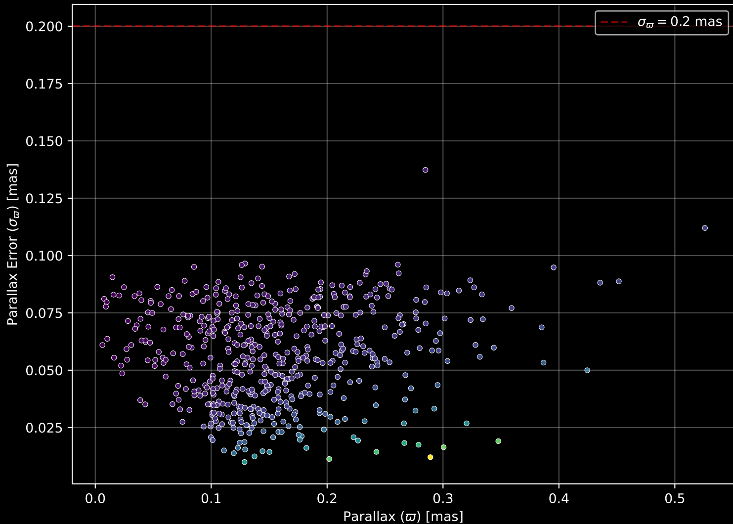
Gaia Cluster: [IC_1311] Parallax Quality (n= 534)
