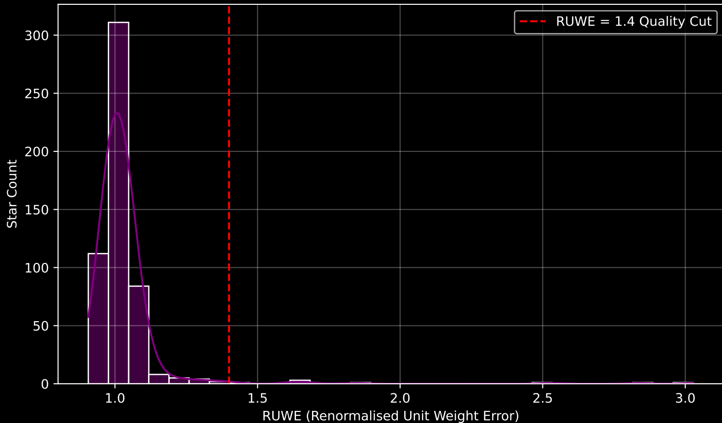
Gaia Cluster: [IC_1311] RUWE Distribution (n= 534)
