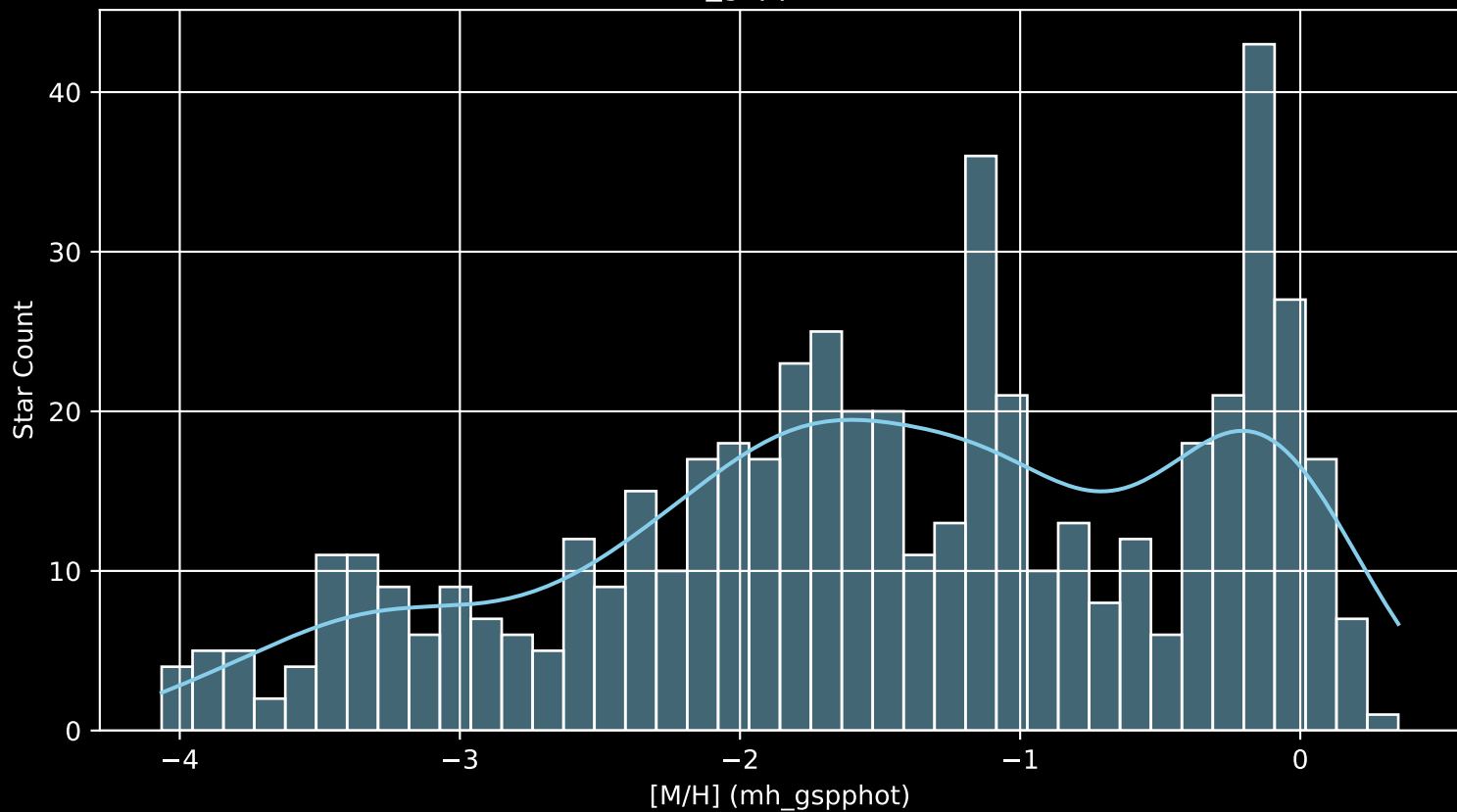
Gaia Cluster: [IC_1311 [M/H] (mh_gspphot) (n= 534)
