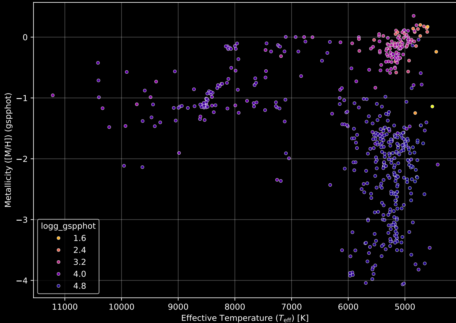
Gaia Cluster: [IC_1311] Stellar Population Parameters (n= 534)
