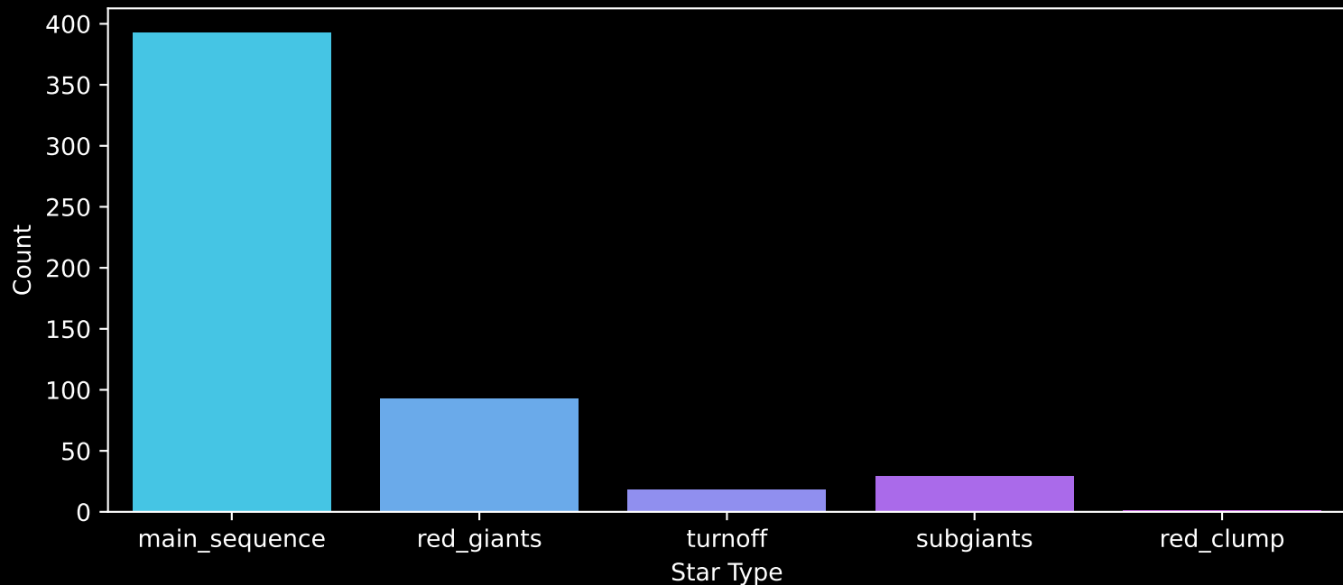
Gaia Cluster: [IC_1311] Count plot of Star Type
