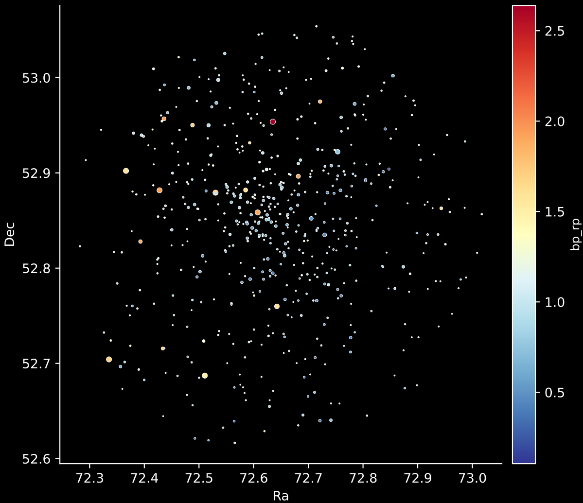
Gaia Cluster: [IC_1434] Stars: 565
