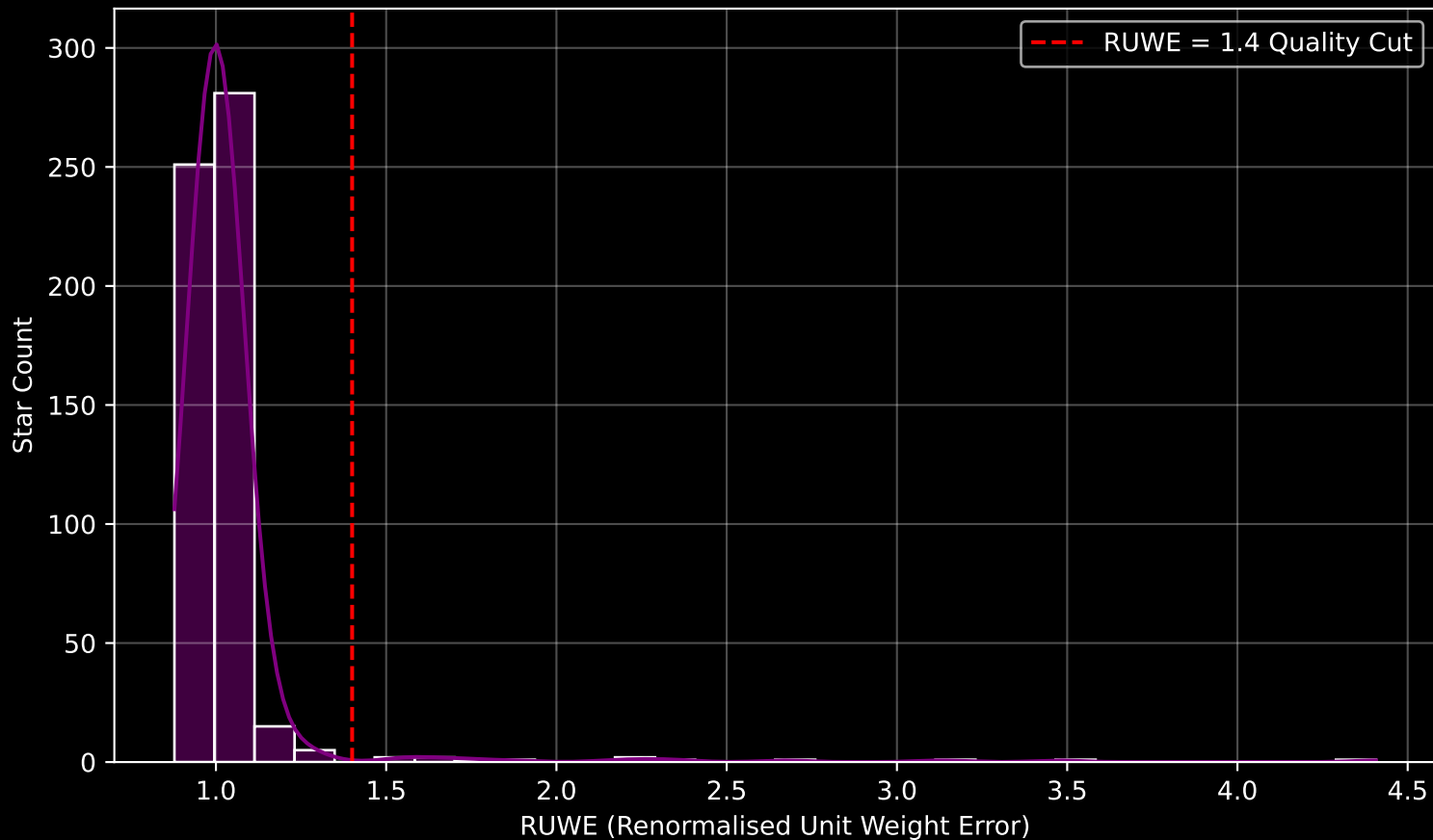
Gaia Cluster: [IC_1434] RUWE Distribution (n= 565)
