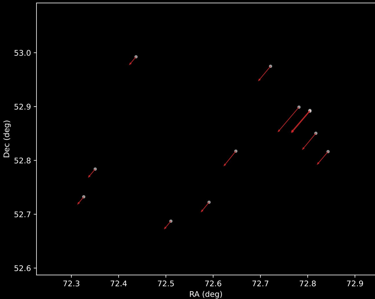
Gaia DR3 Cluster 6 Proper Motion Vectors (n=12)
