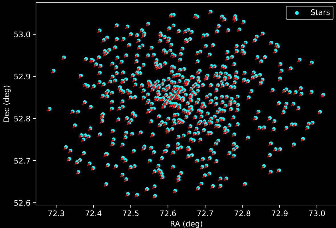
Gaia Cluster: [IC_1434] Proper Motion Vectors for Gaia Star Field (n= 565)
