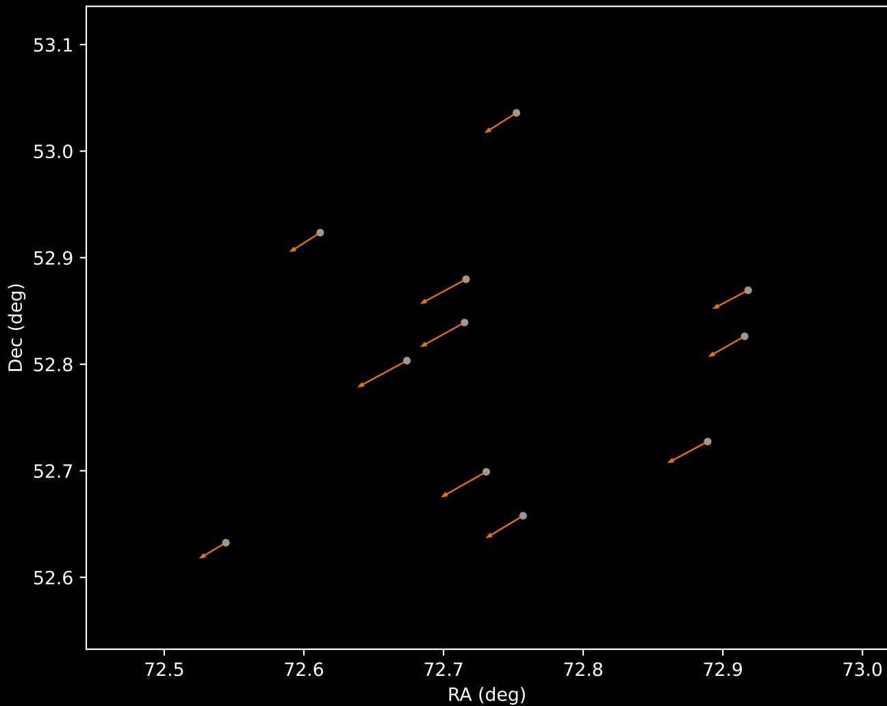
Gaia DR3 Cluster 2 Proper Motion Vectors (n=11)
