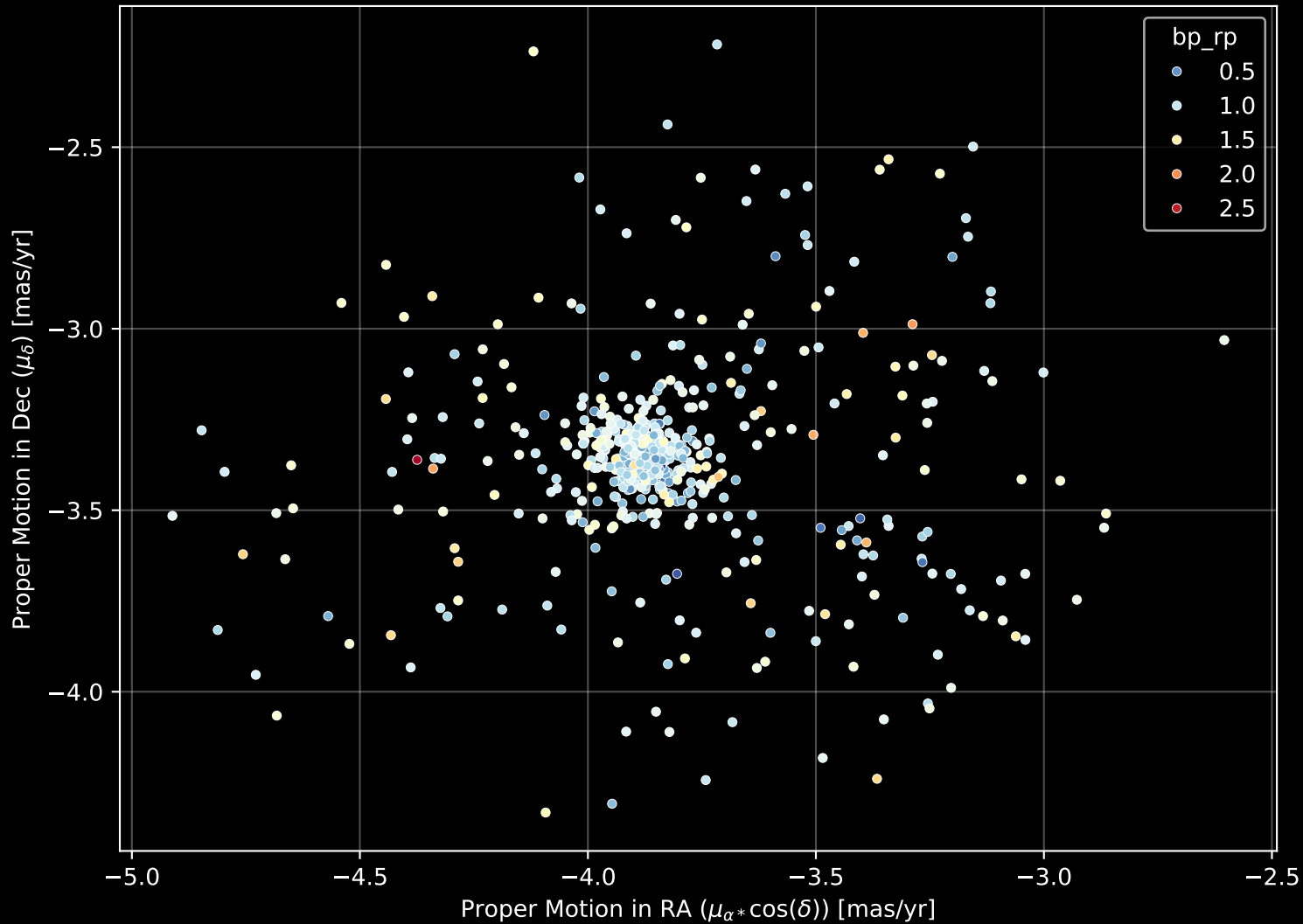
Gaia Cluster: [IC_1434] Proper Motion Diagram (n= 565)
