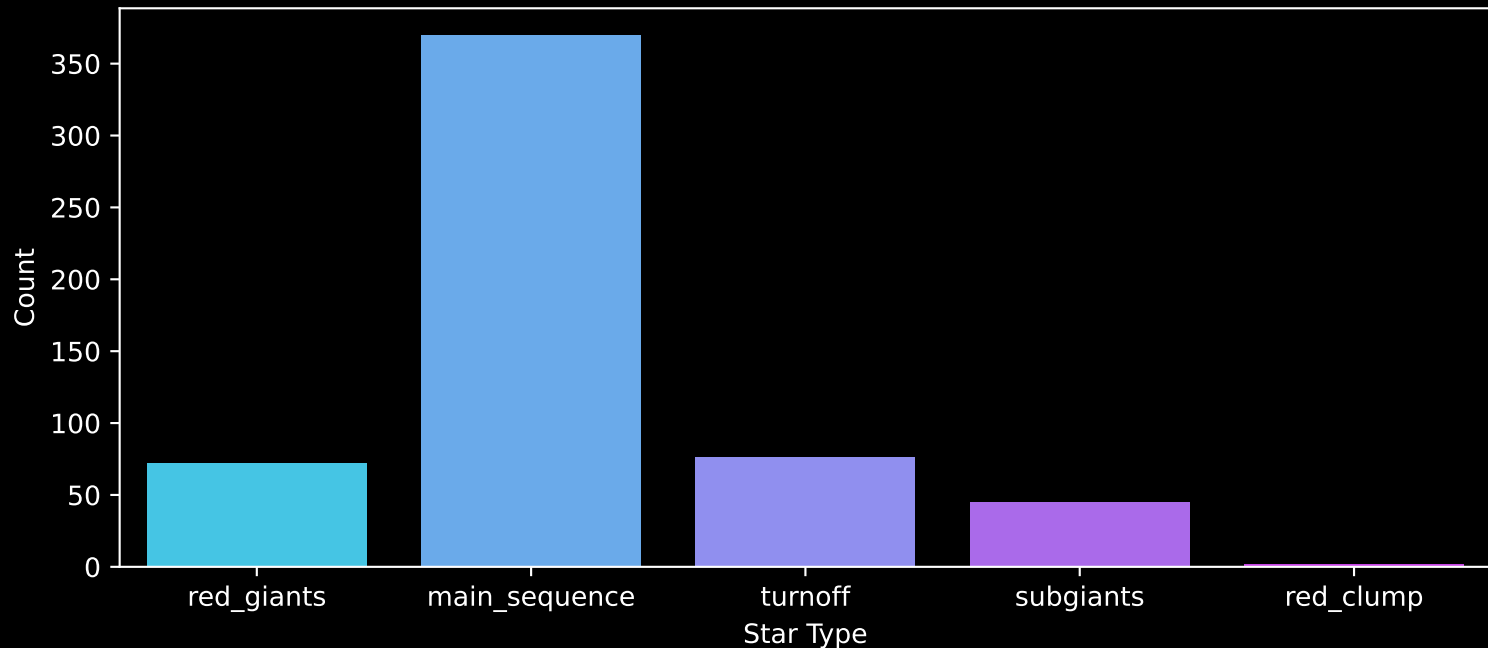
Gaia Cluster: [IC_1434] Count plot of Star Type
