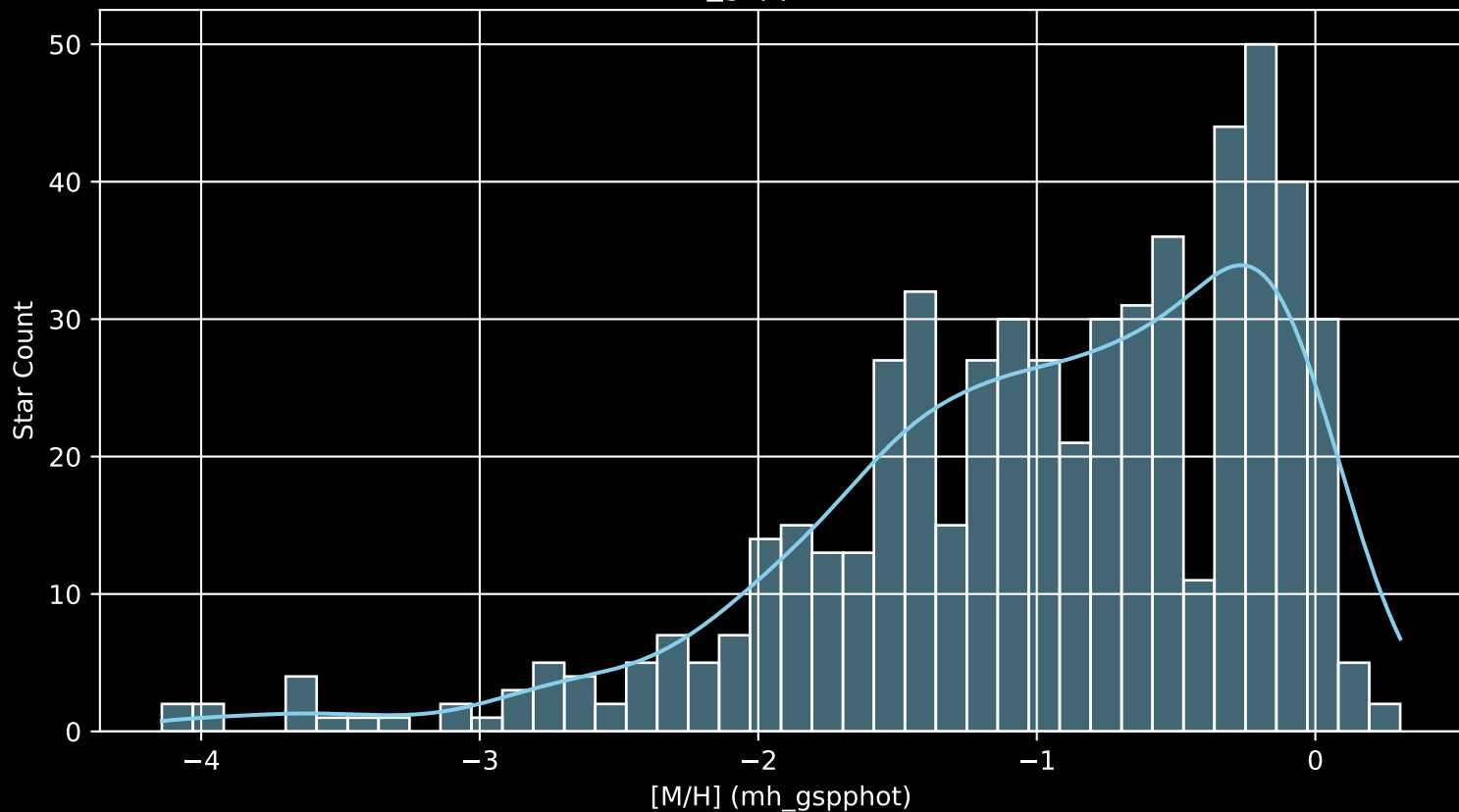
Gaia Cluster: [IC_1434 [M/H] (mh_gspphot) (n= 565)
