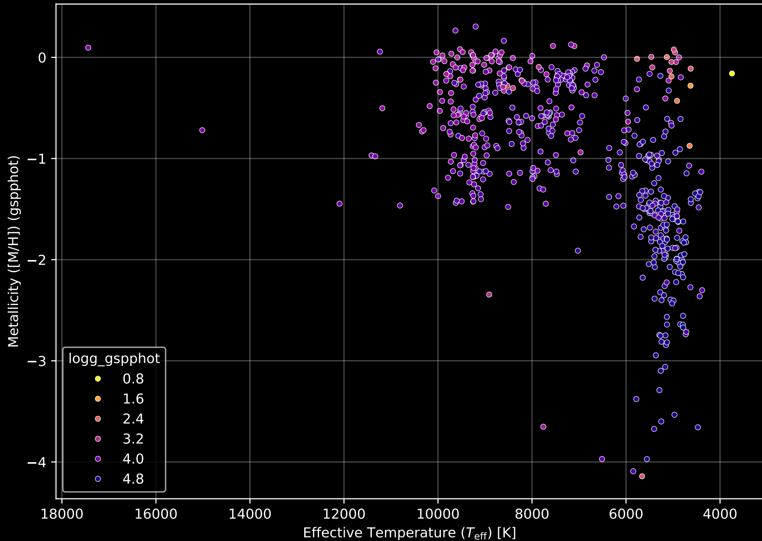
Gaia Cluster: [IC_1434] Stellar Population Parameters (n= 565)
