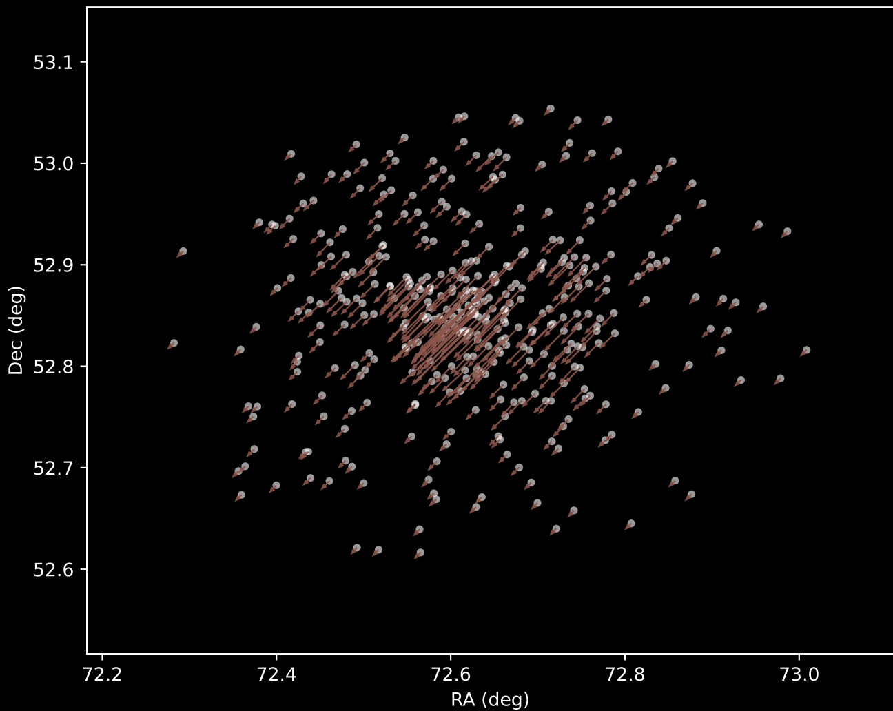
Gaia DR3 Cluster 10 Proper Motion Vectors (n=387)
