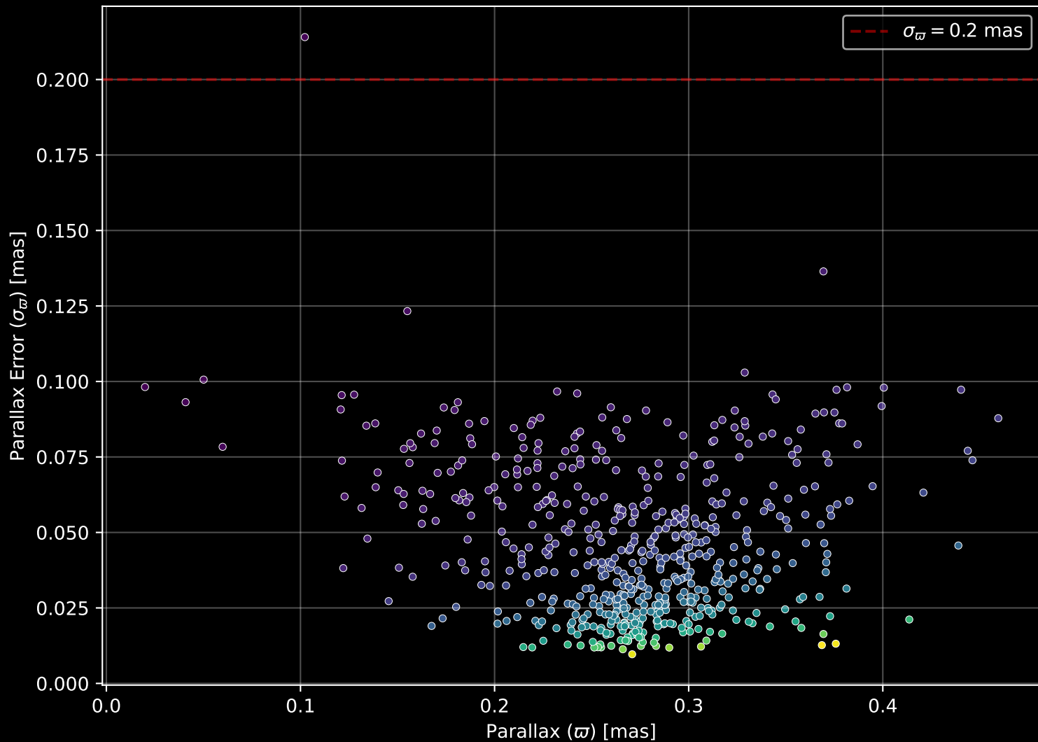
Gaia Cluster: [IC_1434] Parallax Quality (n= 565)
