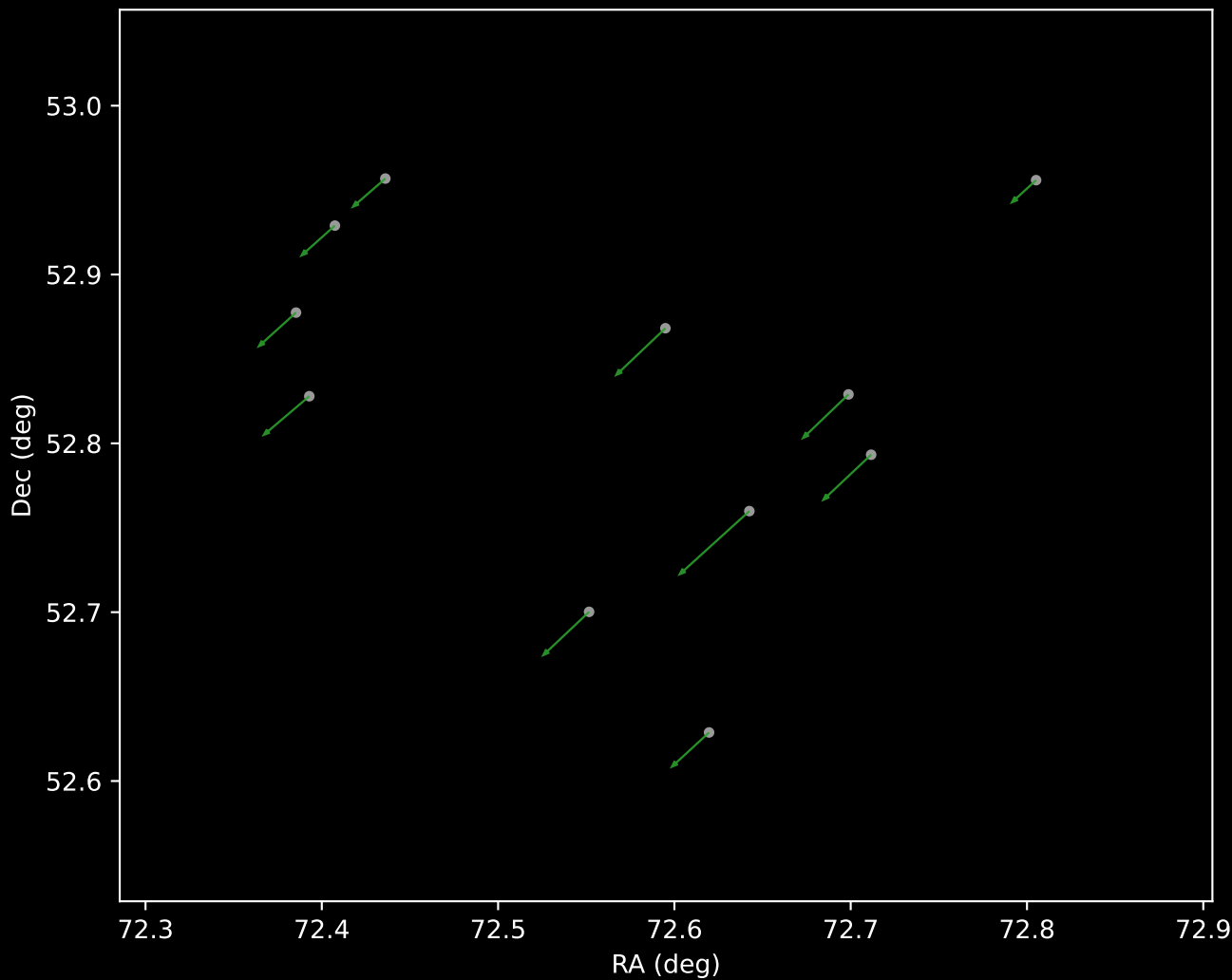
Gaia DR3 Cluster 4 Proper Motion Vectors (n=11)
