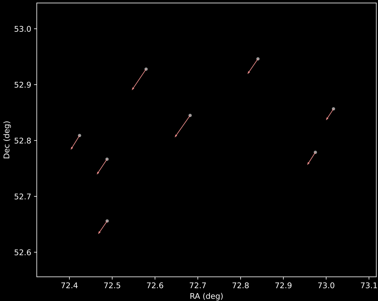
Gaia DR3 Cluster 7 Proper Motion Vectors (n=8)
