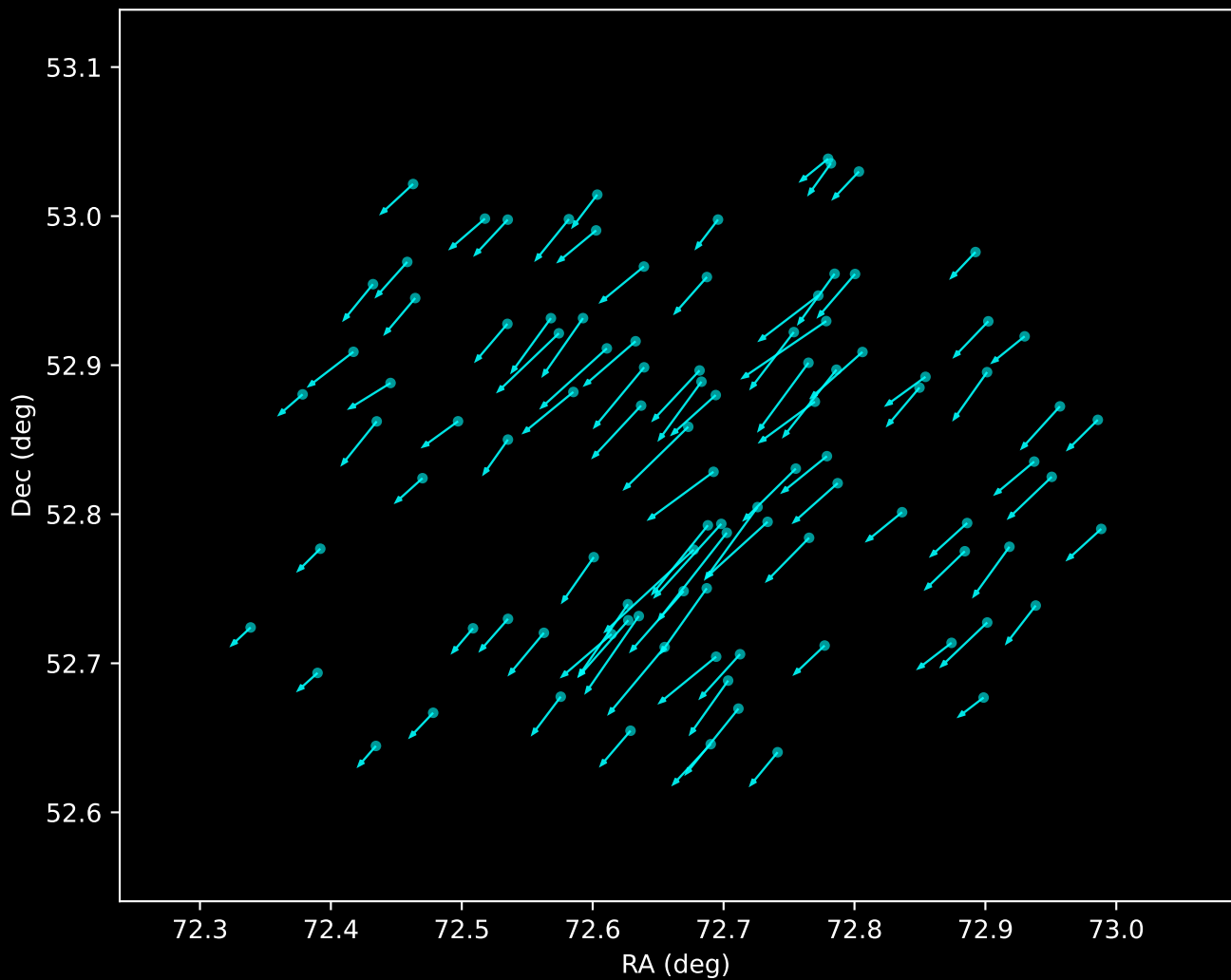
Gaia DR3 Noise Stream Proper Motion Vectors (n=99)
