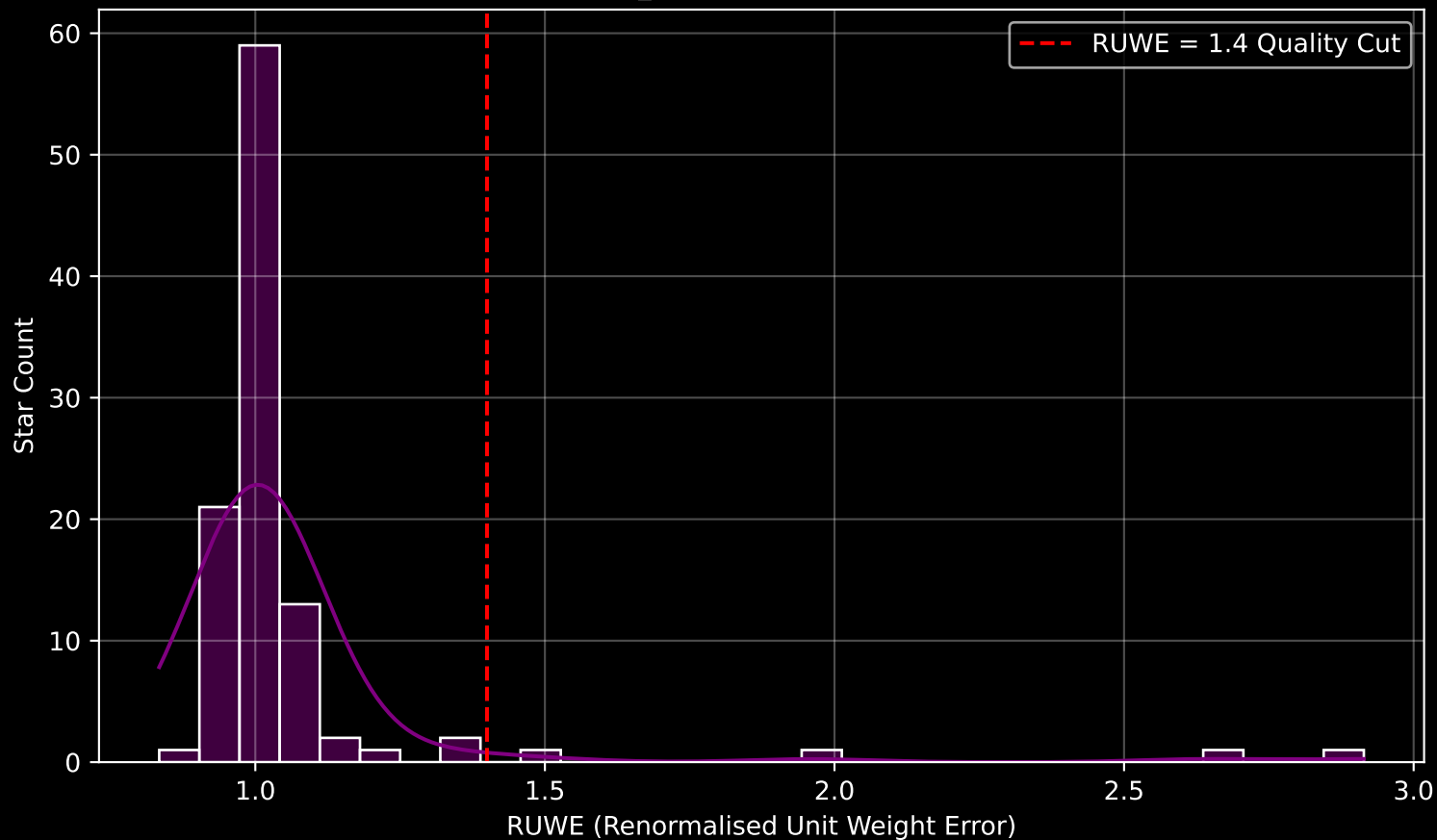
Gaia Cluster: [IC_1590] RUWE Distribution (n= 103)
