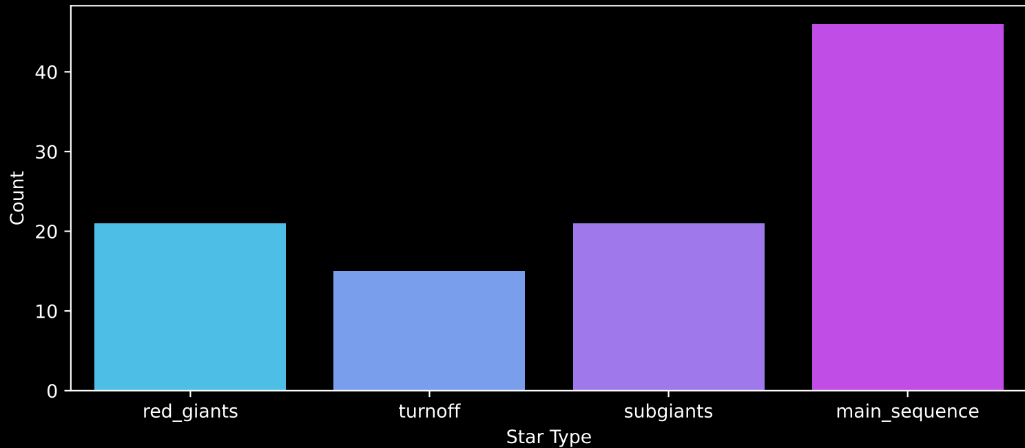
Gaia Cluster: [IC_1590] Count plot of Star Type
