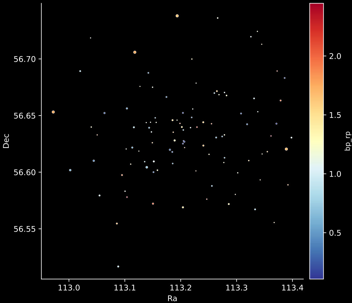
Gaia Cluster: [IC_1590] Stars: 103
