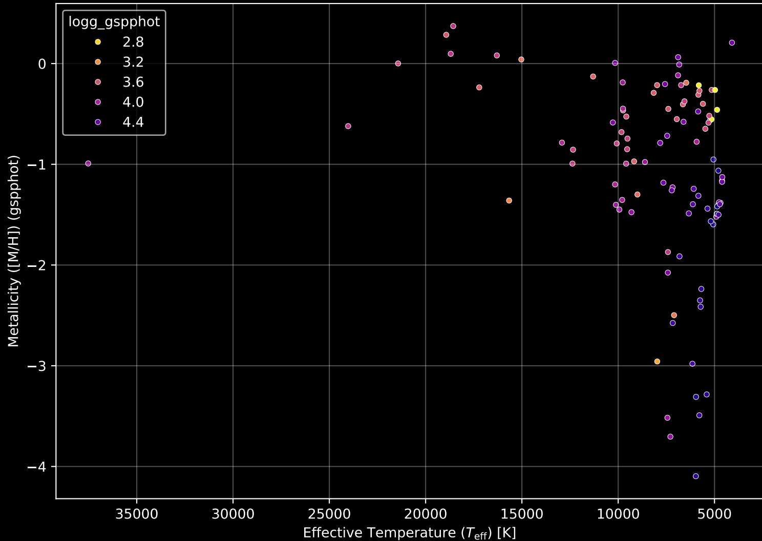
Gaia Cluster: [IC_1590] Stellar Population Parameters (n= 103)
