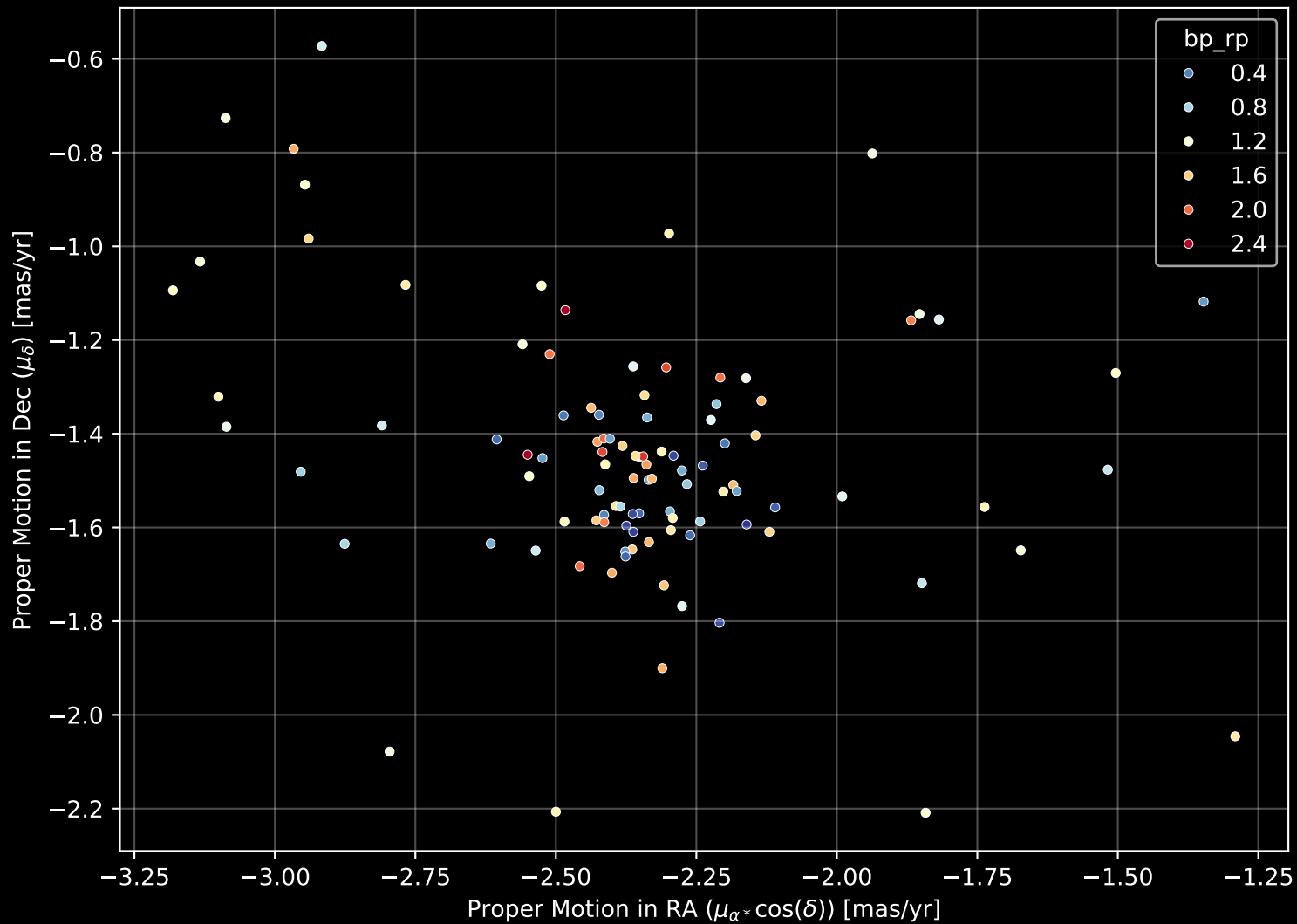
Gaia Cluster: [IC_1590] Proper Motion Diagram (n= 103)
