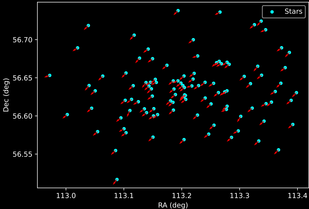
Gaia Cluster: [IC_1590] Proper Motion Vectors for Gaia Star Field (n= 103)
