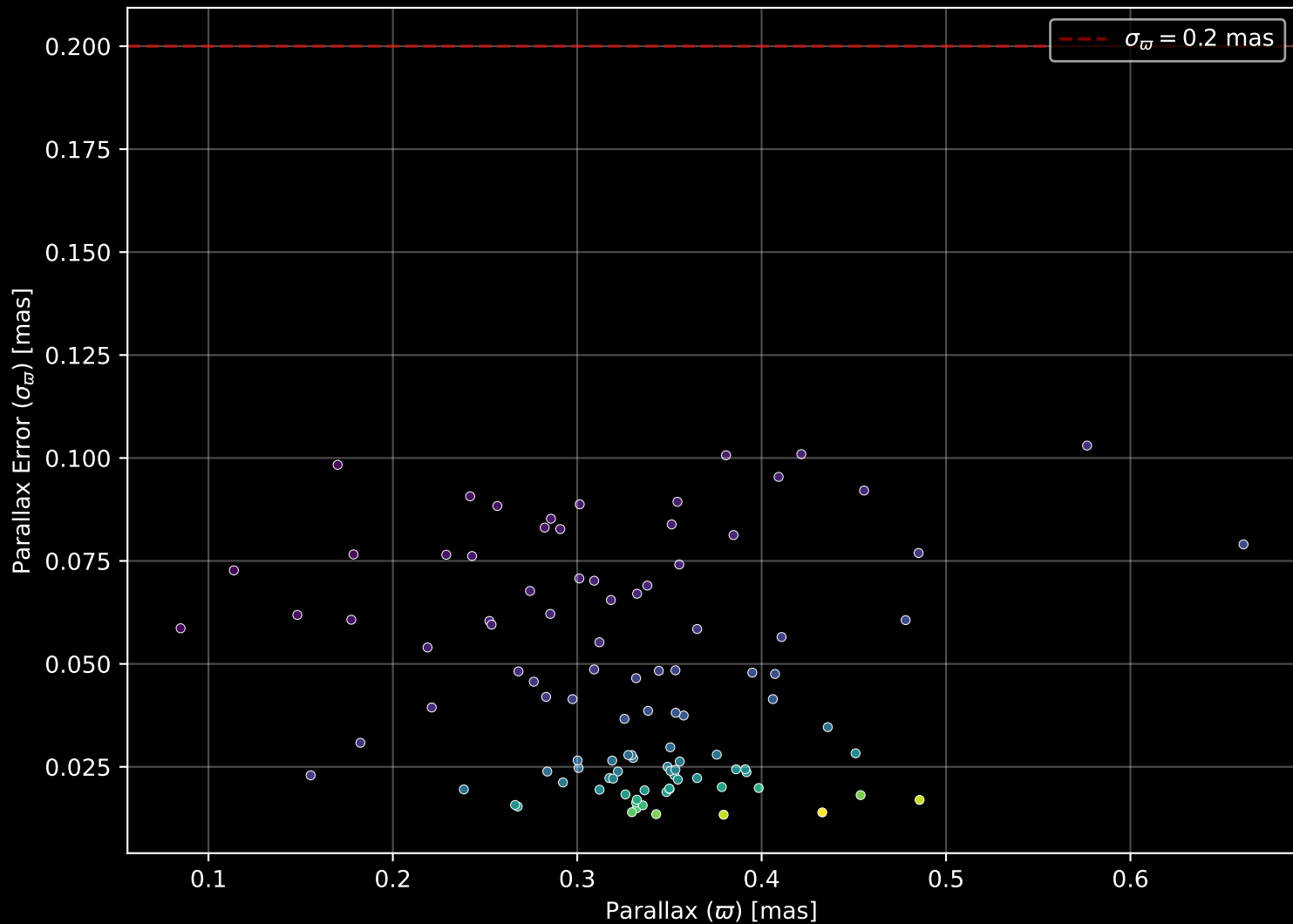
Gaia Cluster: [IC_1590] Parallax Quality (n= 103)
