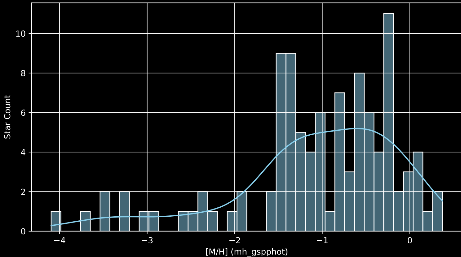
Gaia Cluster: [IC_1590 [M/H] (mh_gspphot) (n= 103)
