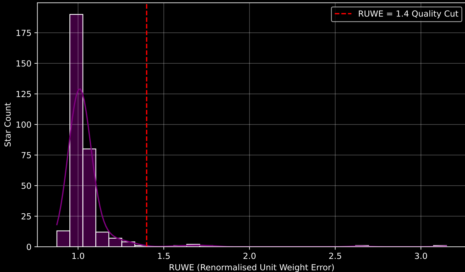
Gaia Cluster: [IC_1805] RUWE Distribution (n= 313)
