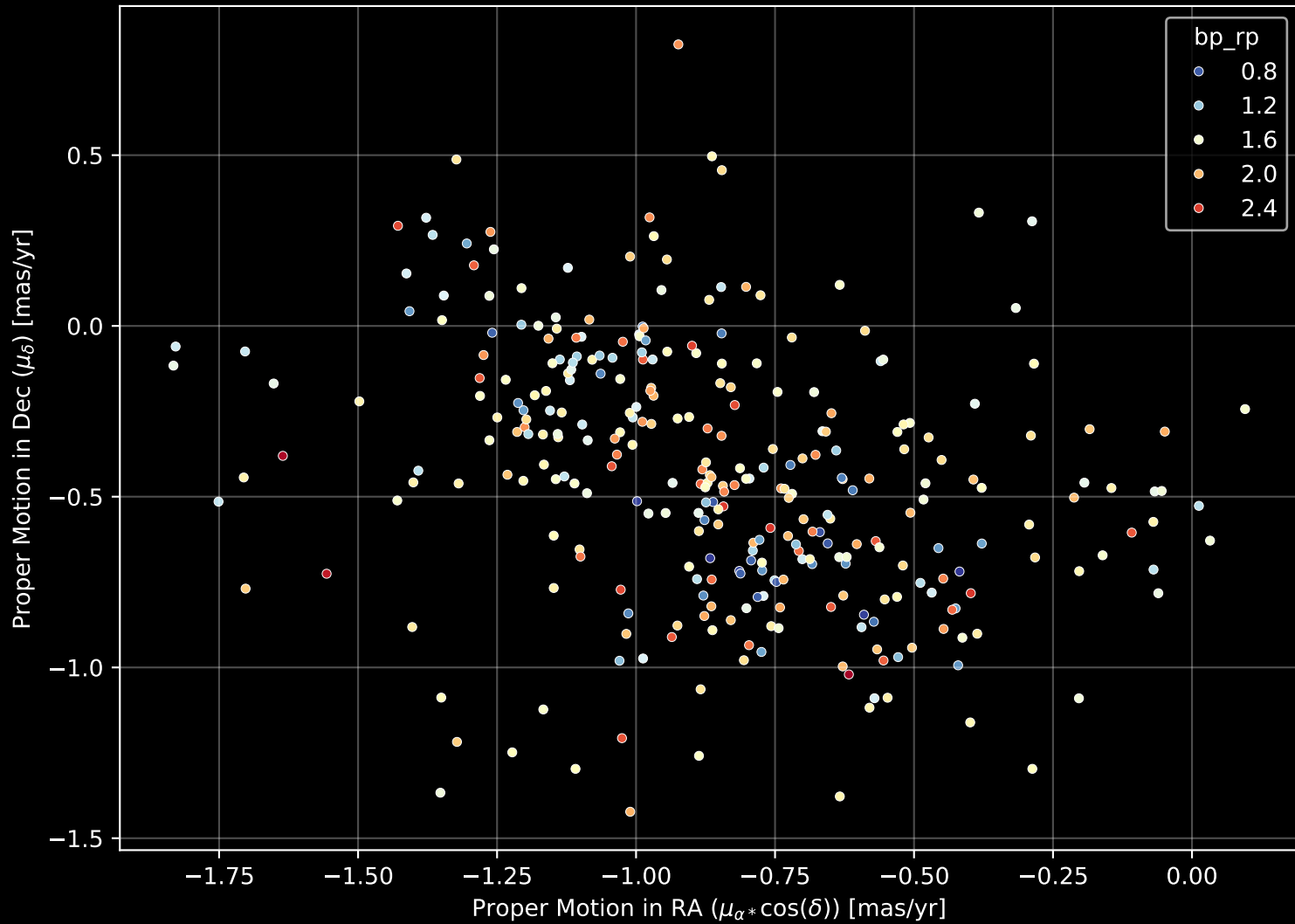
Gaia Cluster: [IC_1805] Proper Motion Diagram (n= 313)
