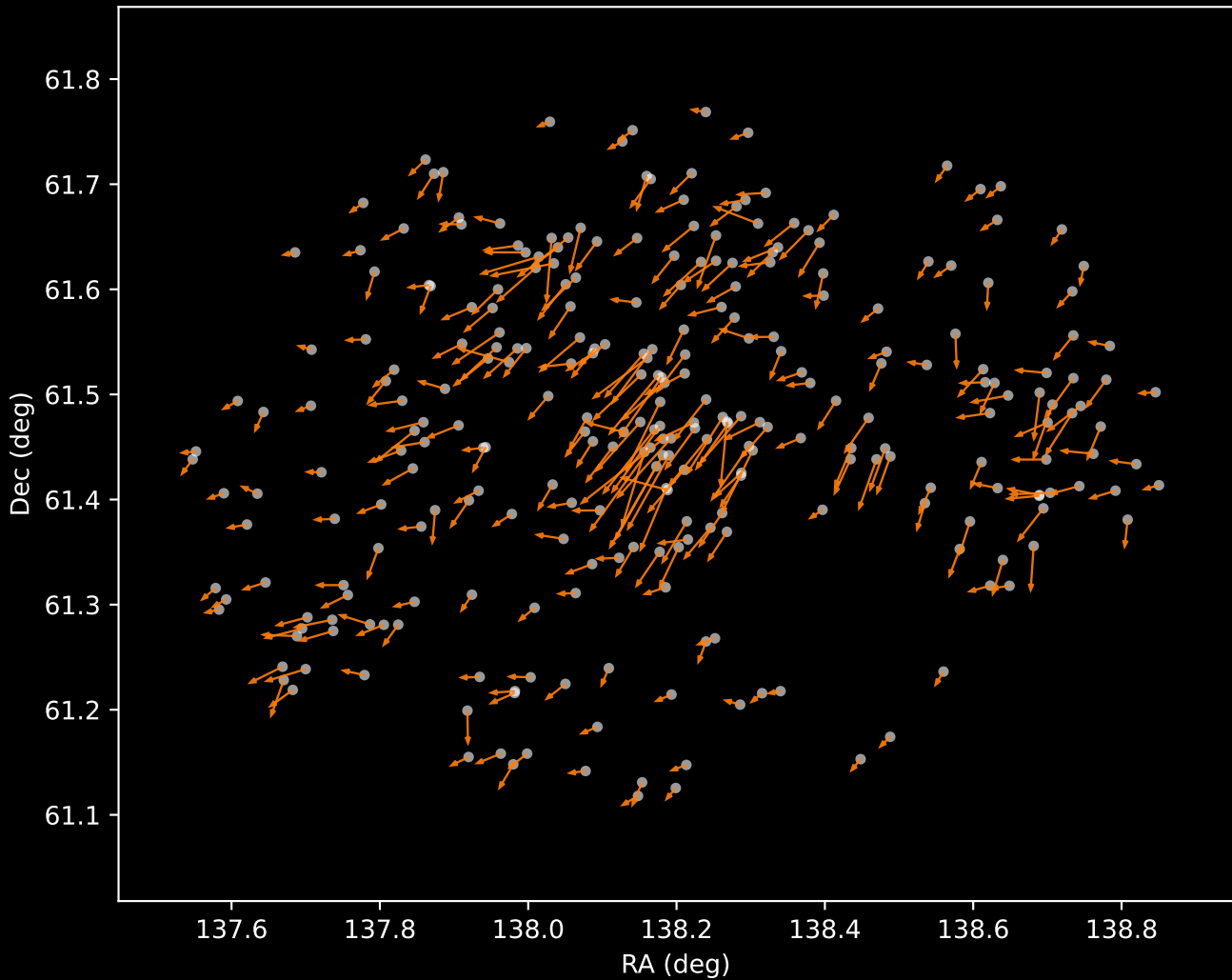
Gaia DR3 Cluster 2 Proper Motion Vectors (n=281)
