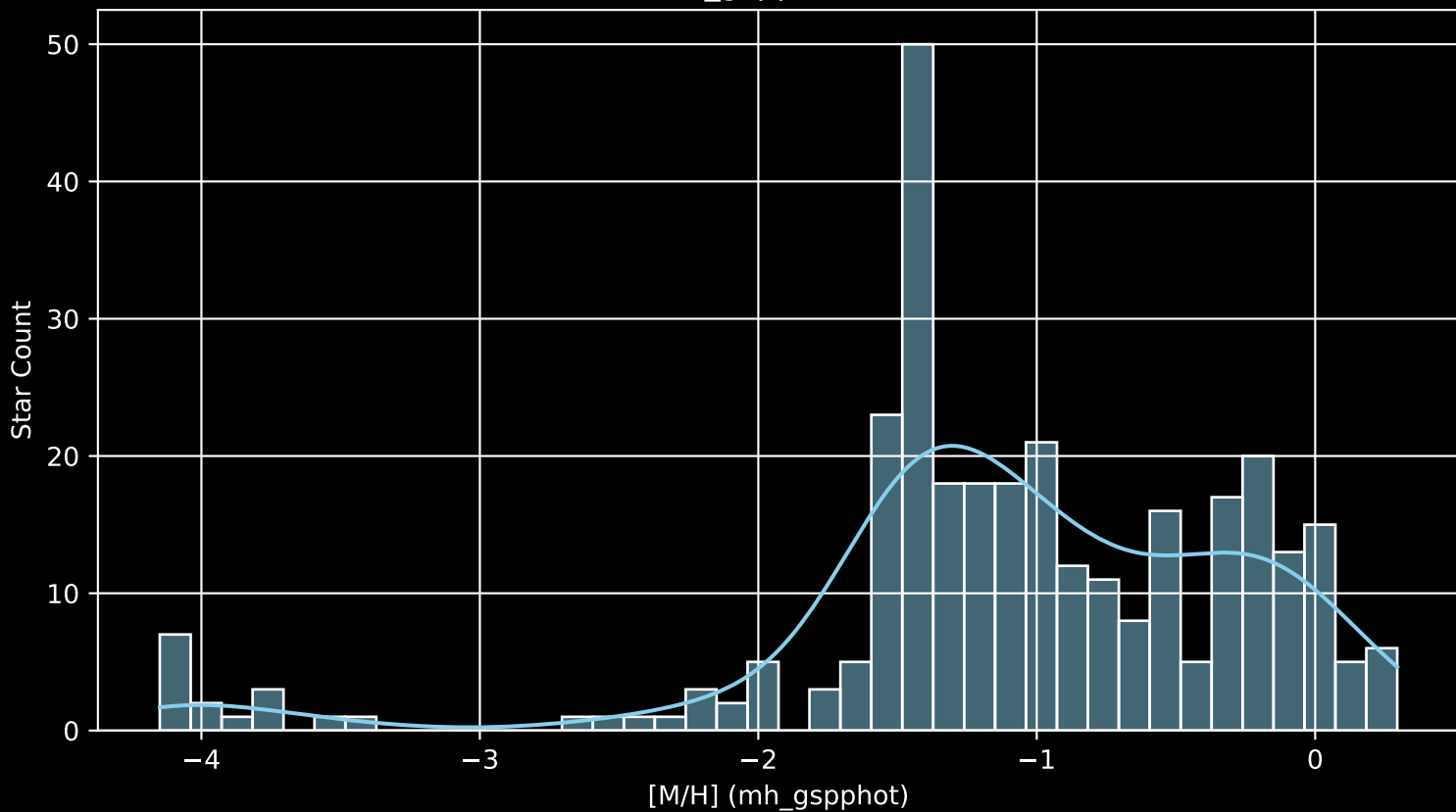
Gaia Cluster: [IC_1805 [M/H] (mh_gspphot) (n= 313)
