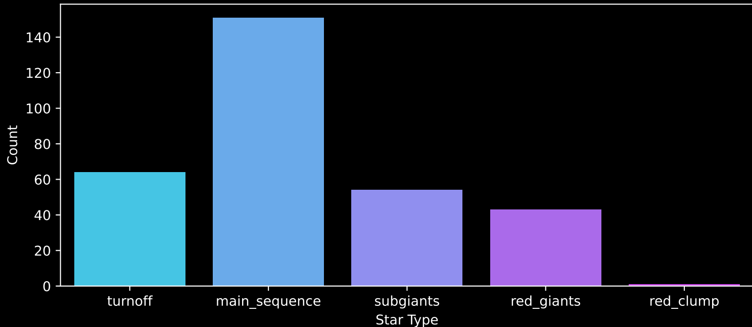
Gaia Cluster: [IC_1805] Count plot of Star Type
