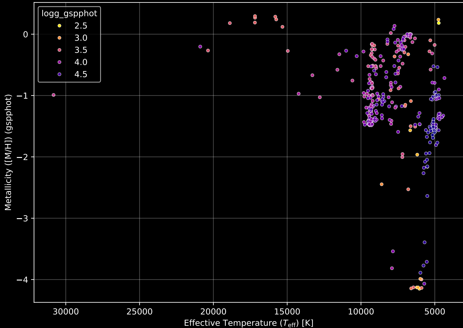
Gaia Cluster: [IC_1805] Stellar Population Parameters (n= 313)
