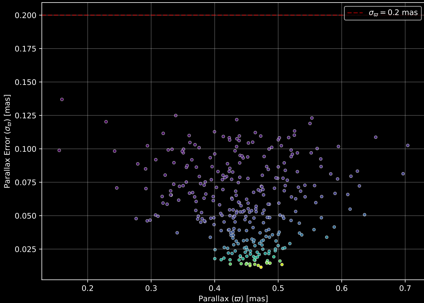
Gaia Cluster: [IC_1805] Parallax Quality (n= 313)
