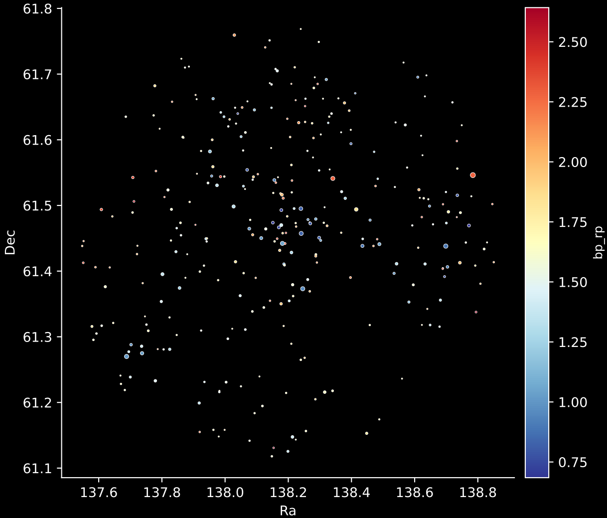
Gaia Cluster: [IC_1805] Stars: 313
