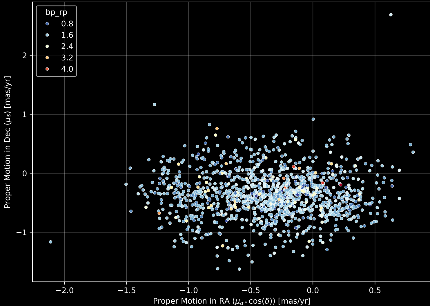
Gaia Cluster: [IC_1848] Proper Motion Diagram (n= 1269)
