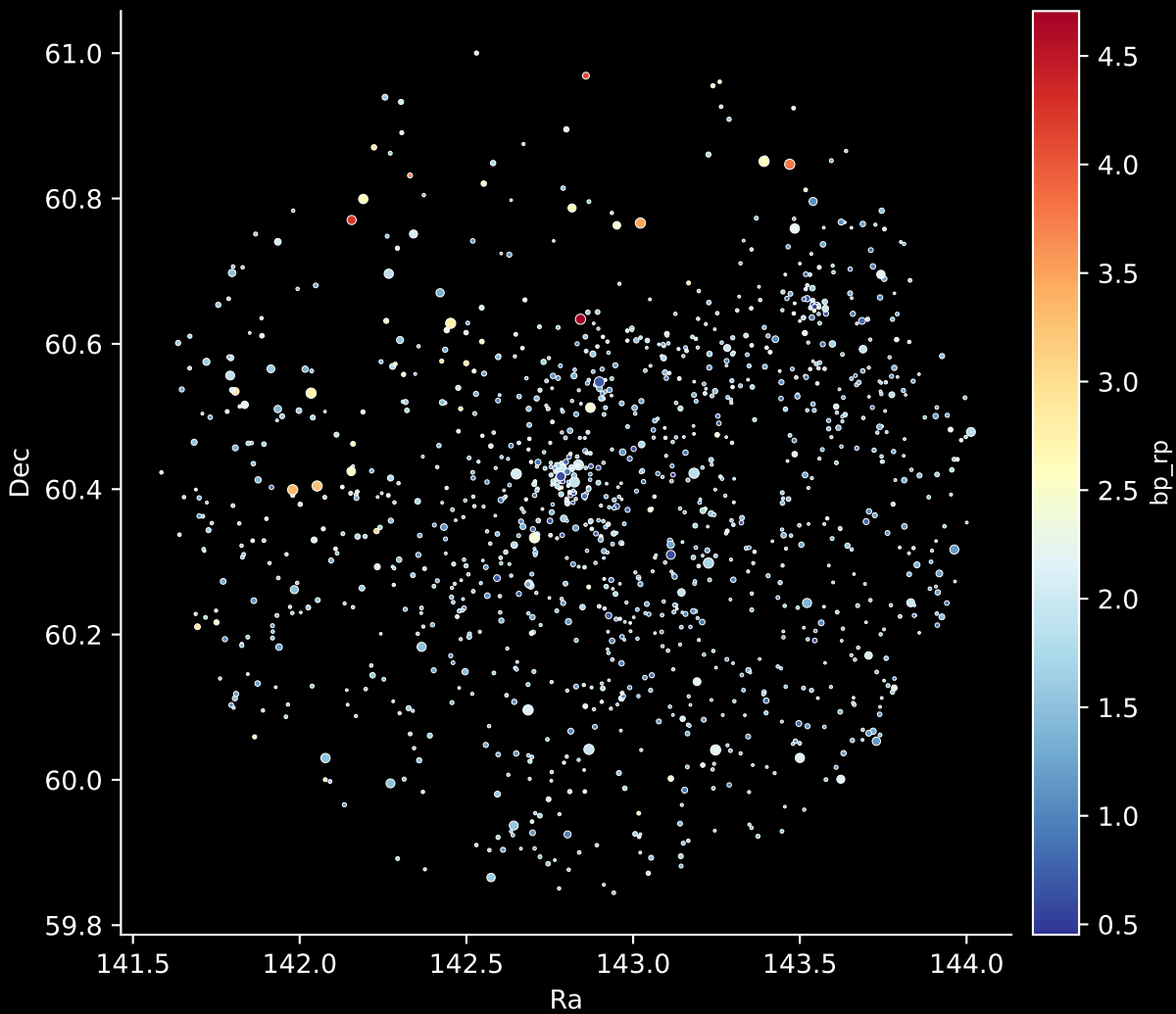
Gaia Cluster: [IC 1848] Stars: 1269
