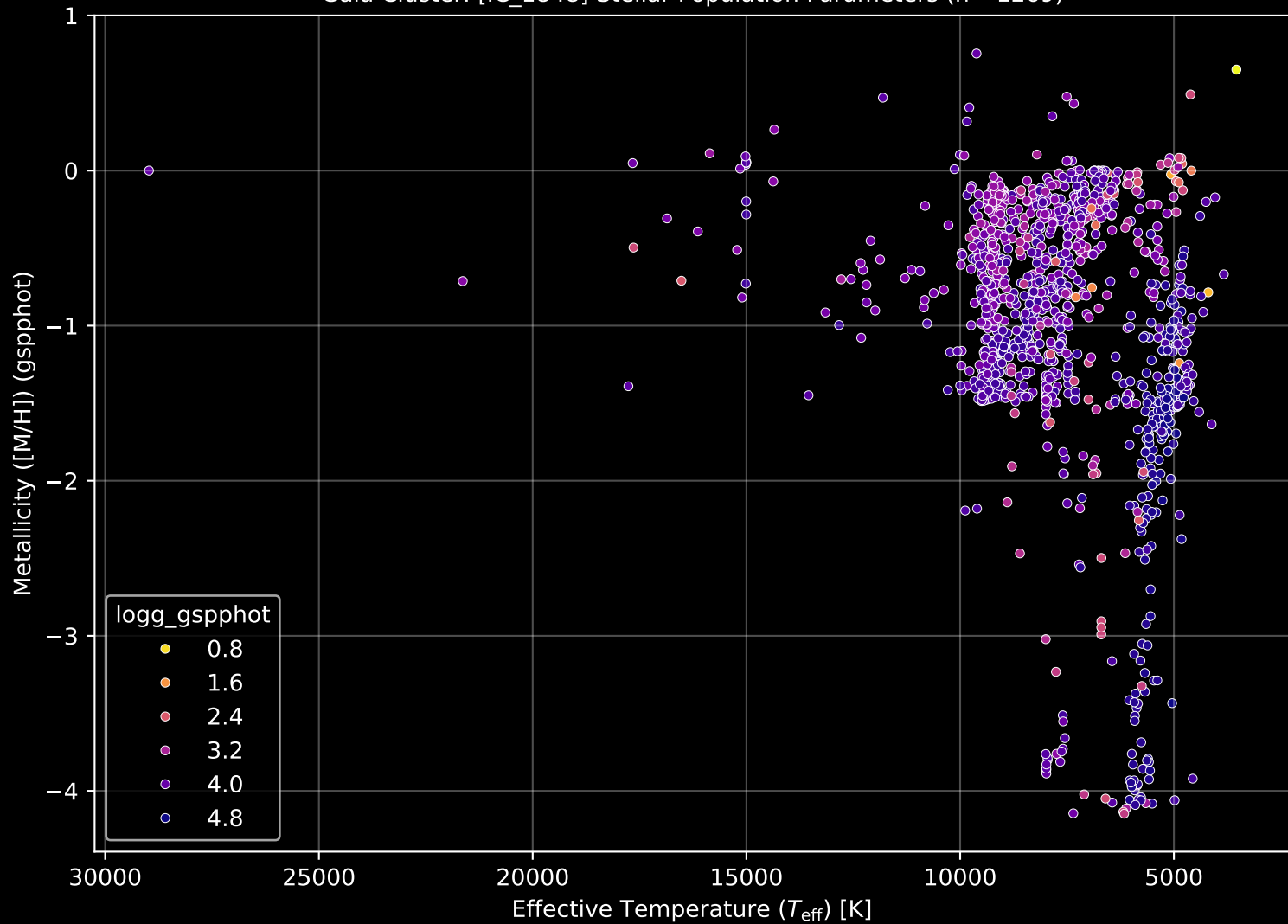
Gaia Cluster: [IC_1848] Stellar Population Parameters (n= 1269)
