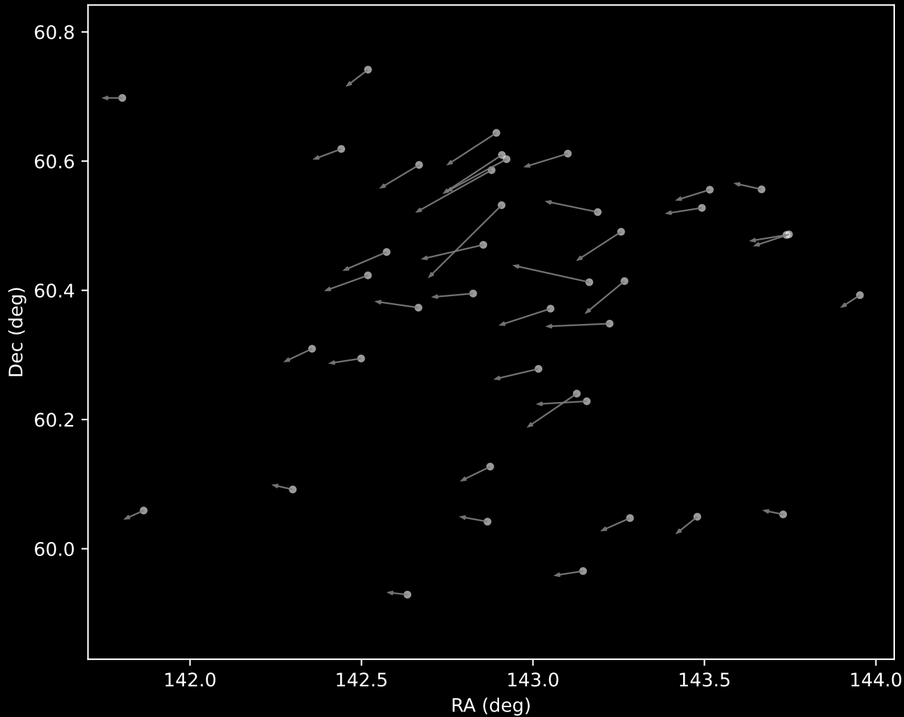
Gaia DR3 Cluster 34 Proper Motion Vectors (n=41)
