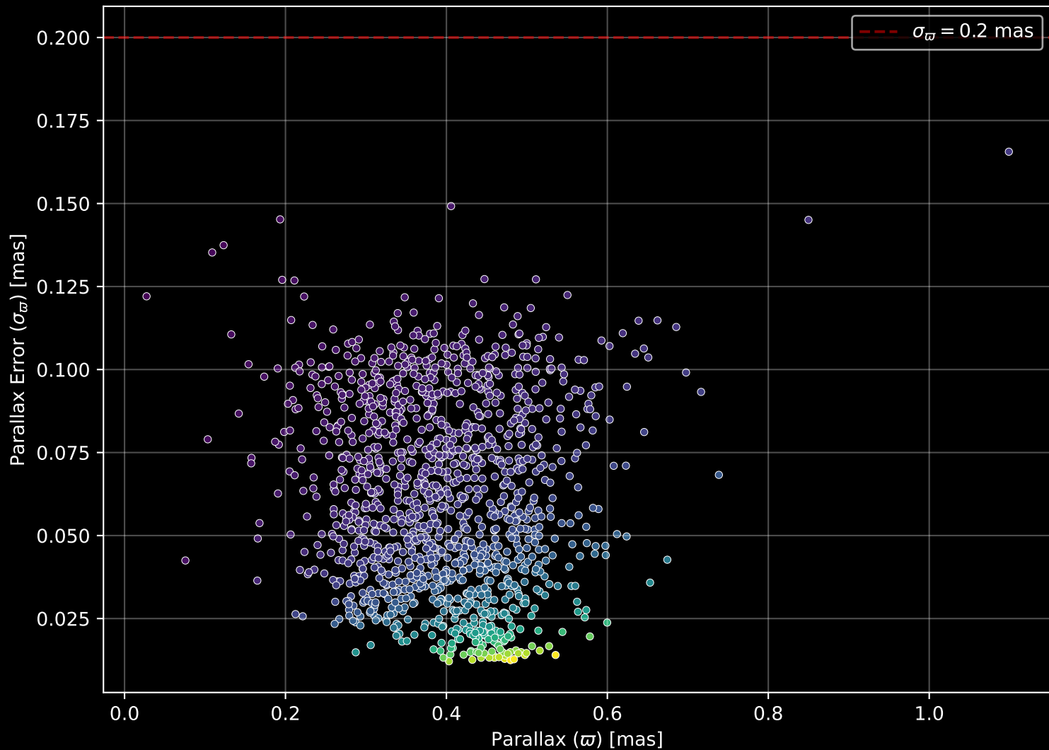
Gaia Cluster: [IC_1848] Parallax Quality (n= 1269)
