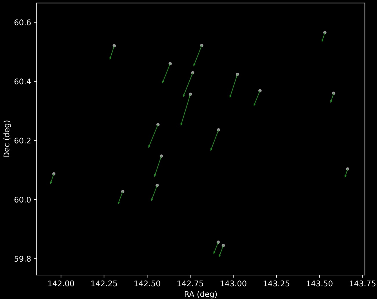
Gaia DR3 Cluster 64 Proper Motion Vectors (n=18)
