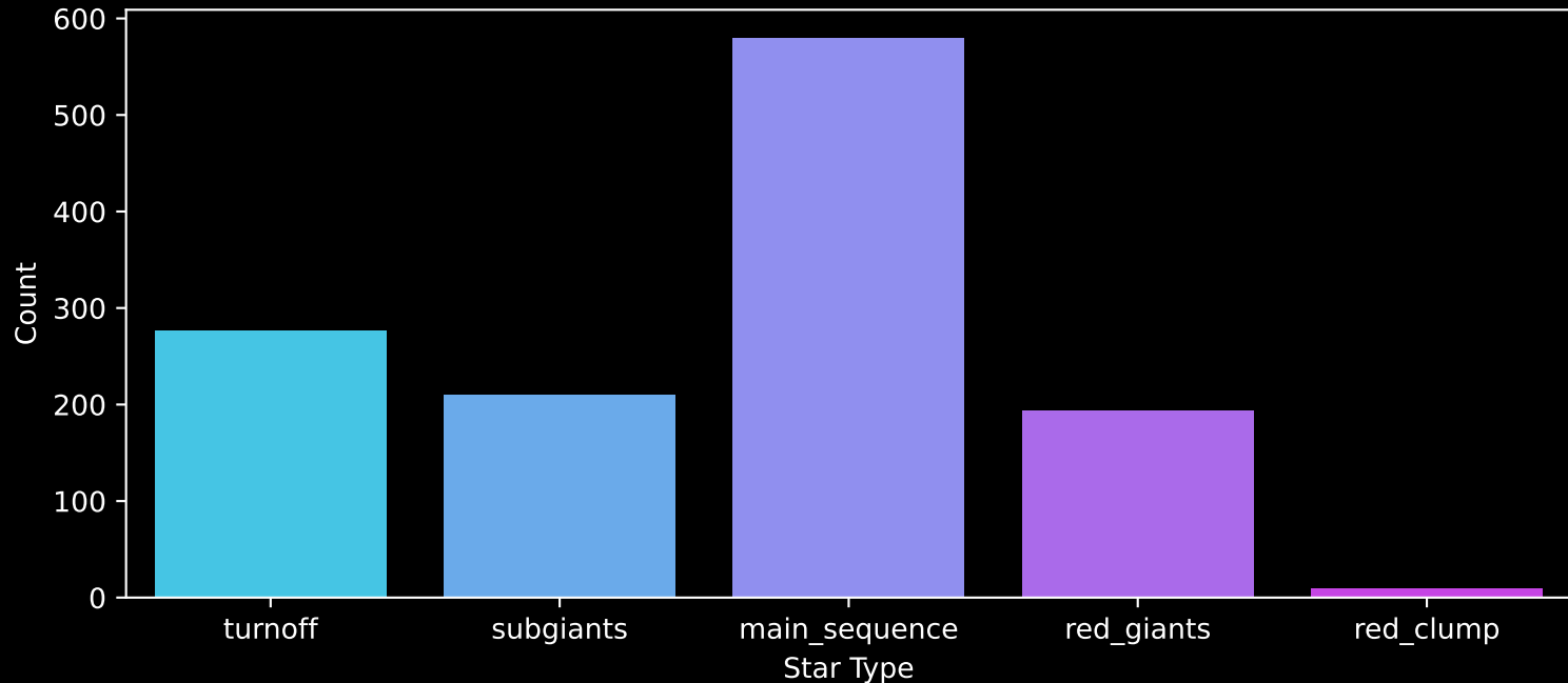
Gaia Cluster: [IC_1848] Count plot of Star Type
