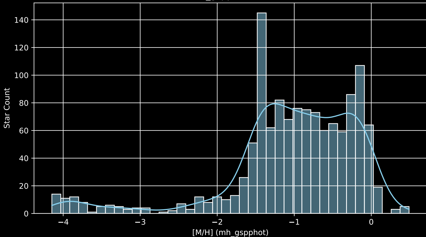
Gaia Cluster: [IC_1848 [M/H] (mh_gspphot) (n= 1267)
