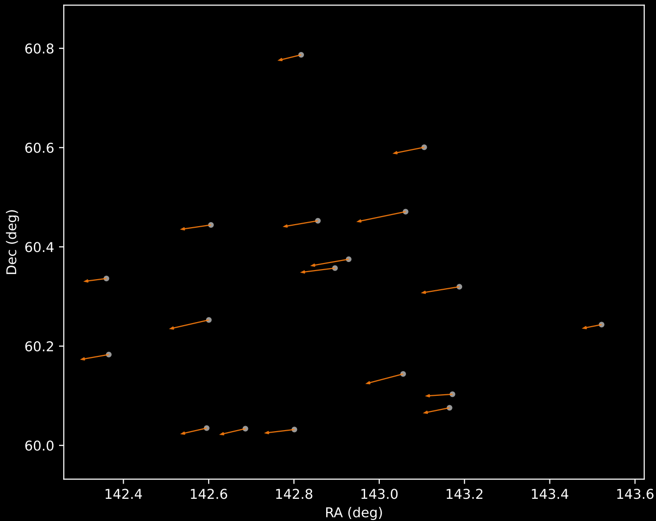
Gaia DR3 Cluster 22 Proper Motion Vectors (n=18)
