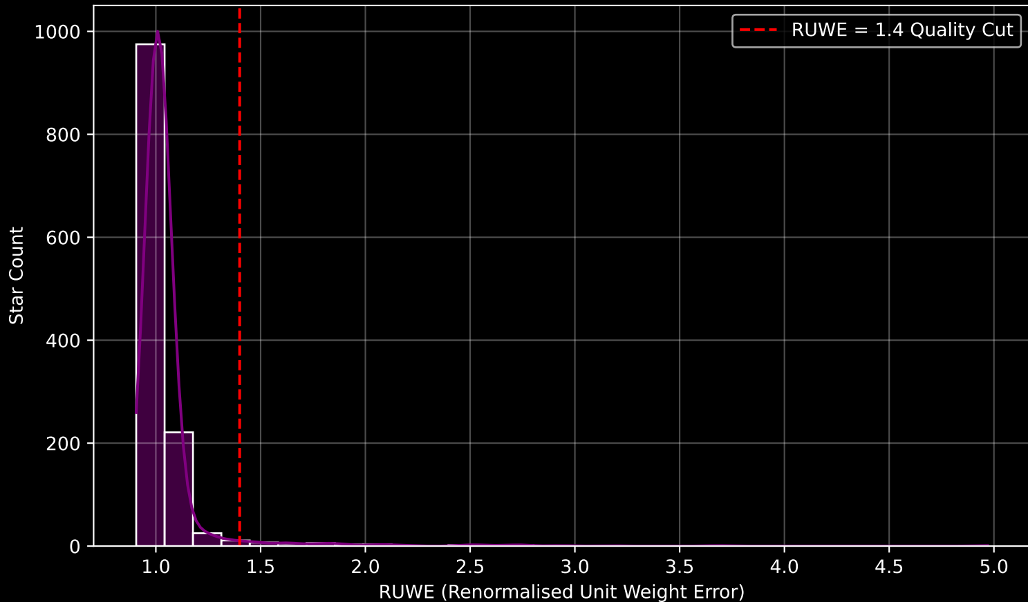
Gaia Cluster: [IC_1848] RUWE Distribution (n= 1267)
