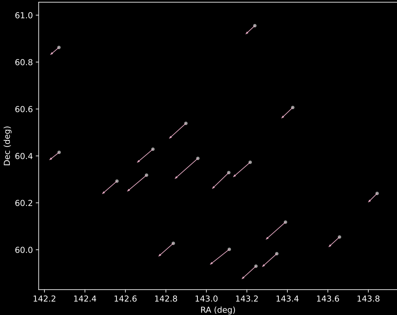
Gaia DR3 Cluster 13 Proper Motion Vectors (n=18)
