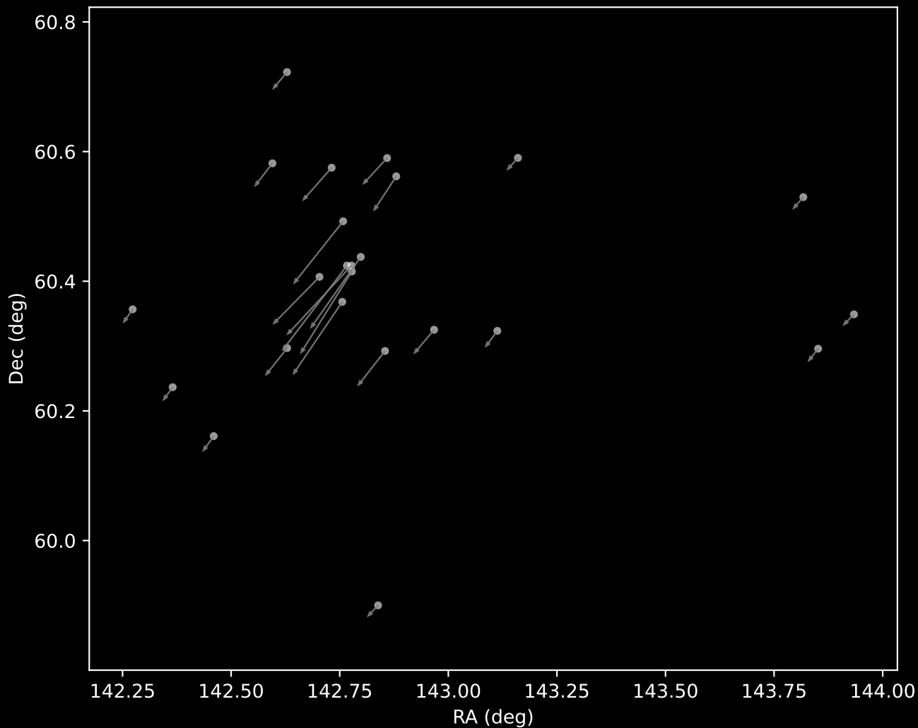
Gaia DR3 Cluster 54 Proper Motion Vectors (n=24)
