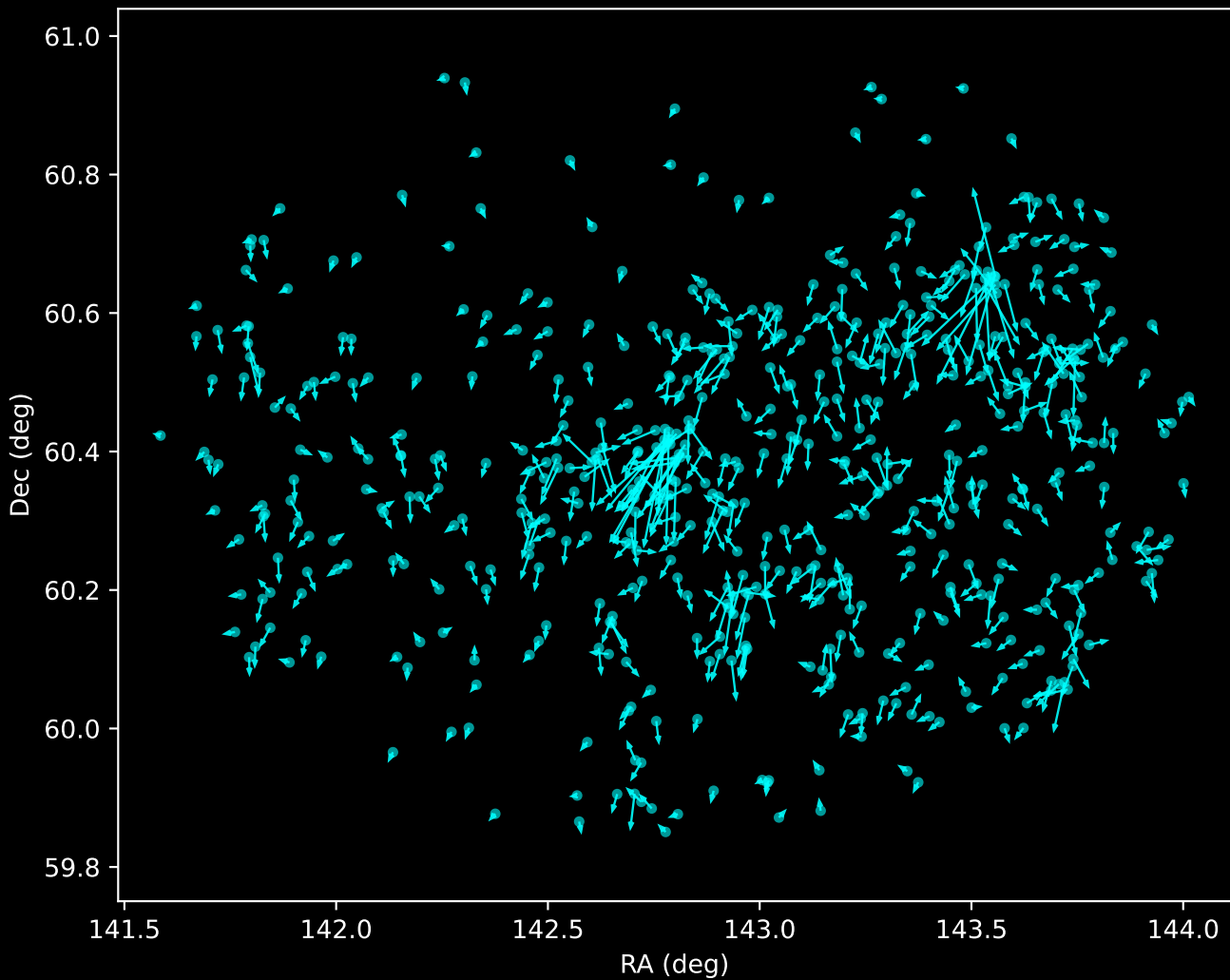
Gaia DR3 Noise Stream Proper Motion Vectors (n=555)
