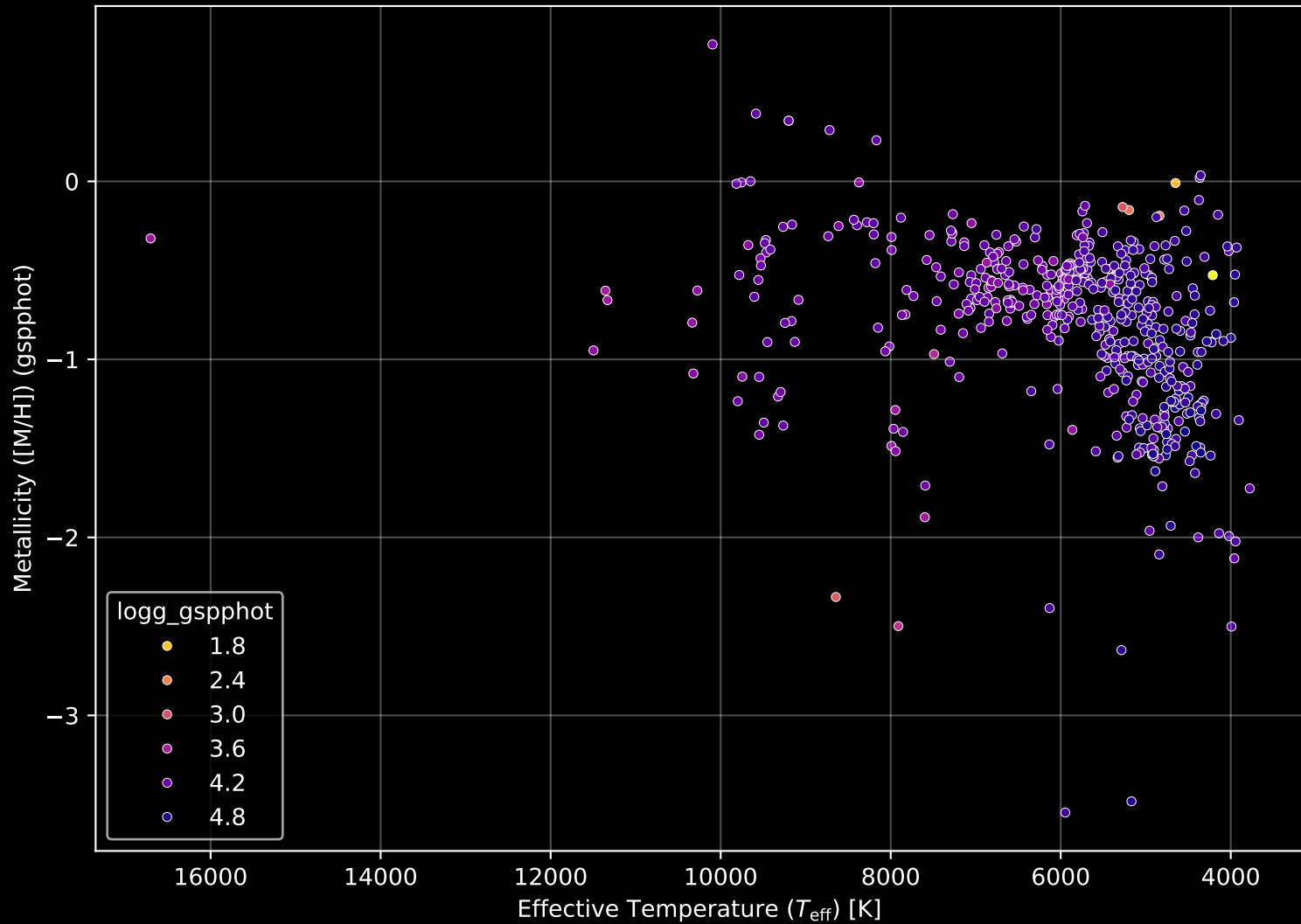
Gaia Cluster: [IC_2488] Stellar Population Parameters (n= 540)
