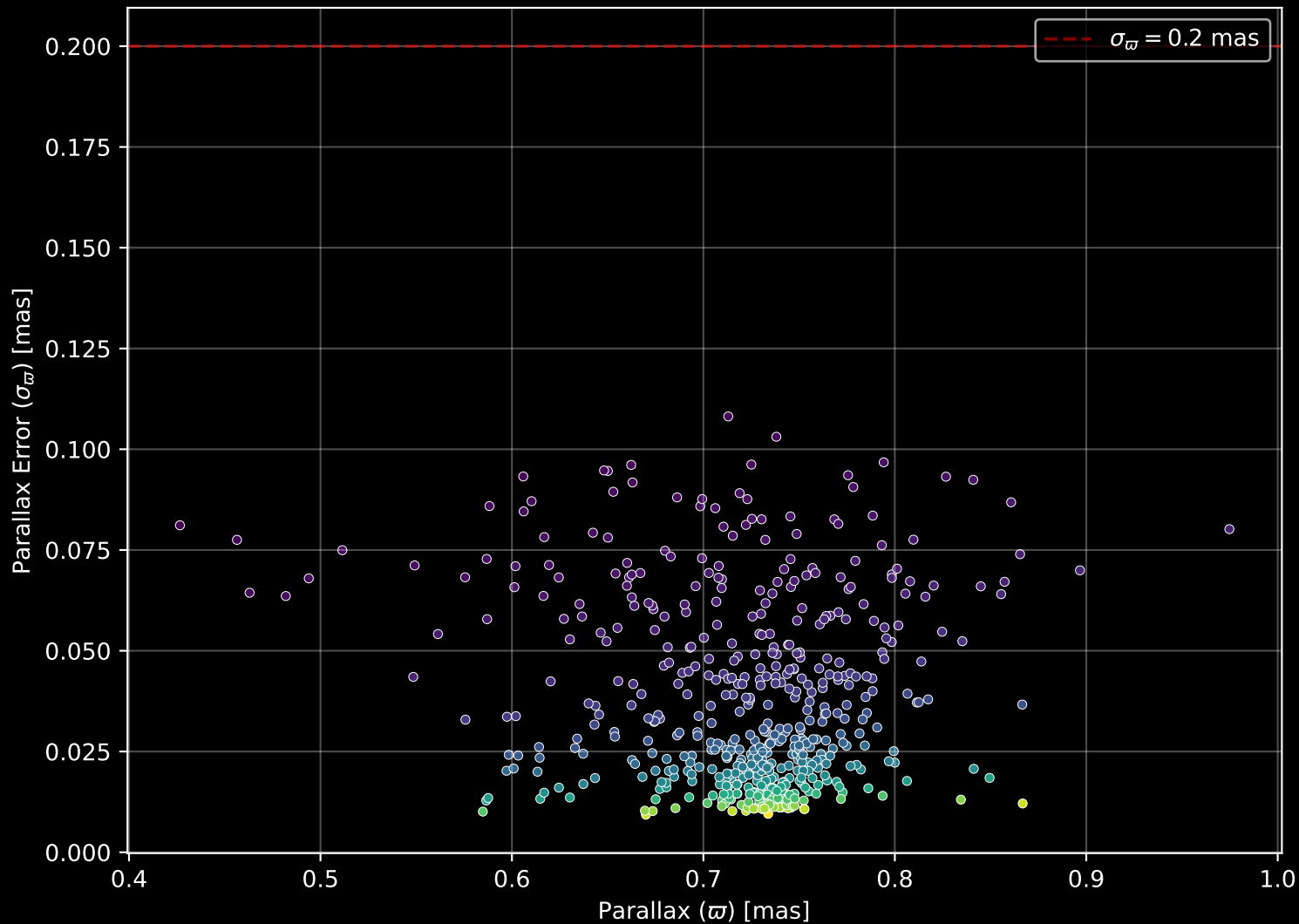
Gaia Cluster: [IC_2488] Parallax Quality (n= 540)
