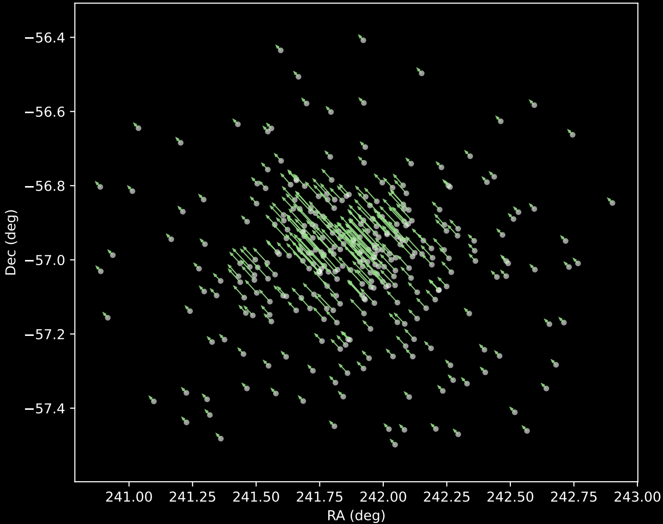
Gaia DR3 Cluster 5 Proper Motion Vectors (n=309)
