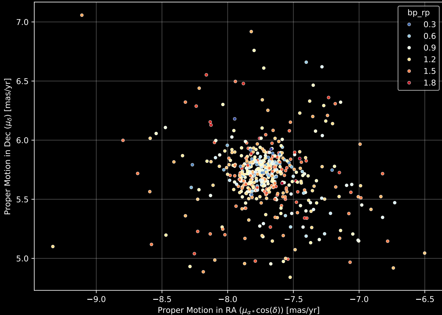
Gaia Cluster: [IC_2488] Proper Motion Diagram (n= 540)
