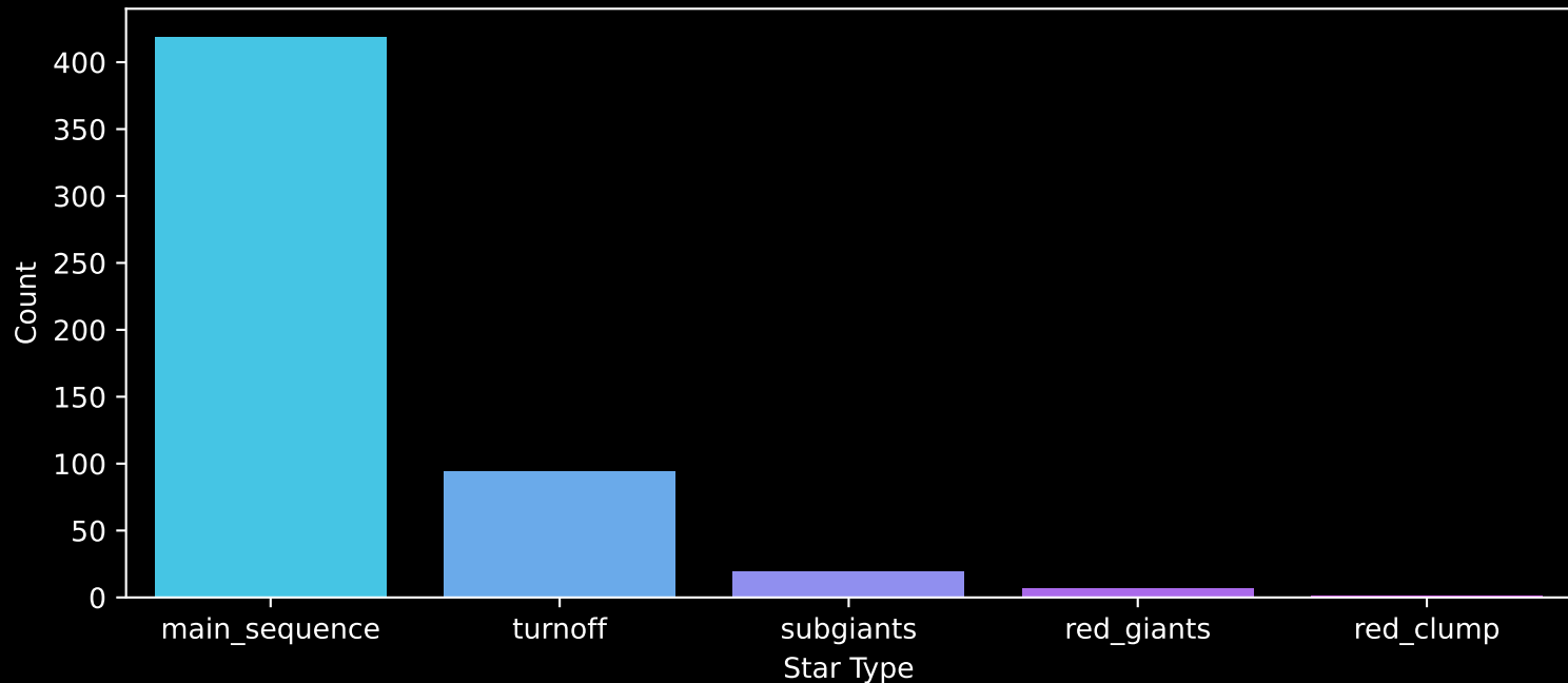
Gaia Cluster: [IC_2488] Count plot of Star Type
