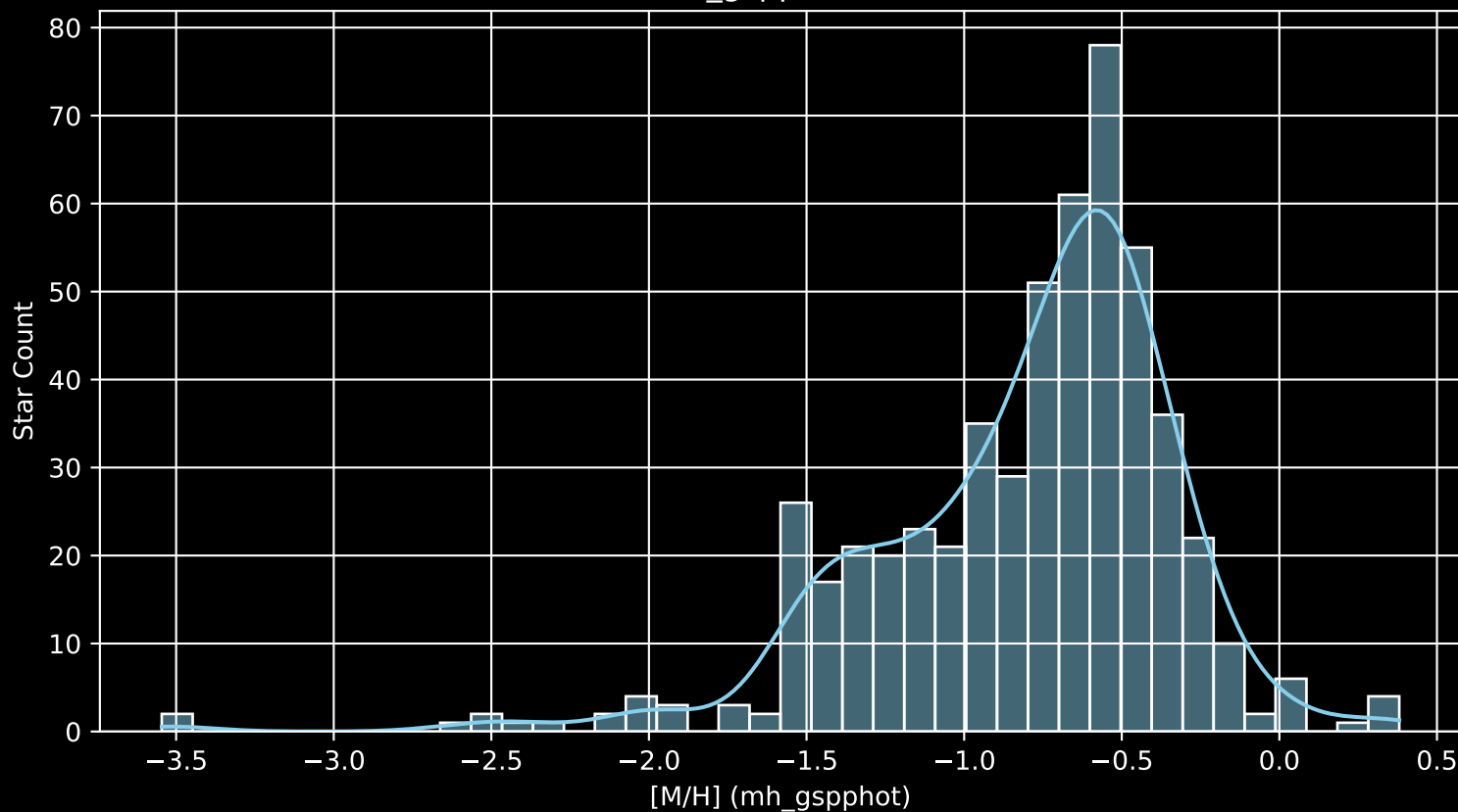
Gaia Cluster: [IC_2488 [M/H] (mh_gspphot) (n= 539)
