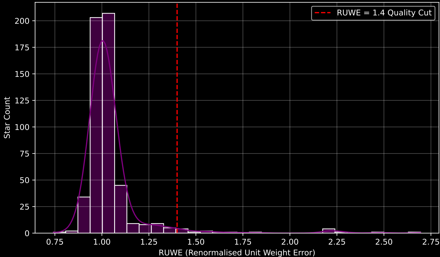
Gaia Cluster: [IC_2488] RUWE Distribution (n= 540)
