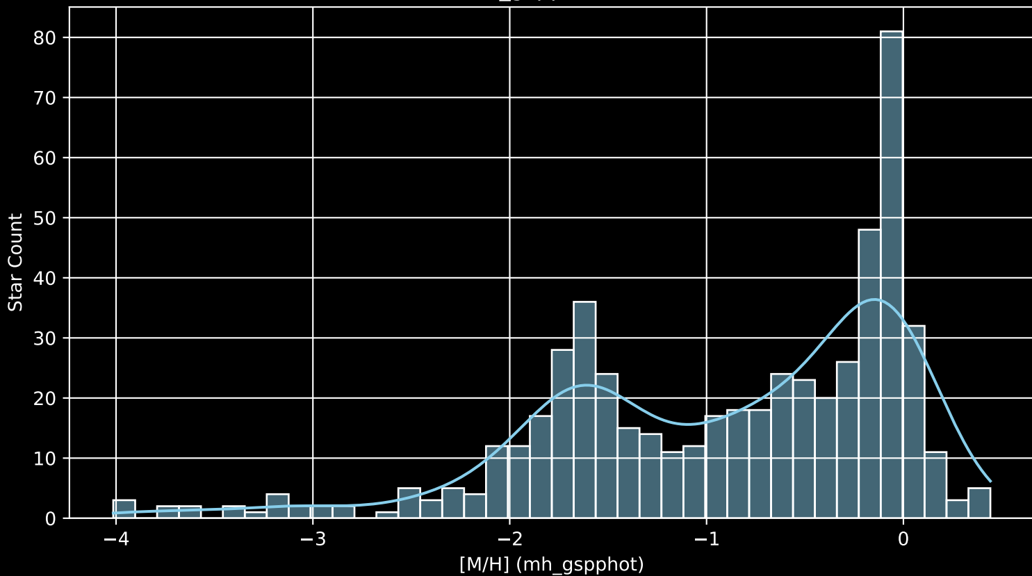
Gaia Cluster: [IC_361 [M/H] (mh_gspphot) (n= 545)
