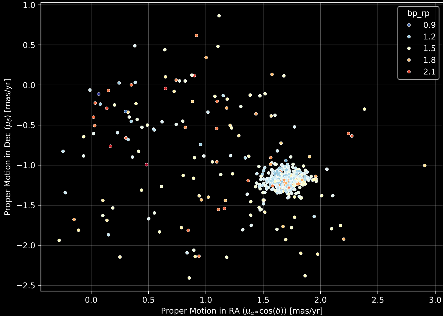
Gaia Cluster: [IC_361] Proper Motion Diagram (n= 545)
