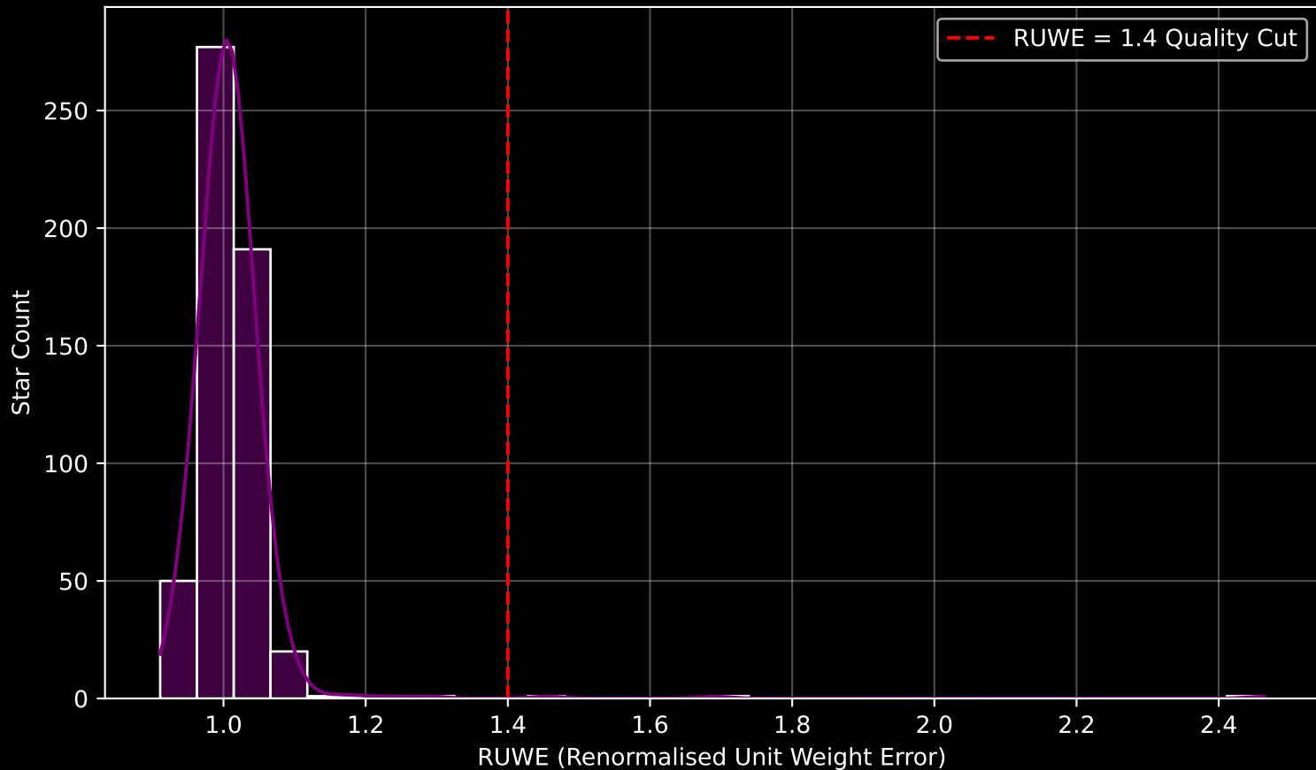
Gaia Cluster: [IC_361] RUWE Distribution (n= 545)
