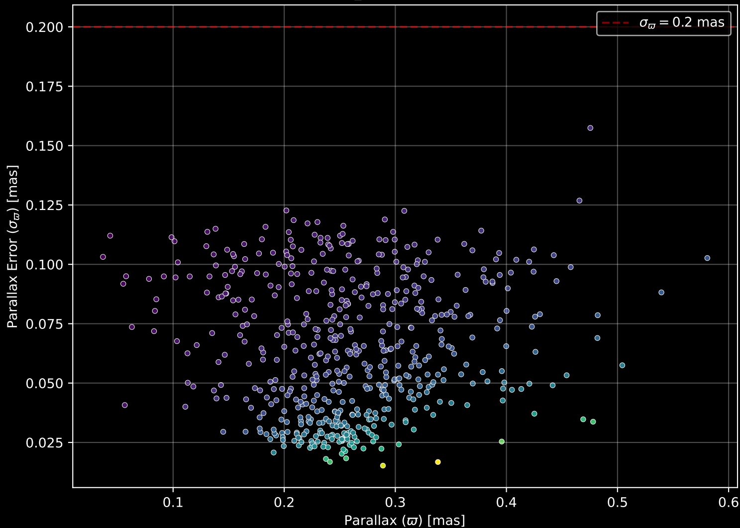
Gaia Cluster: [IC_361] Parallax Quality (n= 545)
