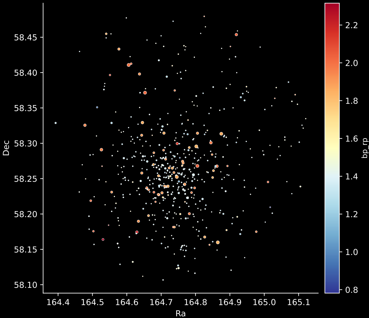
Gaia Cluster: [IC_361] Stars: 545
