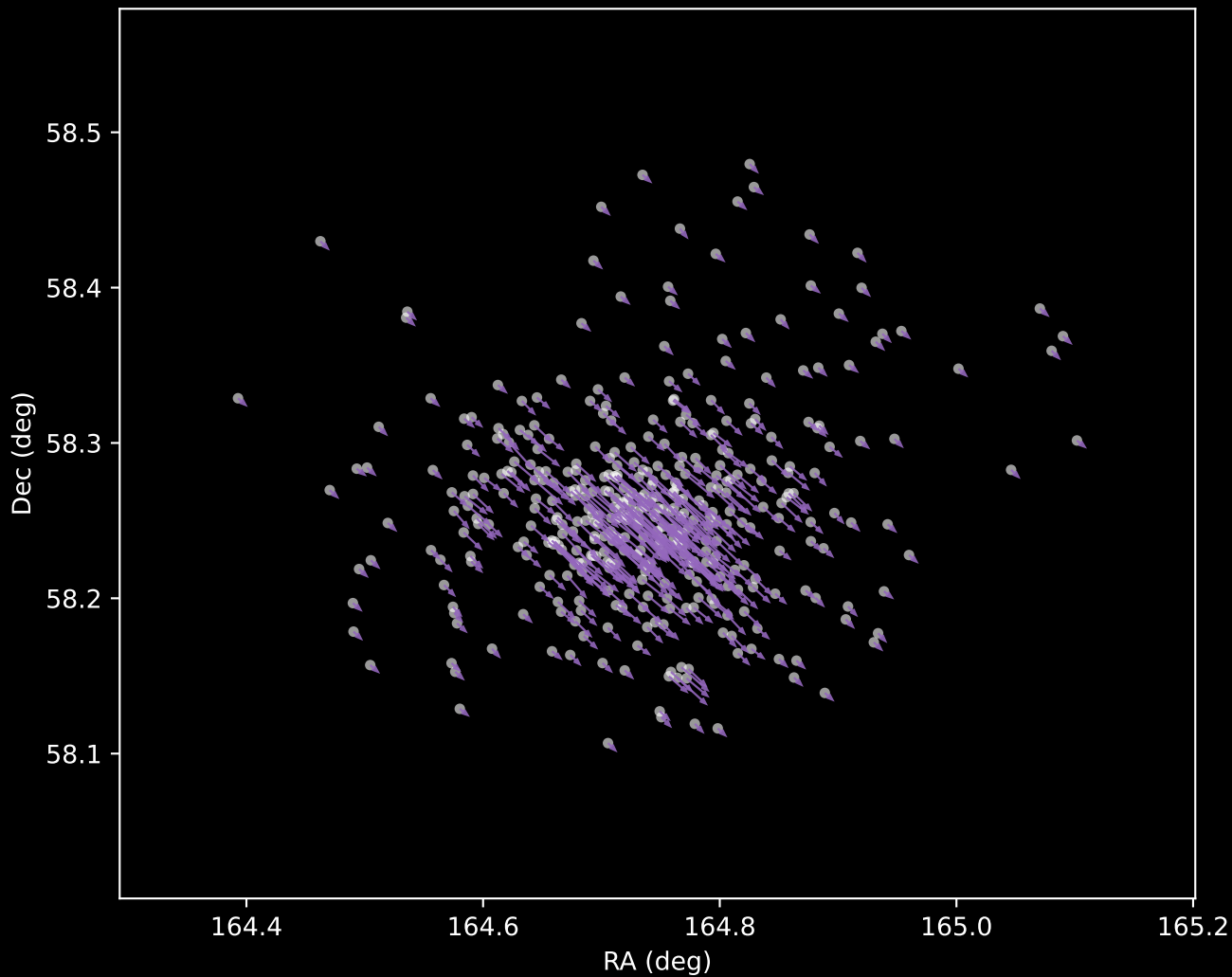
Gaia DR3 Cluster 8 Proper Motion Vectors (n=397)
