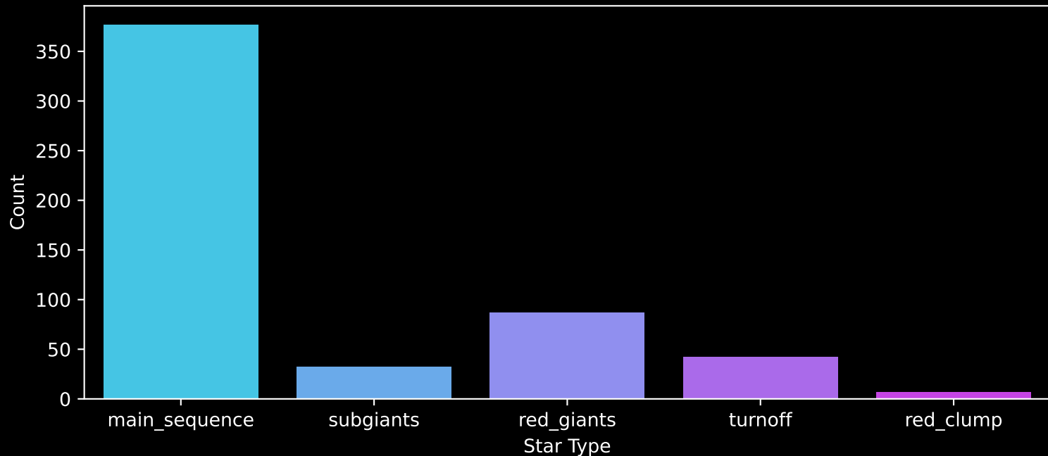
Gaia Cluster: [IC_361] Count plot of Star Type
