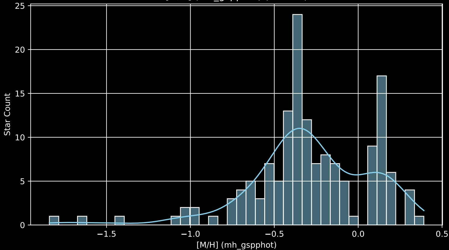
Gaia Cluster: [IC_4665 [M/H] (mh_gspphot) (n= 150)
