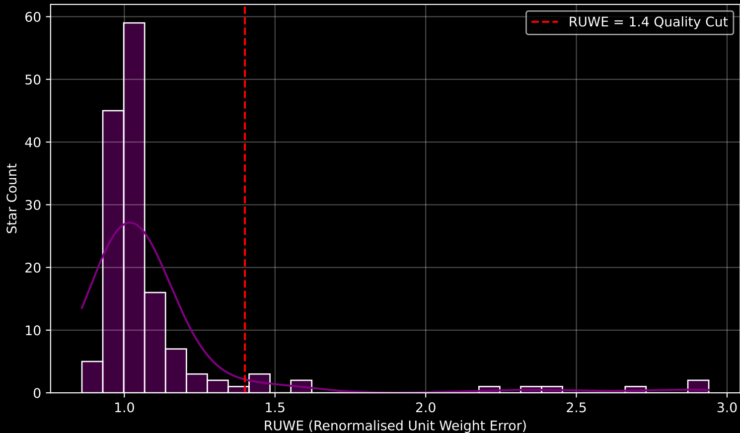
Gaia Cluster: [IC_4665] RUWE Distribution (n= 149)
