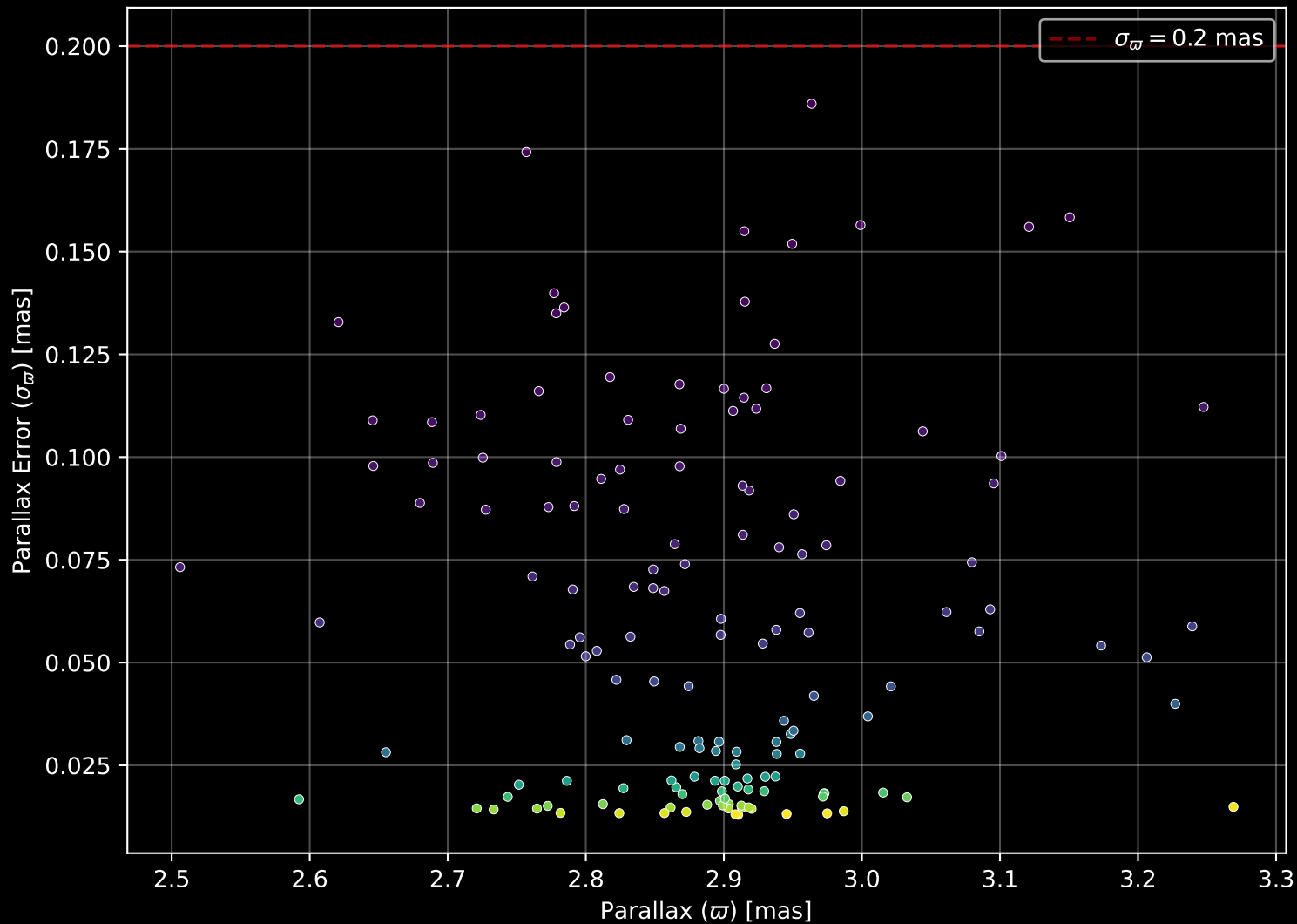
Gaia Cluster: [IC_4665] Parallax Quality (n= 150)
