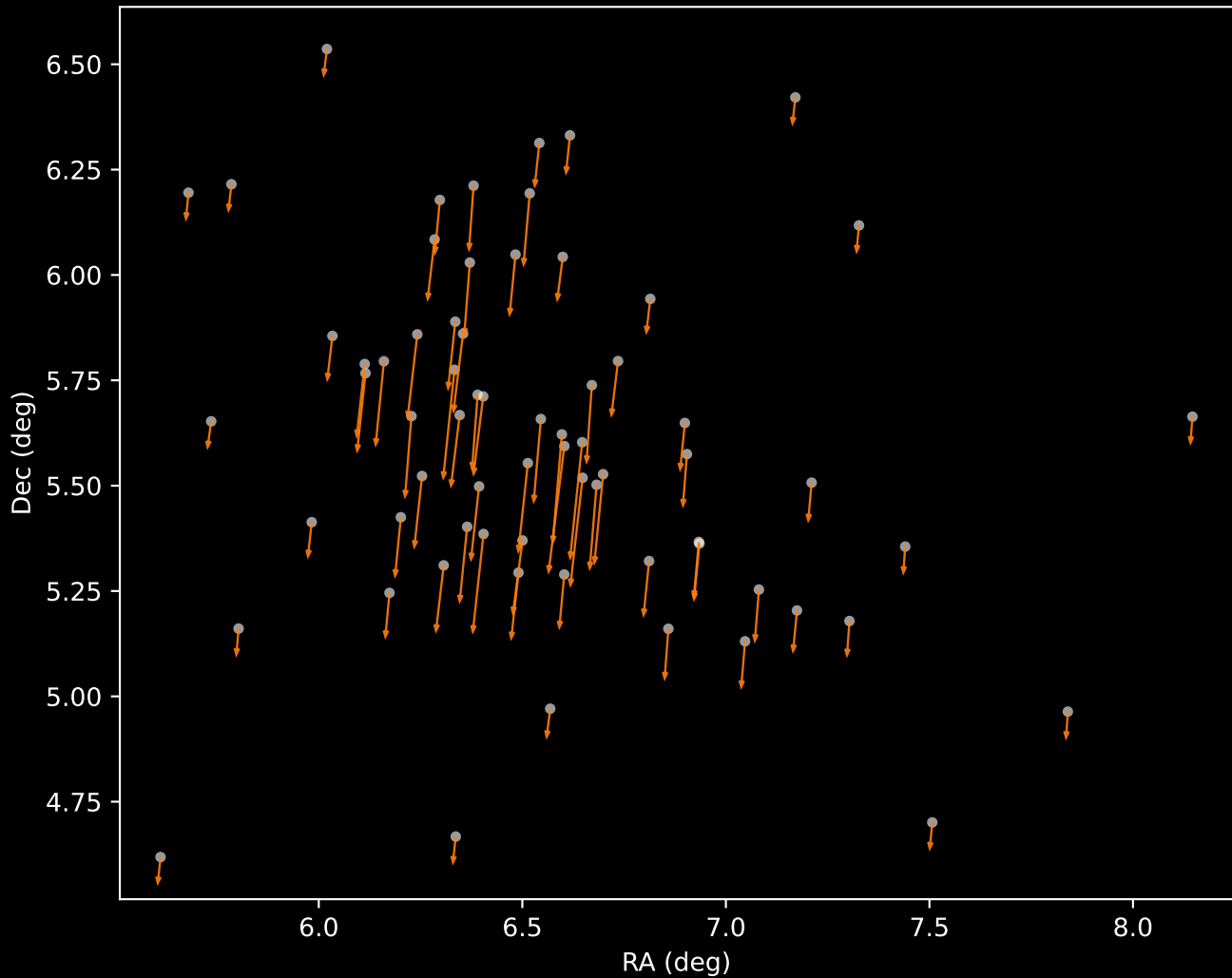
Gaia DR3 Cluster 2 Proper Motion Vectors (n=68)
