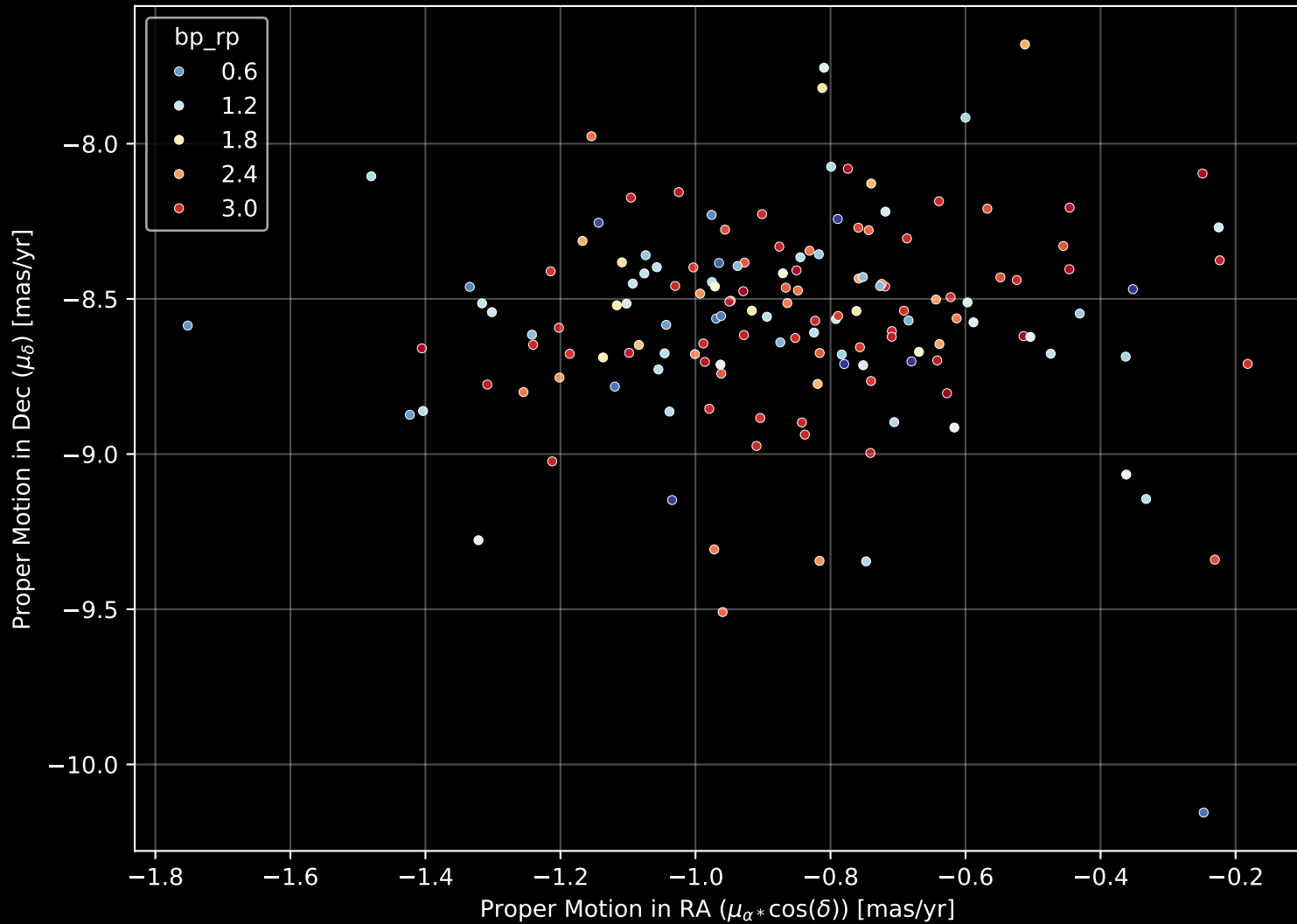
Gaia Cluster: [IC_4665] Proper Motion Diagram (n= 150)
