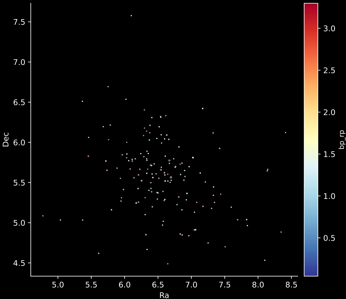
Gaia Cluster: [IC_4665] Stars: 150
