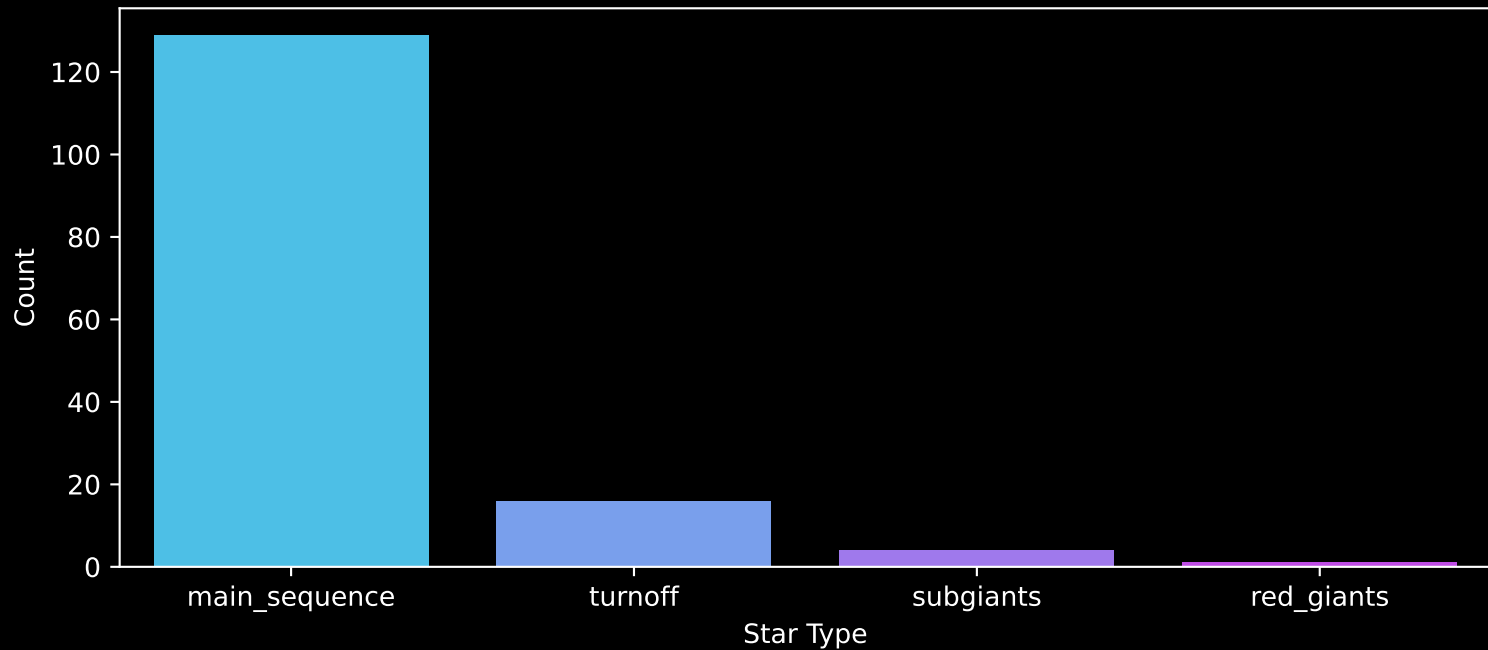
Gaia Cluster: [IC_4665] Count plot of Star Type
