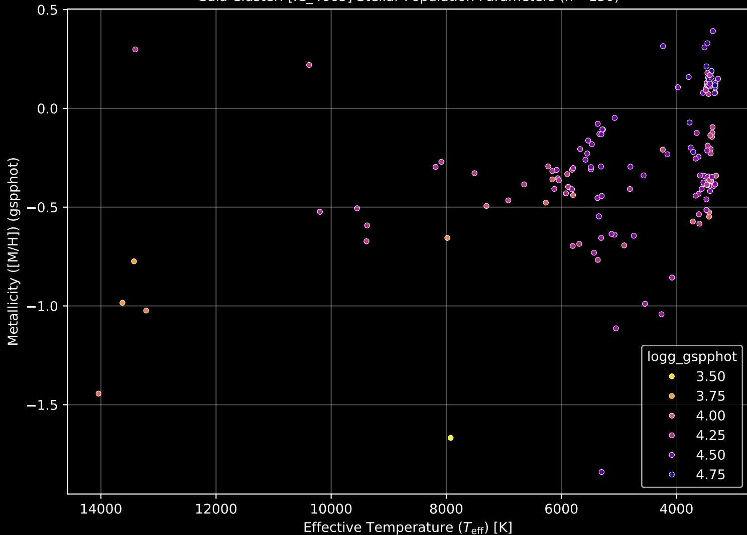
Gaia Cluster: [IC_4665] Stellar Population Parameters (n= 150)
