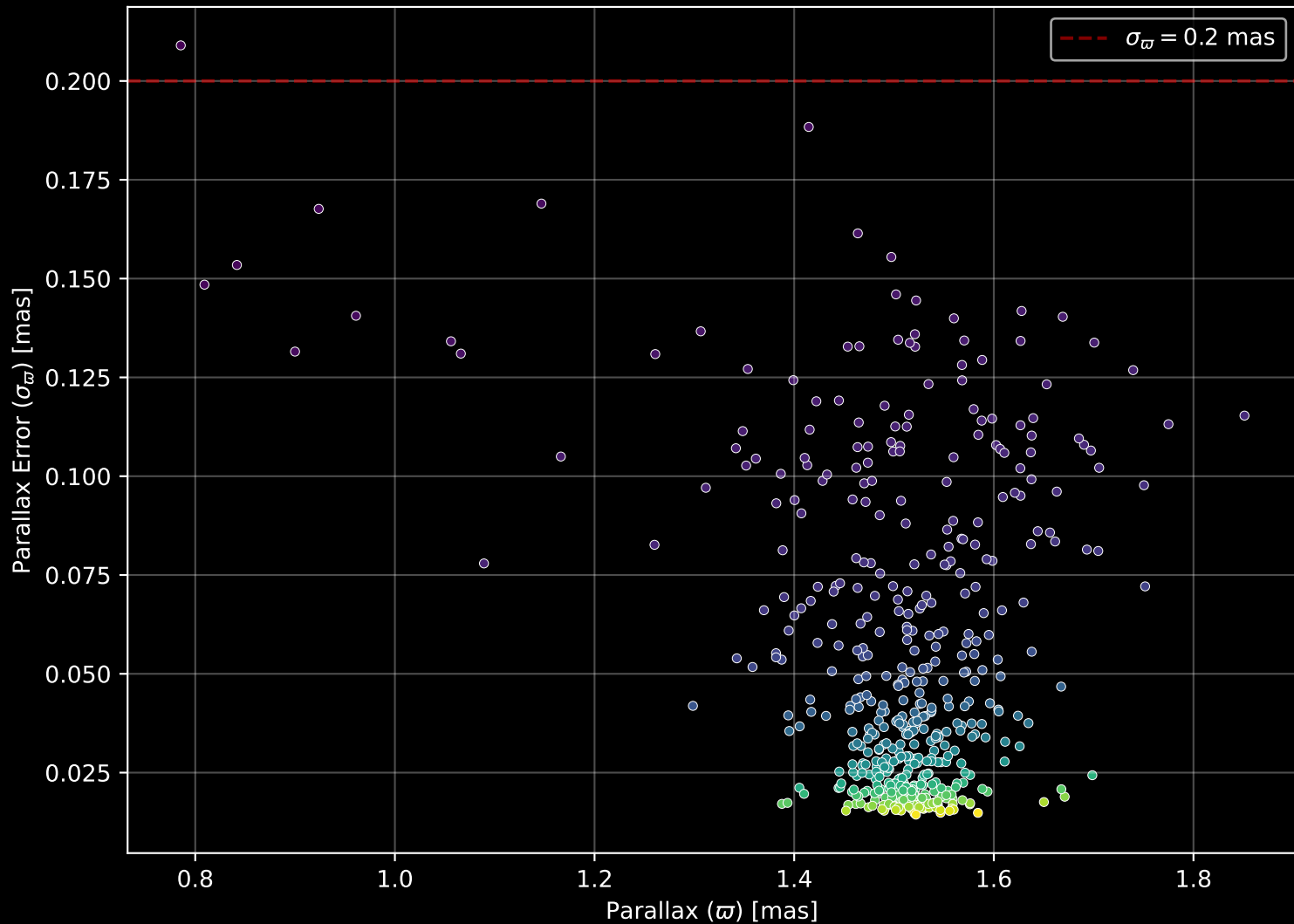
Gaia Cluster: [IC_4725] Parallax Quality (n= 497)
