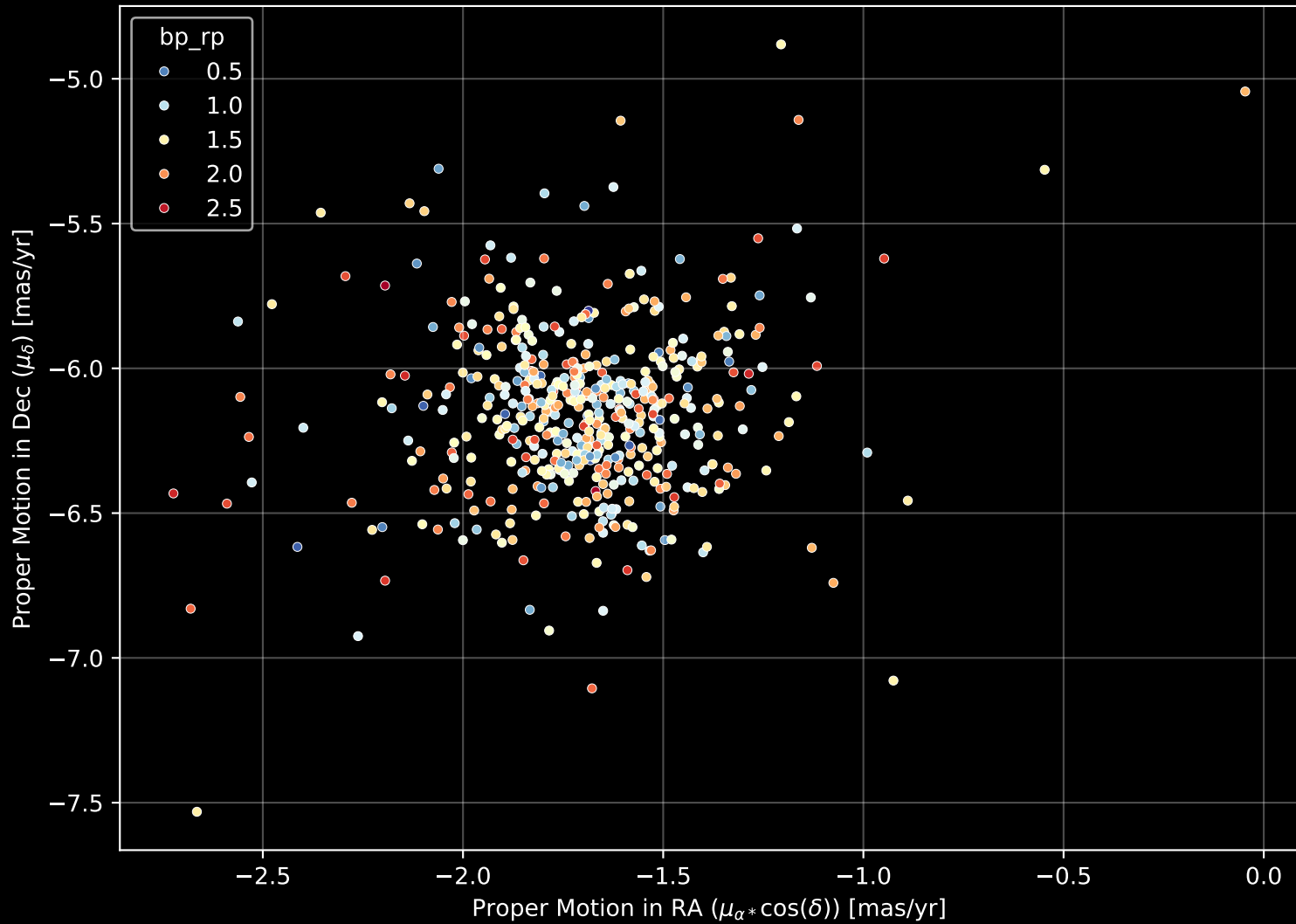
Gaia Cluster: [IC_4725] Proper Motion Diagram (n= 497)
