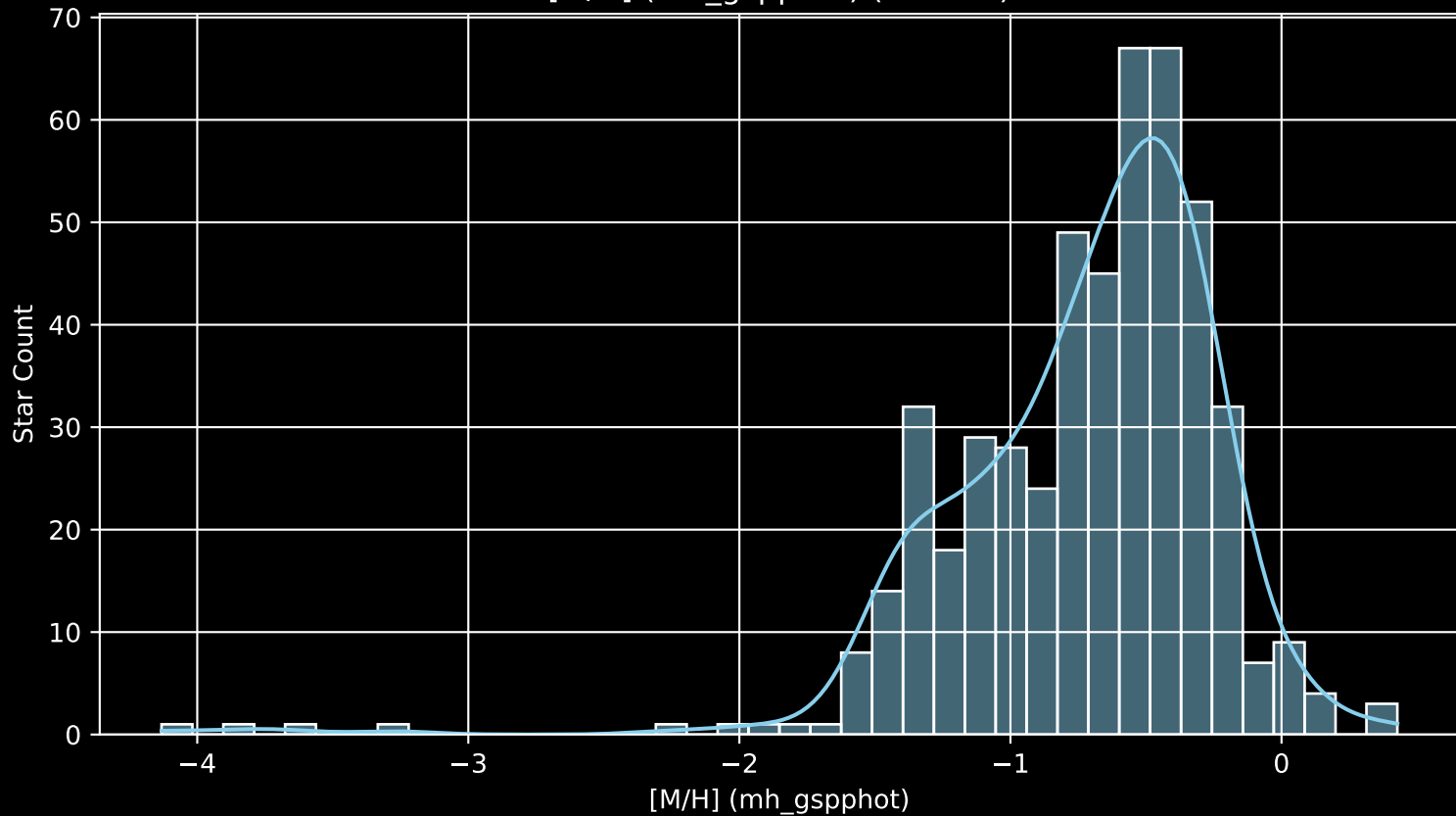
Gaia Cluster: [IC_4725 [M/H] (mh_gspphot) (n= 497)
