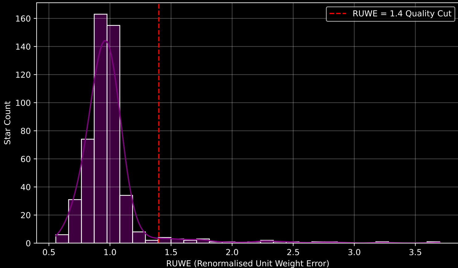
Gaia Cluster: [IC_4725] RUWE Distribution (n= 496)
