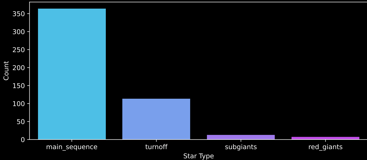
Gaia Cluster: [IC_4725] Count plot of Star Type
