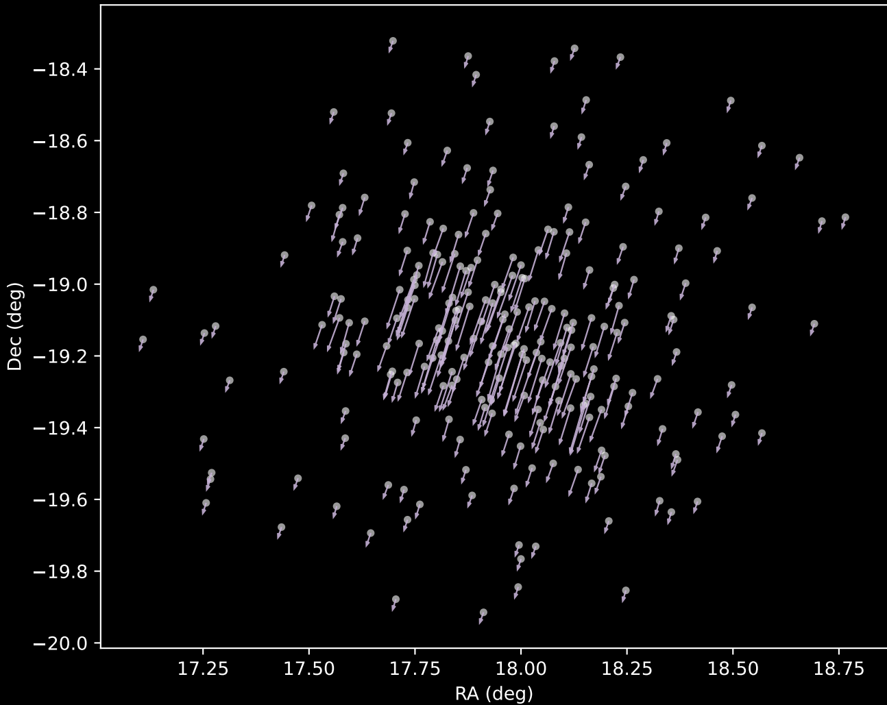
Gaia DR3 Cluster 9 Proper Motion Vectors (n=245)
