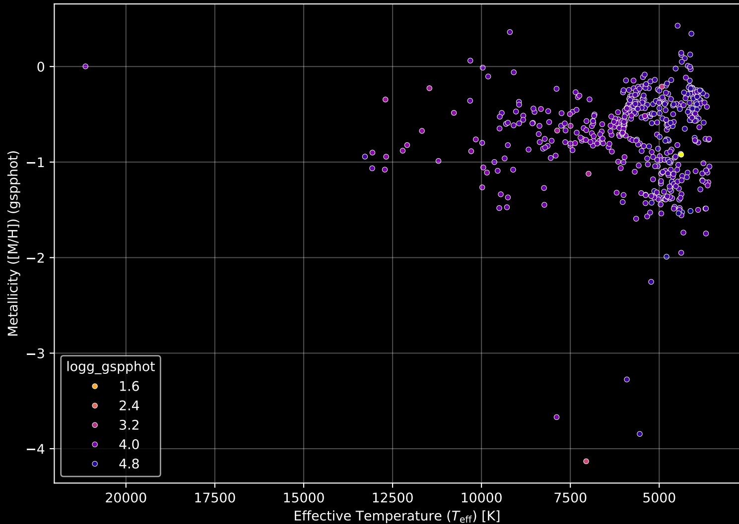
Gaia Cluster: [IC_4725] Stellar Population Parameters (n= 497)
