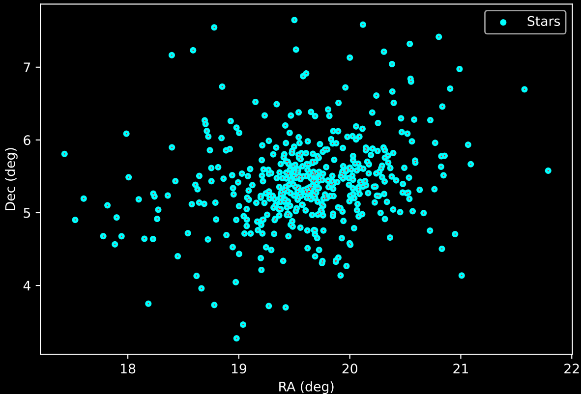
Gaia Cluster: [IC_4756] Proper Motion Vectors for Gaia Star Field (n= 471)
