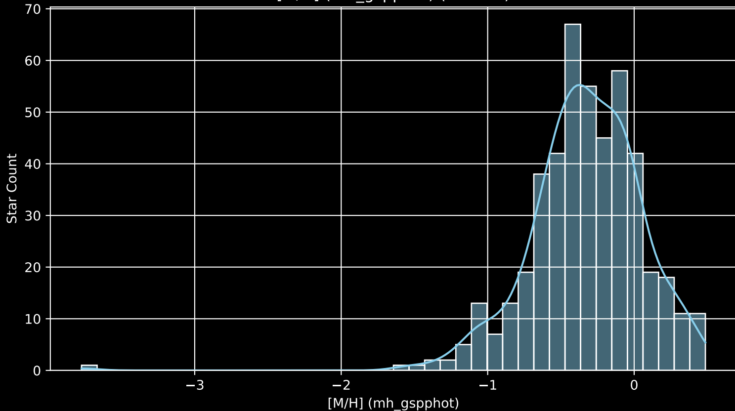
Gaia Cluster: [IC_4756 [M/H] (mh_gspphot) (n= 470)
