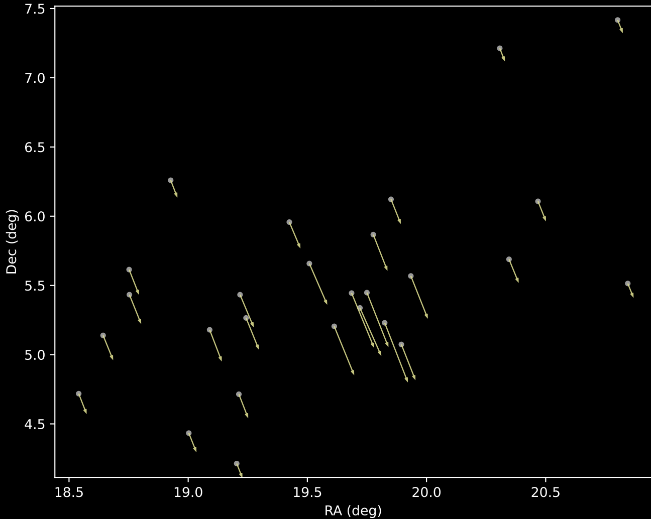
Gaia DR3 Cluster 17 Proper Motion Vectors (n=27)
