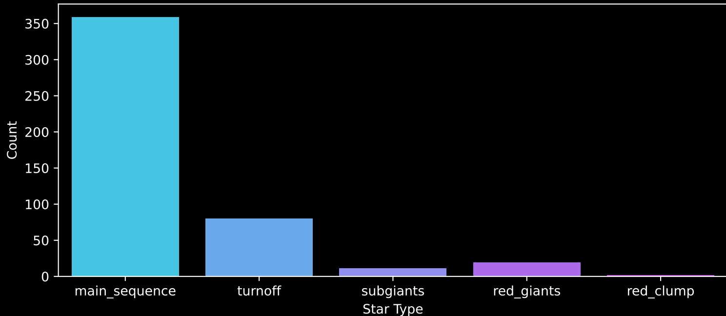
Gaia Cluster: [IC_4756] Count plot of Star Type
