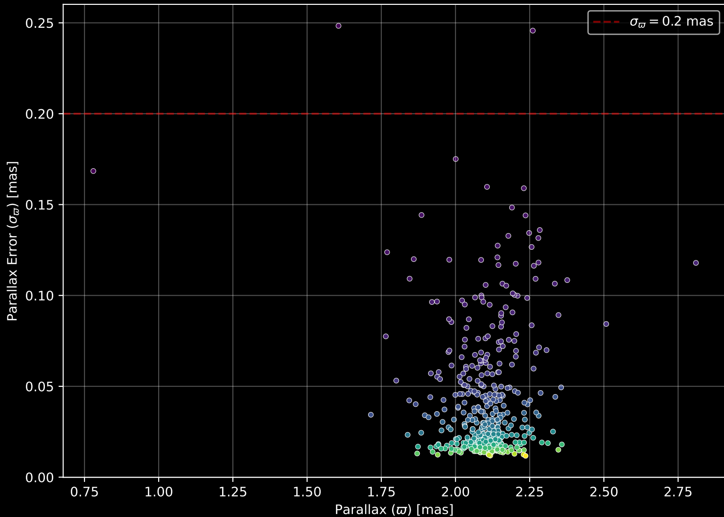
Gaia Cluster: [IC_4756] Parallax Quality (n= 471)
