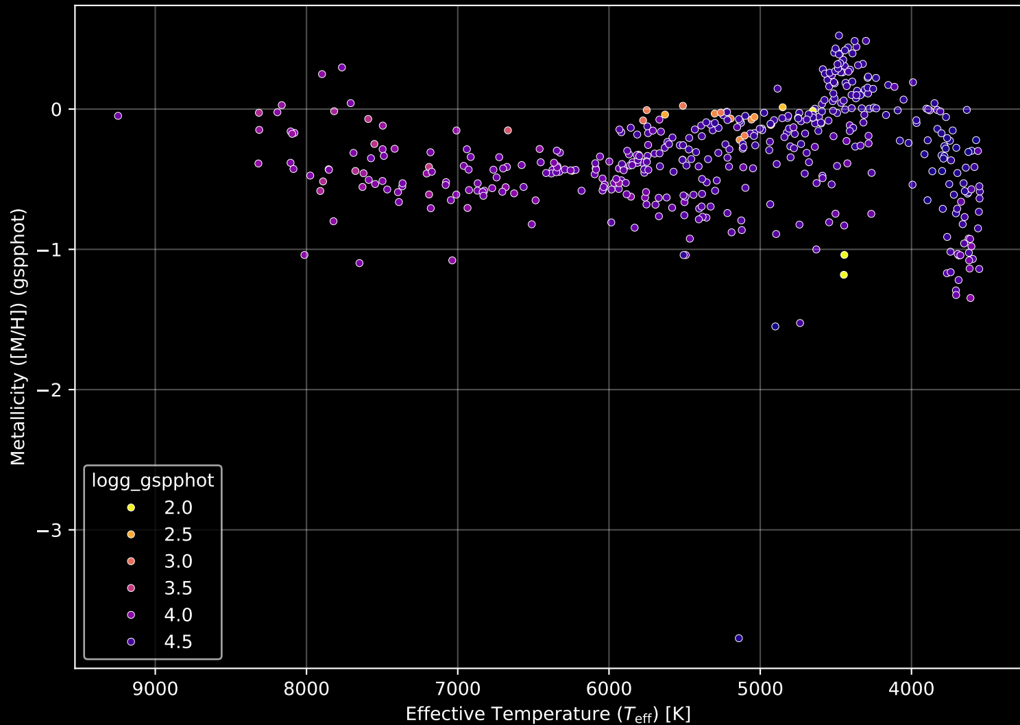
Gaia Cluster: [IC_4756] Stellar Population Parameters (n= 471)
