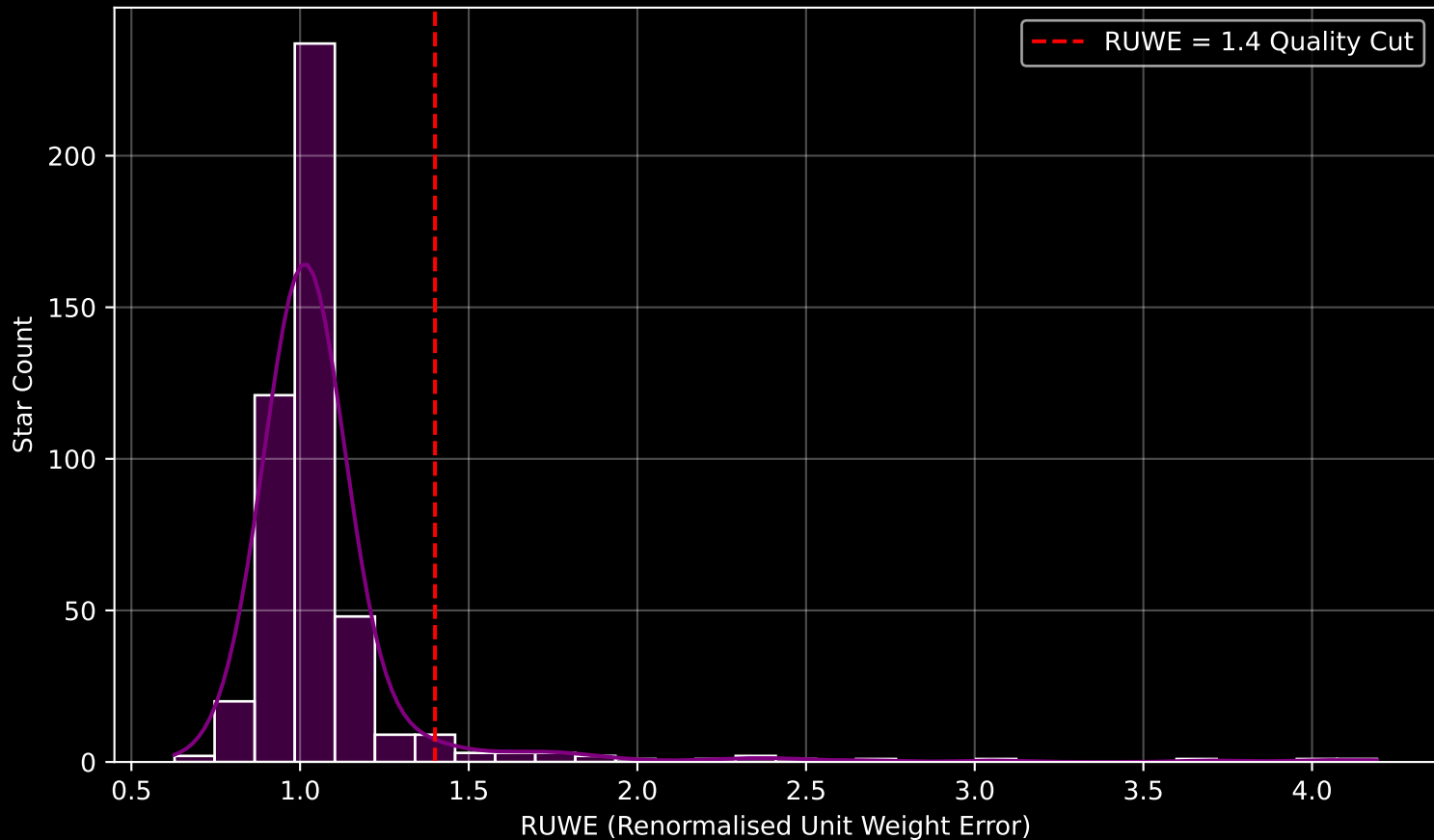
Gaia Cluster: [IC_4756] RUWE Distribution (n= 467)
