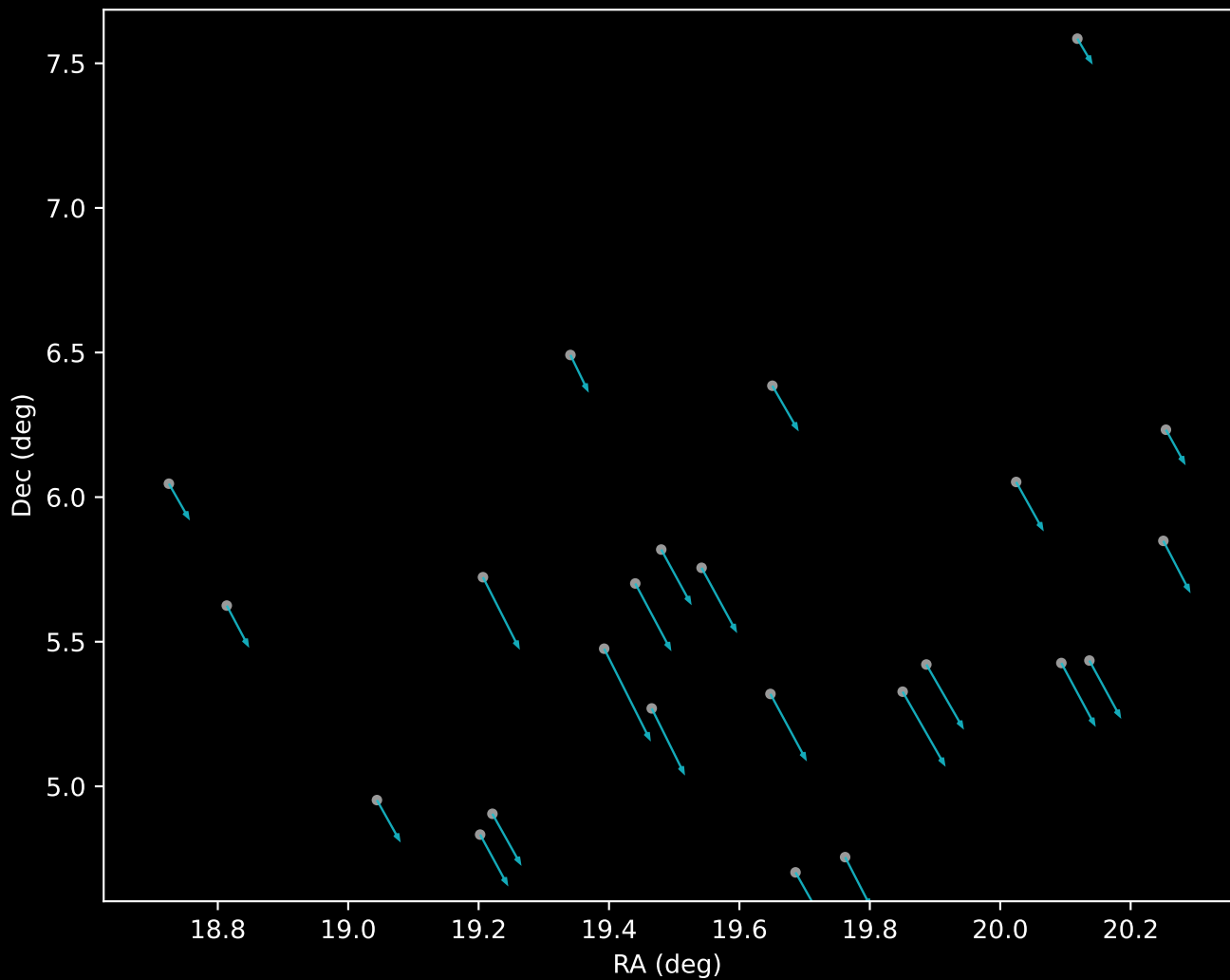
Gaia DR3 Cluster 18 Proper Motion Vectors (n=24)
