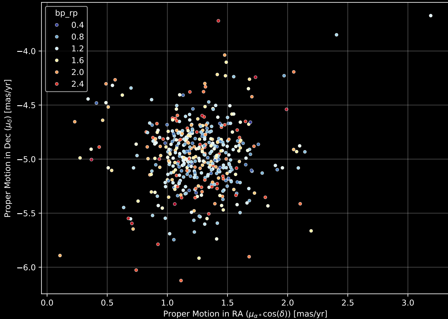
Gaia Cluster: [IC_4756] Proper Motion Diagram (n= 471)
