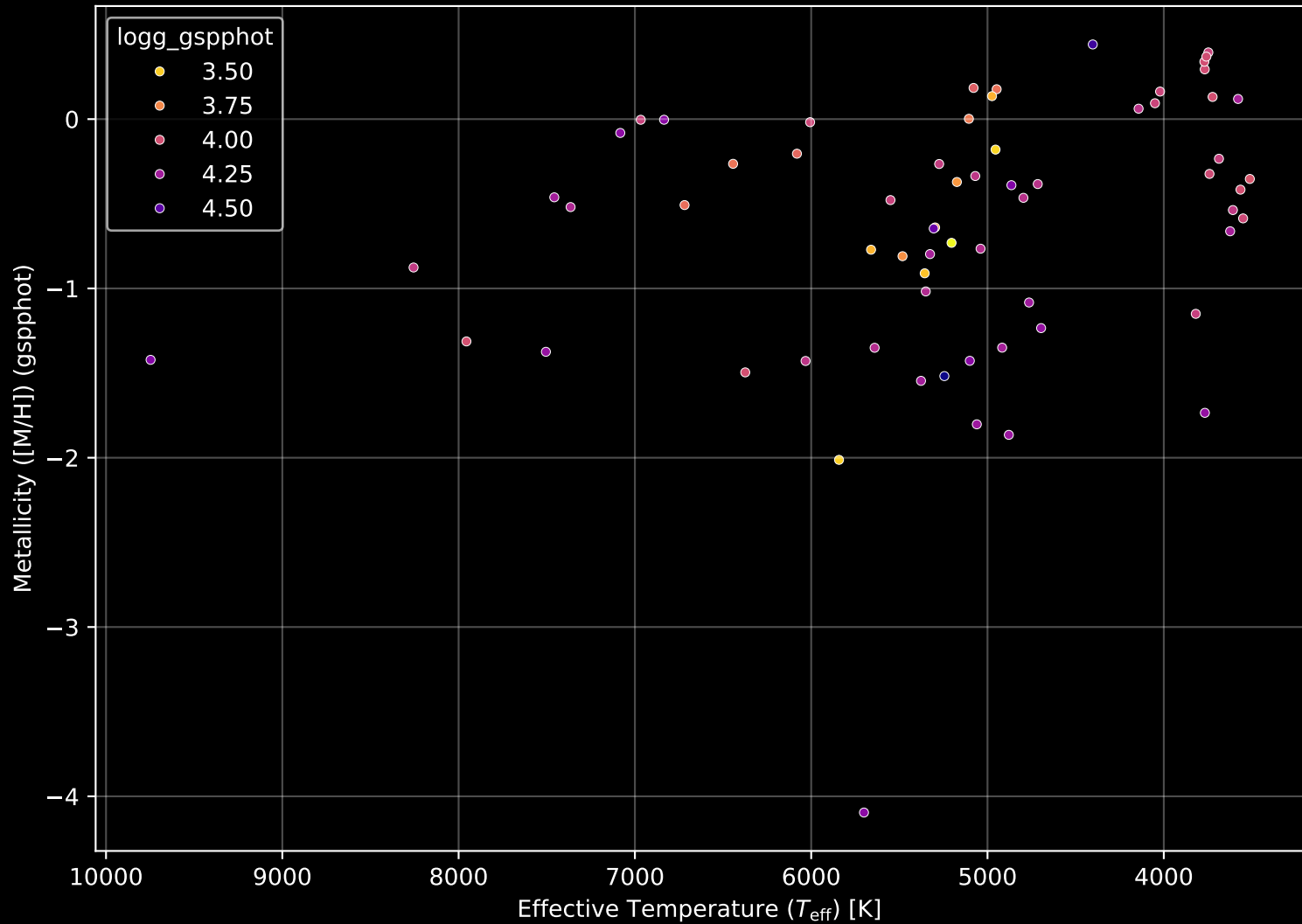
Gaia Cluster: [IC_5146] Stellar Population Parameters (n= 66)
