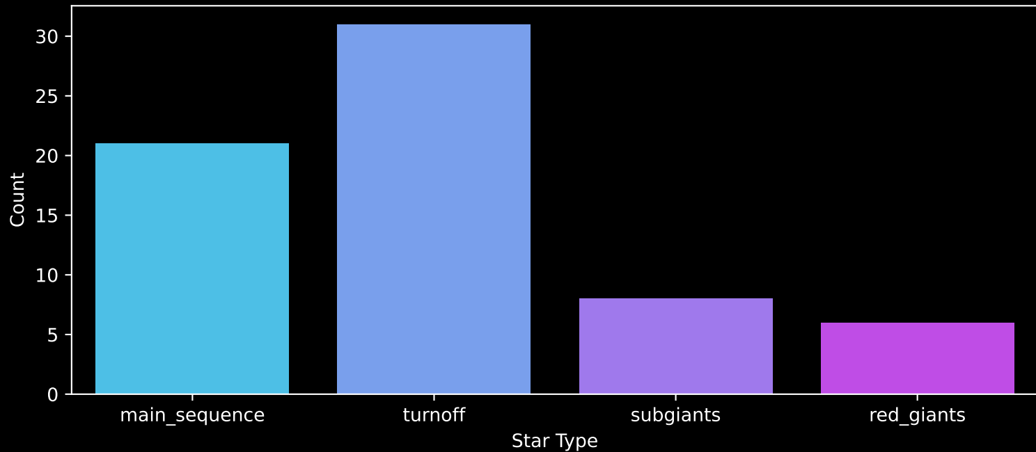
Gaia Cluster: [IC_5146] Count plot of Star Type
