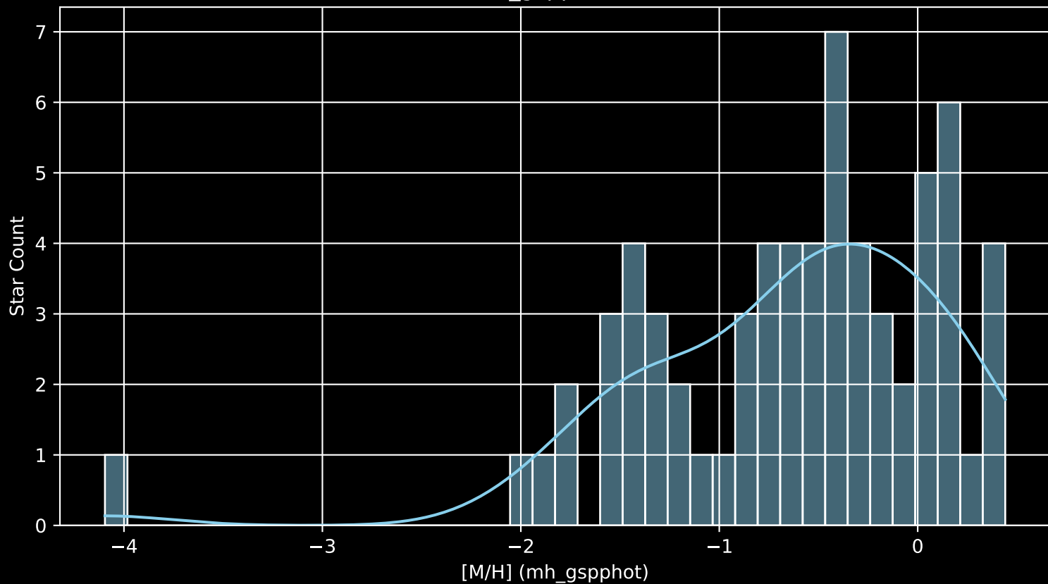
Gaia Cluster: [IC_5146 [M/H] (mh_gspphot) (n= 66)
