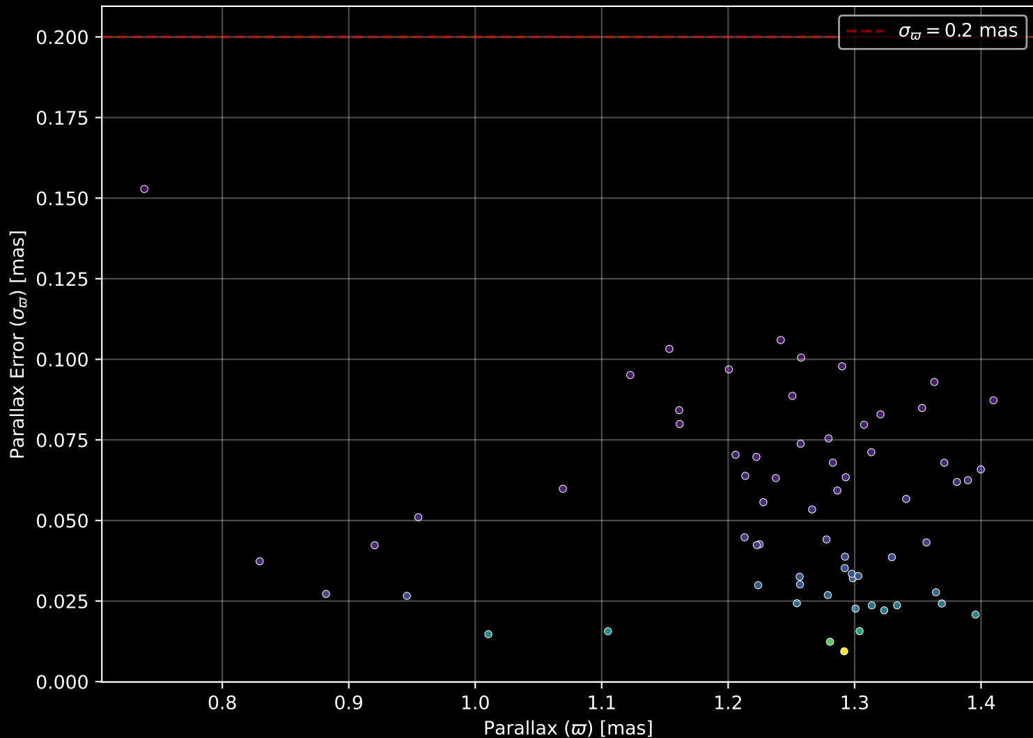
Gaia Cluster: [IC_5146] Parallax Quality (n= 66)
