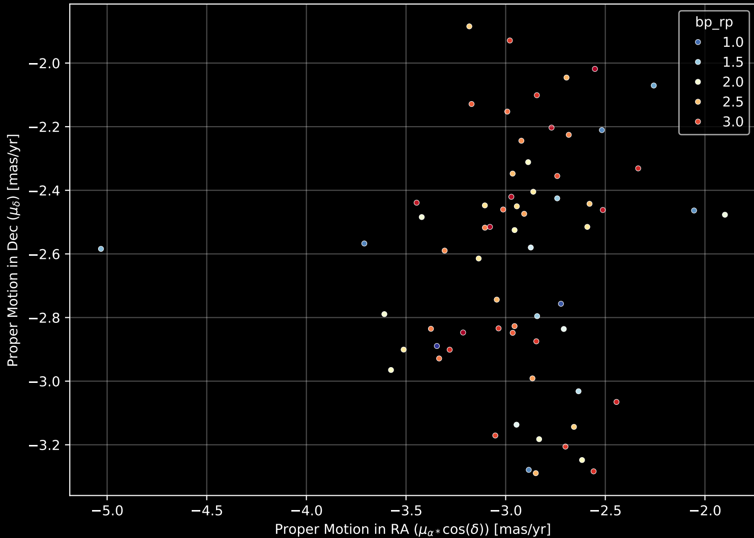
Gaia Cluster: [IC_5146] Proper Motion Diagram (n= 66)
