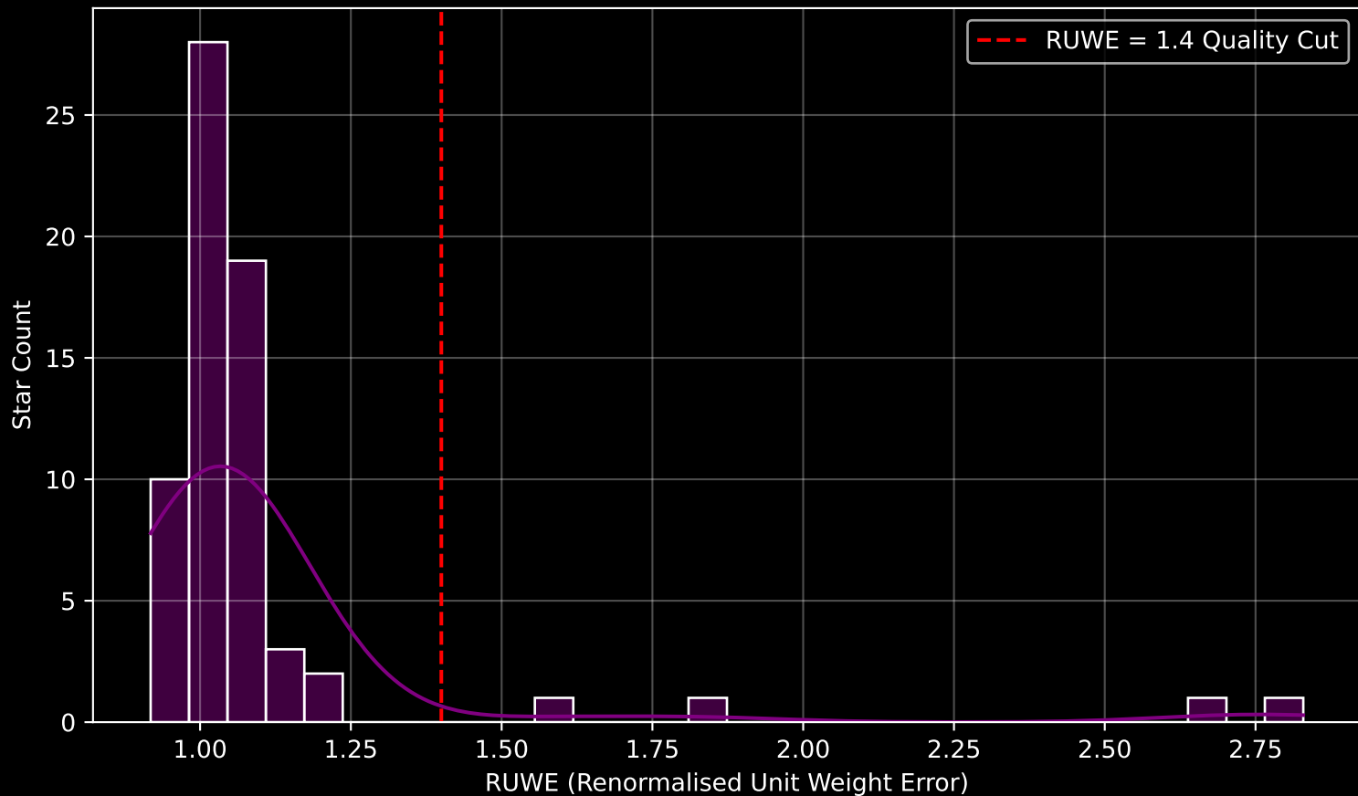
Gaia Cluster: [IC_5146] RUWE Distribution (n= 66)
