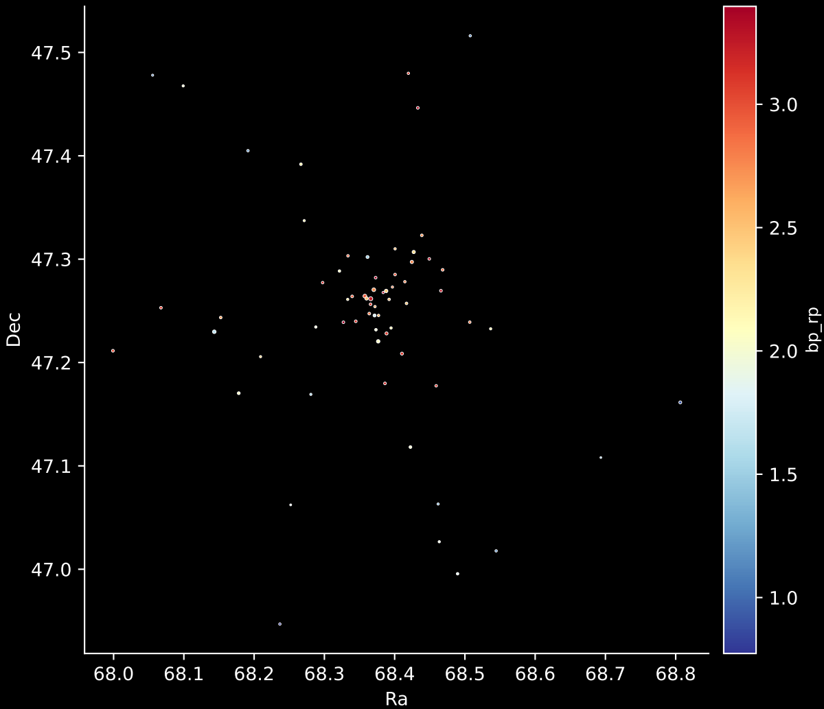
Gaia Cluster: [IC_5146] Stars: 66
