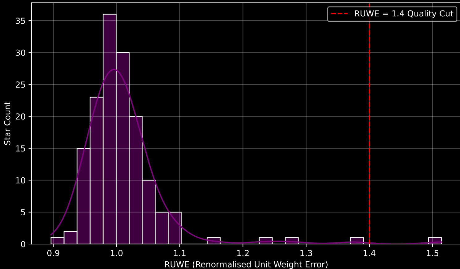
Gaia Cluster: [Juchert_10] RUWE Distribution (n= 152)
