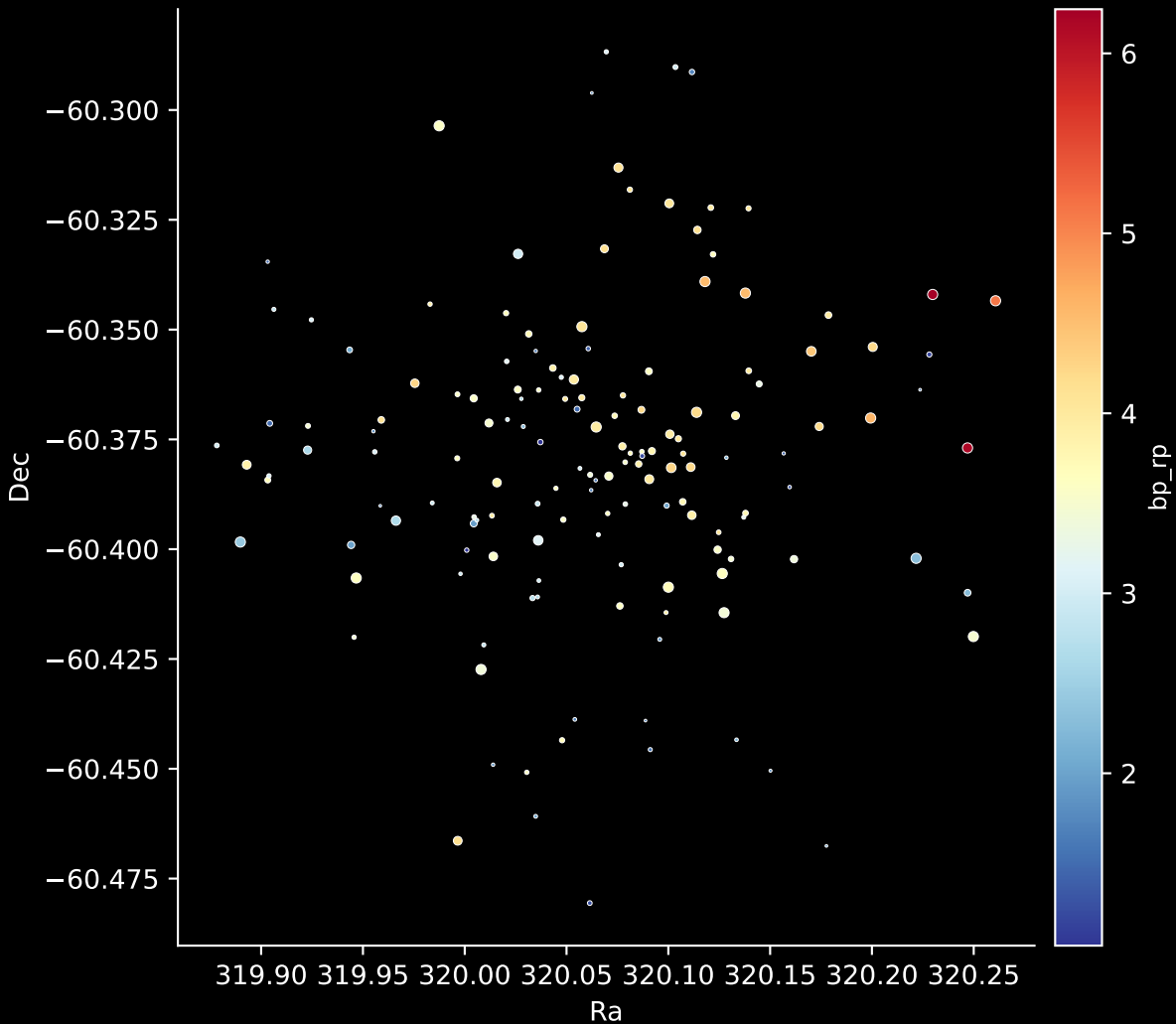
Gaia Cluster: [Juchert_10] Stars: 152
