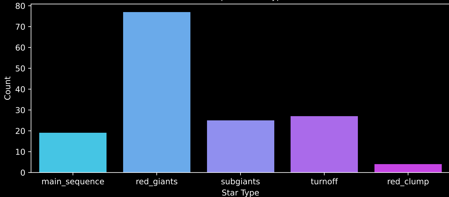
Gaia Cluster: [Juchert_10] Count plot of Star Type
