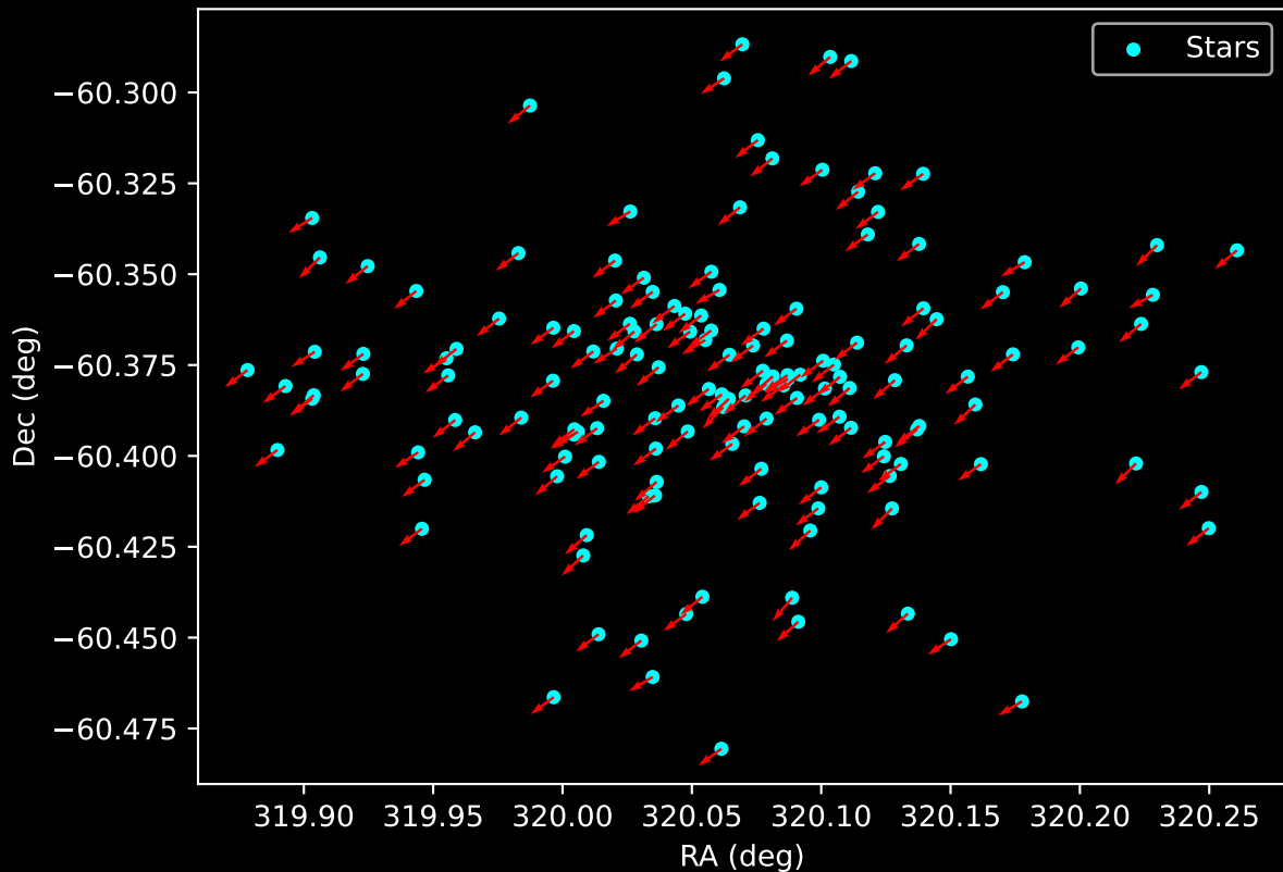
Gaia Cluster: [Juchert_10] Proper Motion Vectors for Gaia Star Field (n= 152)
