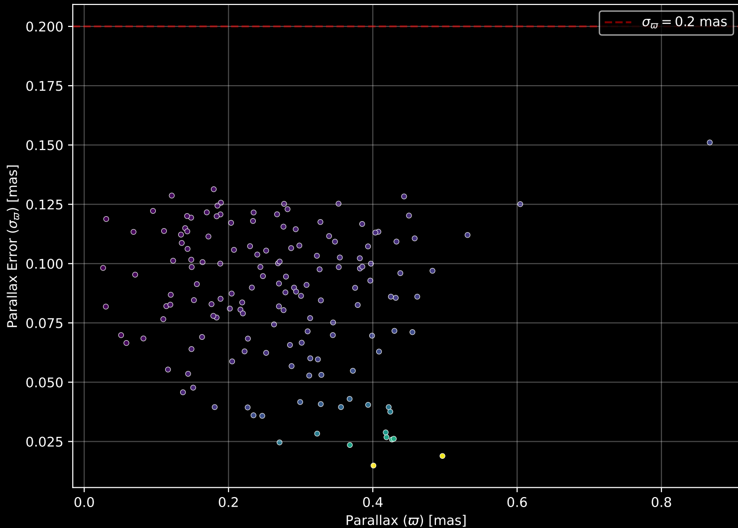
Gaia Cluster: [Juchert_10] Parallax Quality (n= 152)
