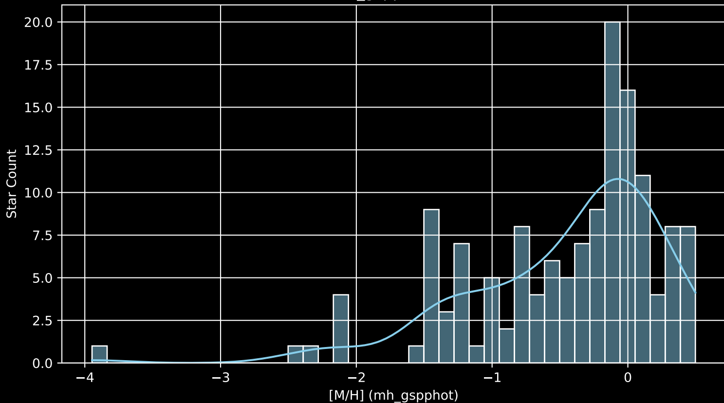
Gaia Cluster: [Juchert_10 [M/H] (mh_gspphot) (n= 141)
