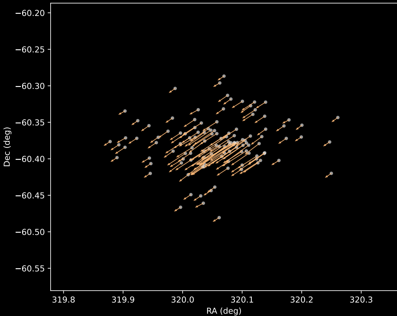
Gaia DR3 Cluster 3 Proper Motion Vectors (n=119)
