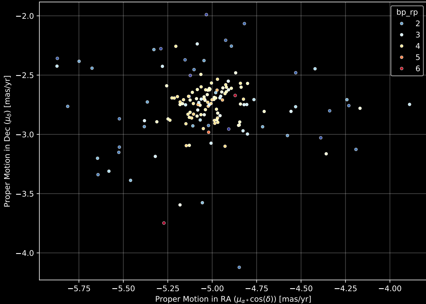
Gaia Cluster: [Juchert_10] Proper Motion Diagram (n= 152)
