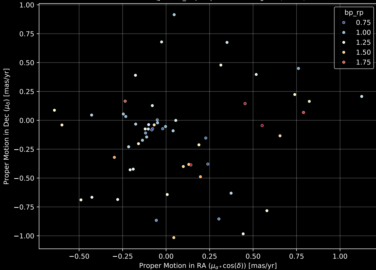
Gaia Cluster: [Juchert_18] Proper Motion Diagram (n= 59)
