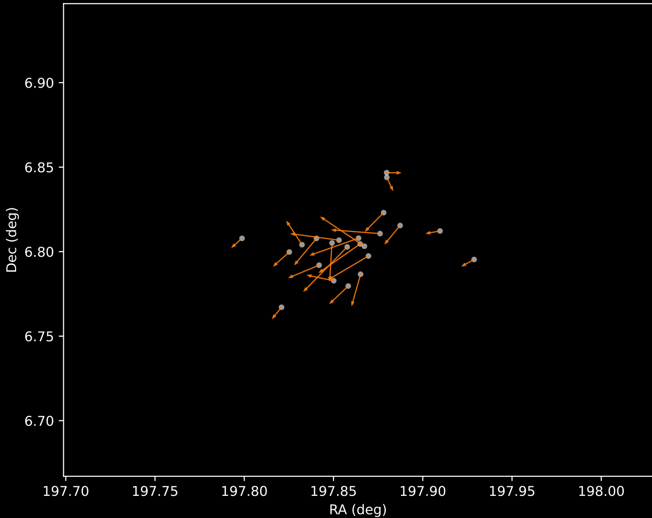
Gaia DR3 Cluster 2 Proper Motion Vectors (n=23)
