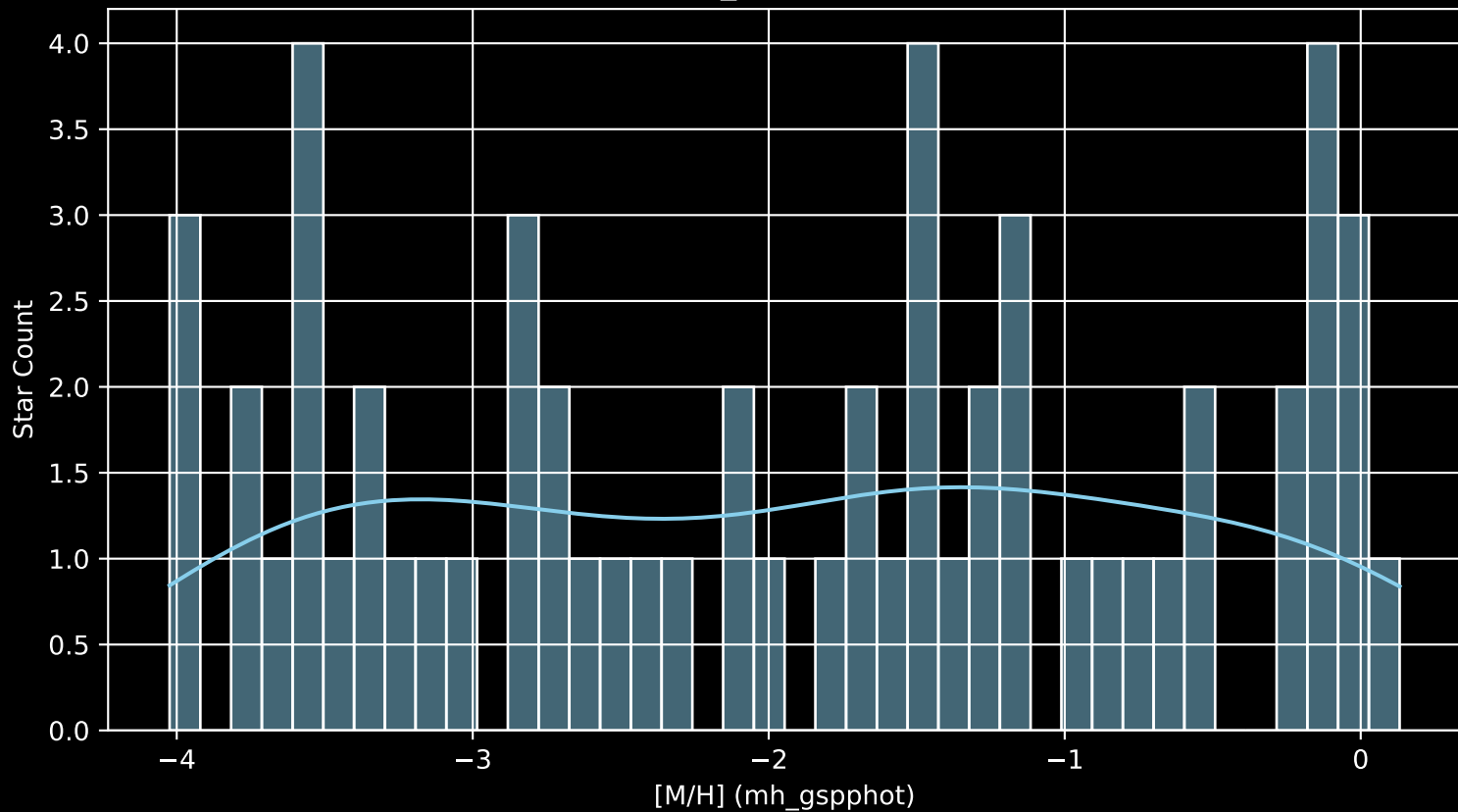
Gaia Cluster: [Juchert_18 [M/H] (mh_gspphot) (n= 58)
