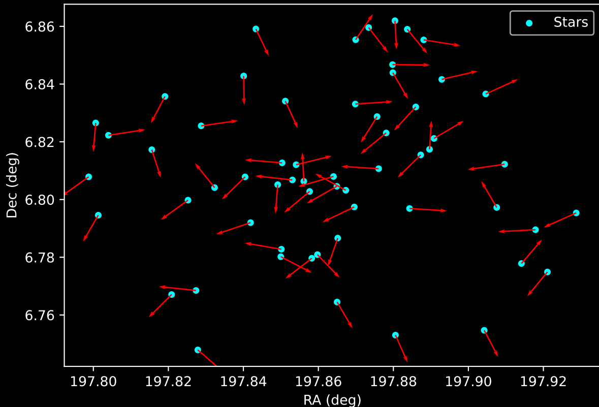
Gaia Cluster: [Juchert_18] Proper Motion Vectors for Gaia Star Field (n= 59)
