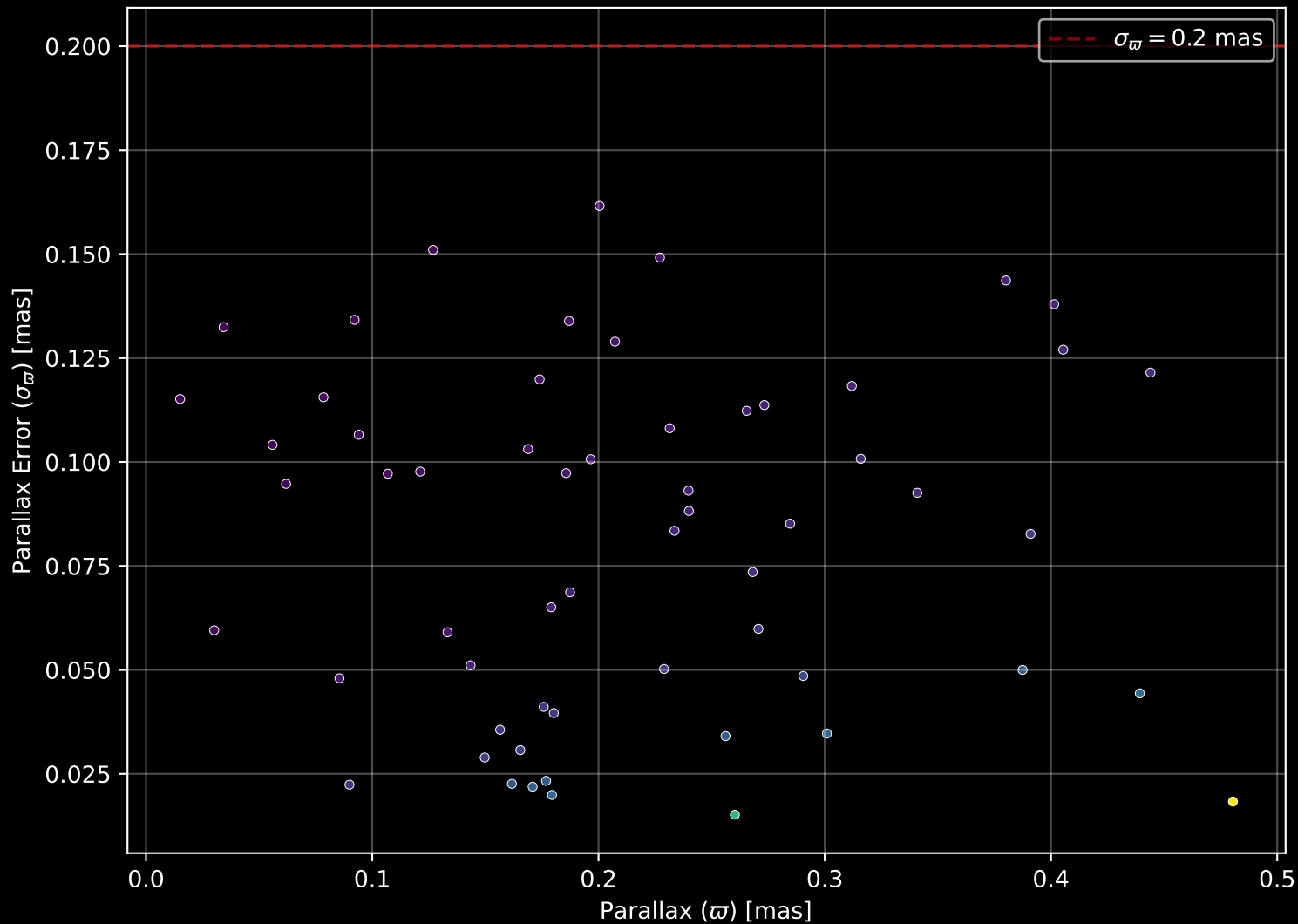
Gaia Cluster: [Juchert_18] Parallax Quality (n= 59)
