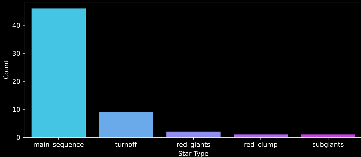
Gaia Cluster: [Juchert_18] Count plot of Star Type
