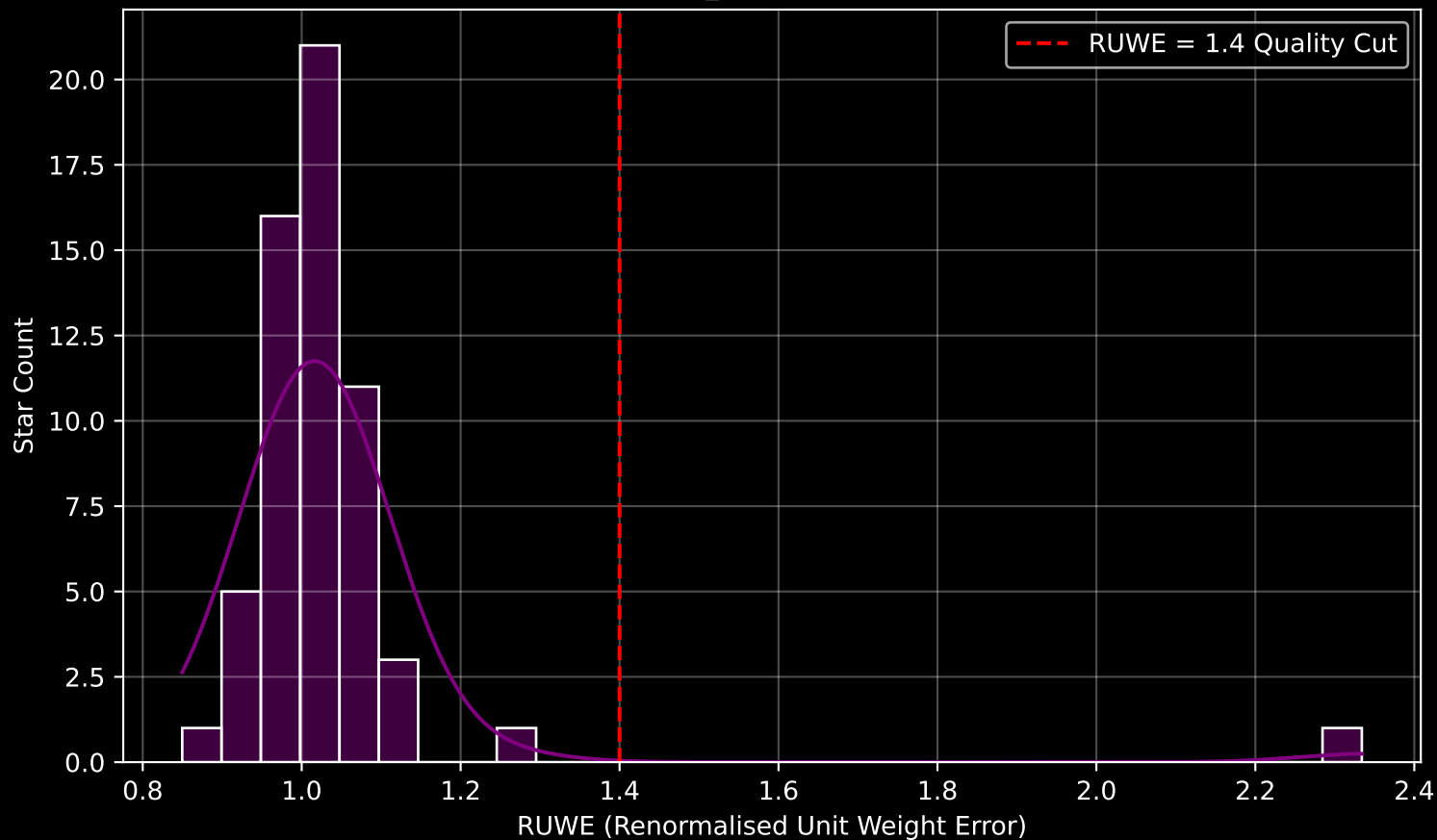
Gaia Cluster: [Juchert_18] RUWE Distribution (n= 59)
