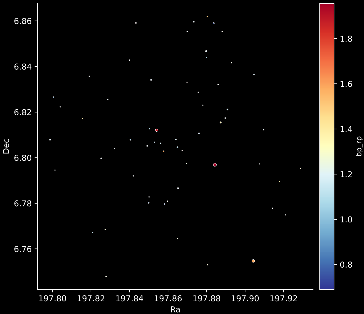
Gaia Cluster: [Juchert_18] Stars: 59
