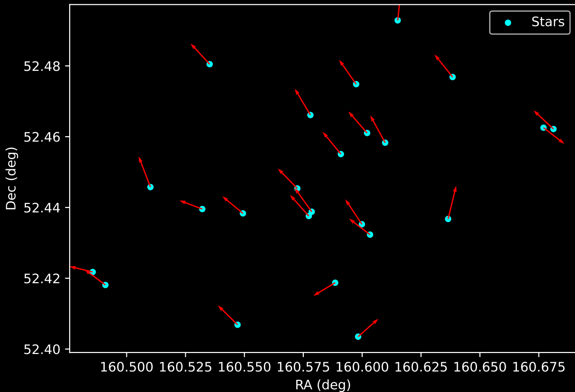
Gaia Cluster: [Juchert_19] Proper Motion Vectors for Gaia Star Field (n= 24)
