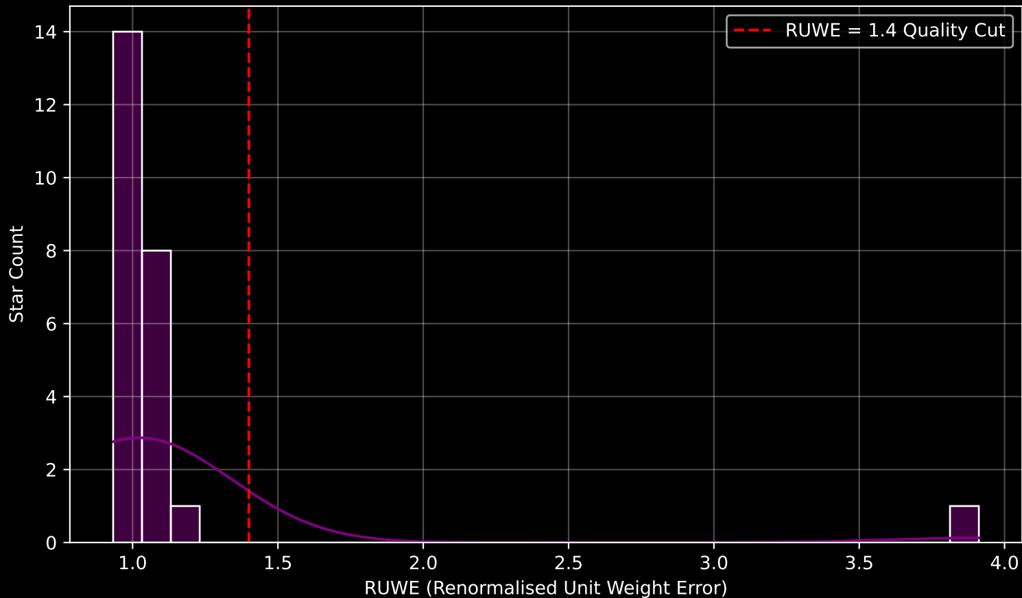
Gaia Cluster: [Juchert_19] RUWE Distribution (n= 24)
