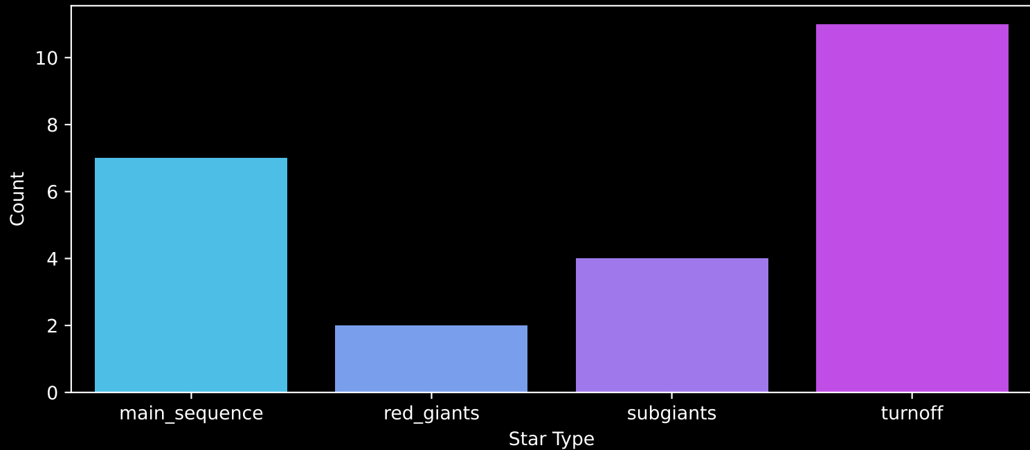
Gaia Cluster: [Juchert_19] Count plot of Star Type
