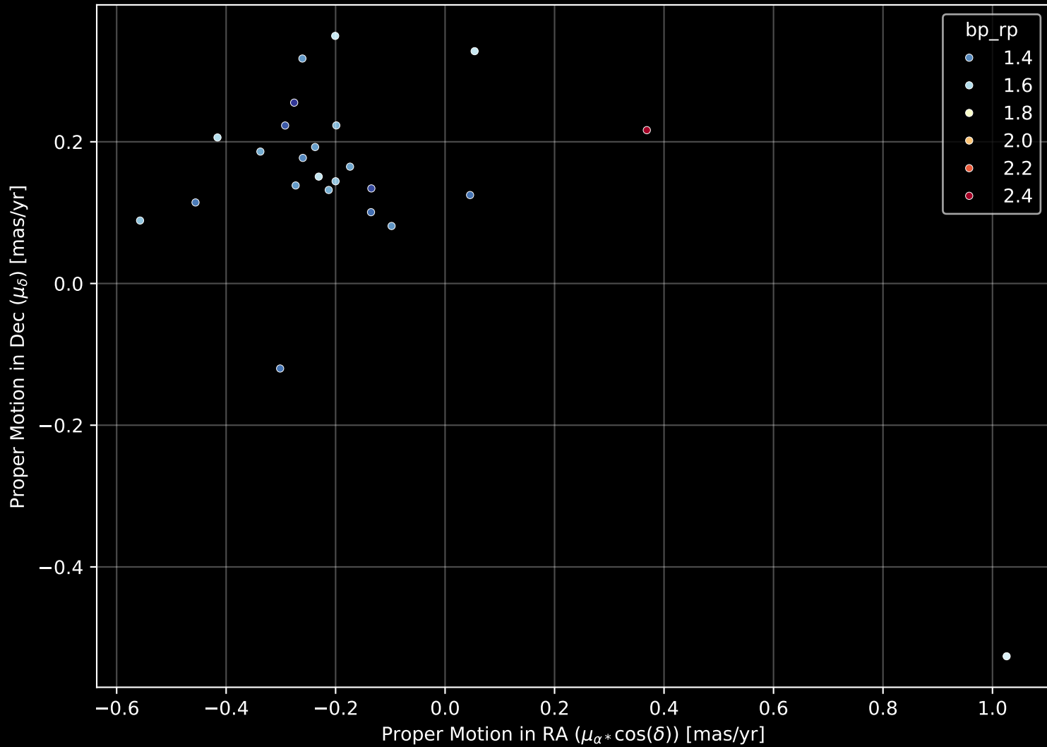
Gaia Cluster: [Juchert_19] Proper Motion Diagram (n= 24)
