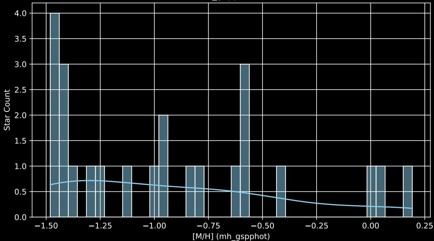
Gaia Cluster: [Juchert_19 [M/H] (mh_gspphot) (n= 24)
