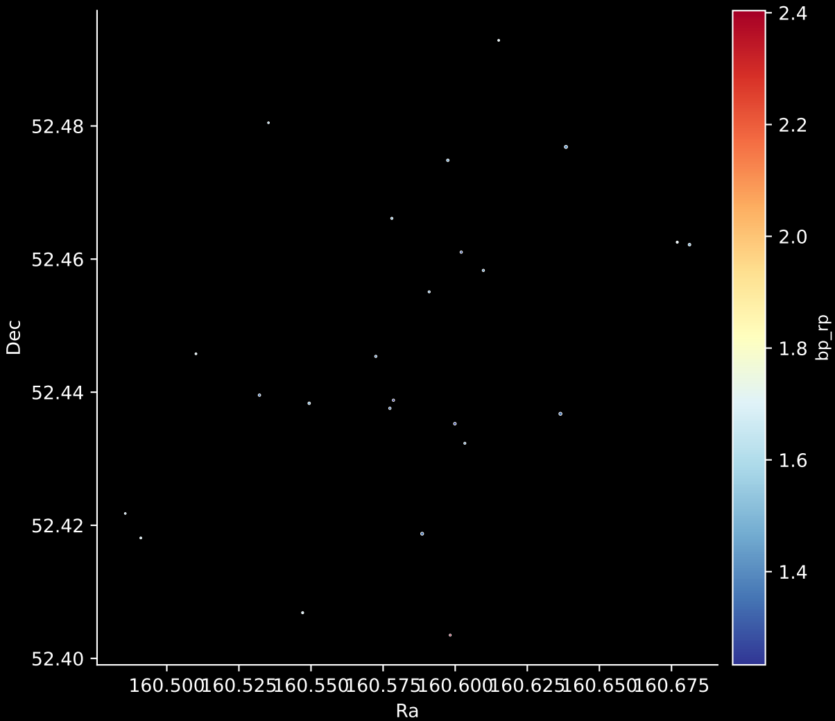
Gaia Cluster: [Juchert_19] Stars: 24
