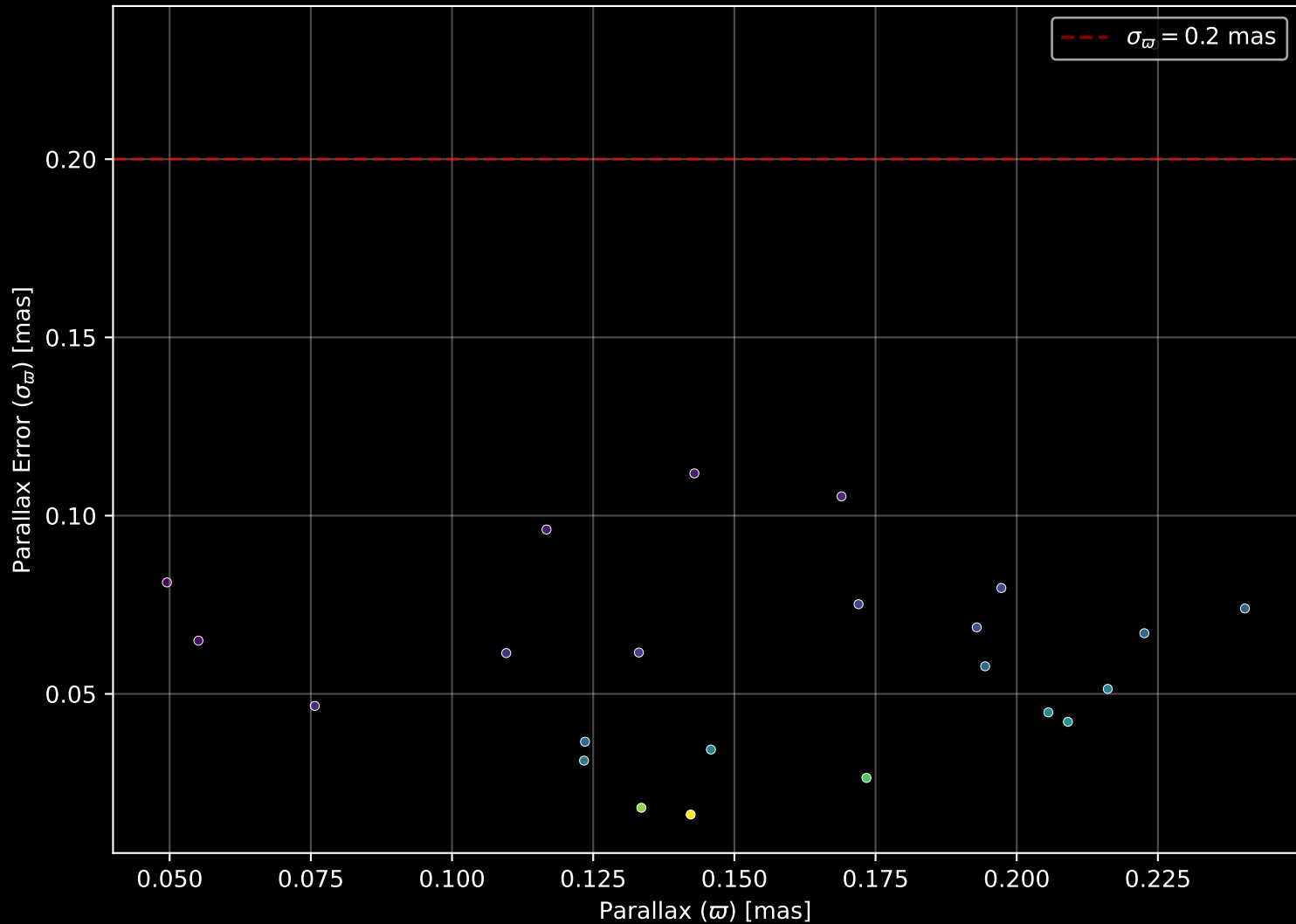
Gaia Cluster: [Juchert_19] Parallax Quality (n= 24)
