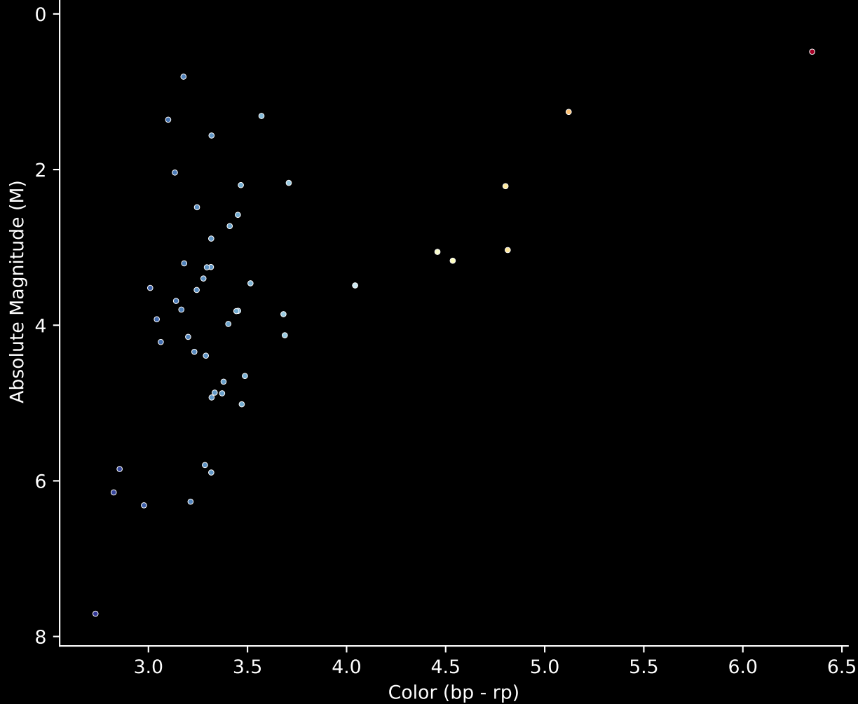
Gaia Cluster: [Juchert_3] Stars (n=51) Hertzsprung-Russel Diagram
