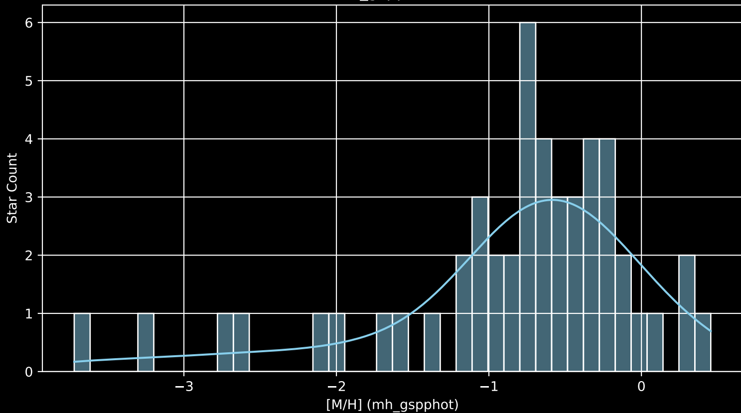
Gaia Cluster: [Juchert_3 [M/H] (mh_gspphot) (n= 49)
