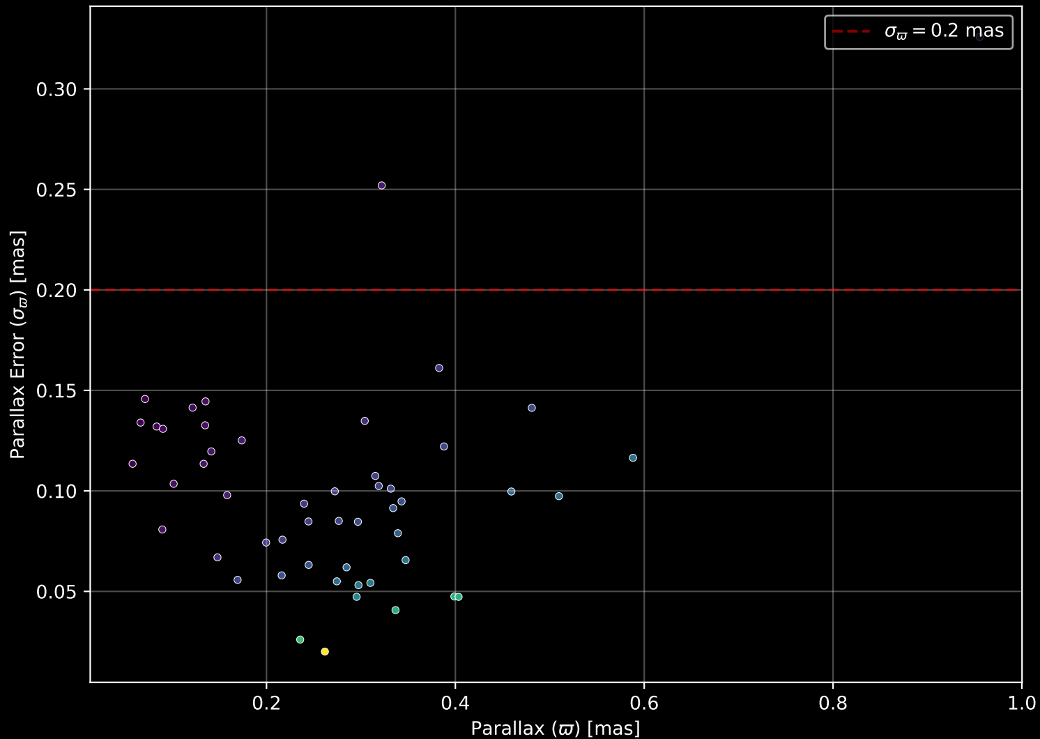
Gaia Cluster: [Juchert_3] Parallax Quality (n= 51)
