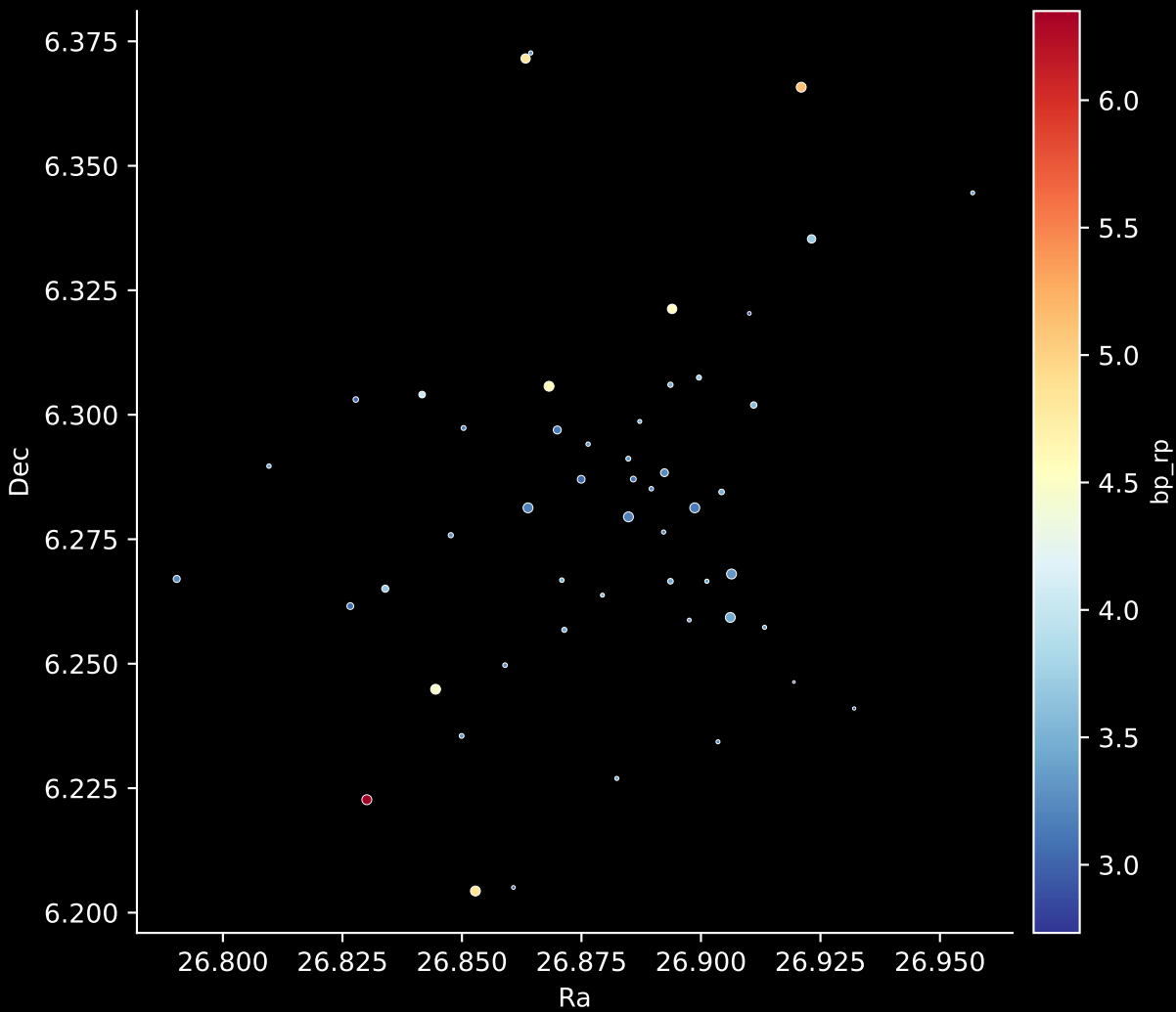
Gaia Cluster: [Juchert_3] Stars: 51
