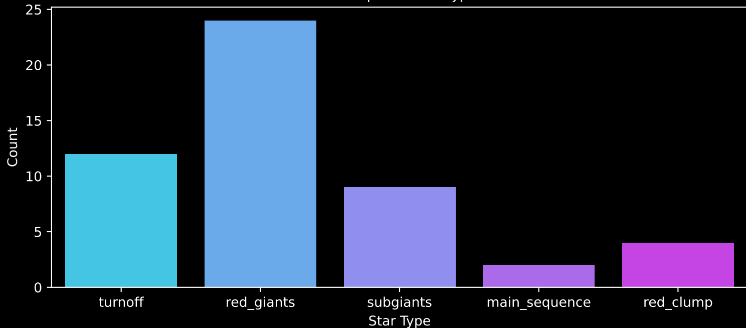
Gaia Cluster: [Juchert_3] Count plot of Star Type
