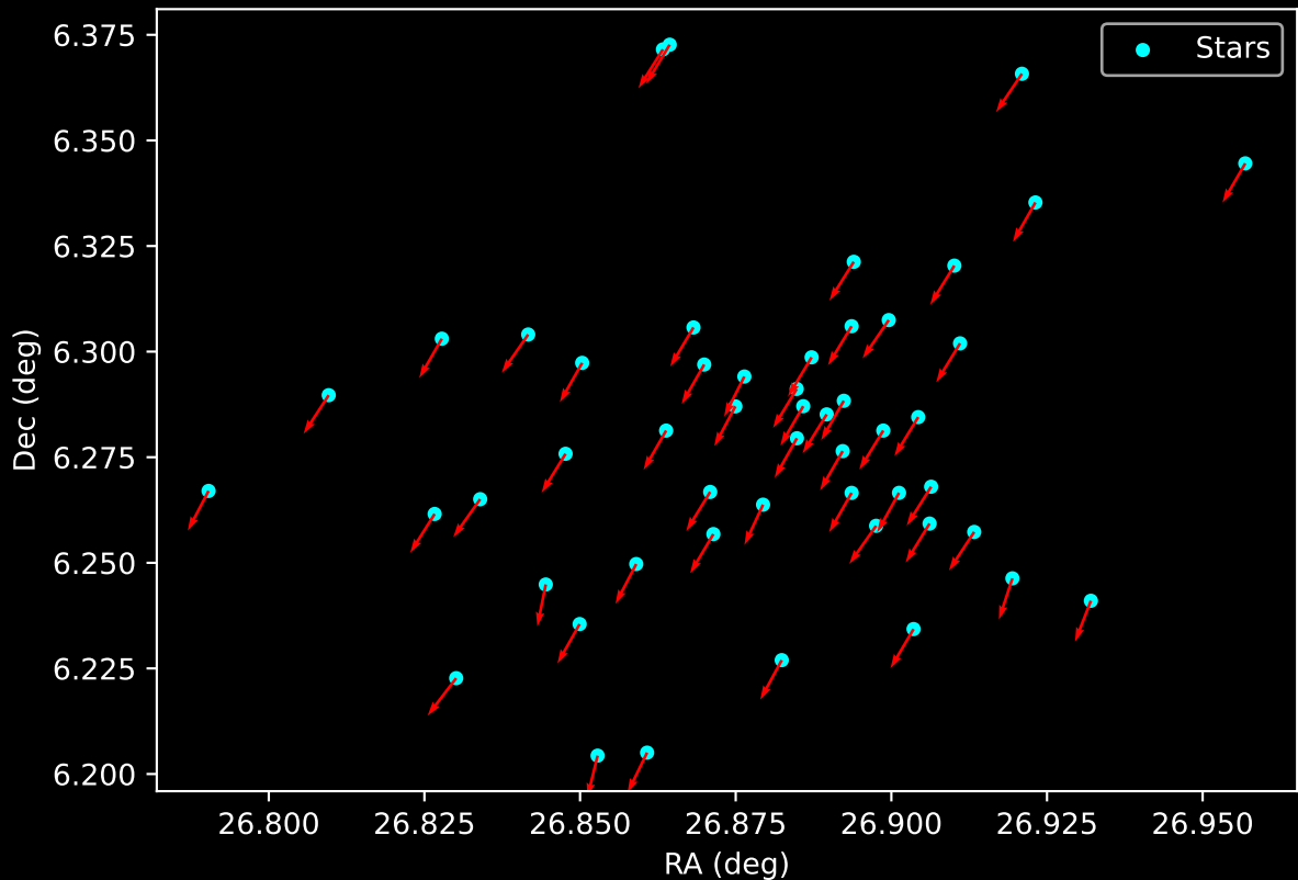
Gaia Cluster: [Juchert_3] Proper Motion Vectors for Gaia Star Field (n= 51)
