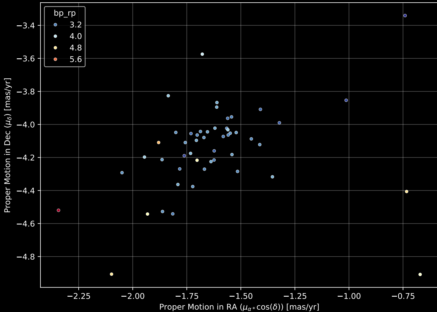
Gaia Cluster: [Juchert_3] Proper Motion Diagram (n= 51)
