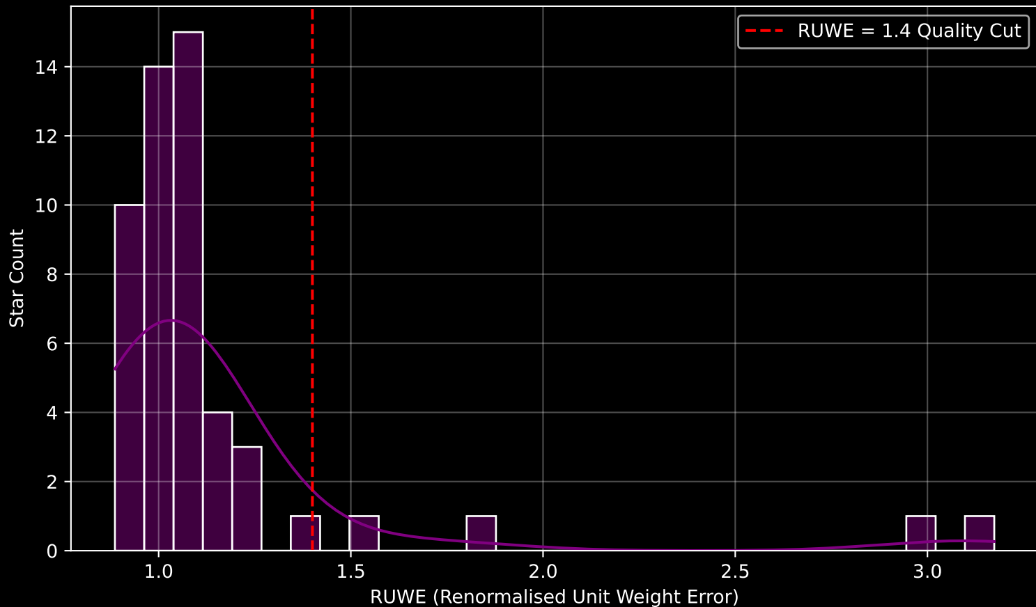
Gaia Cluster: [Juchert_3] RUWE Distribution (n= 51)
