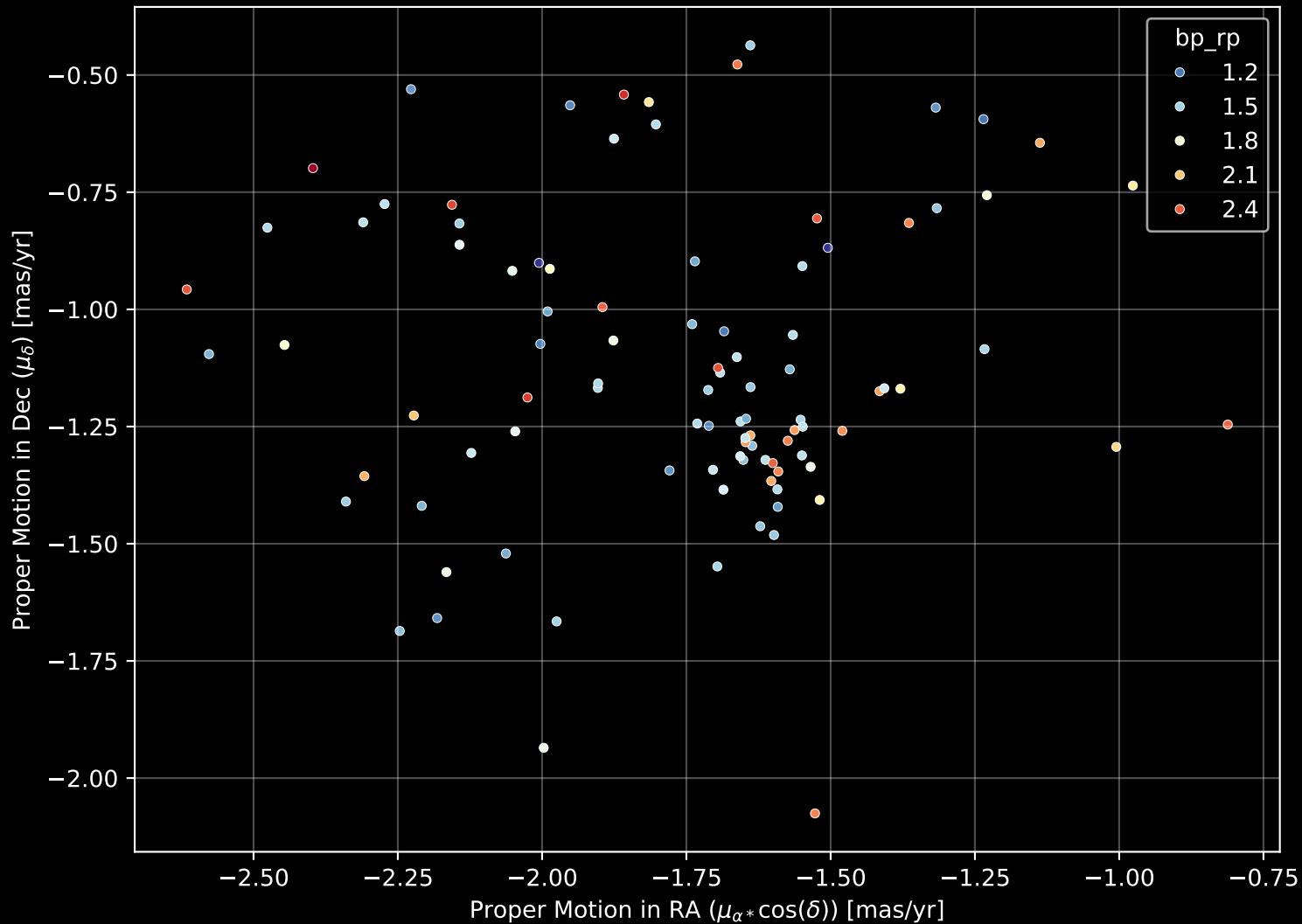
Gaia Cluster: [Juchert_Saloran_1] Proper Motion Diagram (n= 97)
