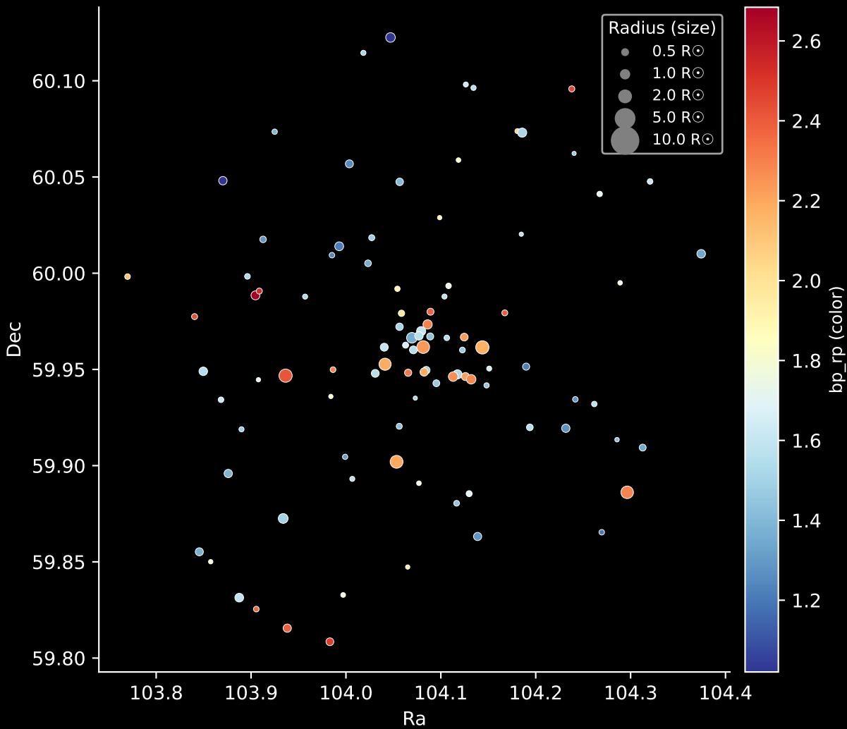
Gaia Cluster: [Juchert_Saloran_1] Stars: 97
