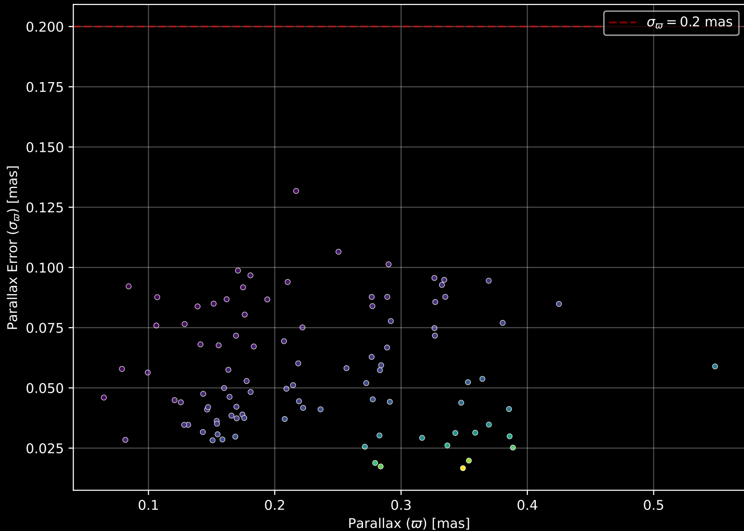
Gaia Cluster: [Juchert_Saloran_1] Parallax Quality (n= 97)
