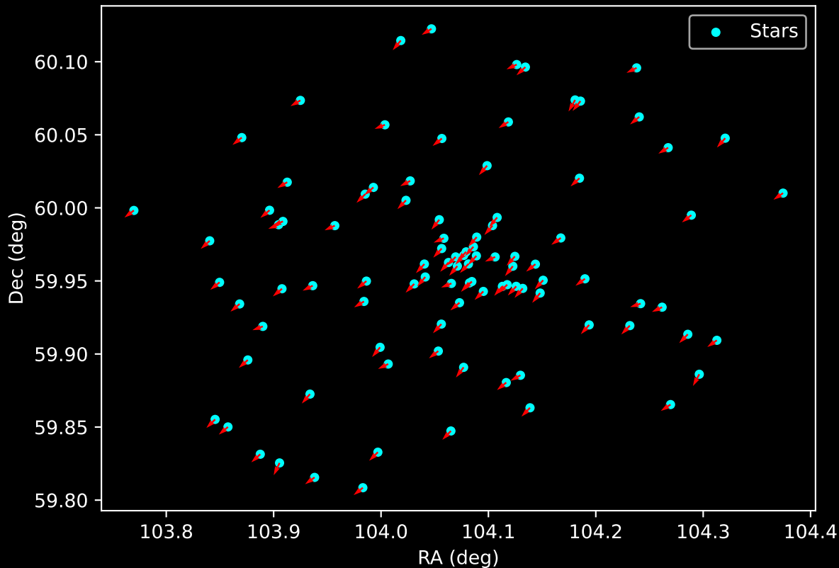
Gaia Cluster: [Juchert_Saloran_1] Proper Motion Vectors for Gaia Star Field (n= 97)
