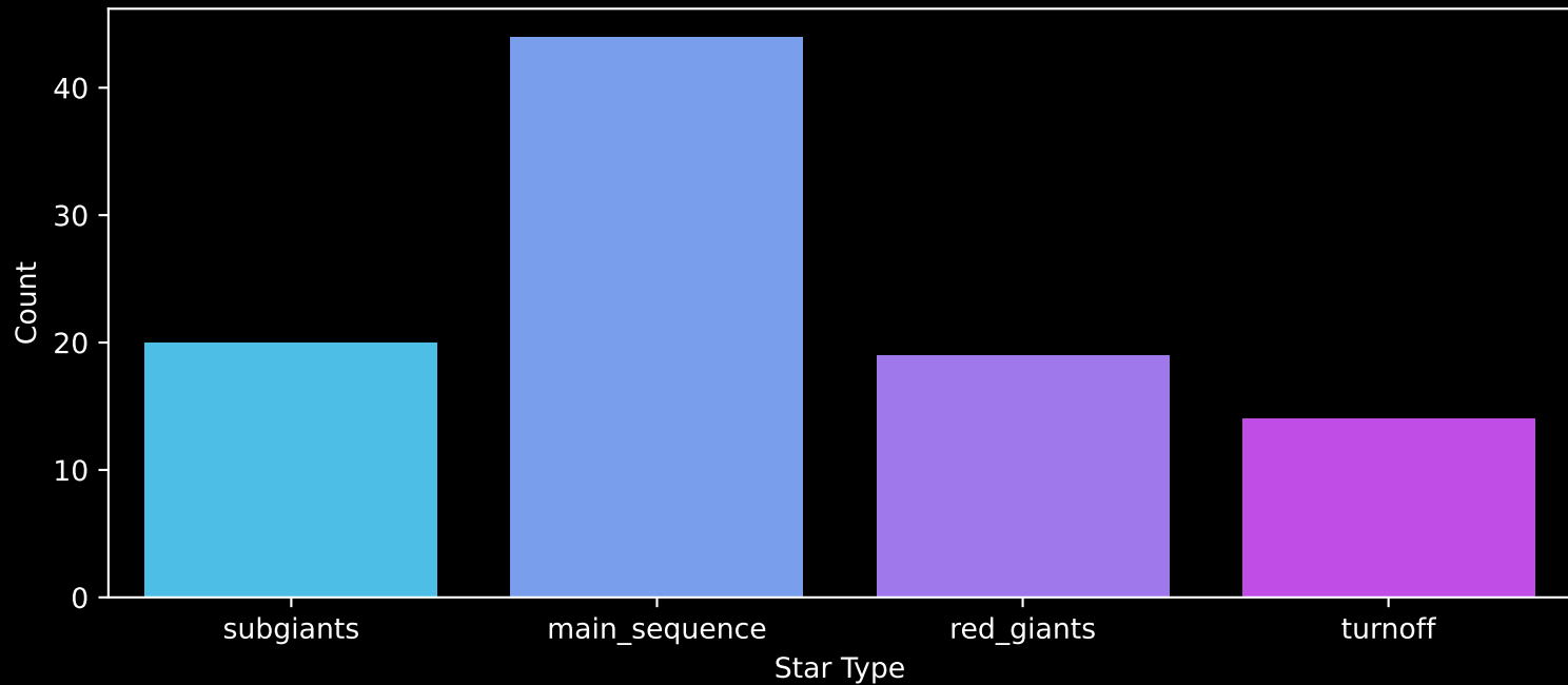
Gaia Cluster: [Juchert_Saloran_1] Count plot of Star Type
