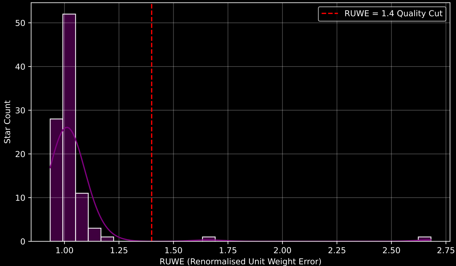
Gaia Cluster: [Juchert_Saloran_1] RUWE Distribution (n= 97)
