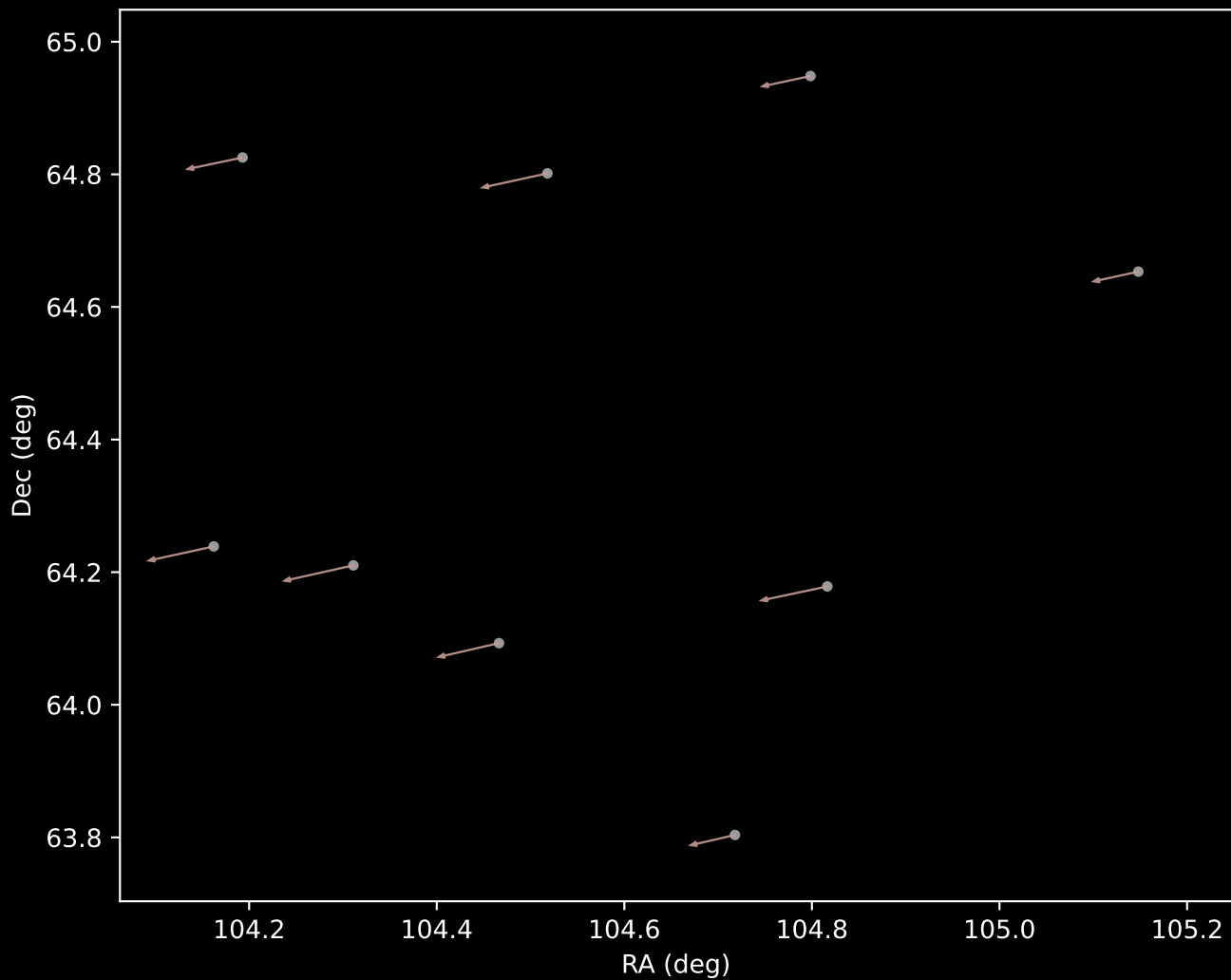
Gaia DR3 Cluster 11 Proper Motion Vectors (n=9)
