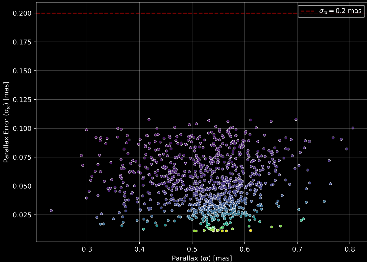
Gaia Cluster: [King_1] Parallax Quality (n= 947)
