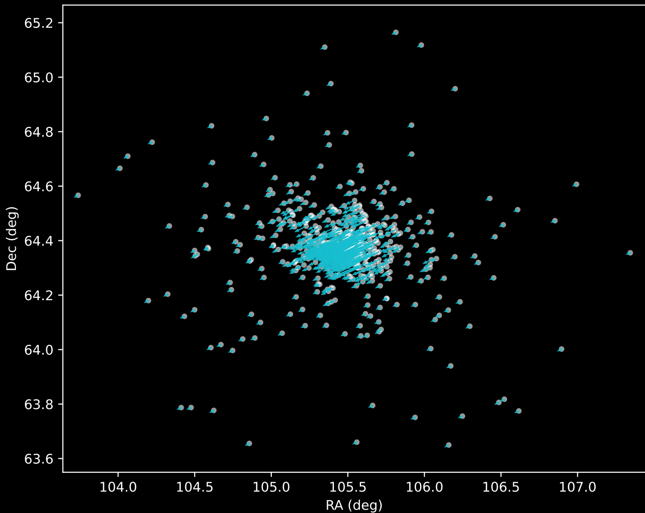
Gaia DR3 Cluster 18 Proper Motion Vectors (n=560)
