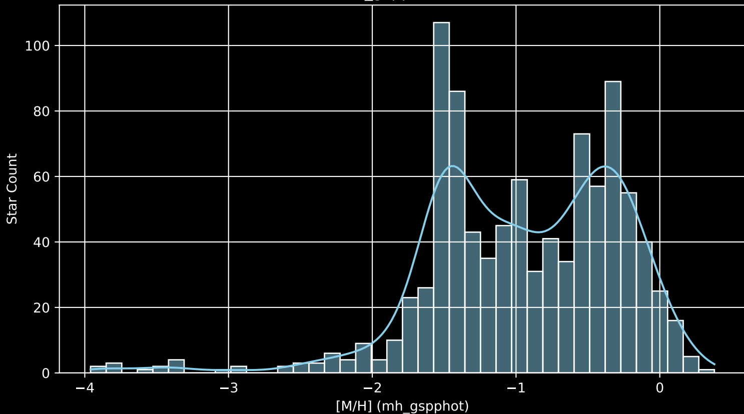
Gaia Cluster: [King_1 [M/H] (mh_gspphot) (n= 947)
