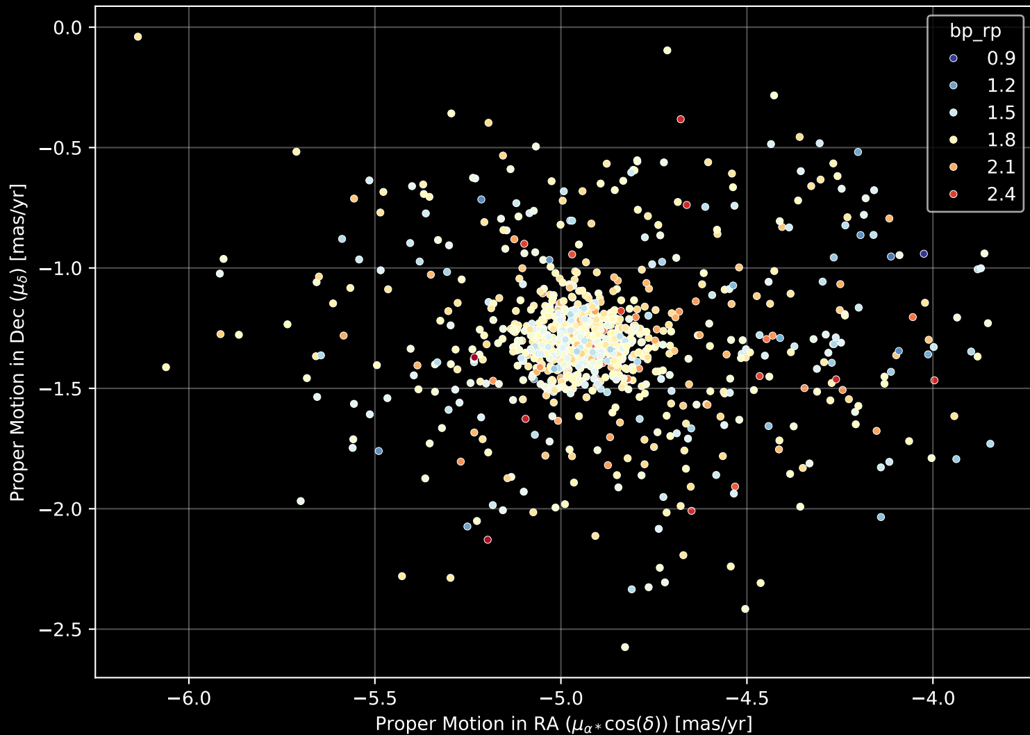
Gaia Cluster: [King_1] Proper Motion Diagram (n= 947)
