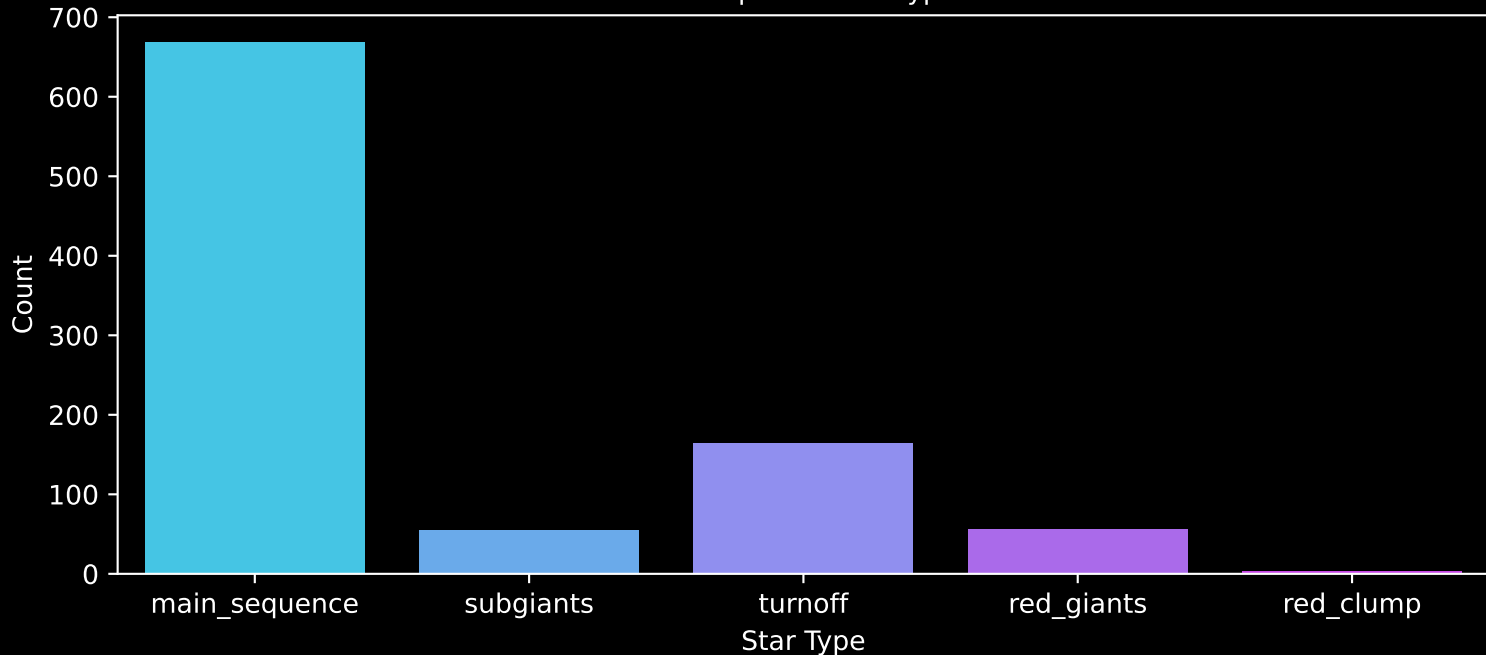
Gaia Cluster: [King_1] Count plot of Star Type
