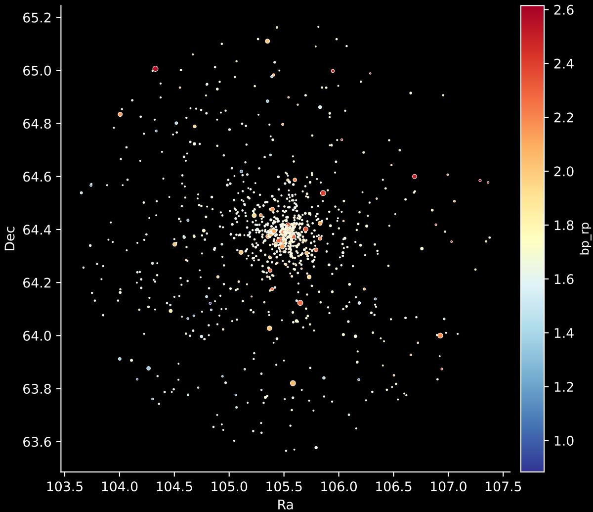
Gaia Cluster: [King_1] Stars: 947
