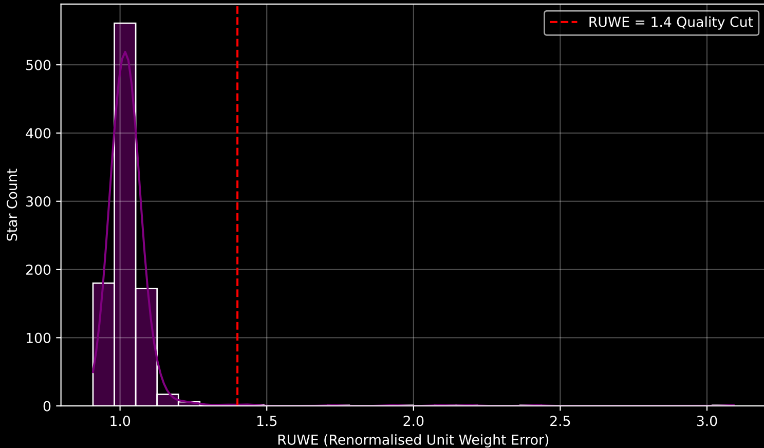
Gaia Cluster: [King_1] RUWE Distribution (n= 947)
