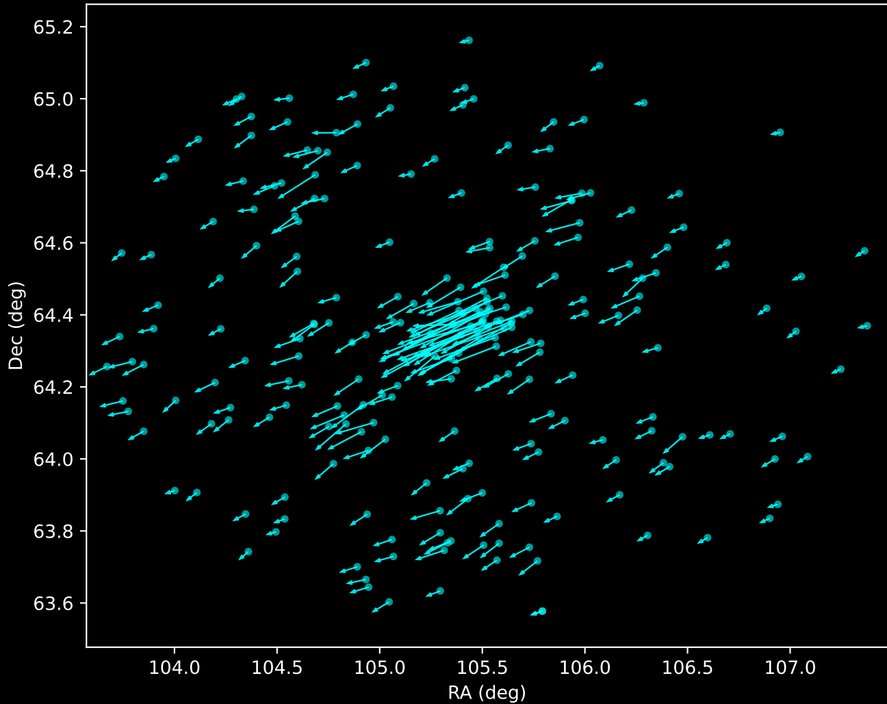
Gaia DR3 Noise Stream Proper Motion Vectors (n=238)
