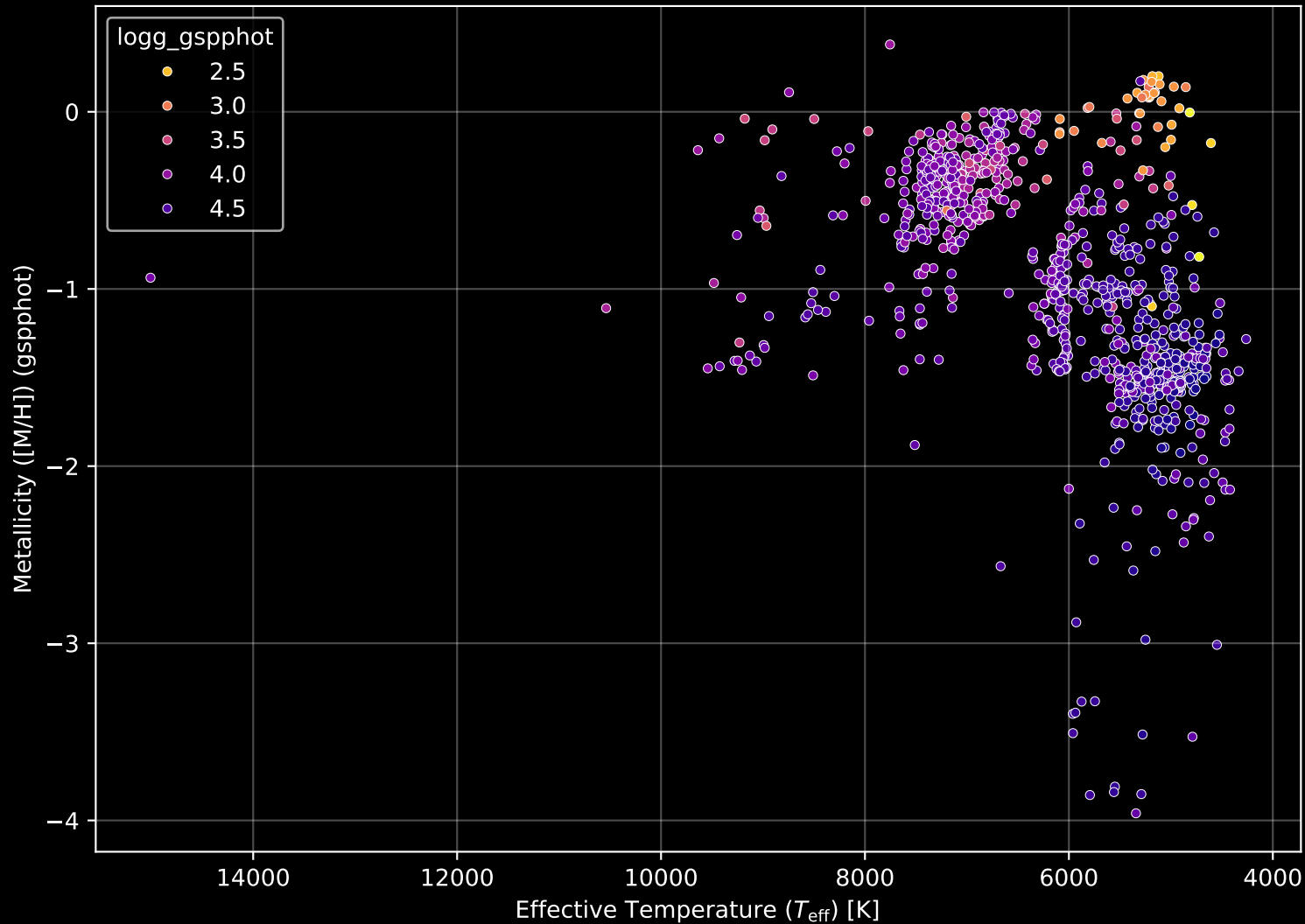
Gaia Cluster: [King_1] Stellar Population Parameters (n= 947)
