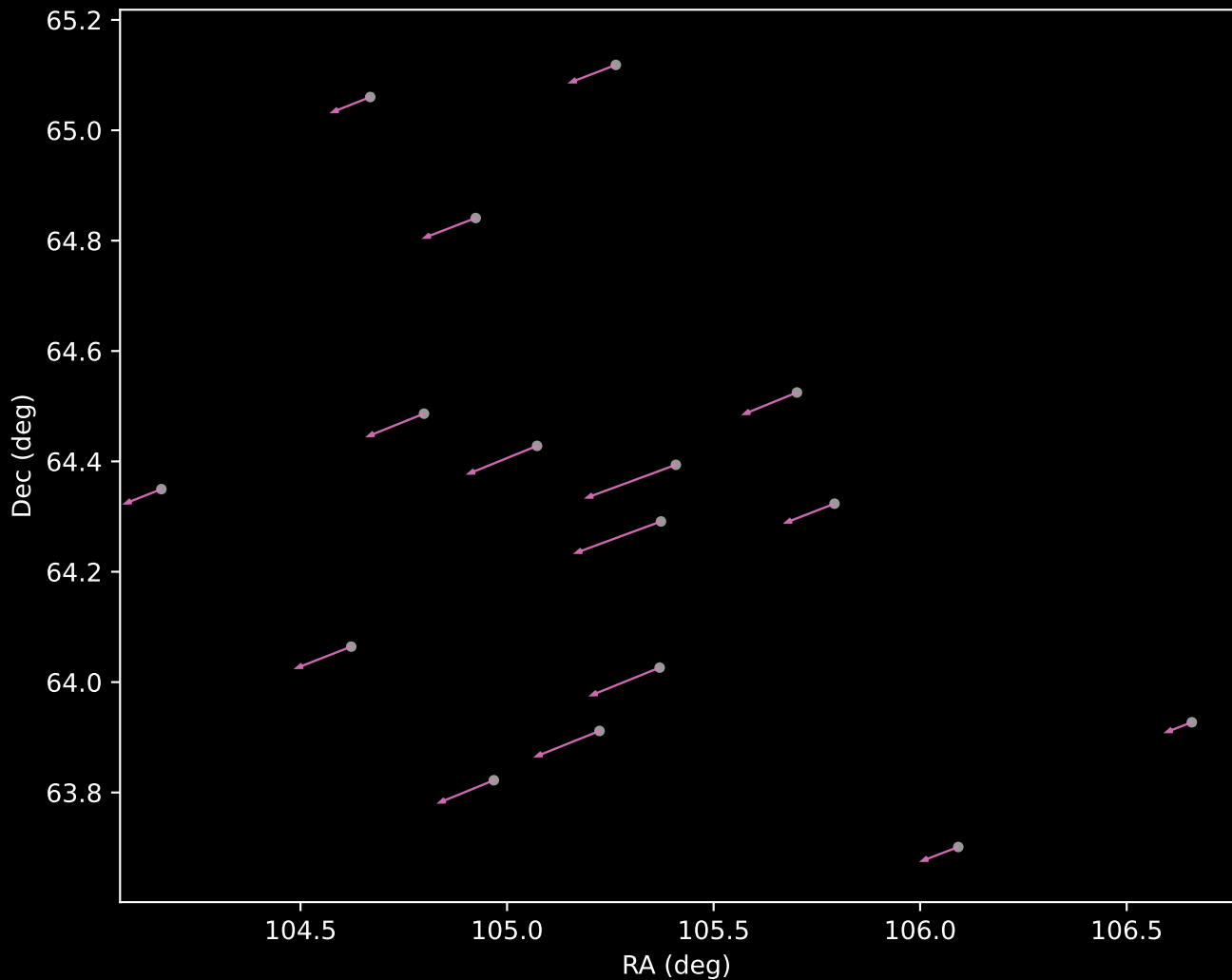
Gaia DR3 Cluster 12 Proper Motion Vectors (n=16)
