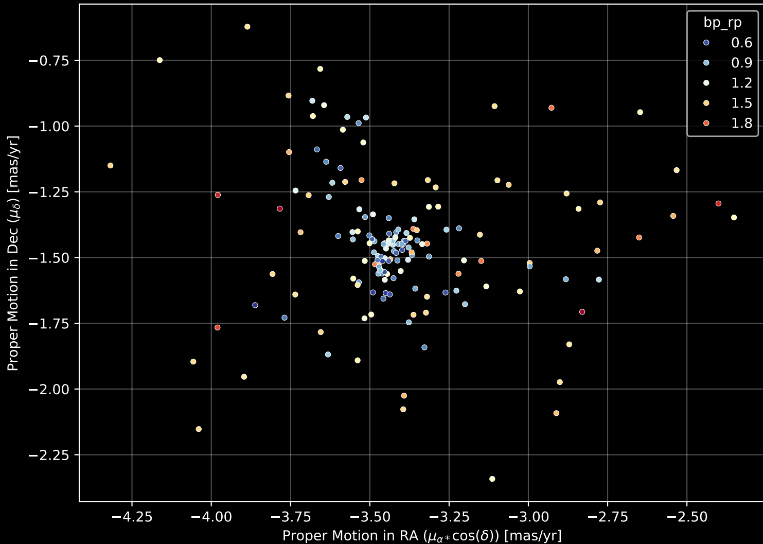
Gaia Cluster: [King_12] Proper Motion Diagram (n= 165)
