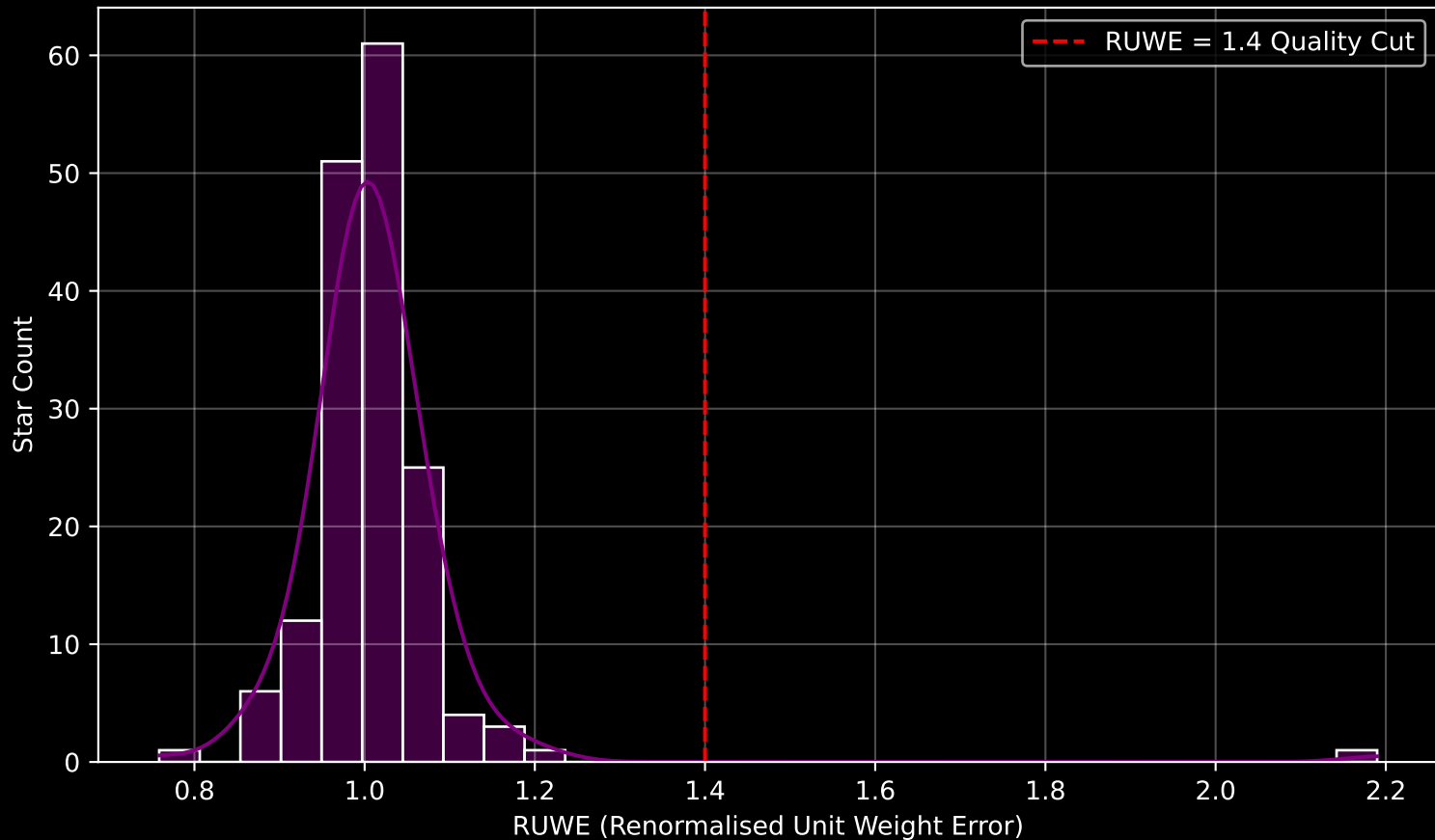
Gaia Cluster: [King_12] RUWE Distribution (n= 165)
