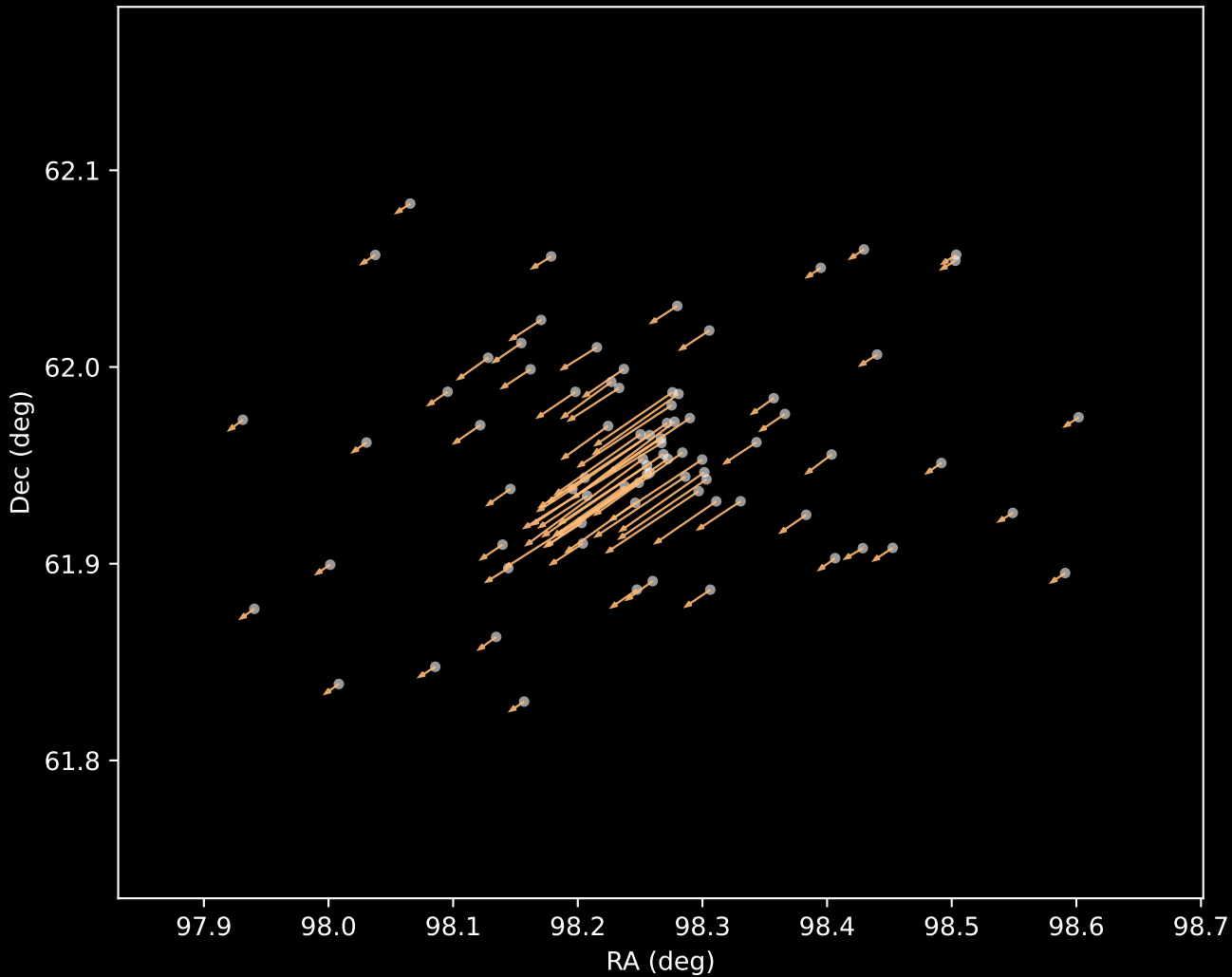
Gaia DR3 Cluster 3 Proper Motion Vectors (n=80)
