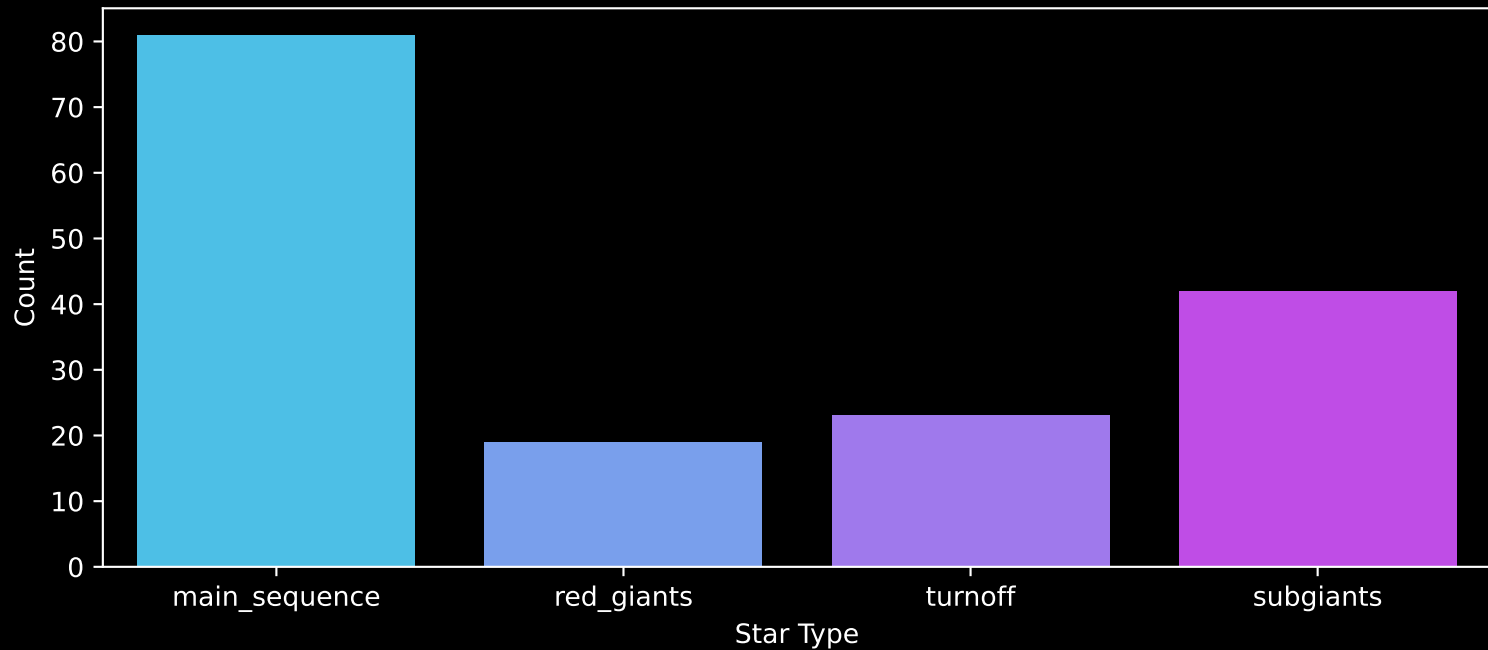
Gaia Cluster: [King_12] Count plot of Star Type
