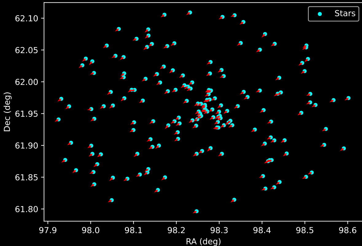
Gaia Cluster: [King_12] Proper Motion Vectors for Gaia Star Field (n= 165)
