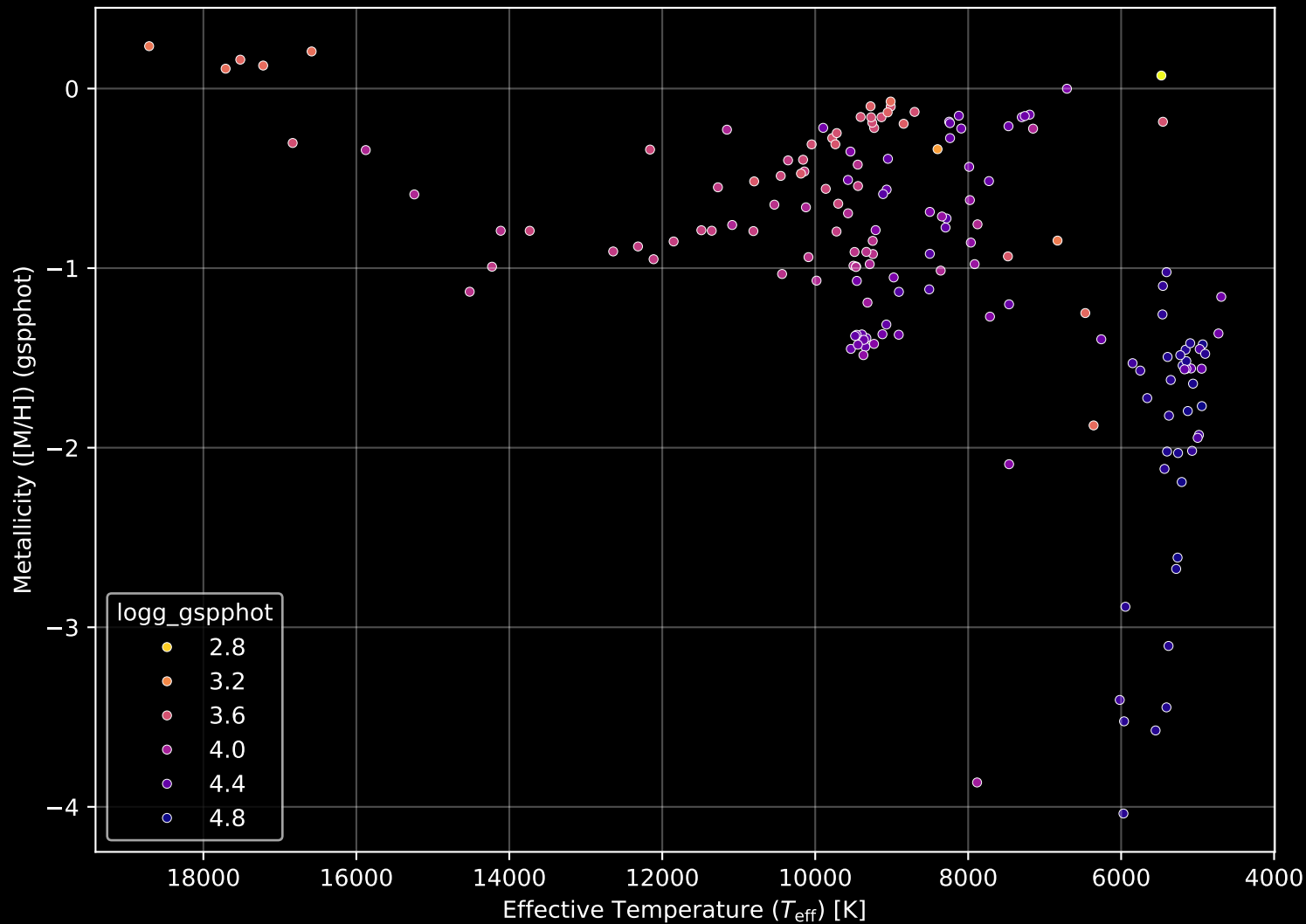
Gaia Cluster: [King_12] Stellar Population Parameters (n= 165)
