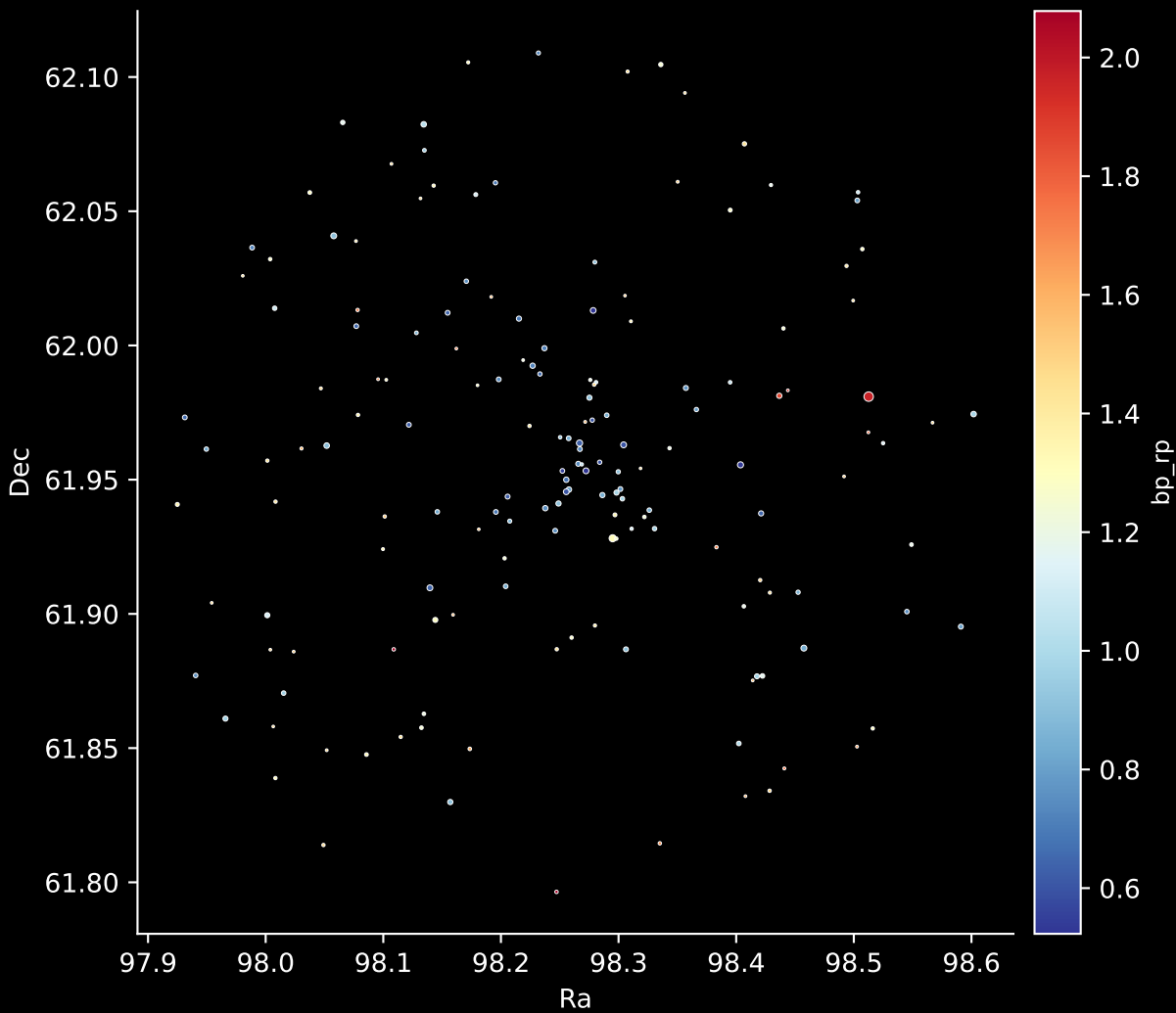
Gaia Cluster: [King_12] Stars: 165
