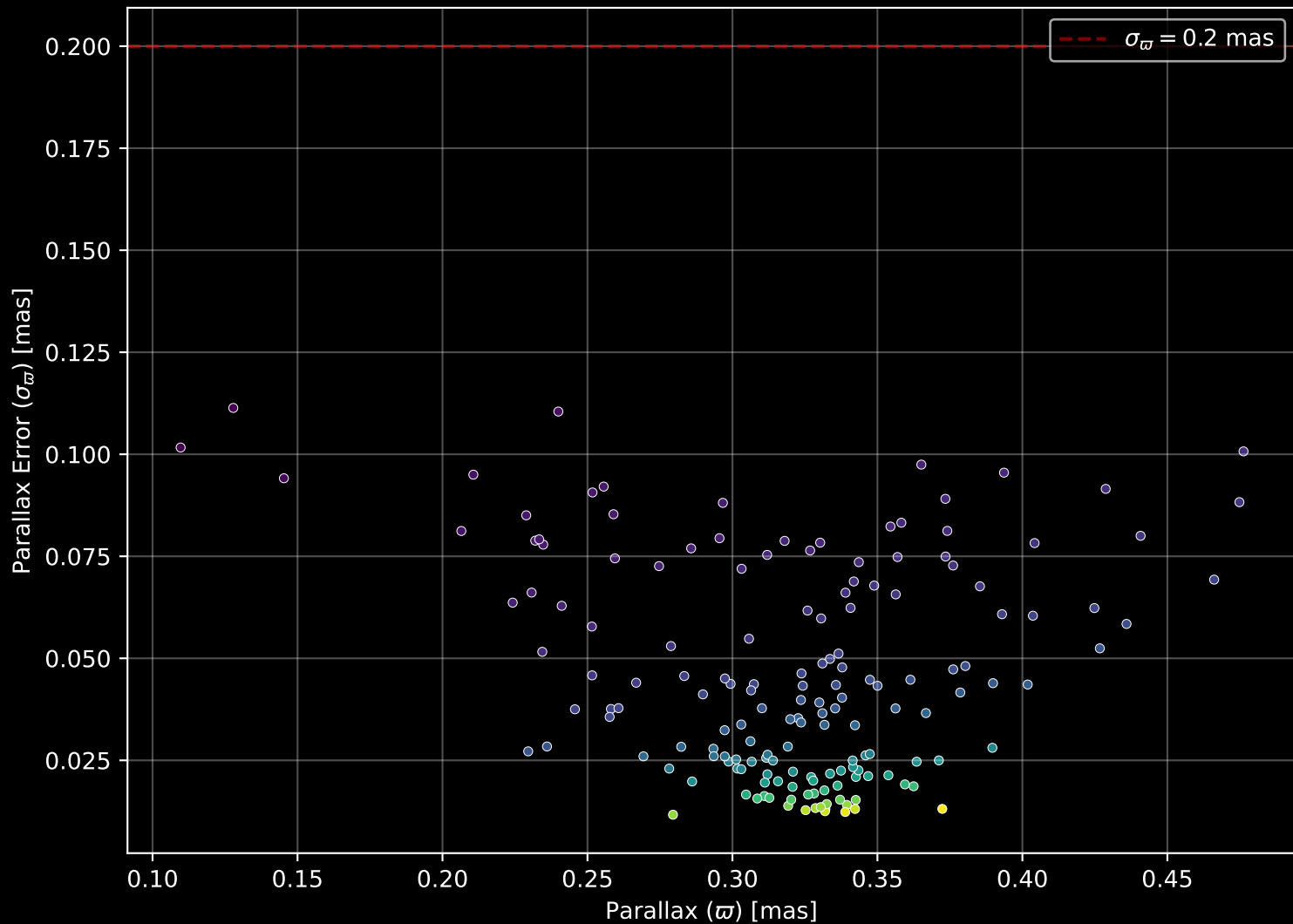
Gaia Cluster: [King_12] Parallax Quality (n= 165)
