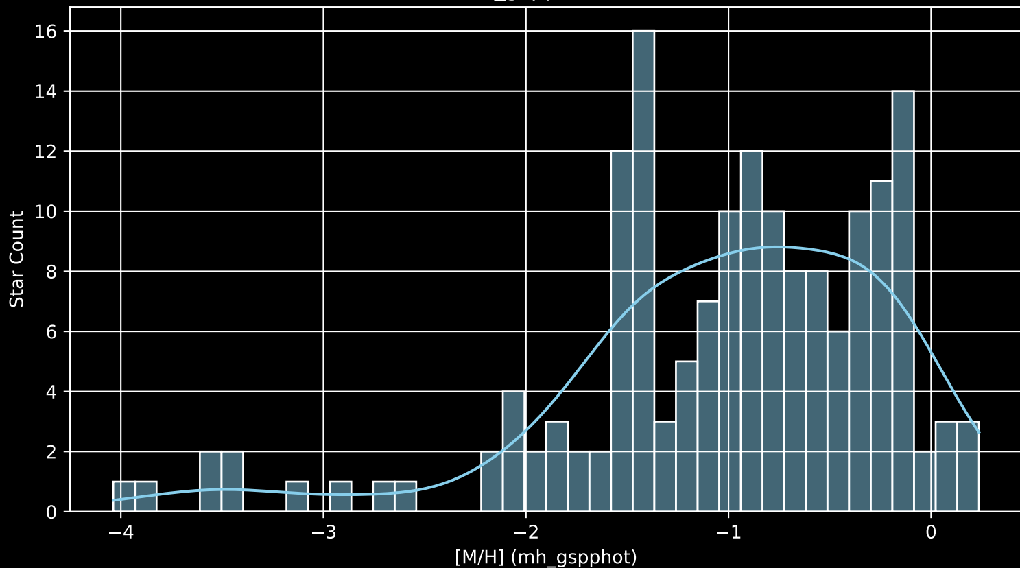
Gaia Cluster: [King_12 [M/H] (mh_gspphot) (n= 165)
