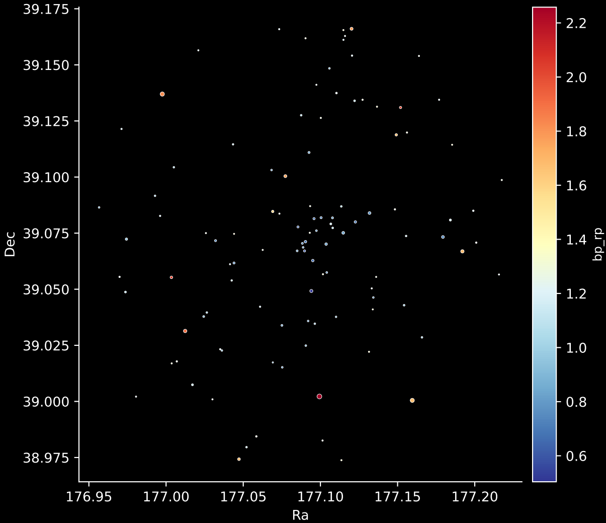
Gaia Cluster: [King_17] Stars: 109
