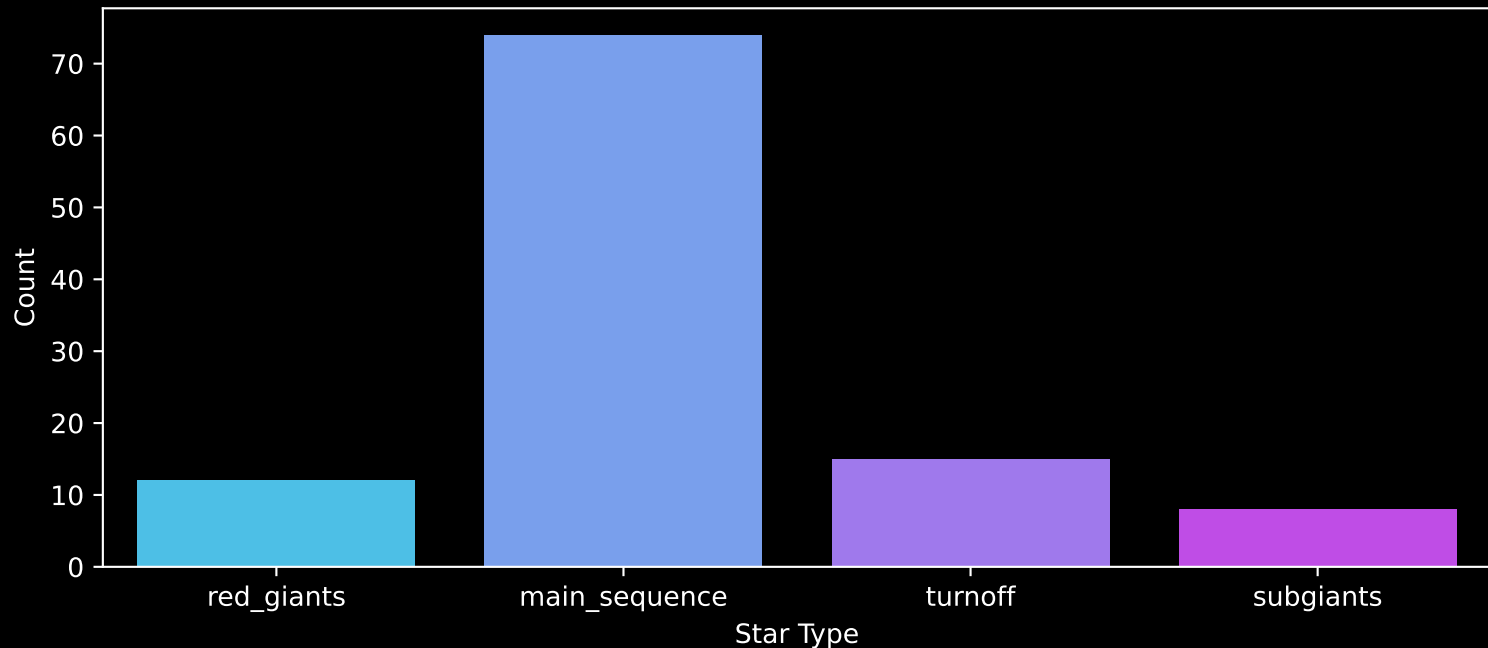
Gaia Cluster: [King_17] Count plot of Star Type
