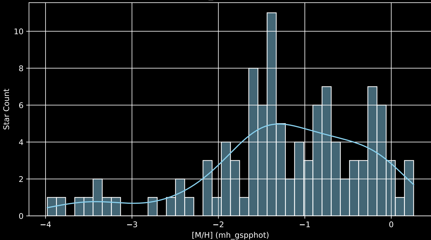
Gaia Cluster: [King_17 [M/H] (mh_gspphot) (n= 109)
