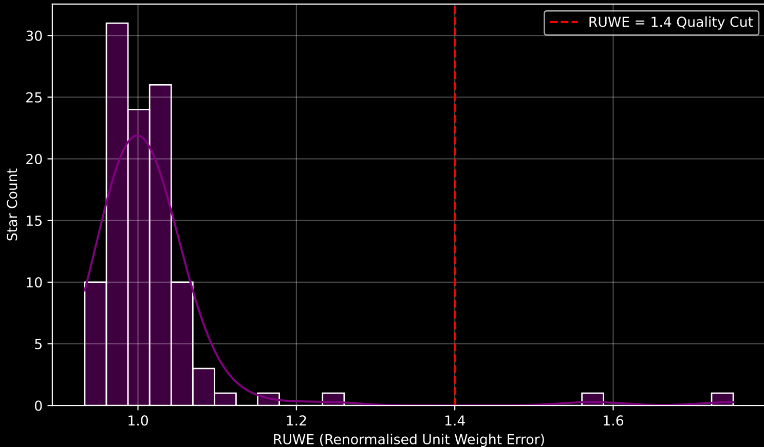
Gaia Cluster: [King_17] RUWE Distribution (n= 109)
