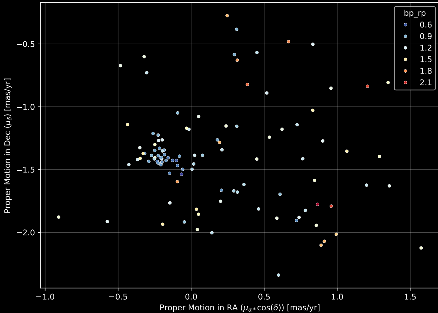
Gaia Cluster: [King_17] Proper Motion Diagram (n= 109)
