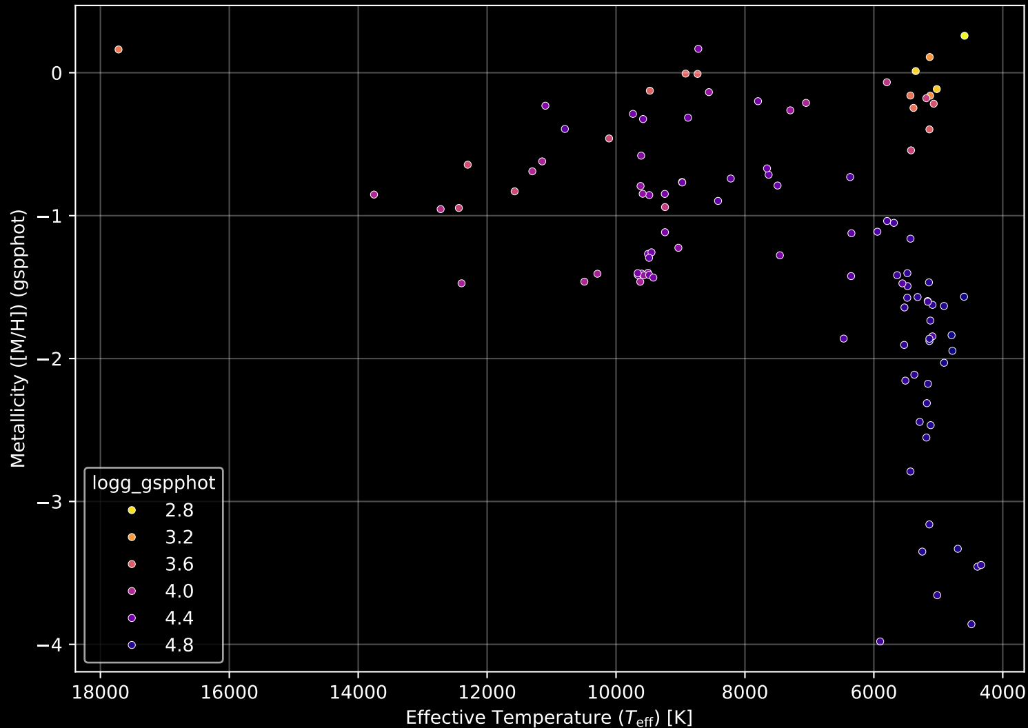
Gaia Cluster: [King_17] Stellar Population Parameters (n= 109)
