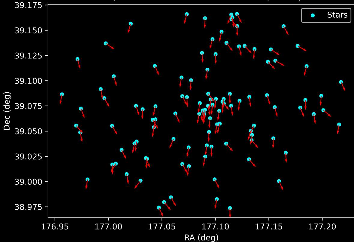
Gaia Cluster: [King_17] Proper Motion Vectors for Gaia Star Field (n= 109)
