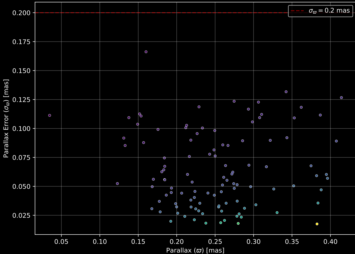
Gaia Cluster: [King_17] Parallax Quality (n= 109)
