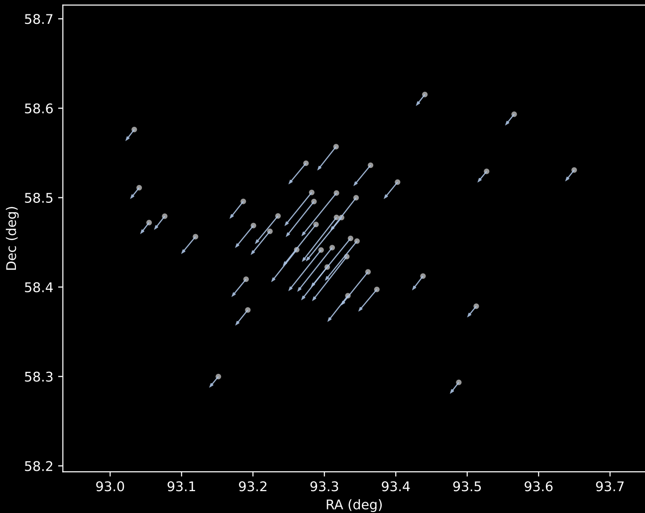
Gaia DR3 Cluster 1 Proper Motion Vectors (n=40)
