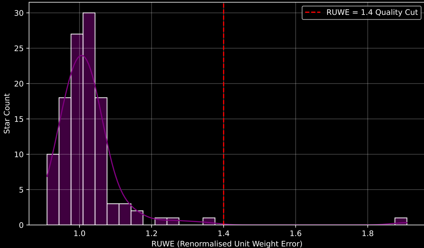
Gaia Cluster: [King_20] RUWE Distribution (n= 115)
