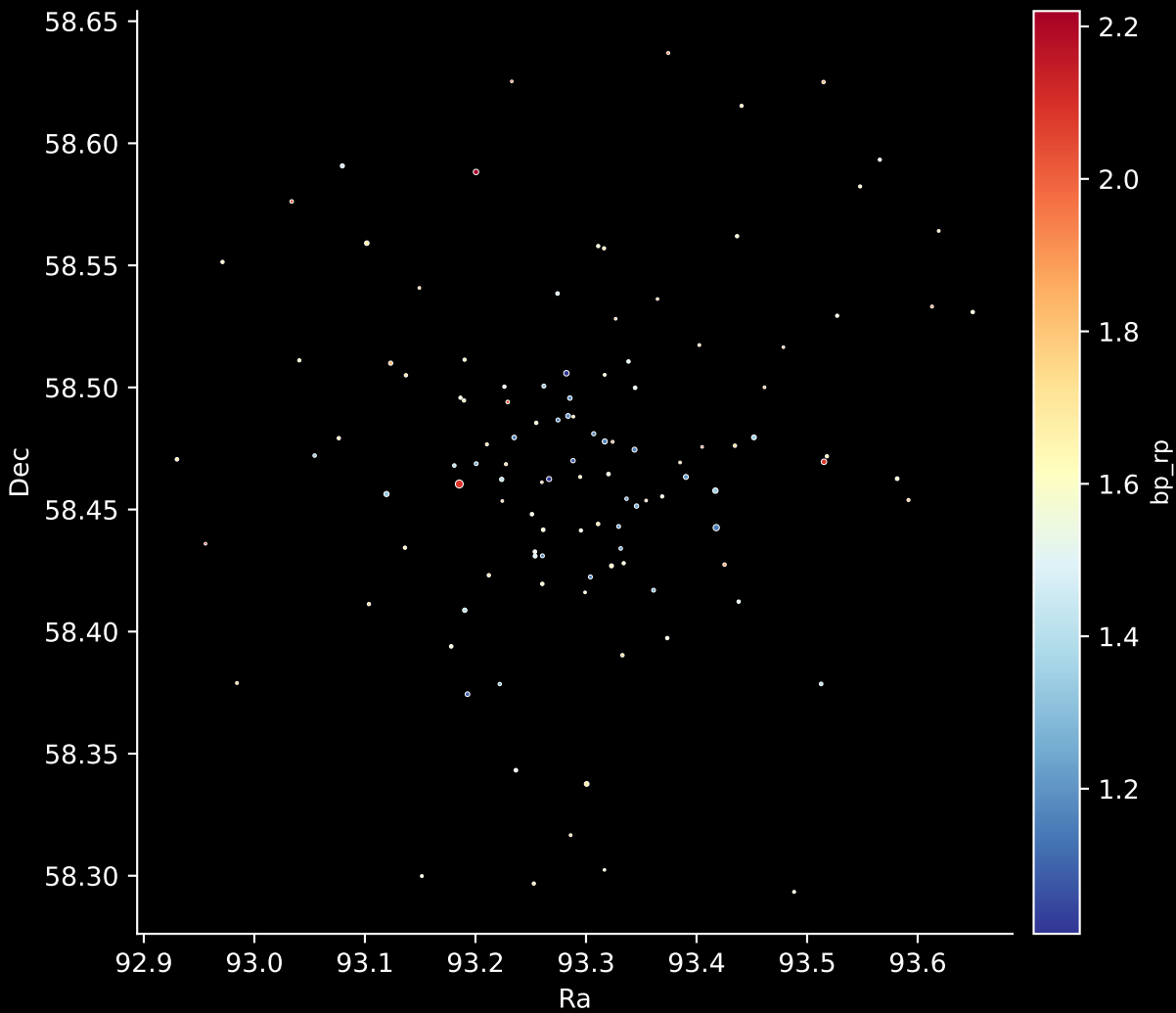
Gaia Cluster: [King_20] Stars: 115
