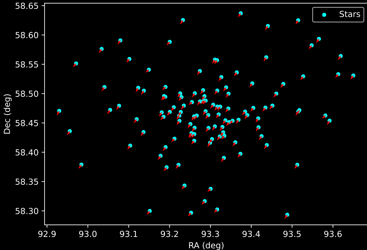
Gaia Cluster: [King_20] Proper Motion Vectors for Gaia Star Field (n= 115)
