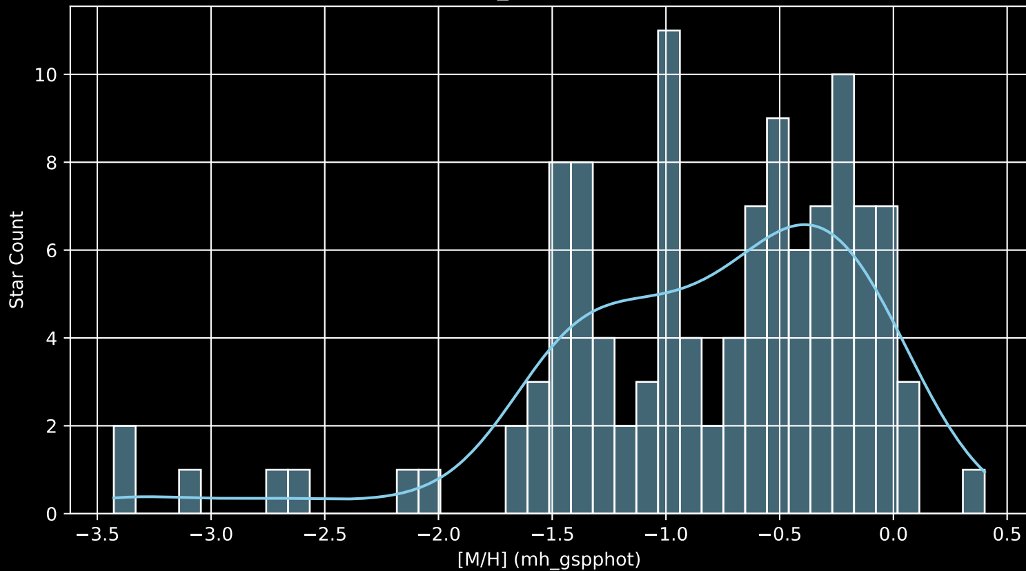
Gaia Cluster: [King_20 [M/H] (mh_gspphot) (n= 115)
