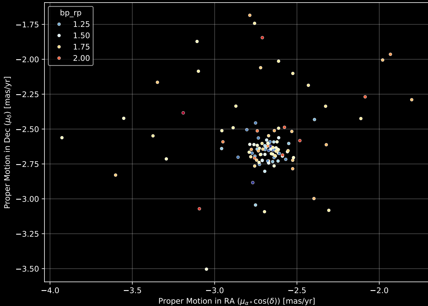
Gaia Cluster: [King_20] Proper Motion Diagram (n= 115)
