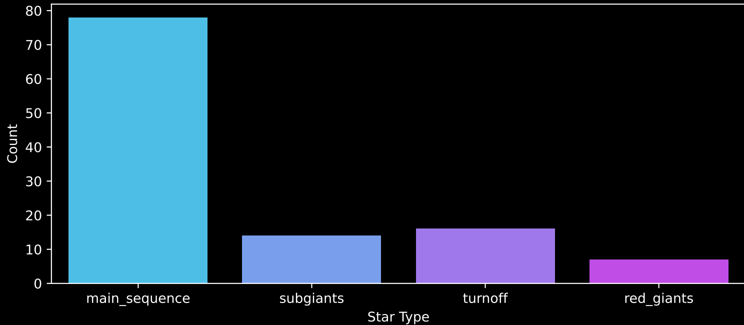
Gaia Cluster: [King_20] Count plot of Star Type
