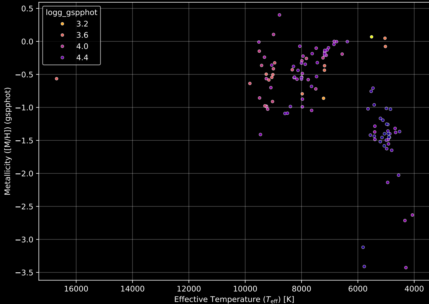
Gaia Cluster: [King_20] Stellar Population Parameters (n= 115)
