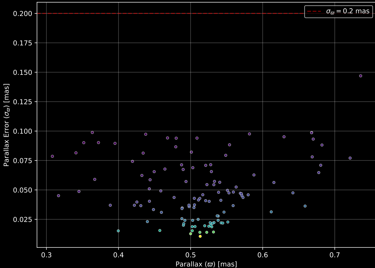
Gaia Cluster: [King_20] Parallax Quality (n= 115)
