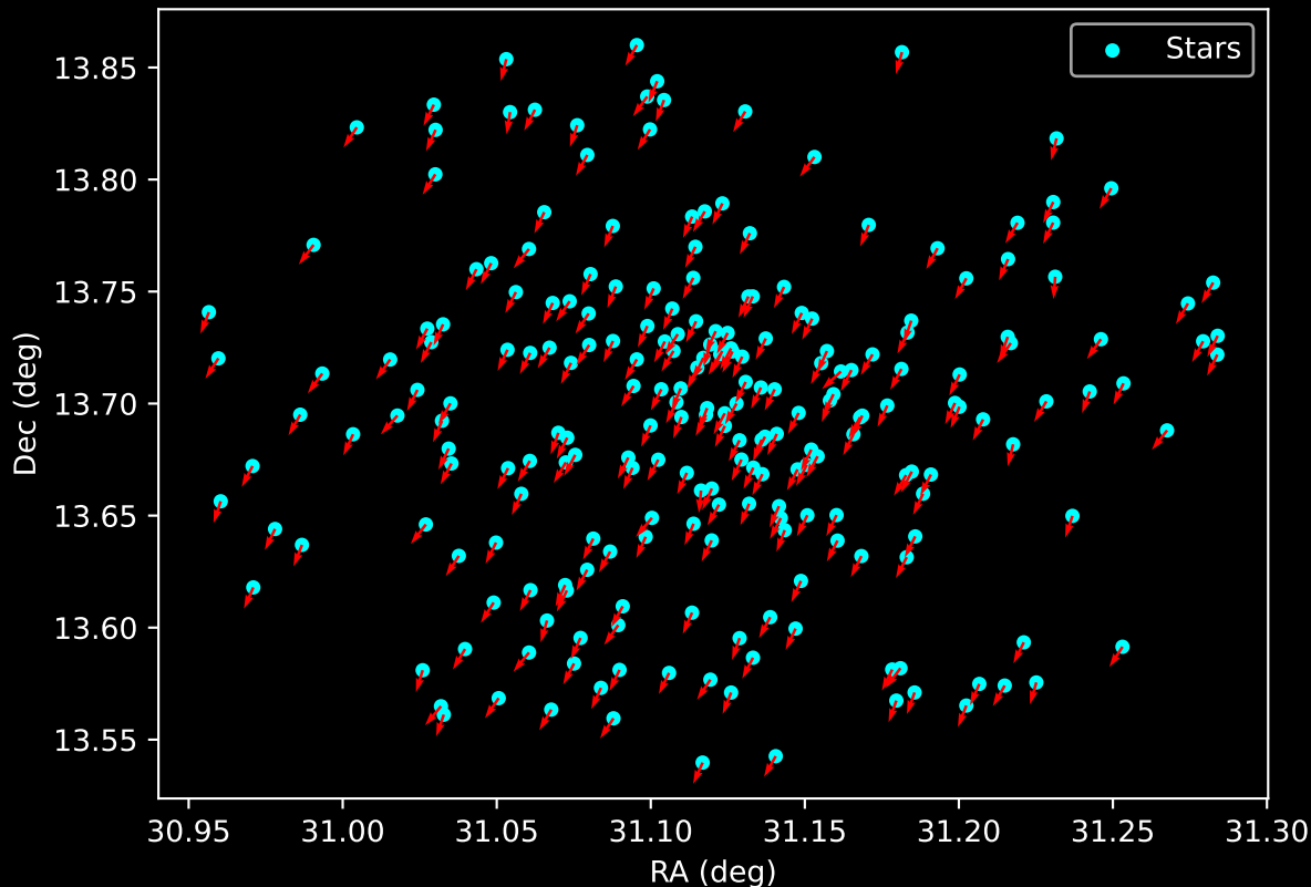
Gaia Cluster: [King_25] Proper Motion Vectors for Gaia Star Field (n= 231)
