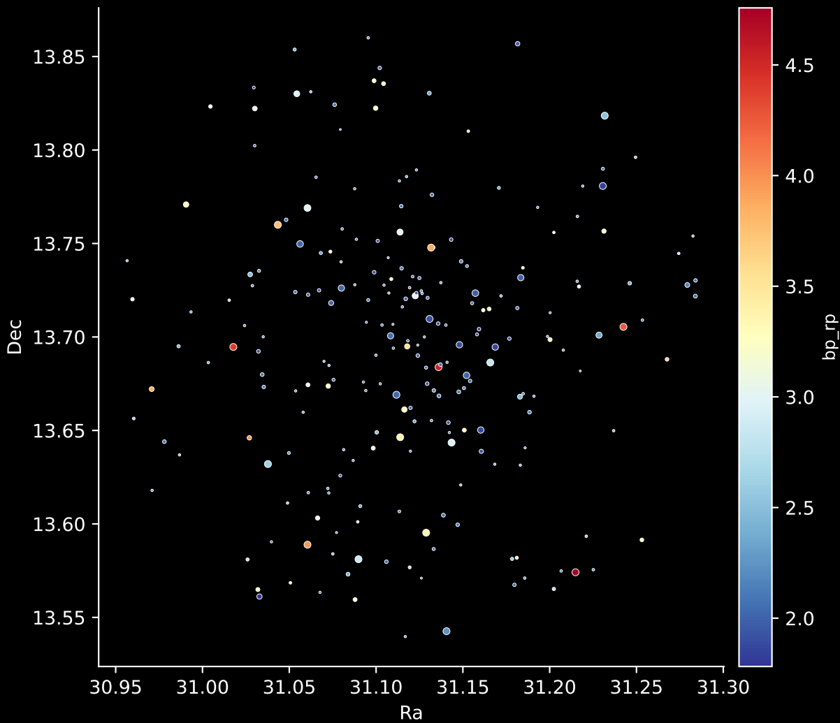
Gaia Cluster: [King_25] Stars: 231
