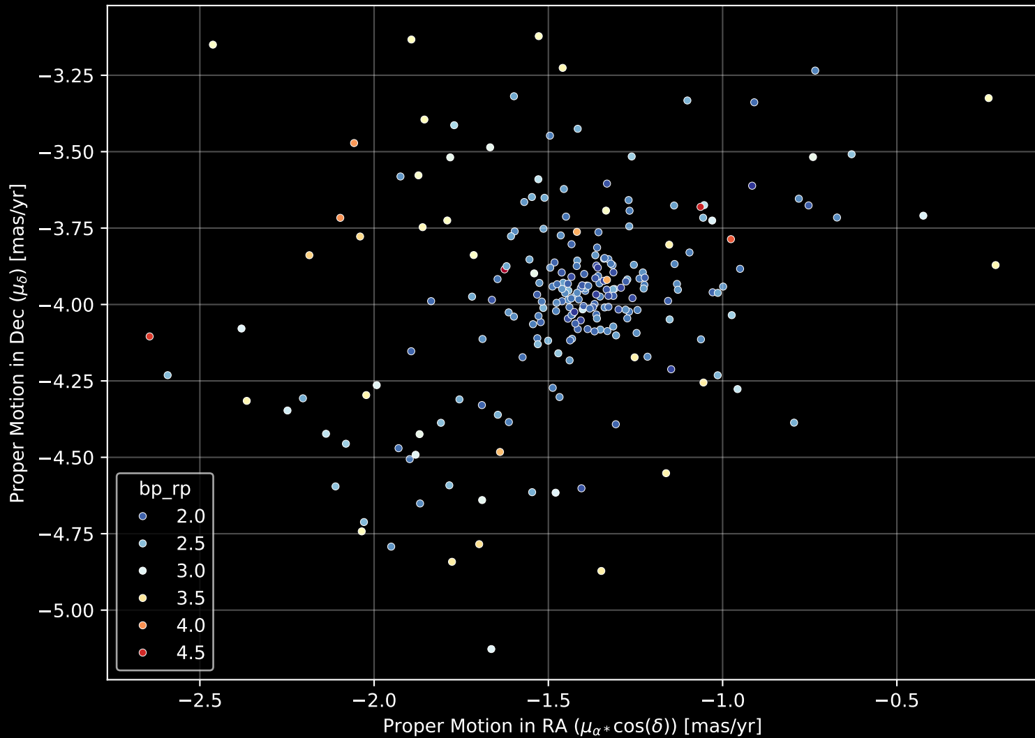
Gaia Cluster: [King_25] Proper Motion Diagram (n= 231)
