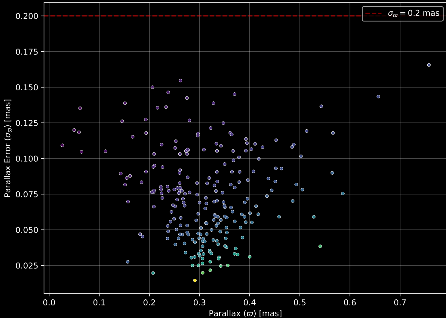
Gaia Cluster: [King_25] Parallax Quality (n= 231)
