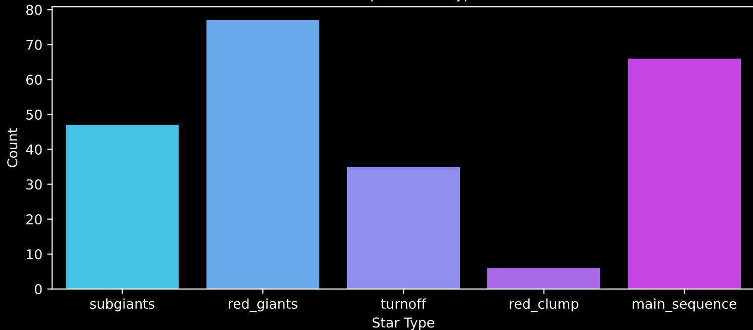
Gaia Cluster: [King_25] Count plot of Star Type
