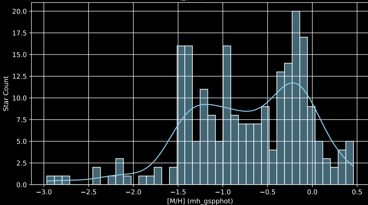
Gaia Cluster: [King_25 [M/H] (mh_gspphot) (n= 227)
