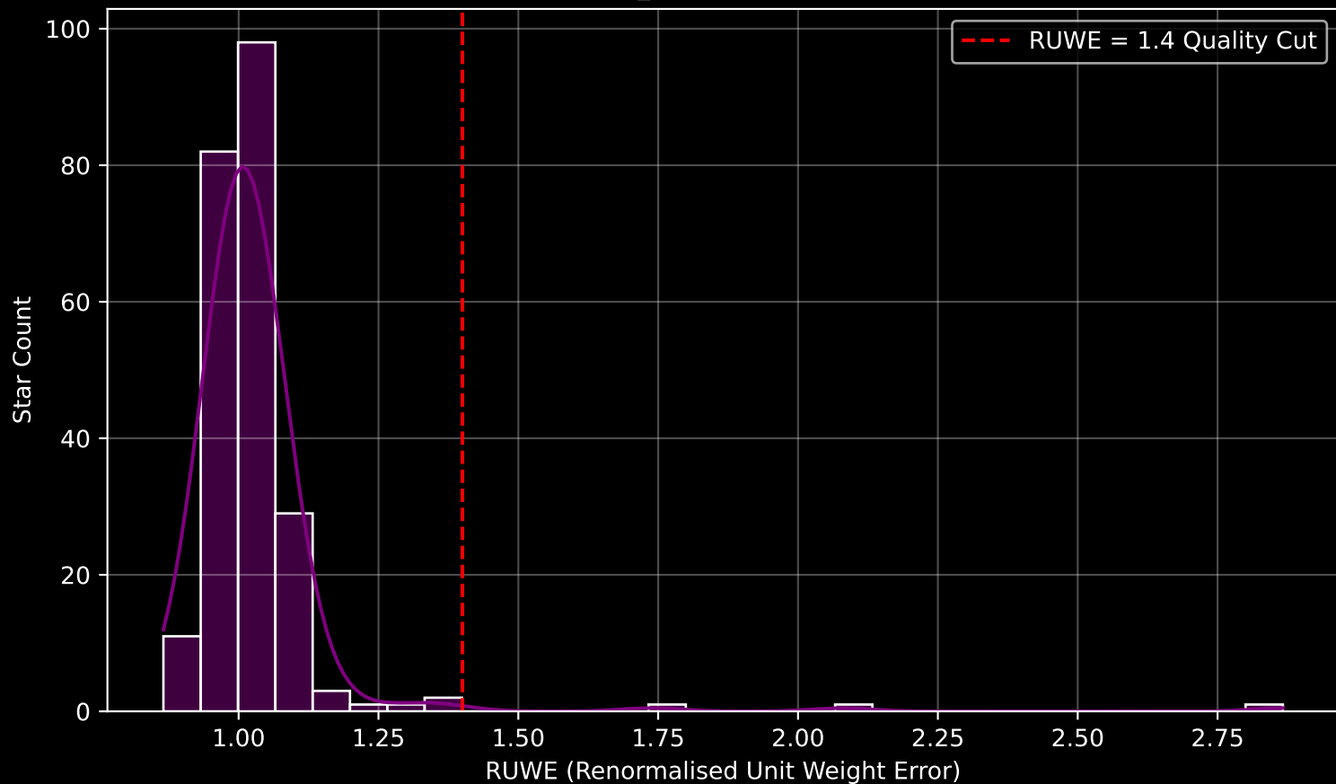
Gaia Cluster: [King_25] RUWE Distribution (n= 230)
