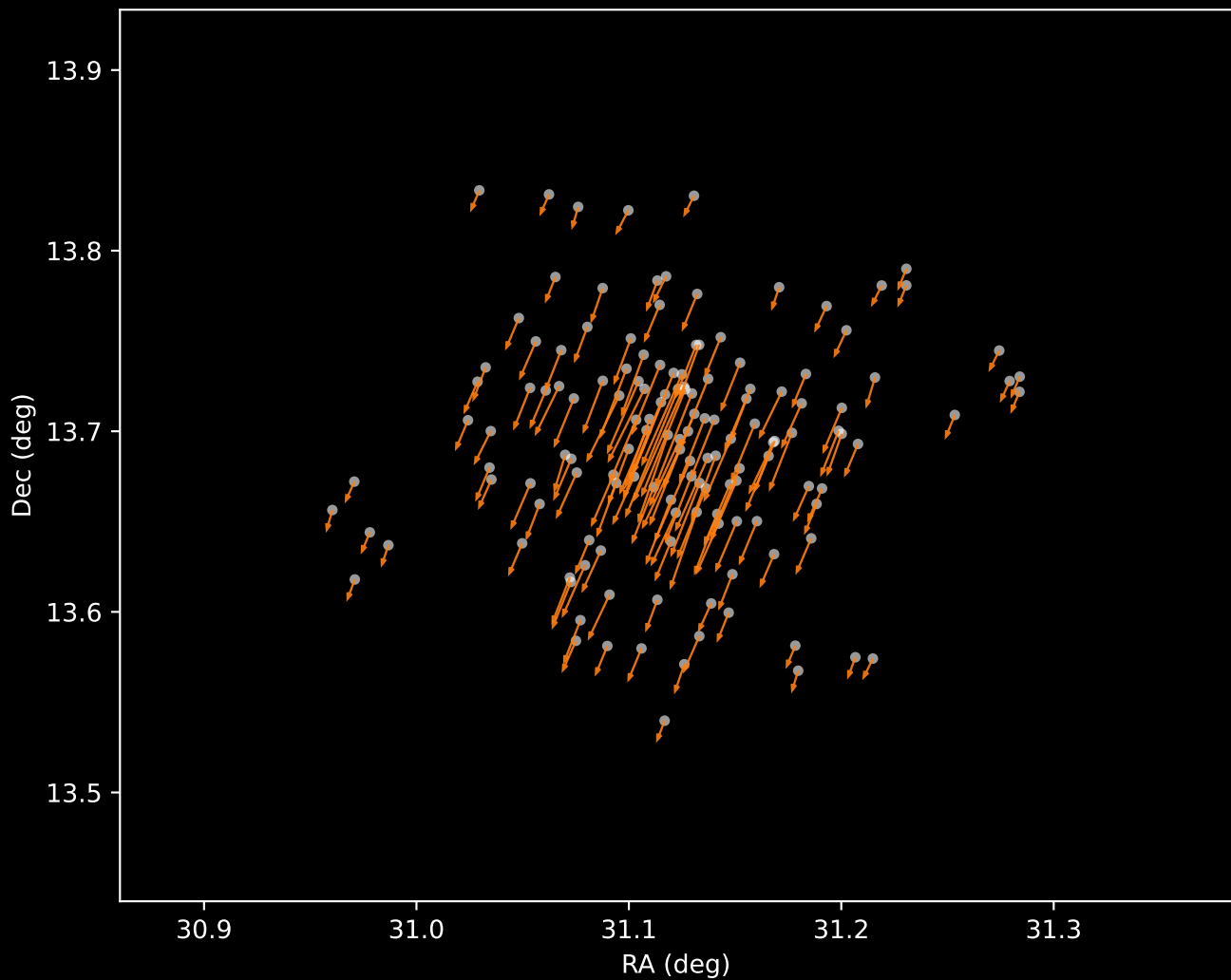
Gaia DR3 Cluster 2 Proper Motion Vectors (n=142)
