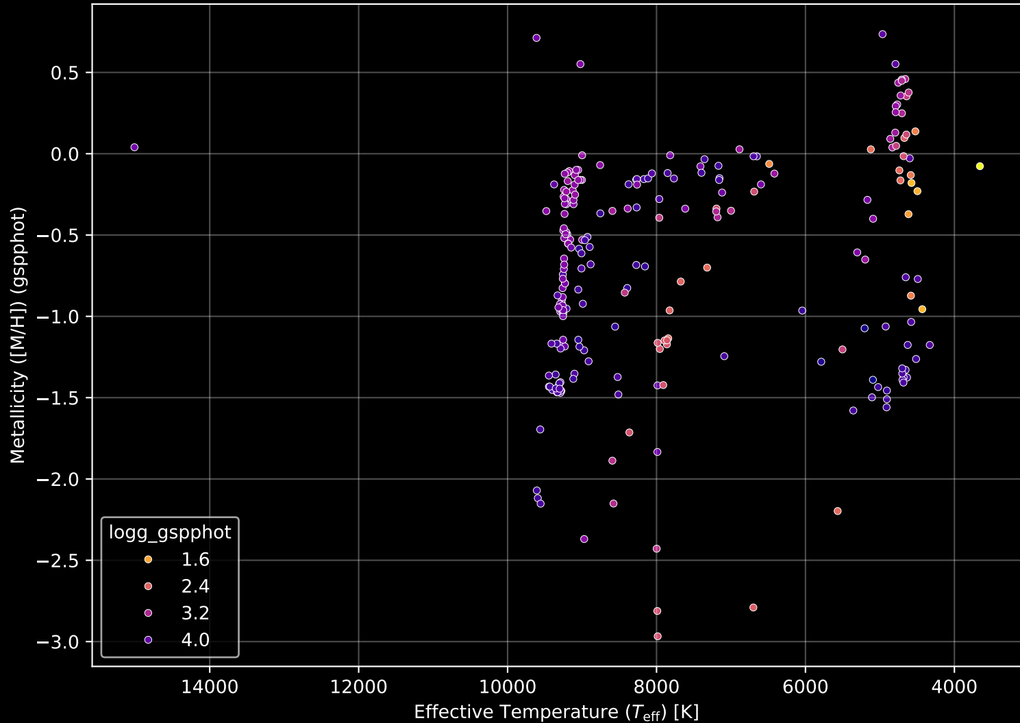
Gaia Cluster: [King_25] Stellar Population Parameters (n= 231)
