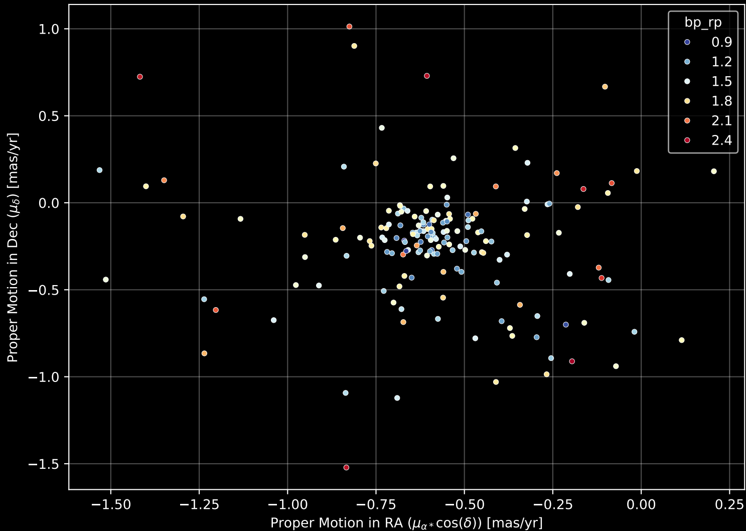
Gaia Cluster: [King_4] Proper Motion Diagram (n= 171)
