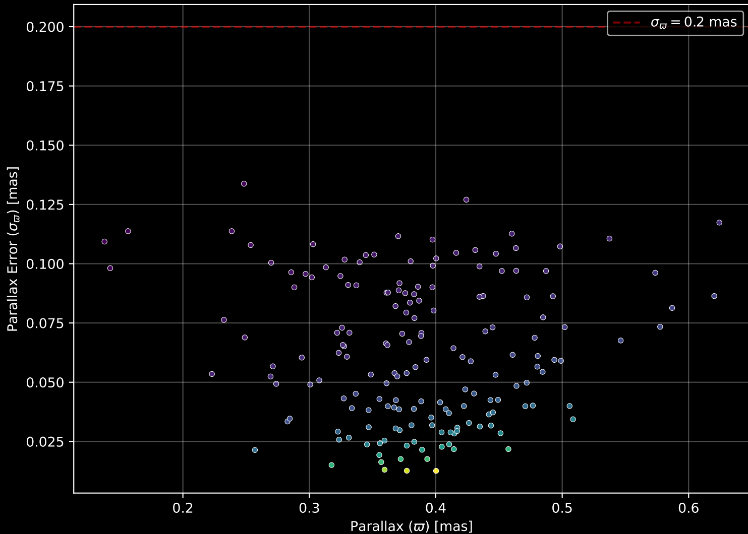
Gaia Cluster: [King_4] Parallax Quality (n= 171)
