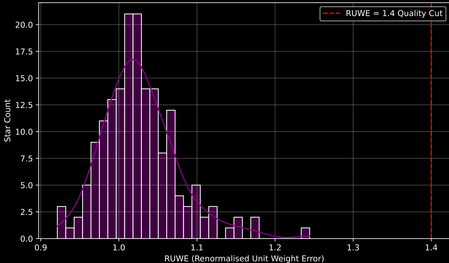
Gaia Cluster: [King_4] RUWE Distribution (n= 171)
