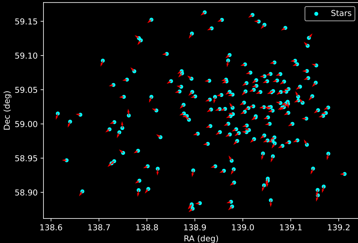
Gaia Cluster: [King_4] Proper Motion Vectors for Gaia Star Field (n= 171)
