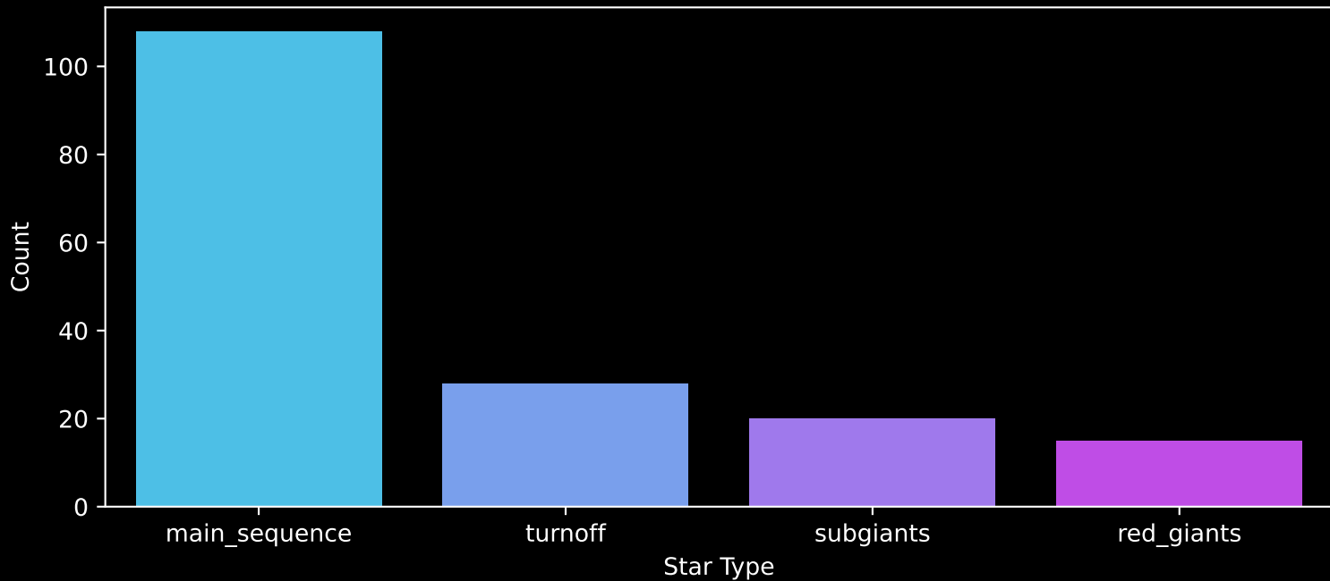
Gaia Cluster: [King_4] Count plot of Star Type
