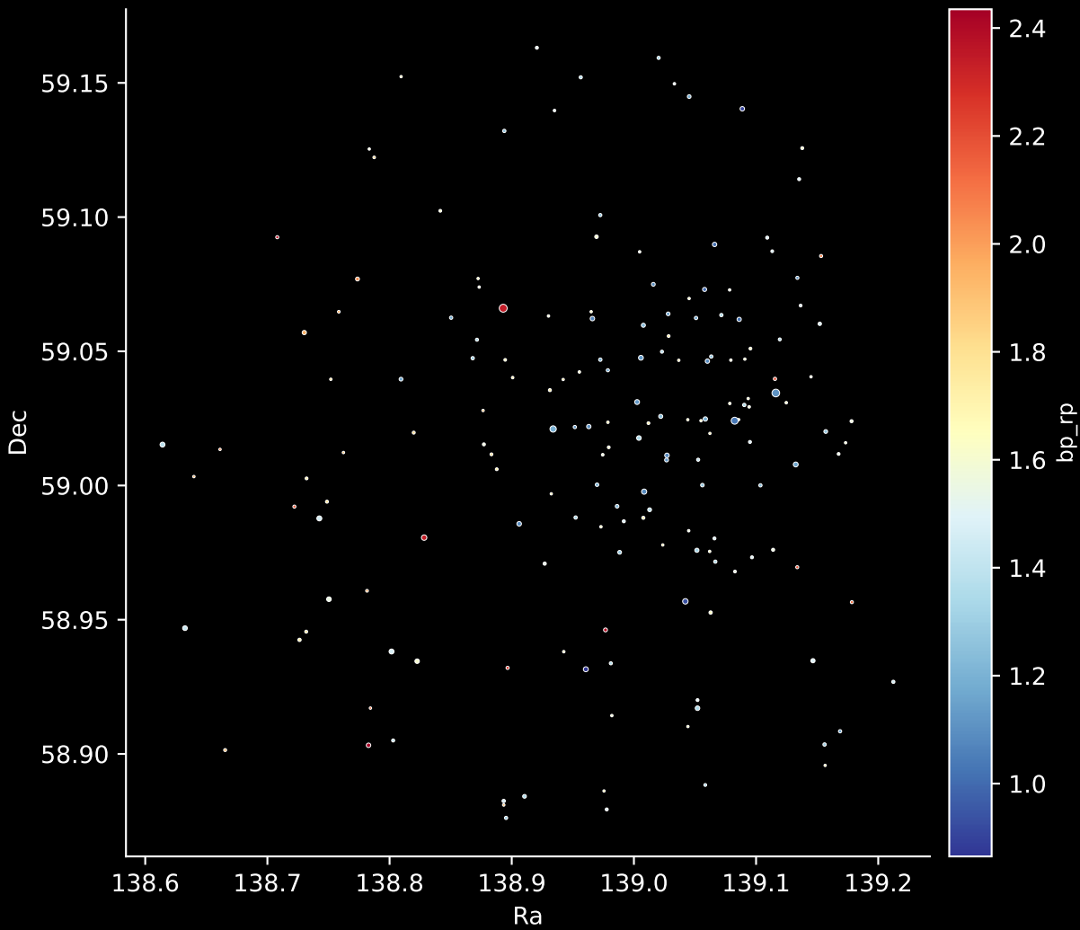
Gaia Cluster: [King_4] Stars: 171
