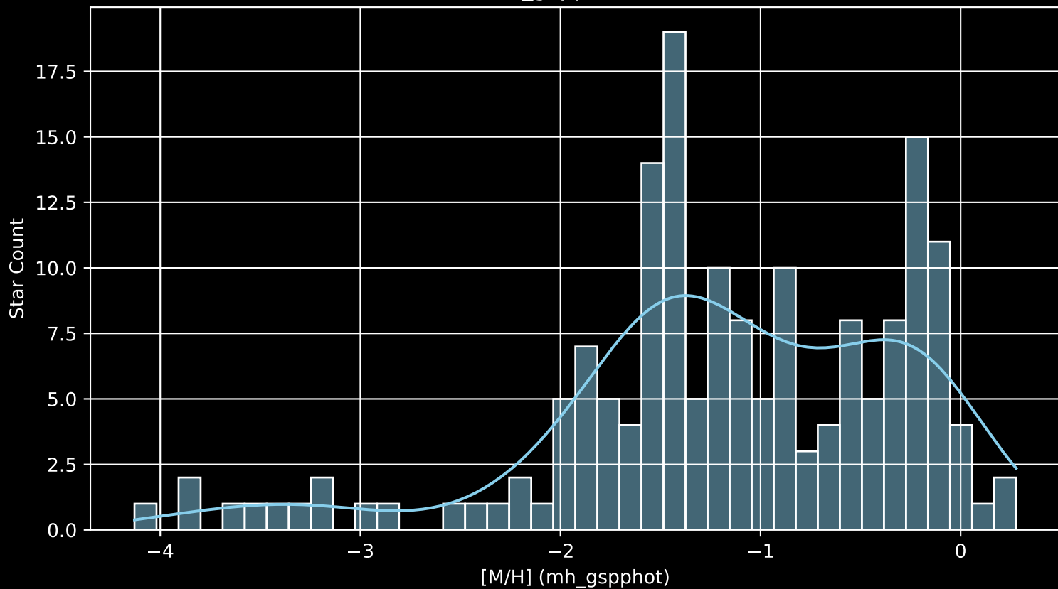
Gaia Cluster: [King_4 [M/H] (mh_gspphot) (n= 170)
