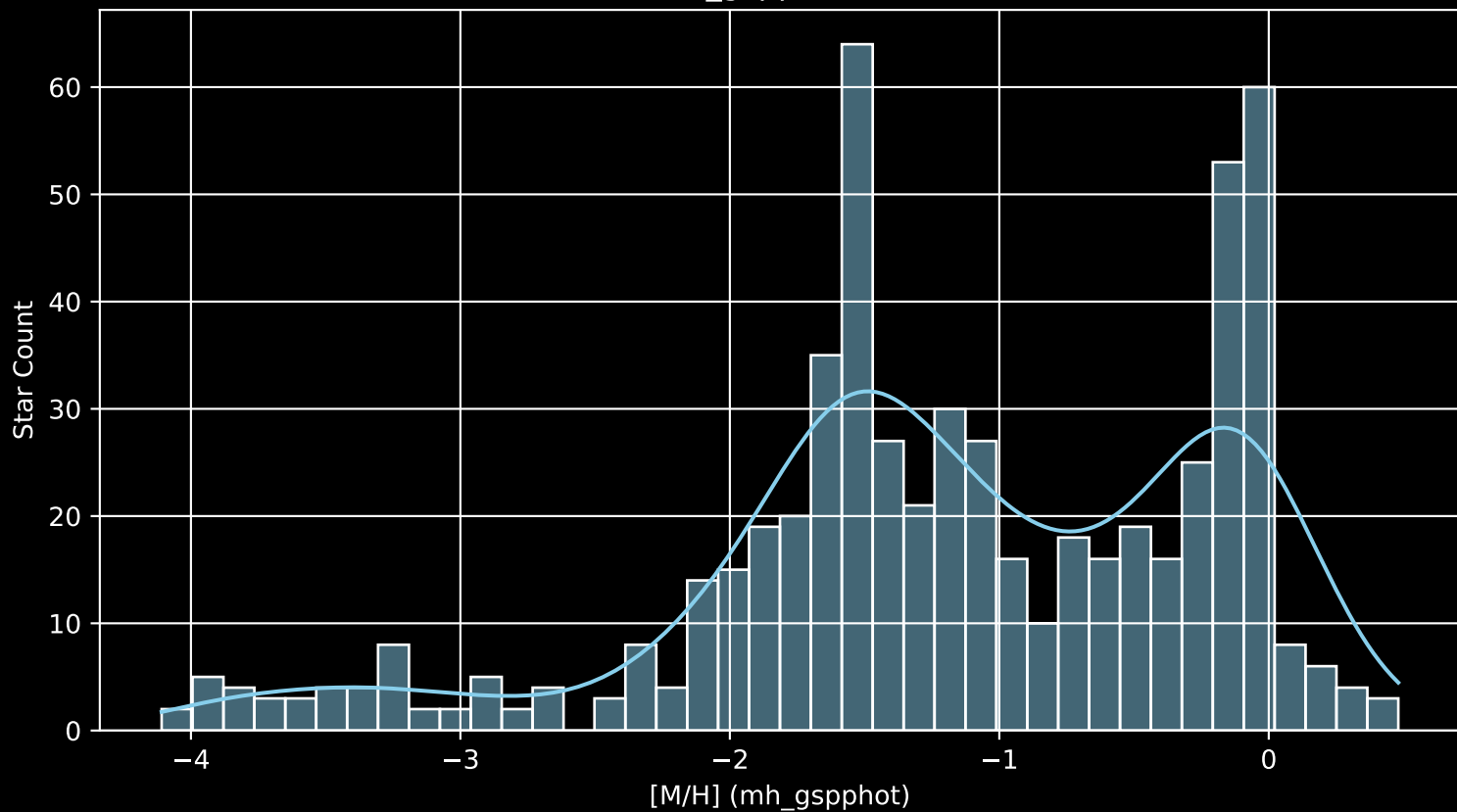
Gaia Cluster: [King_5 [M/H] (mh_gspphot) (n= 589)
