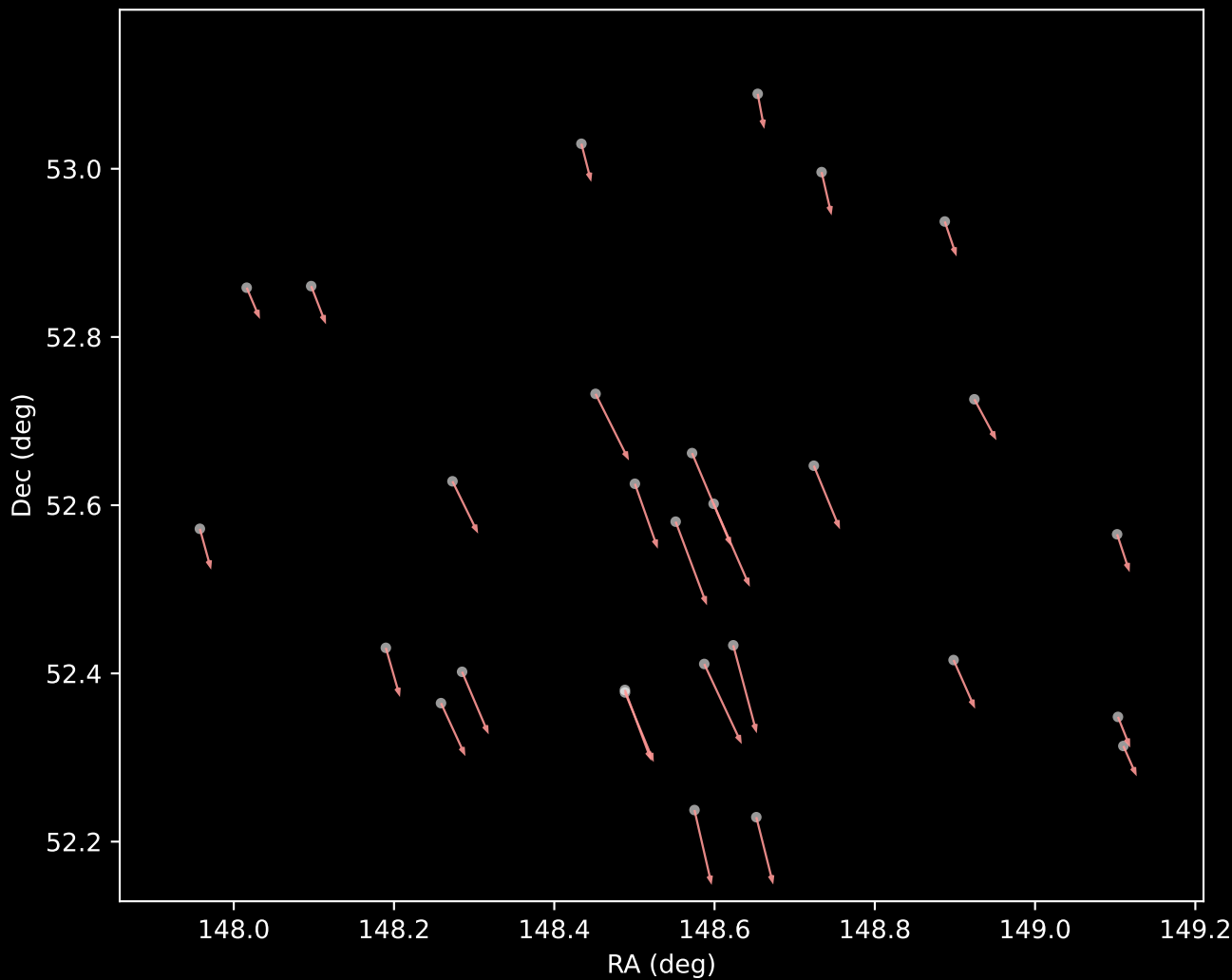
Gaia DR3 Cluster 7 Proper Motion Vectors (n=28)
