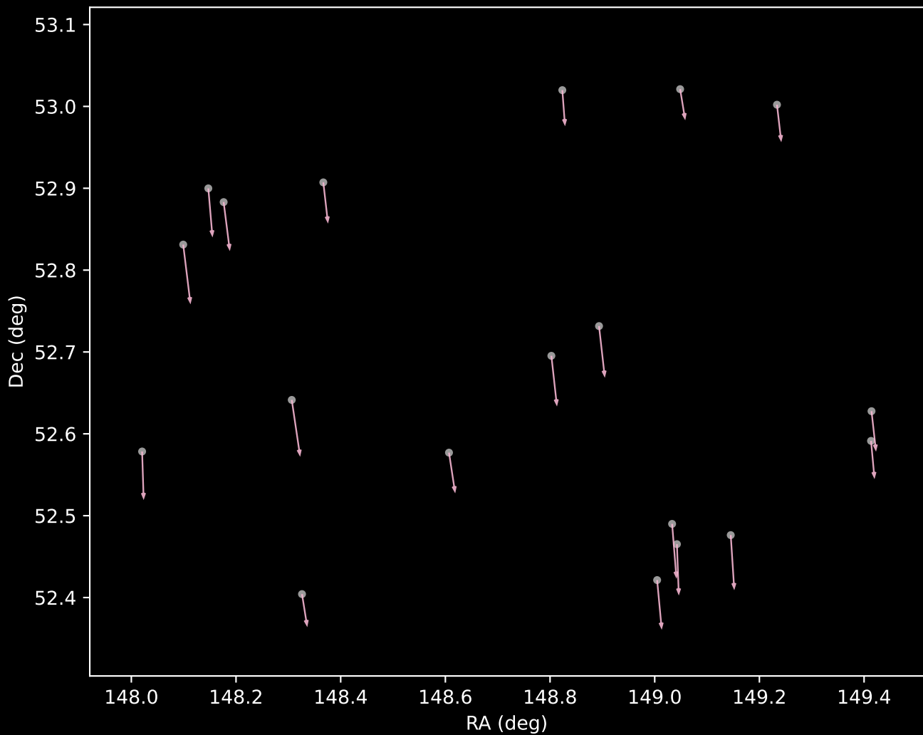
Gaia DR3 Cluster 13 Proper Motion Vectors (n=19)
