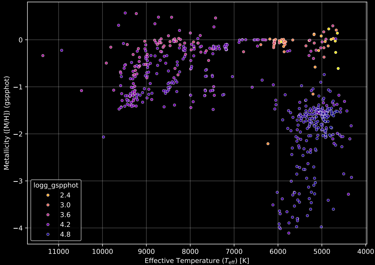
Gaia Cluster: [King_5] Stellar Population Parameters (n= 591)
