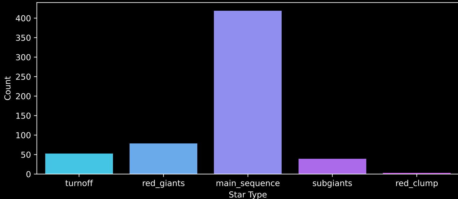
Gaia Cluster: [King_5] Count plot of Star Type
