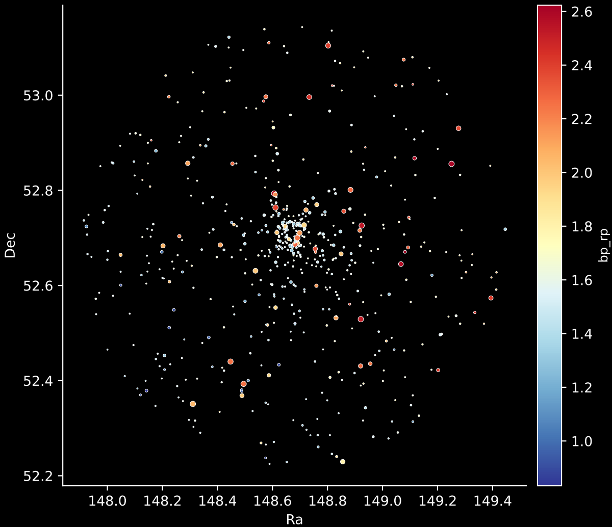
Gaia Cluster: [King_5] Stars: 591
