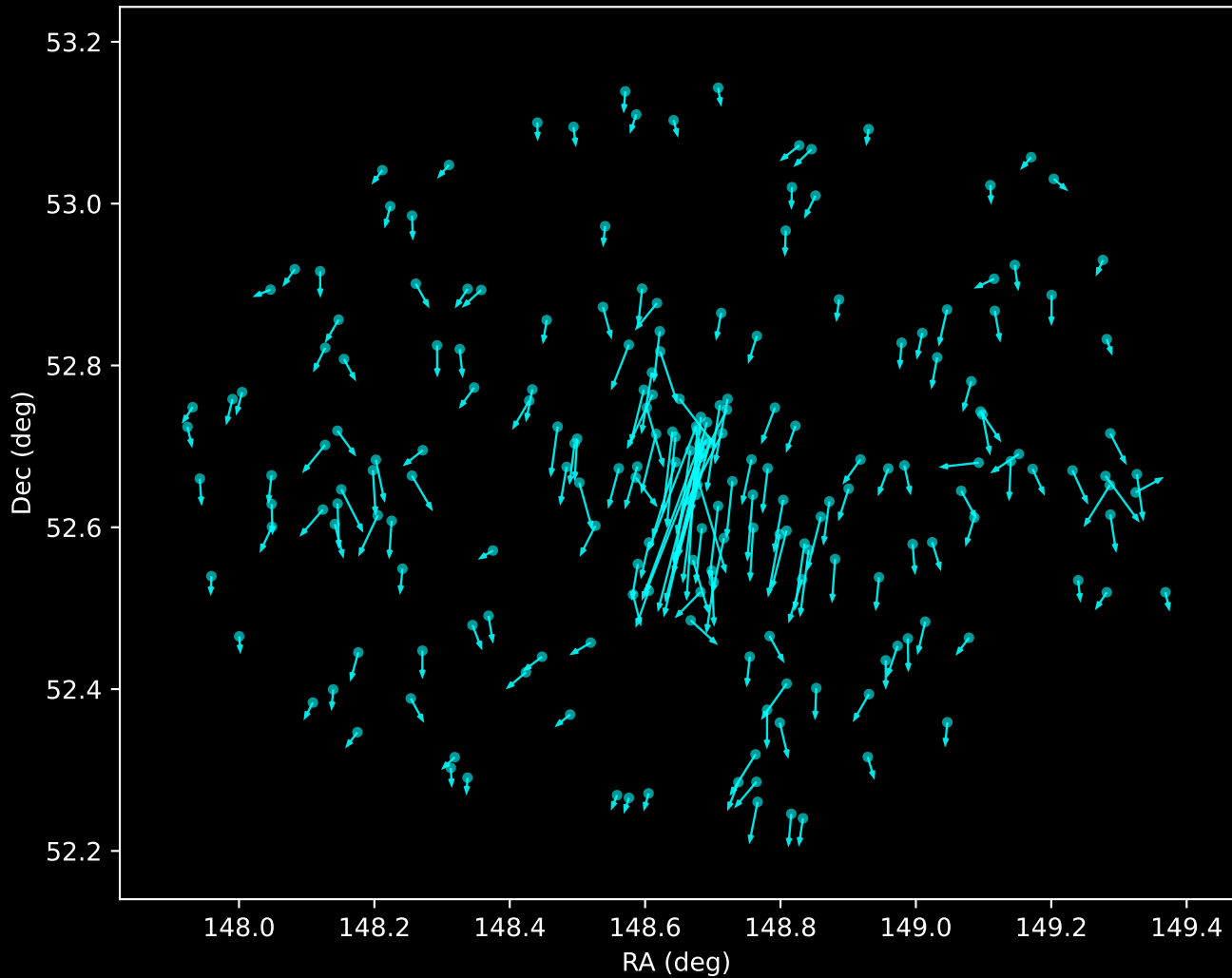
Gaia DR3 Noise Stream Proper Motion Vectors (n=207)
