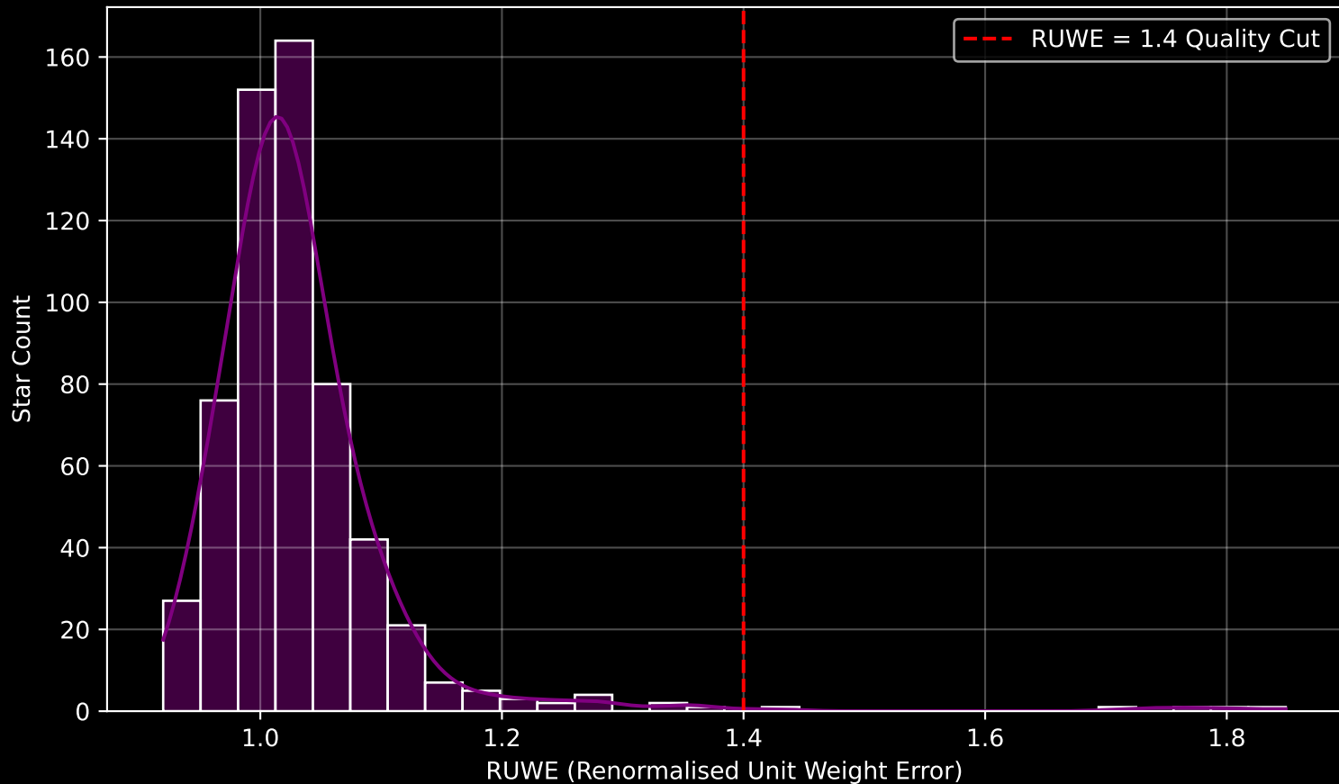
Gaia Cluster: [King_5] RUWE Distribution (n= 591)
