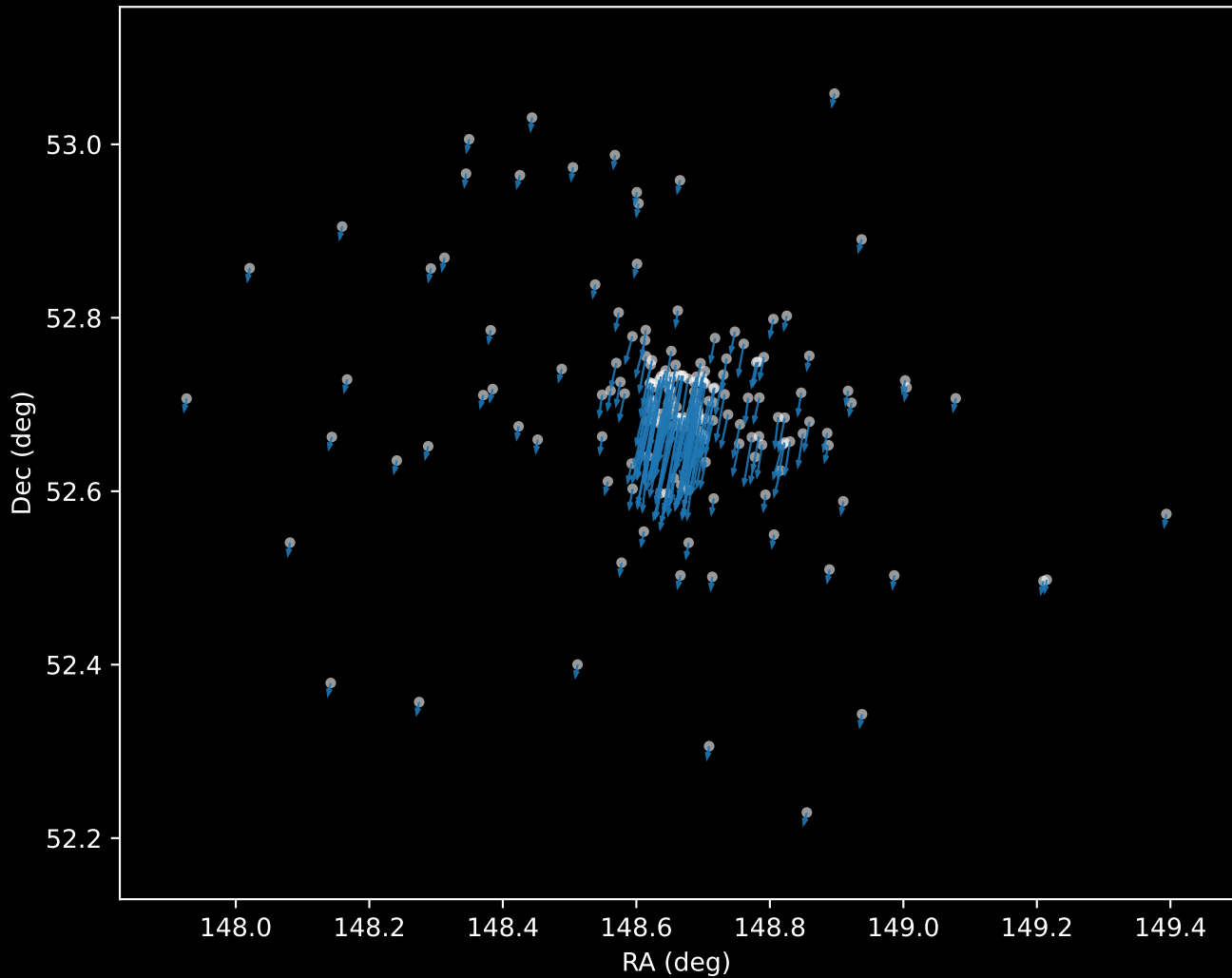
Gaia DR3 Cluster 20 Proper Motion Vectors (n=178)
