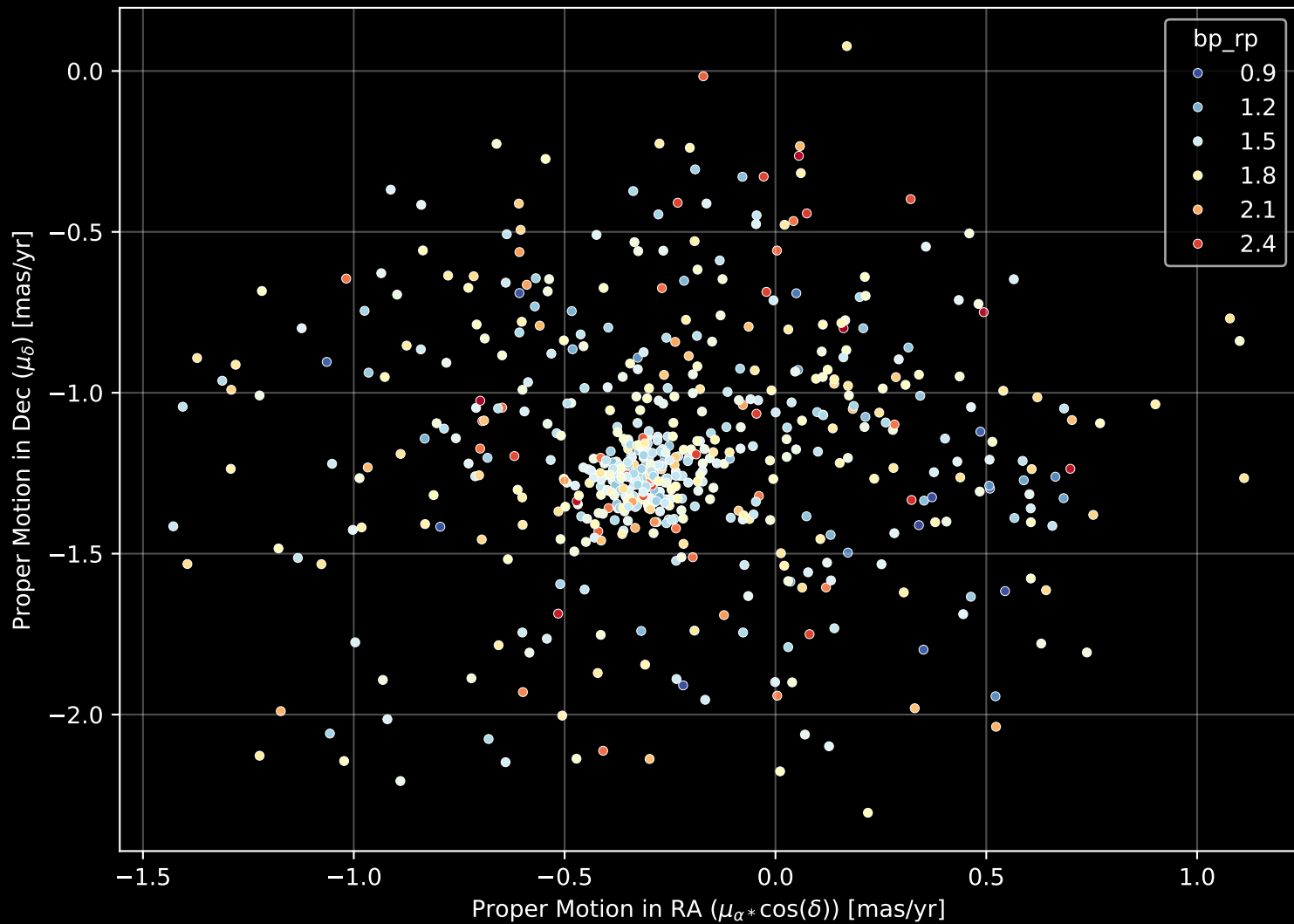
Gaia Cluster: [King_5] Proper Motion Diagram (n= 591)
