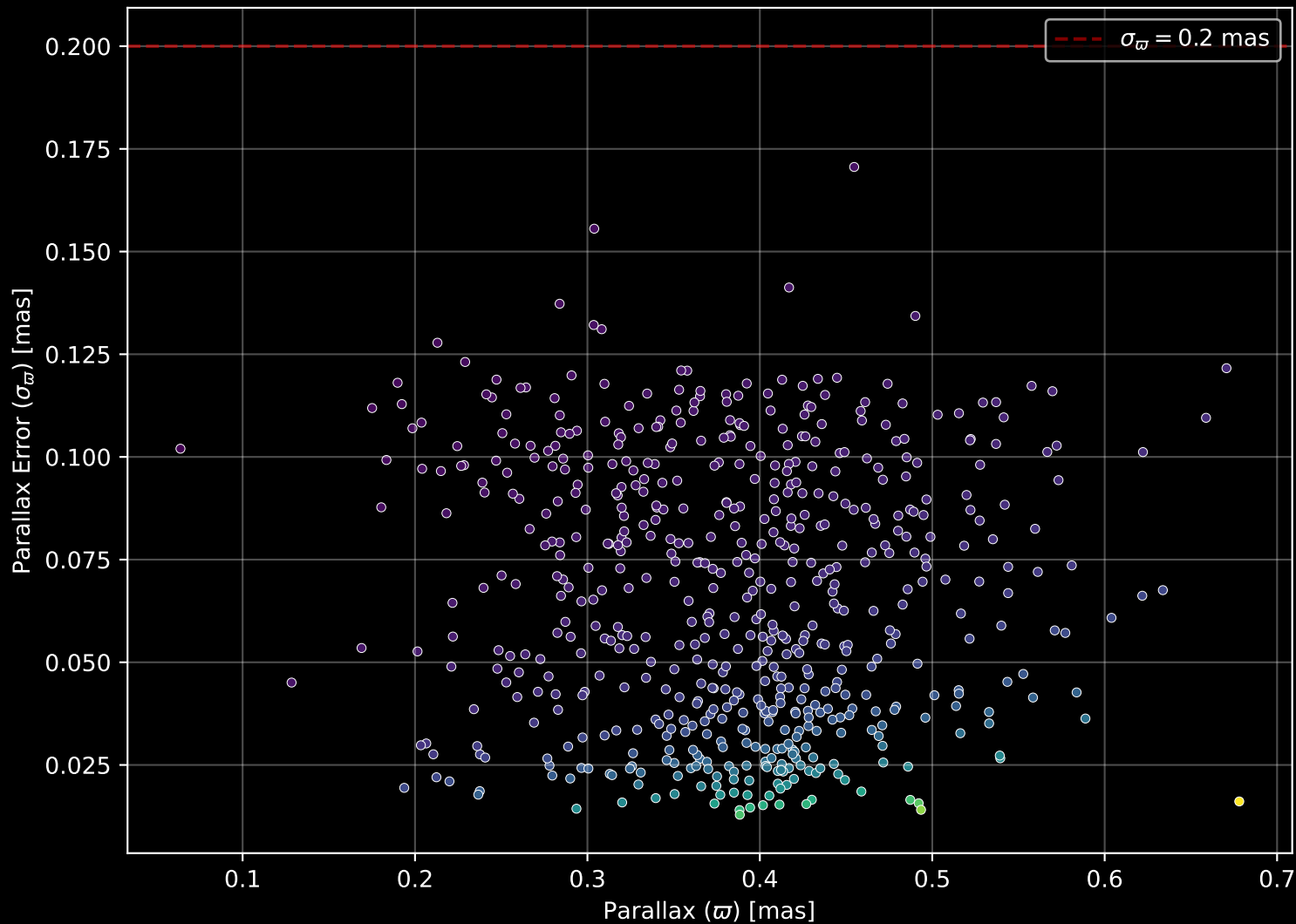
Gaia Cluster: [King_5] Parallax Quality (n= 591)
