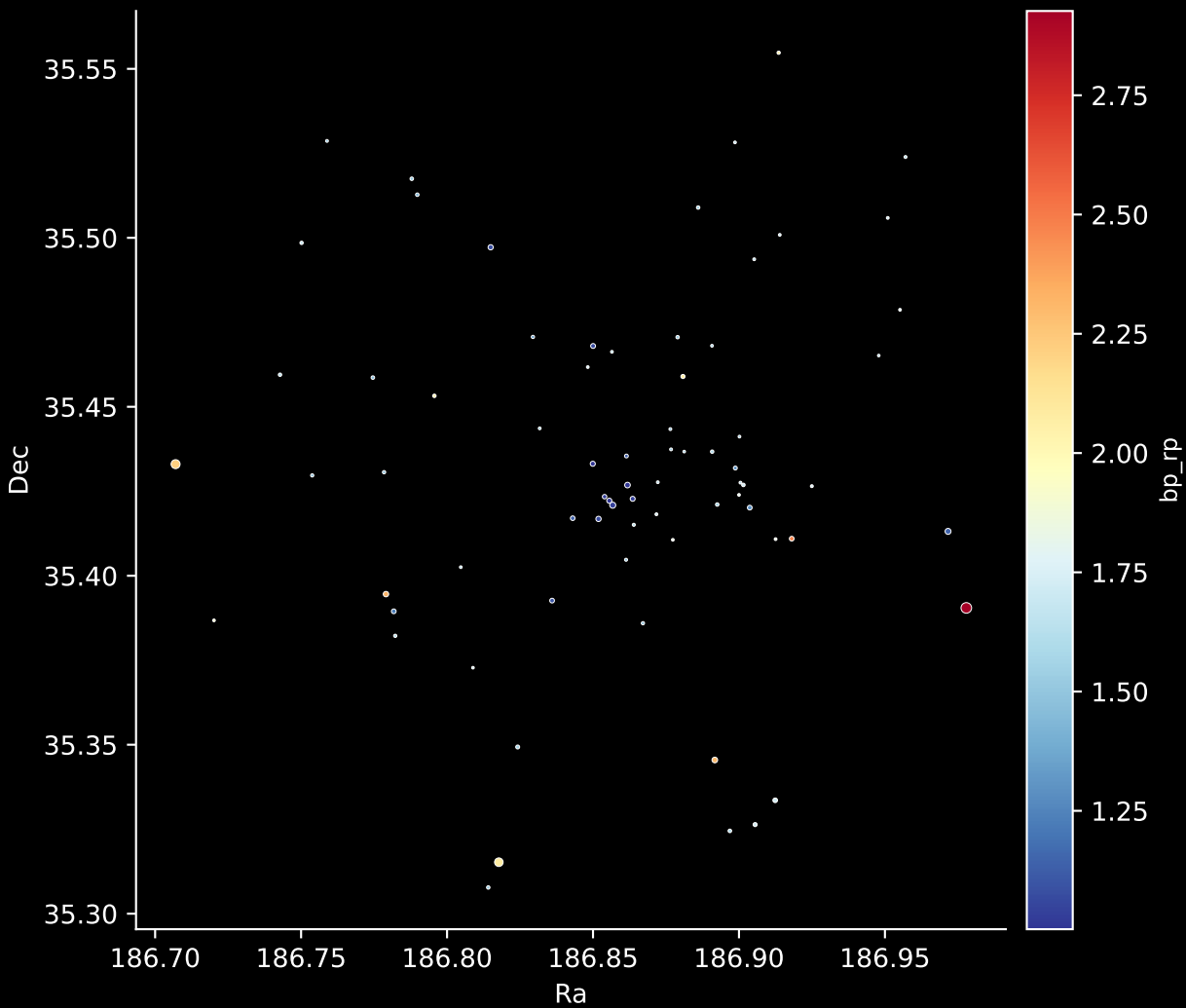
Gaia Cluster: [Koposov_10] Stars: 73
