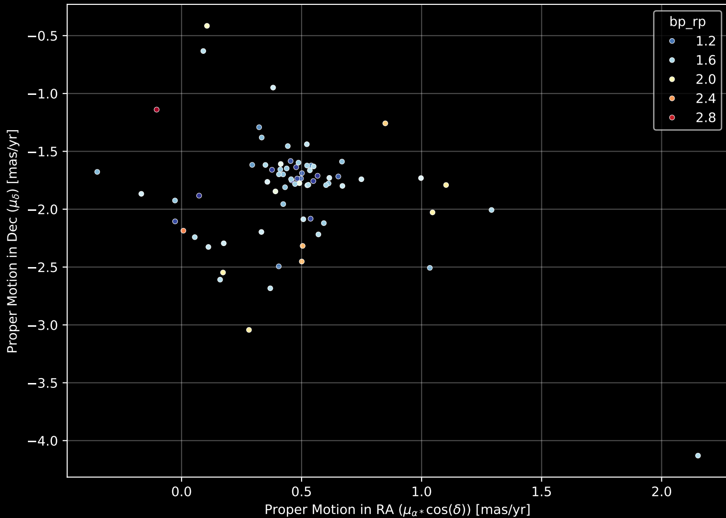
Gaia Cluster: [Koposov_10] Proper Motion Diagram (n= 73)
