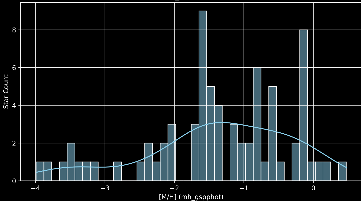
Gaia Cluster: [Koposov_10 [M/H] (mh_gspphot) (n= 73)
