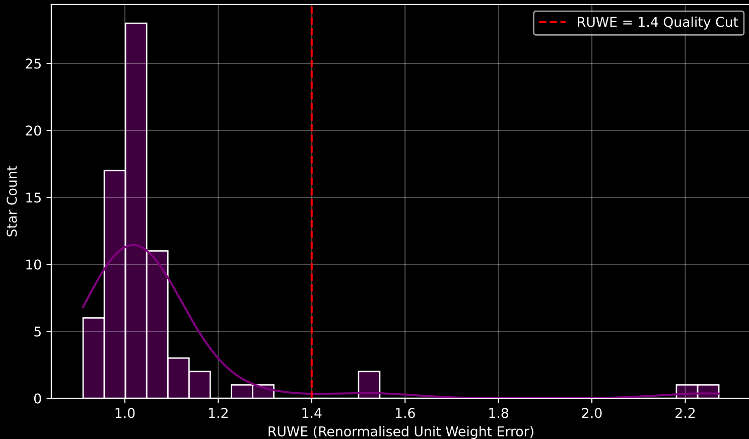
Gaia Cluster: [Koposov_10] RUWE Distribution (n= 73)
