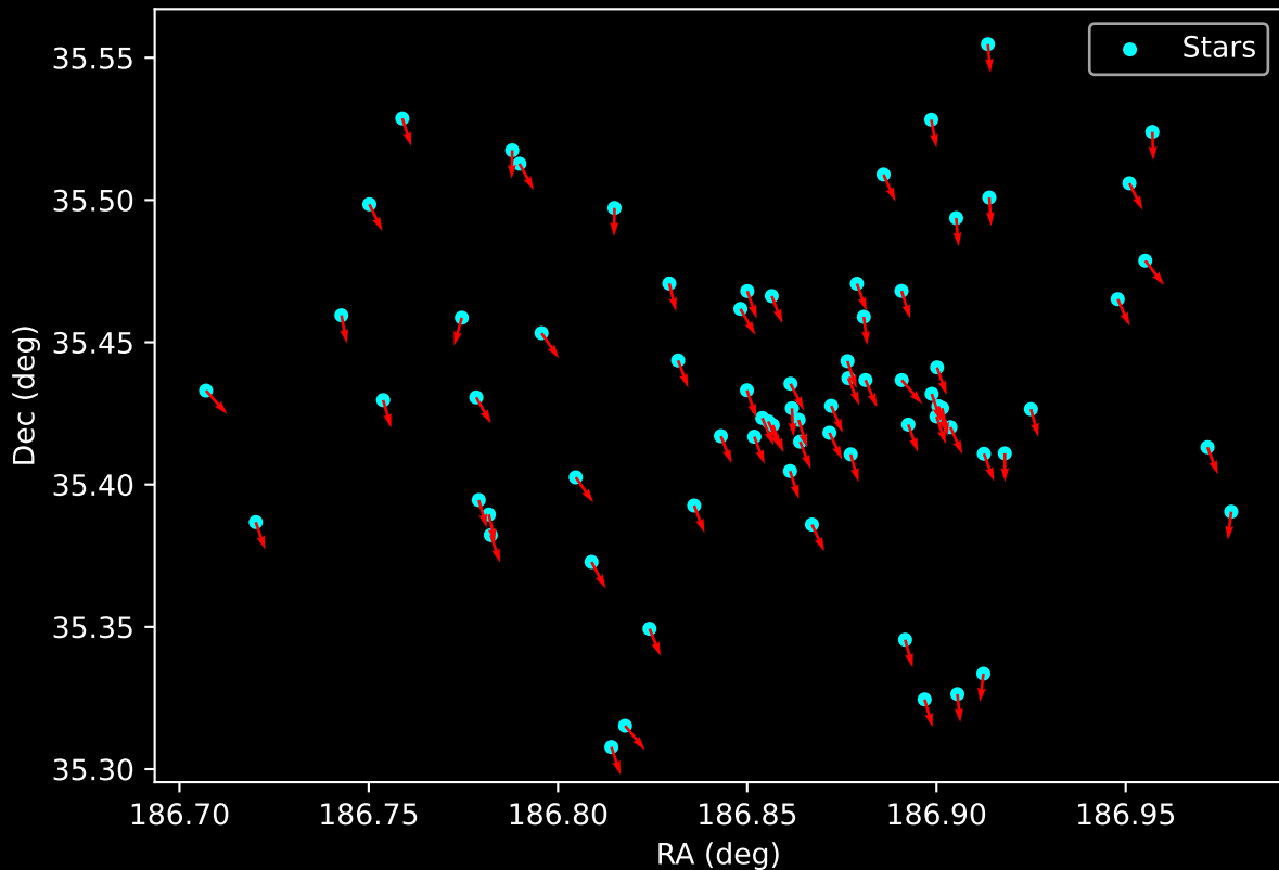
Gaia Cluster: [Koposov_10] Proper Motion Vectors for Gaia Star Field (n= 73)
