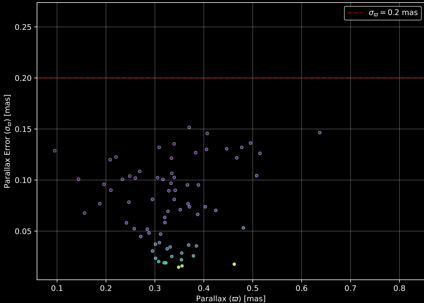
Gaia Cluster: [Koposov_10] Parallax Quality (n= 73)
