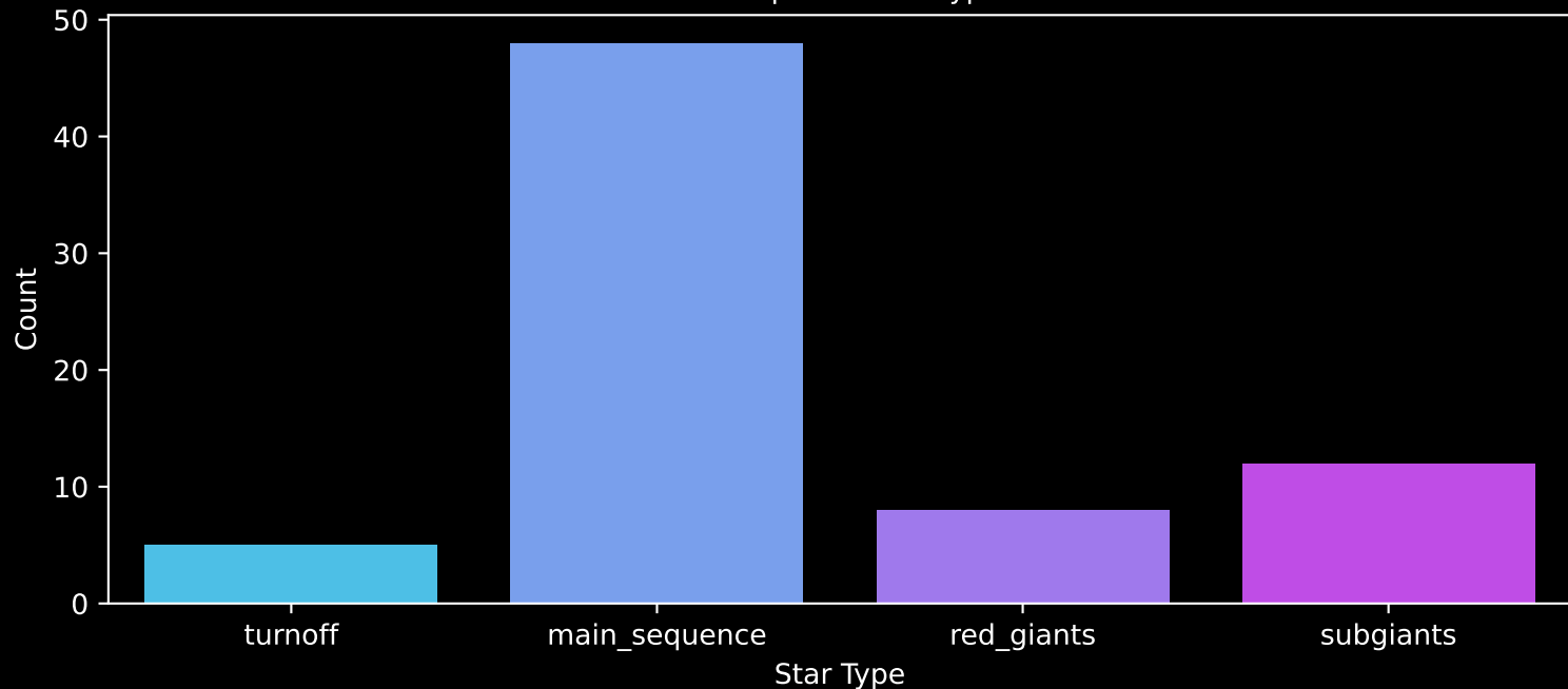
Gaia Cluster: [Koposov_10] Count plot of Star Type
