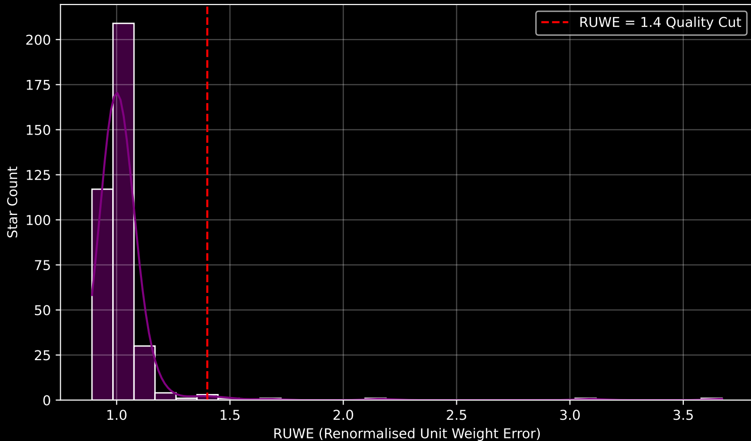
Gaia Cluster: [Koposov_12] RUWE Distribution (n= 369)
