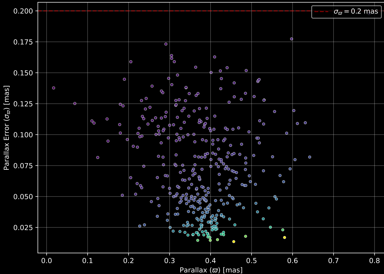
Gaia Cluster: [Koposov_12] Parallax Quality (n= 369)
