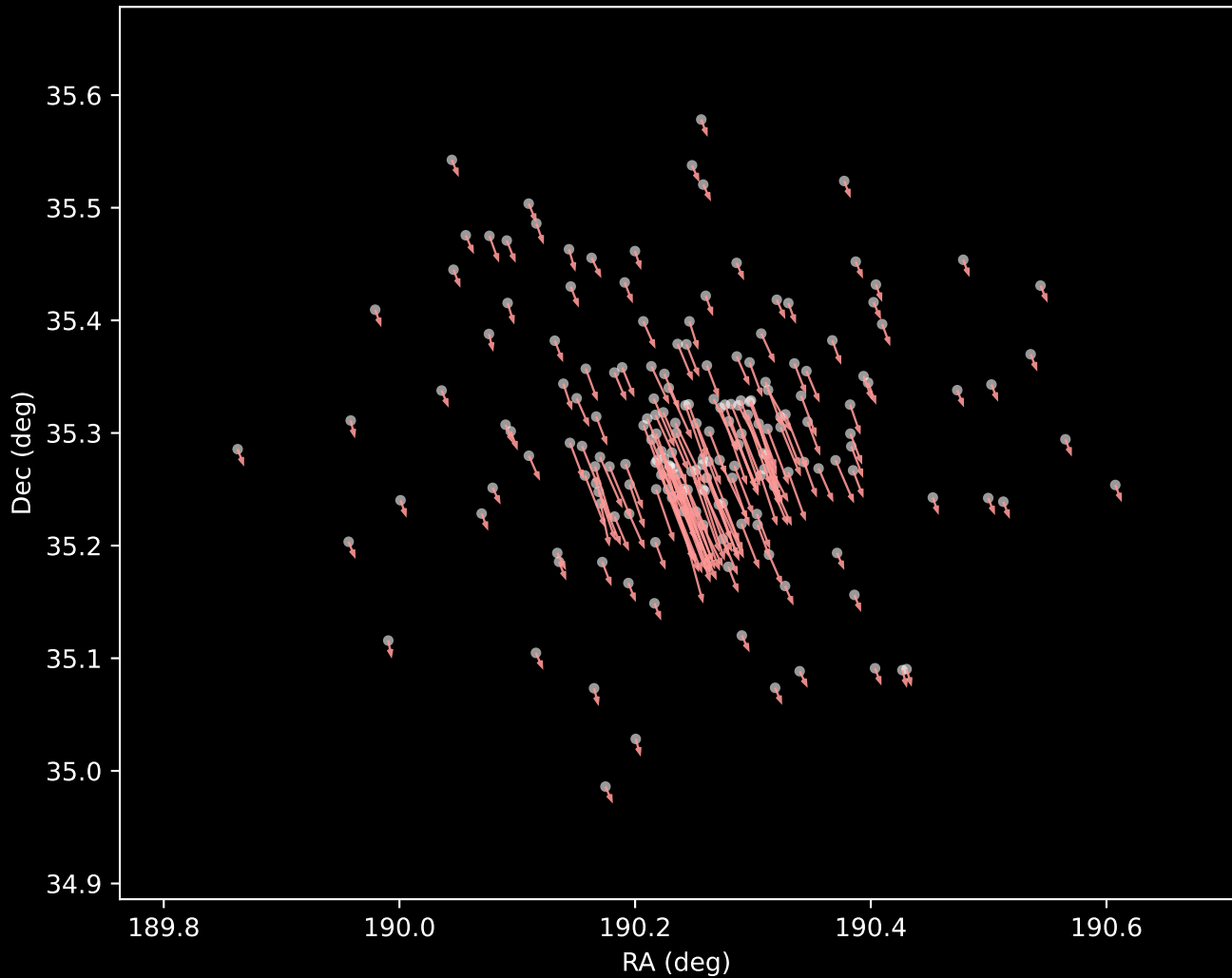
Gaia DR3 Cluster 7 Proper Motion Vectors (n=188)
