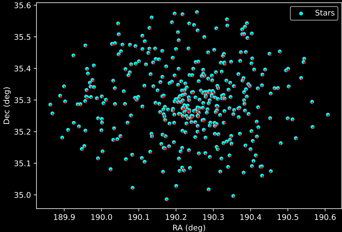
Gaia Cluster: [Koposov_12] Proper Motion Vectors for Gaia Star Field (n= 369)
