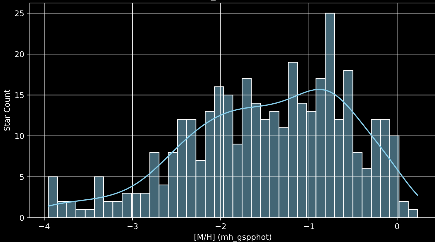
Gaia Cluster: [Koposov_12 [M/H] (mh_gspphot) (n= 369)
