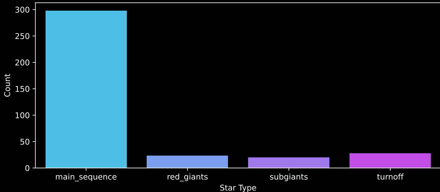
Gaia Cluster: [Koposov_12] Count plot of Star Type
