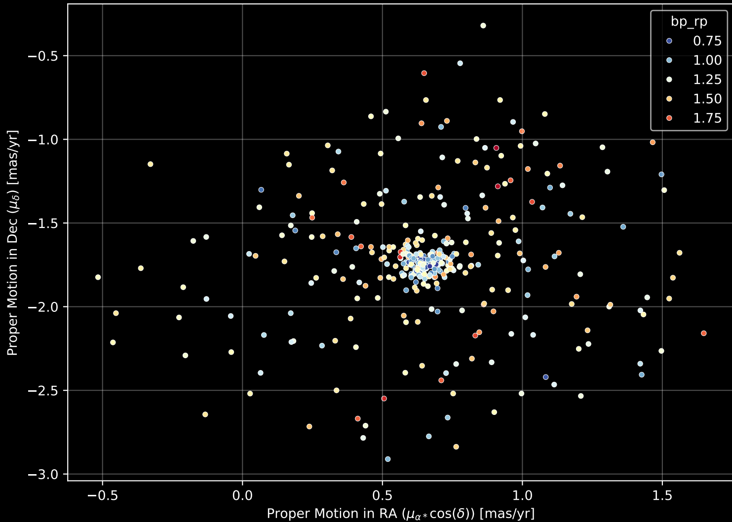
Gaia Cluster: [Koposov_12] Proper Motion Diagram (n= 369)
