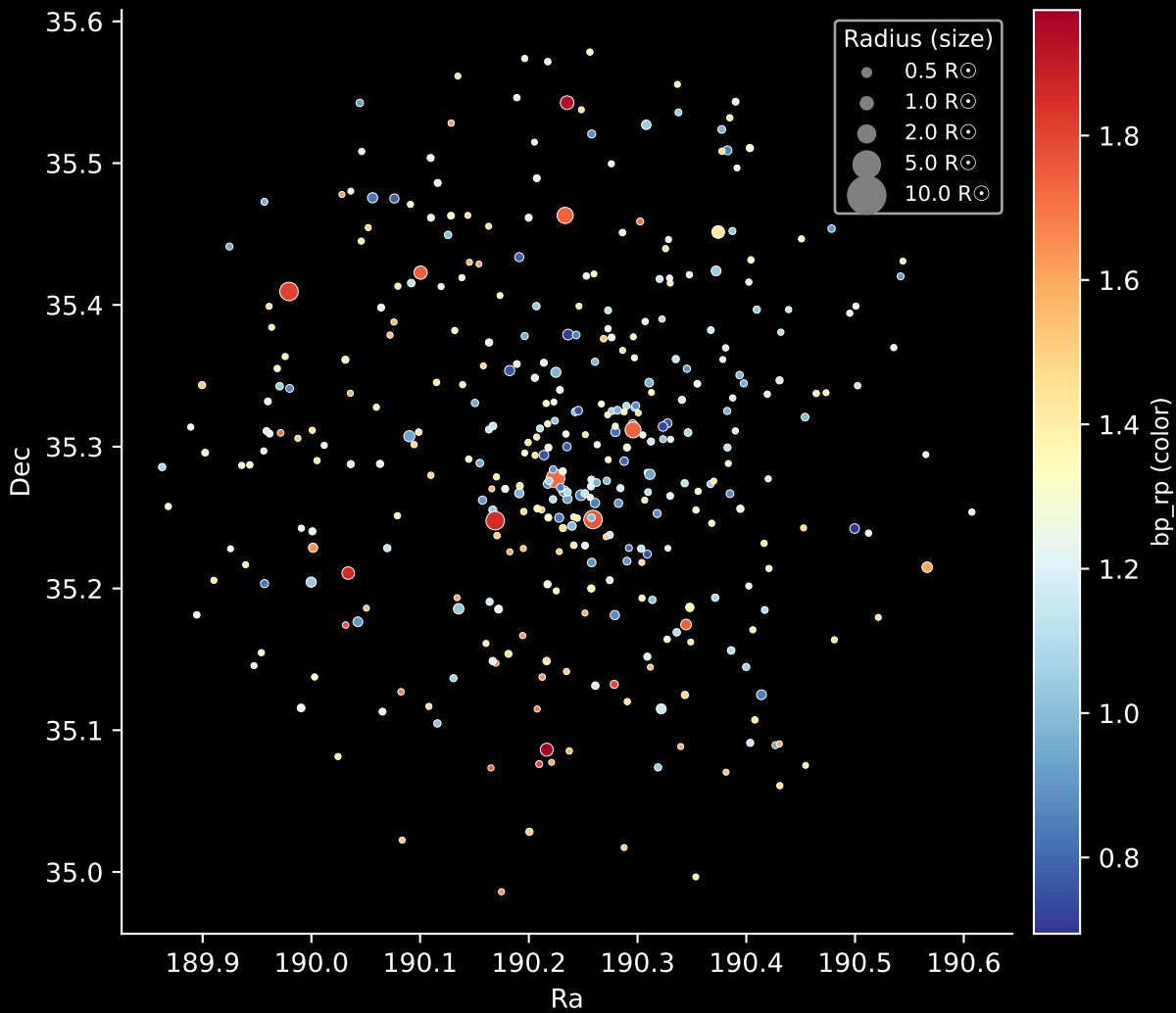
Gaia Cluster: [Koposov_12] Stars: 369
