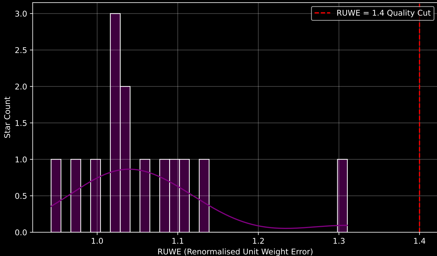
Gaia Cluster: [Kronberger_25] RUWE Distribution (n= 14)
