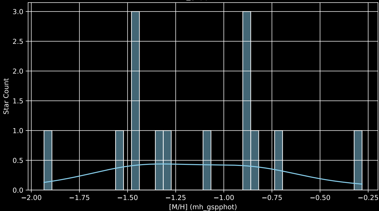
Gaia Cluster: [Kronberger_25 [M/H] (mh_gspphot) (n= 14)
