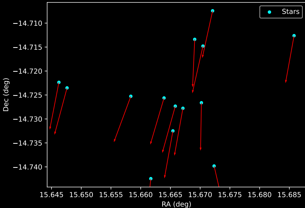
Gaia Cluster: [Kronberger_25] Proper Motion Vectors for Gaia Star Field (n= 14)
