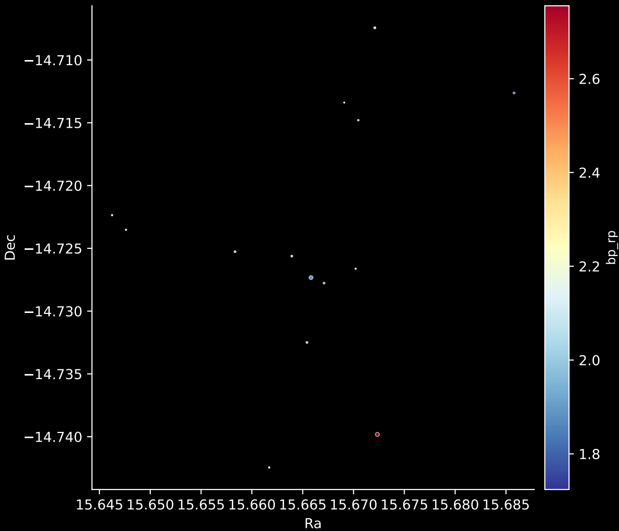
Gaia Cluster: [Kronberger_25] Stars: 14
