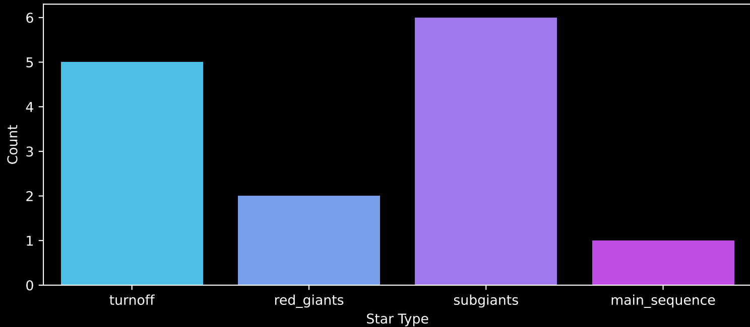
Gaia Cluster: [Kronberger_25] Count plot of Star Type
