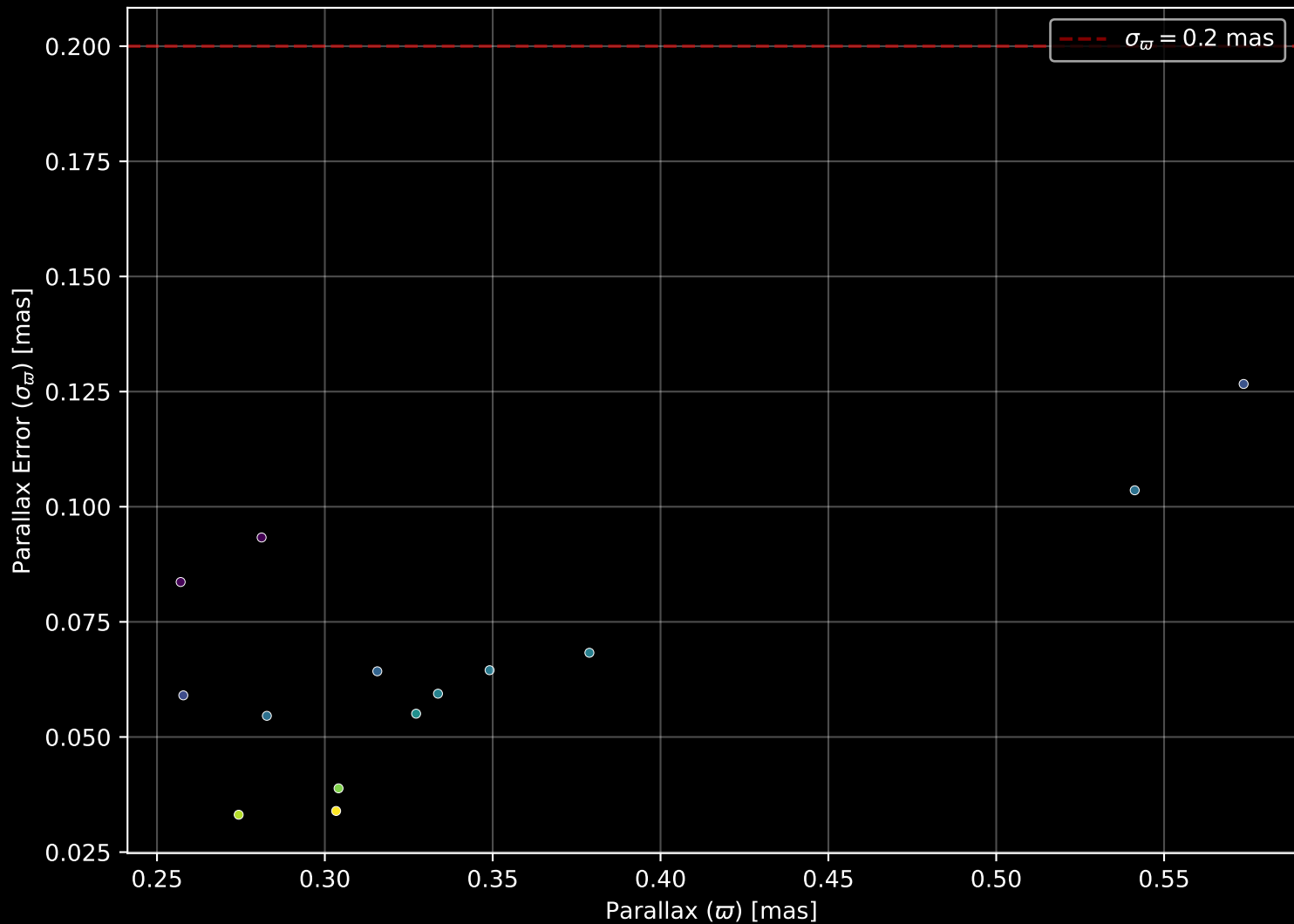
Gaia Cluster: [Kronberger_25] Parallax Quality (n= 14)
