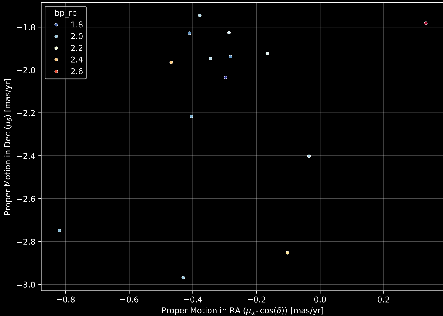
Gaia Cluster: [Kronberger_25] Proper Motion Diagram (n= 14)
