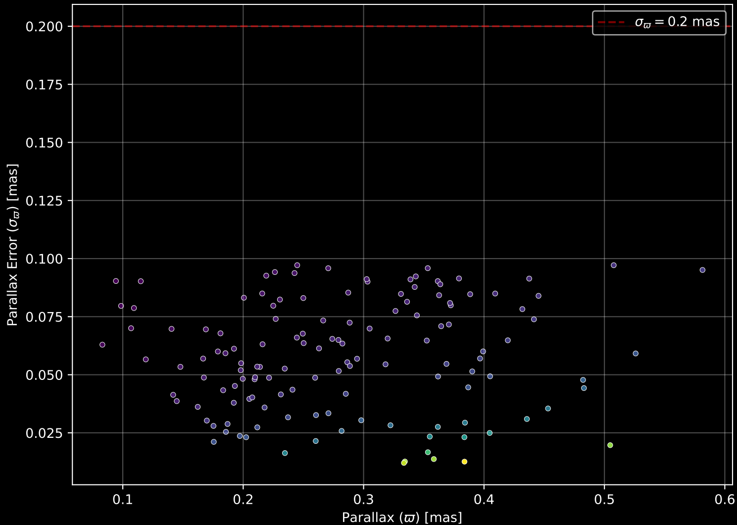
Gaia Cluster: [Kronberger_69] Parallax Quality (n= 134)
