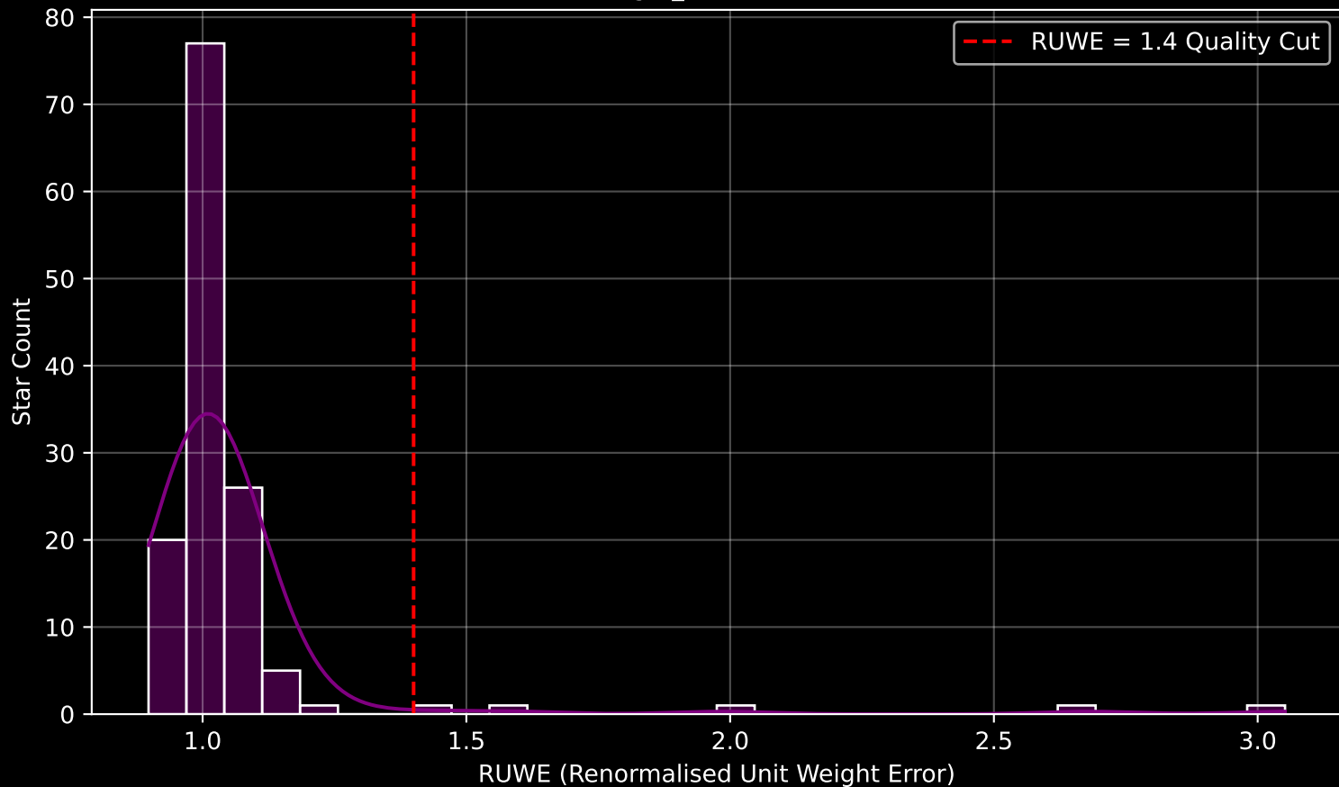
Gaia Cluster: [Kronberger_69] RUWE Distribution (n= 134)
