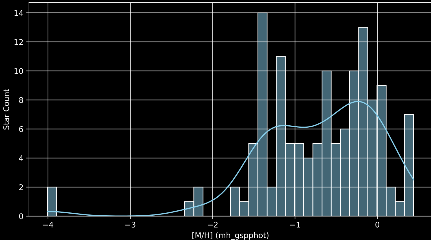
Gaia Cluster: [Kronberger_69 [M/H] (mh_gspphot) (n= 130)
