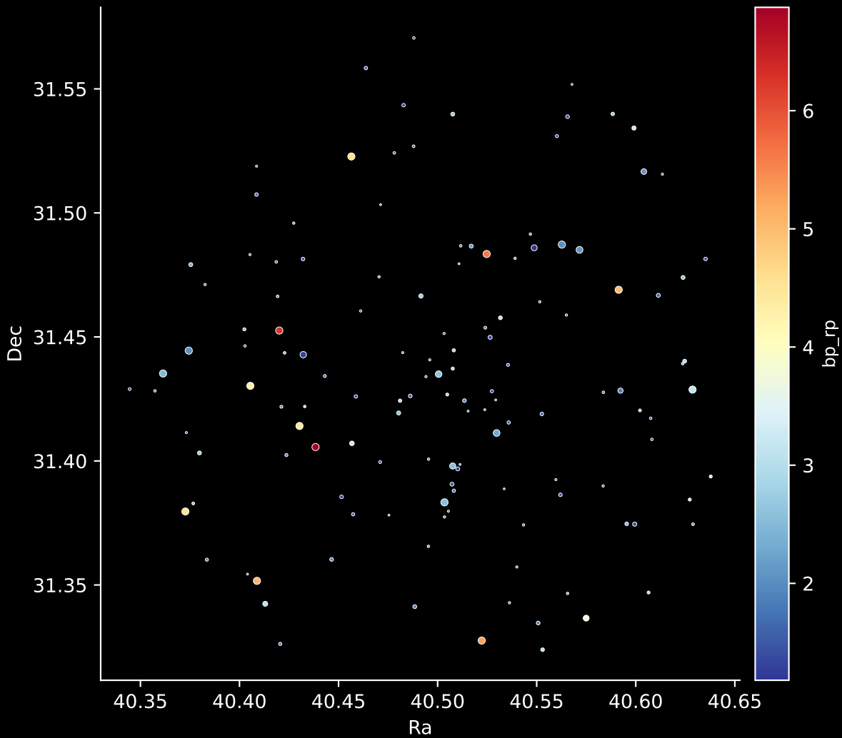
Gaia Cluster: [Kronberger_69] Stars: 134
