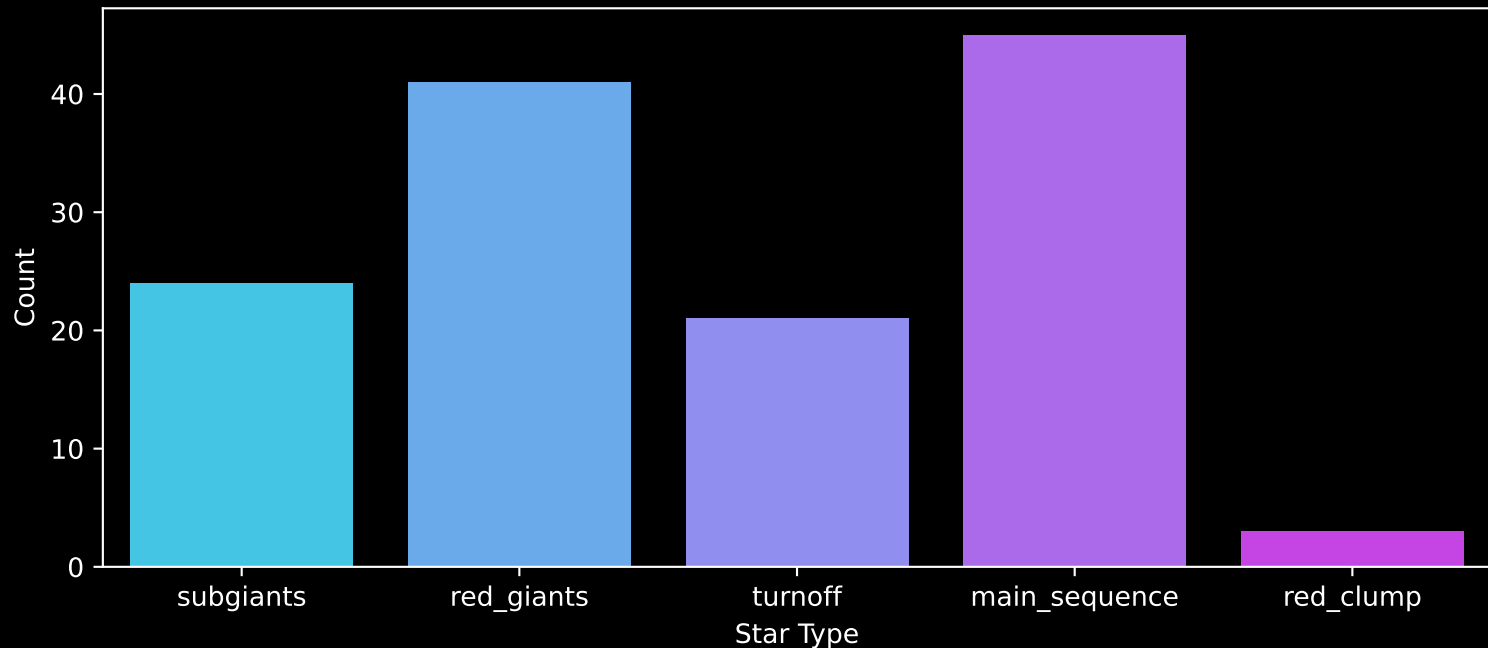
Gaia Cluster: [Kronberger_69] Count plot of Star Type
