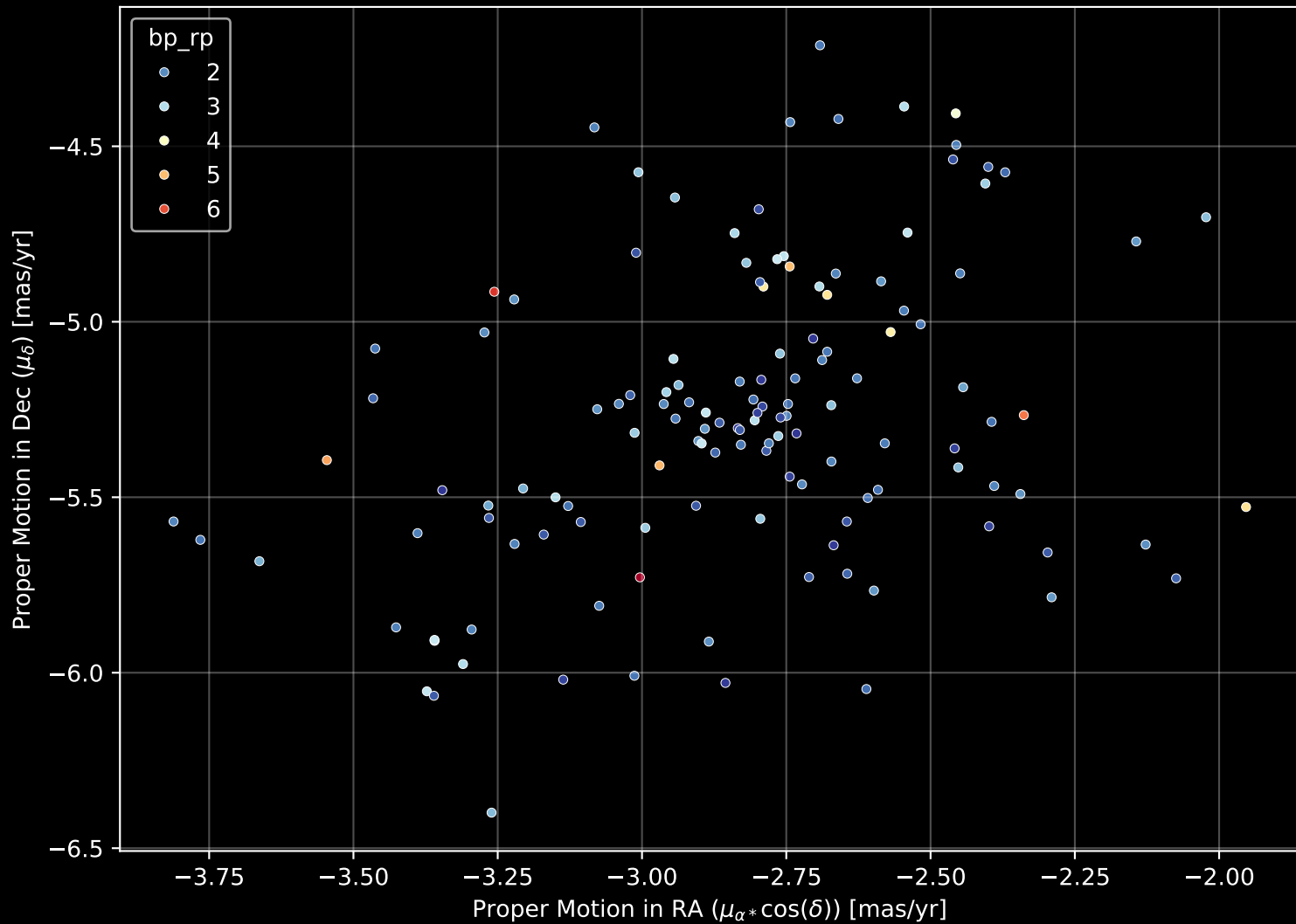
Gaia Cluster: [Kronberger_69] Proper Motion Diagram (n= 134)
