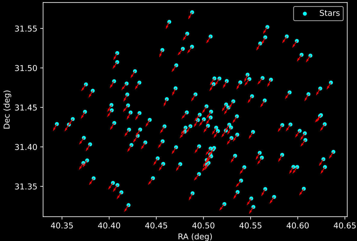
Gaia Cluster: [Kronberger_69] Proper Motion Vectors for Gaia Star Field (n= 134)
