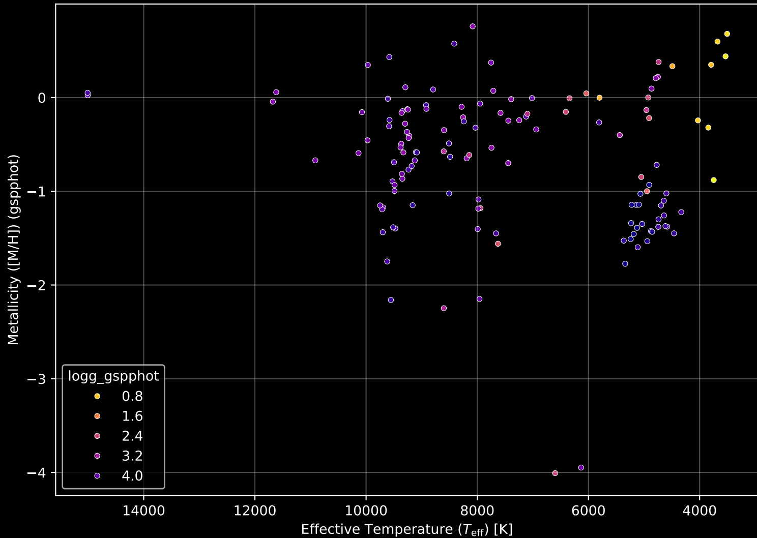
Gaia Cluster: [Kronberger_69] Stellar Population Parameters (n= 134)
