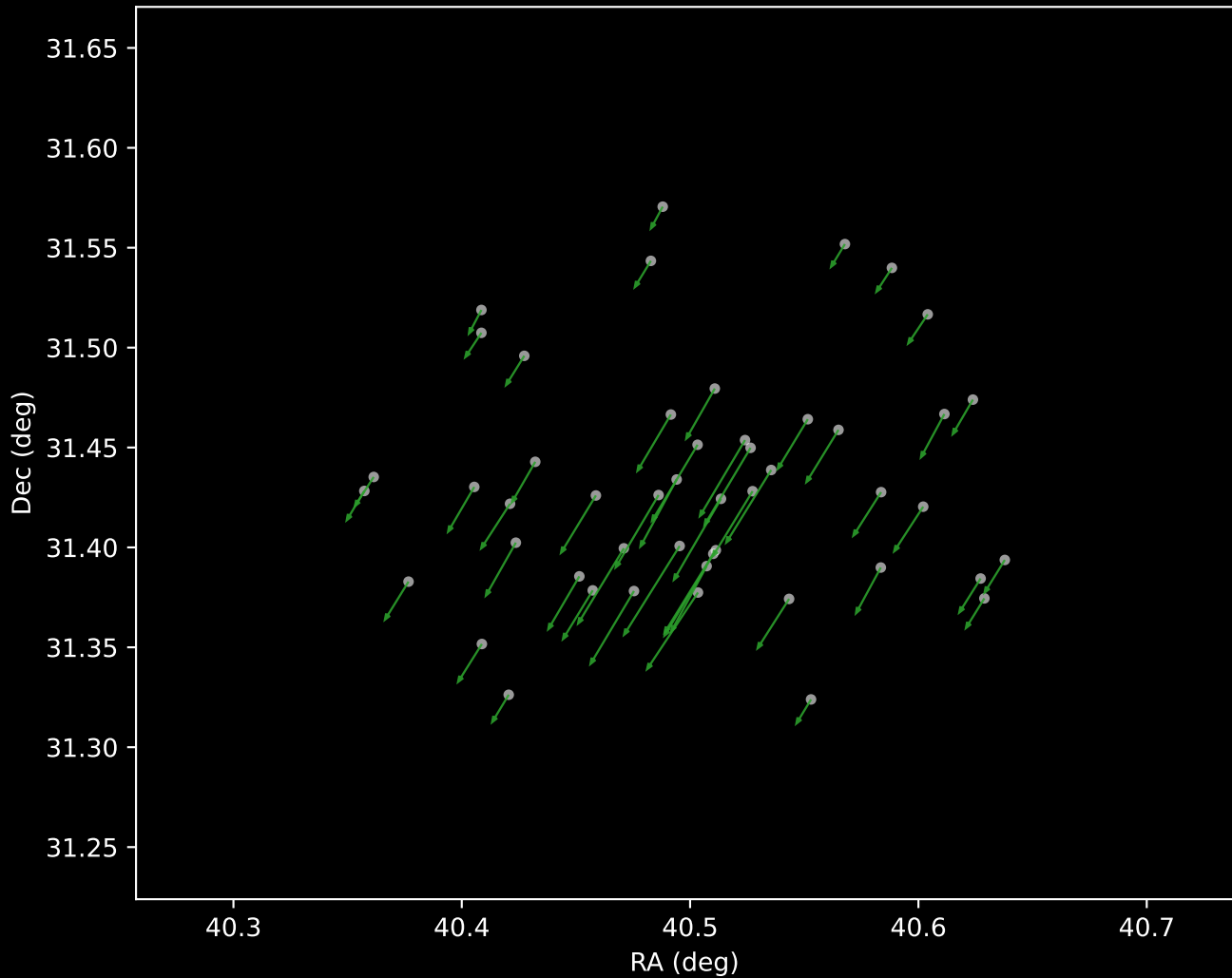
Gaia DR3 Cluster 4 Proper Motion Vectors (n=49)
