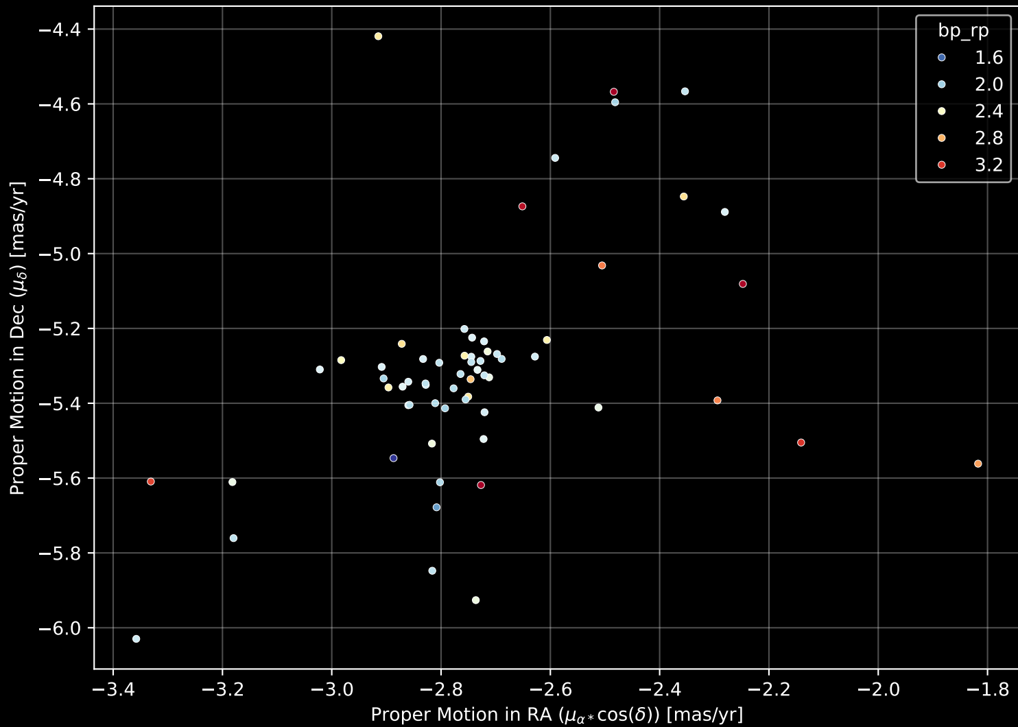
Gaia Cluster: [Kronberger_79] Proper Motion Diagram (n= 63)
