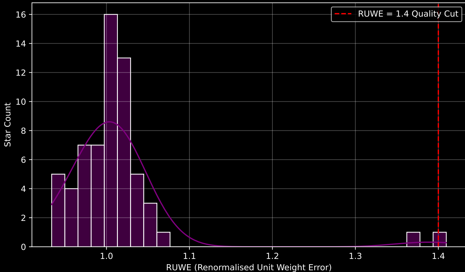
Gaia Cluster: [Kronberger_79] RUWE Distribution (n= 63)
