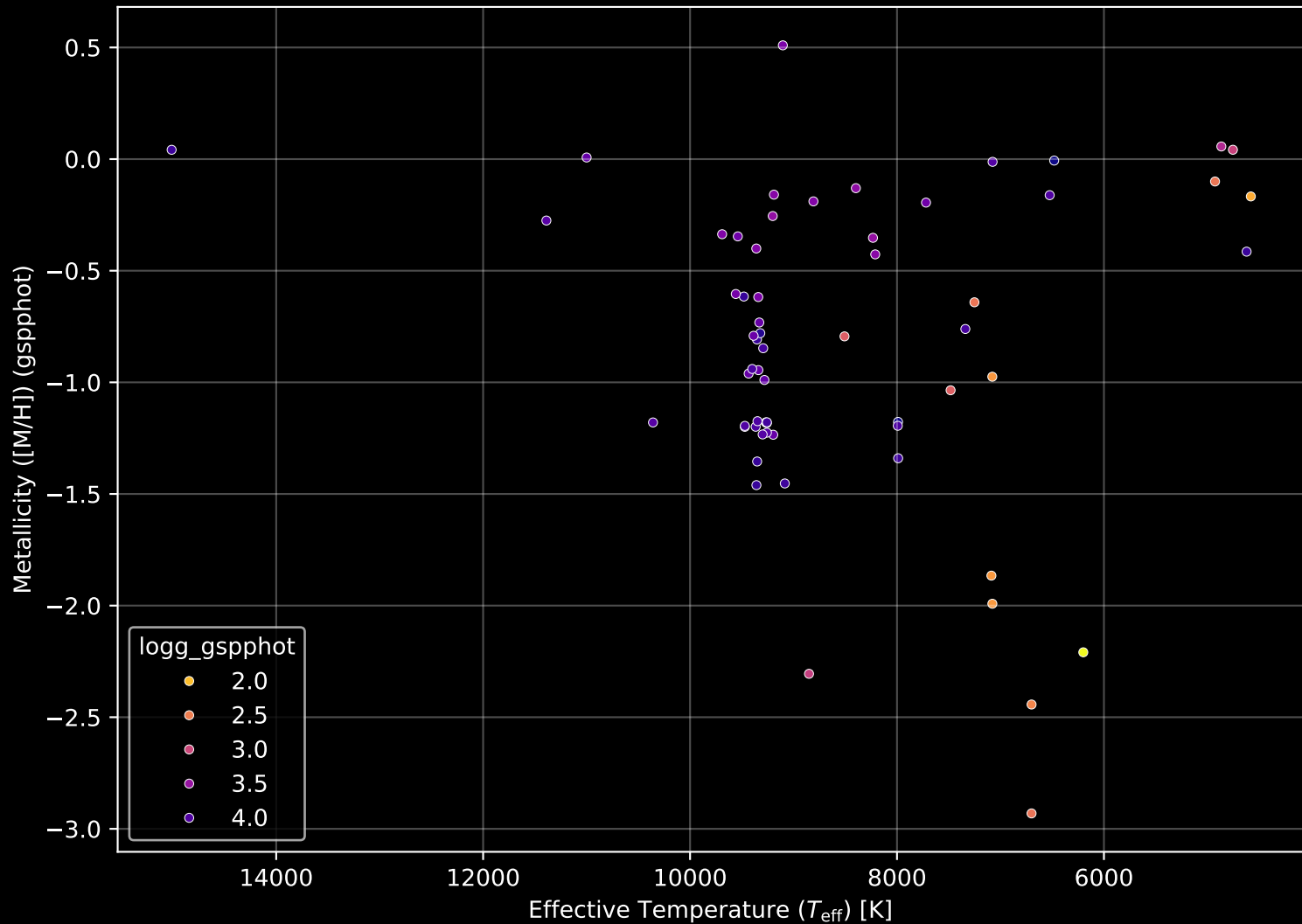
Gaia Cluster: [Kronberger_79] Stellar Population Parameters (n= 63)
