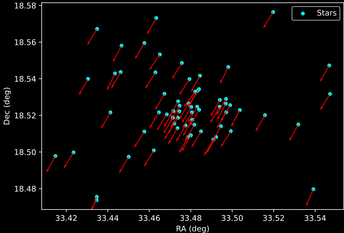
Gaia Cluster: [Kronberger_79] Proper Motion Vectors for Gaia Star Field (n= 63)
