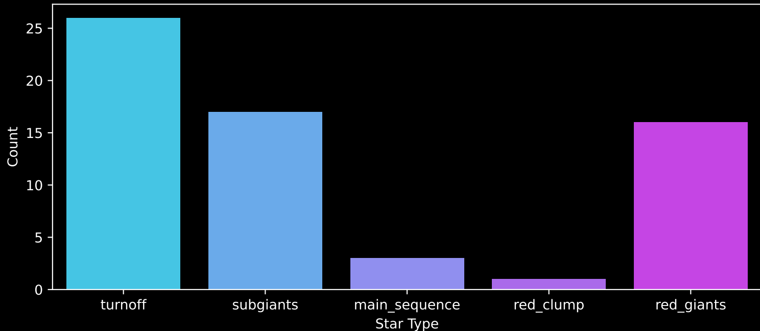
Gaia Cluster: [Kronberger_79] Count plot of Star Type
