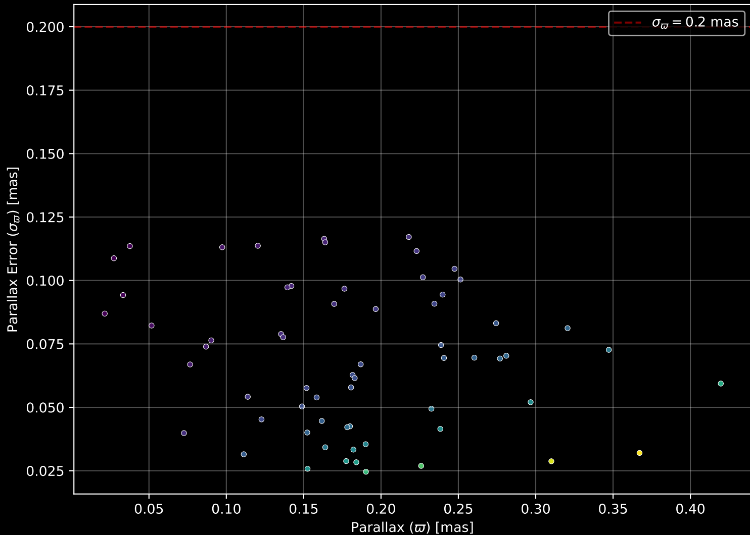
Gaia Cluster: [Kronberger_79] Parallax Quality (n= 63)
