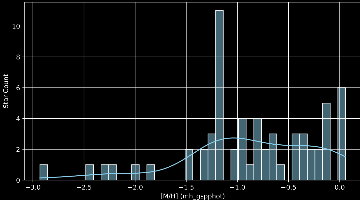
Gaia Cluster: [Kronberger_79 [M/H] (mh_gspphot) (n= 62)
