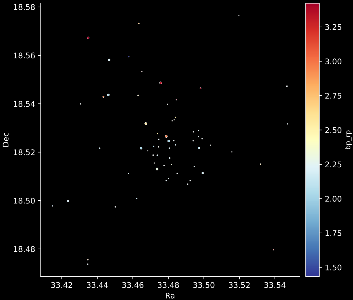
Gaia Cluster: [Kronberger_79] Stars: 63
